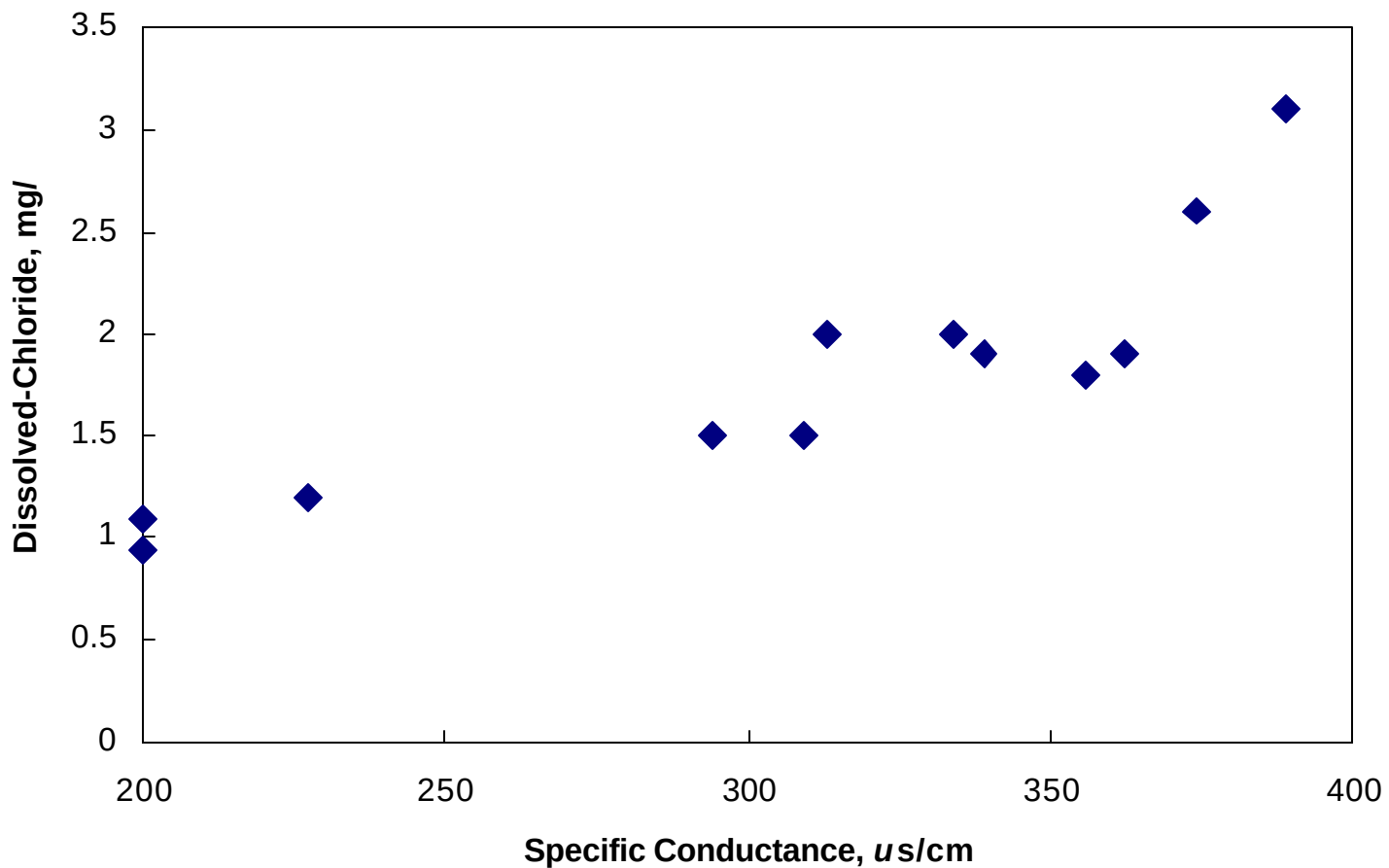
Dissolved Chloride Related to Specific Conductance Roaring Fork River near Emma - Water Years 1998-2000 Figure 4-D
