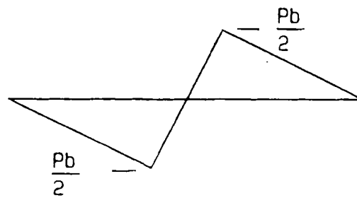
c. Moment Diagram
