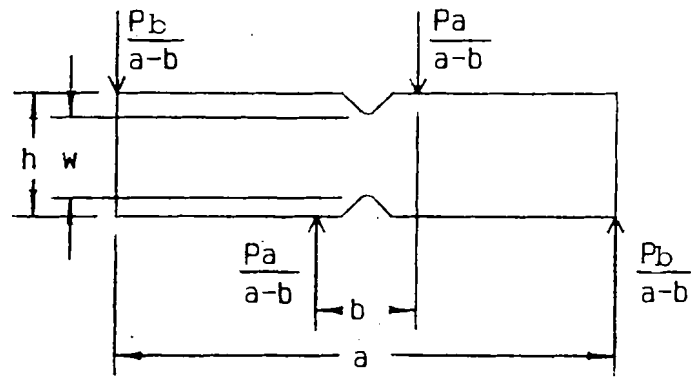
a. Force Diagram
