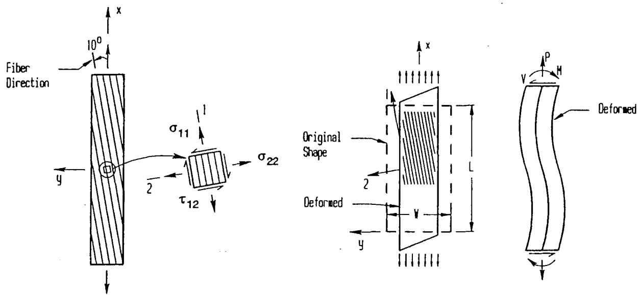
Local stresses in specimen originally suggested in [40]
