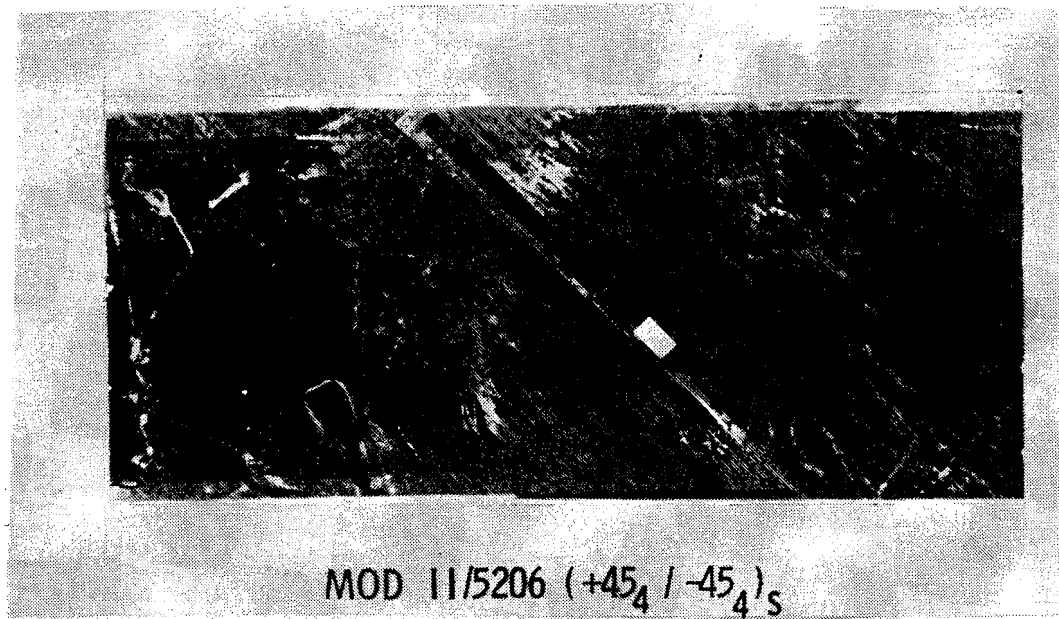
Figure 12. A Typical Undesirable Failure Mode due to Lumped Layup (45_4/-45_4)_s . Courtesy: D.W. Oplinger, FAA Technical Center
