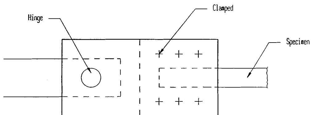
Hinged grip fixture [42,43,45]
