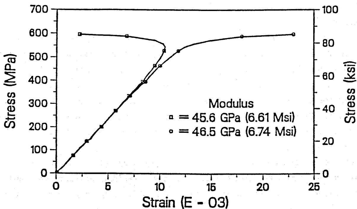
Figure 7. Suddenly Diverging Strain Gage Readings Indicating Buckling (32-Ply Unidirectional S2 Glass/3501-6 Epoxy Composite) [25]
