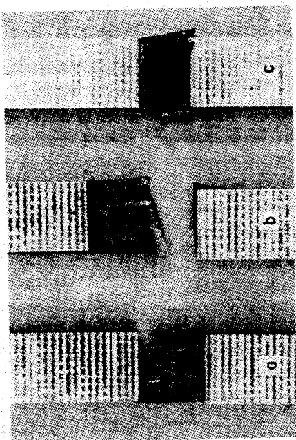
Failure modes of untapered glass/epoxy tabbed specimens: (a) branched transverse; (b) transverse; and (c) broomed
