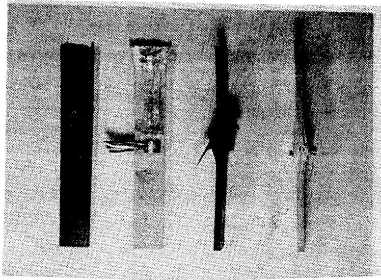
Figure 34. Typical Failures of Wyoming End-Loaded, Side-Supported Compression Test Specimens [25]
