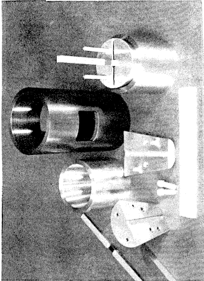
Fixture Components
