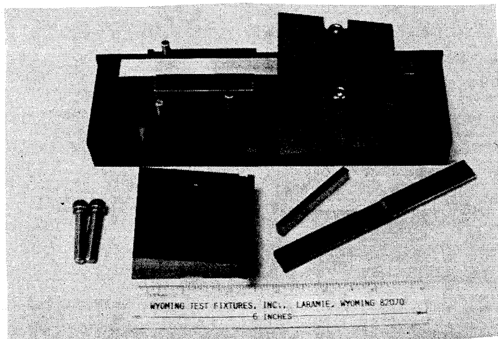
Figure 18. Specimen Installation Jig for Use with IITRI Compression Test Fixture, Showing Test Specimens, Alignment Bar, and End Loading Bar [9]
