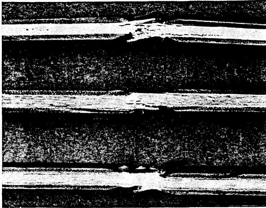
Figure 3. Typical Failures of Celanese Compression Test Specimens of Randomly Oriented, Short Glass Fiber/Epoxy Composites [6]
