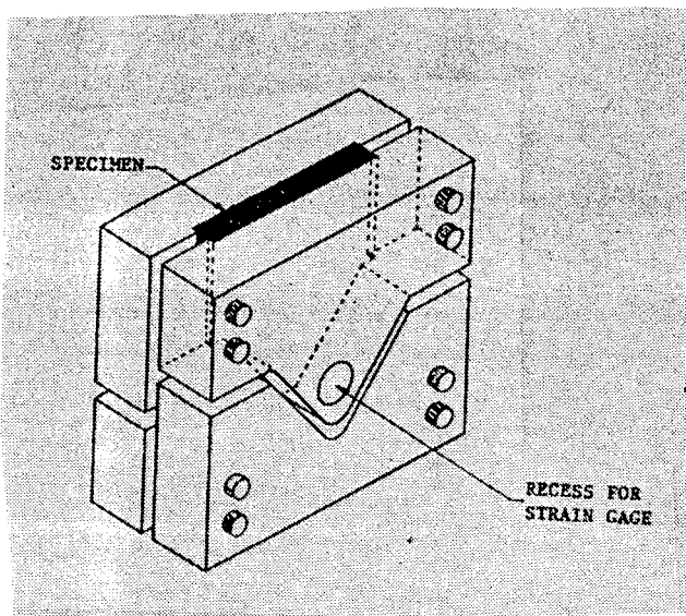
Northrop Compression Test Fixture [25]
