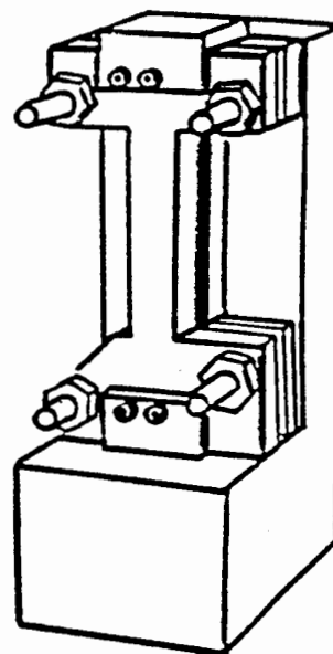
LOADING FIXTURE
