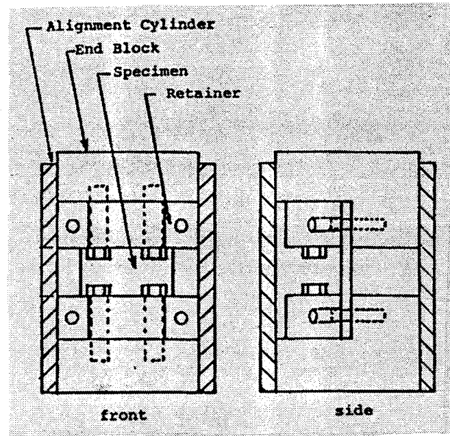
NASA End-Loaded Compression Test Fixture [39]
