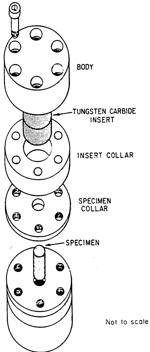
MODIFIED AXIAL COMPRESSION FIXTURE
