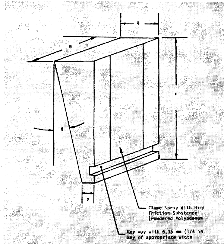
Figure 17. Detail of Wedge Design for Procedure B (IITRI) Test Fixture (Figure 3b of ASTM Standard D 3410-87 [1])
