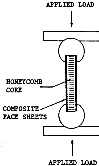
a) ASTM C 364 Edgewise Compression Test Fixture and Specimen [65]
