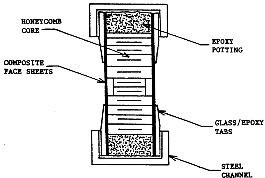
b) Convair Edgewise Compression Sandwich Test Specimen [25]
