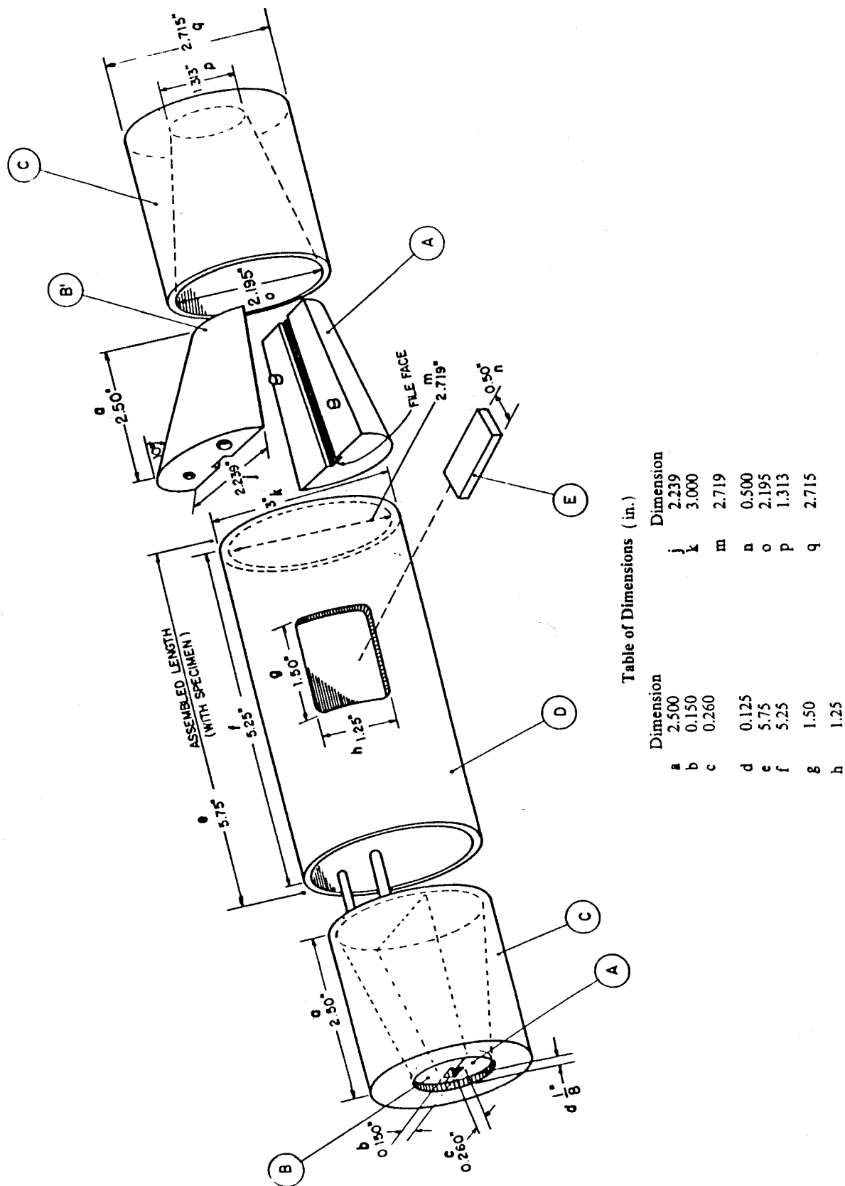
Figure 1. Celanese Compression Test Fixture [1]
