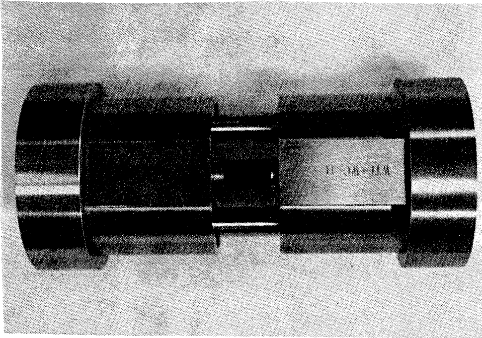
Assembled Fixture With Specimen
