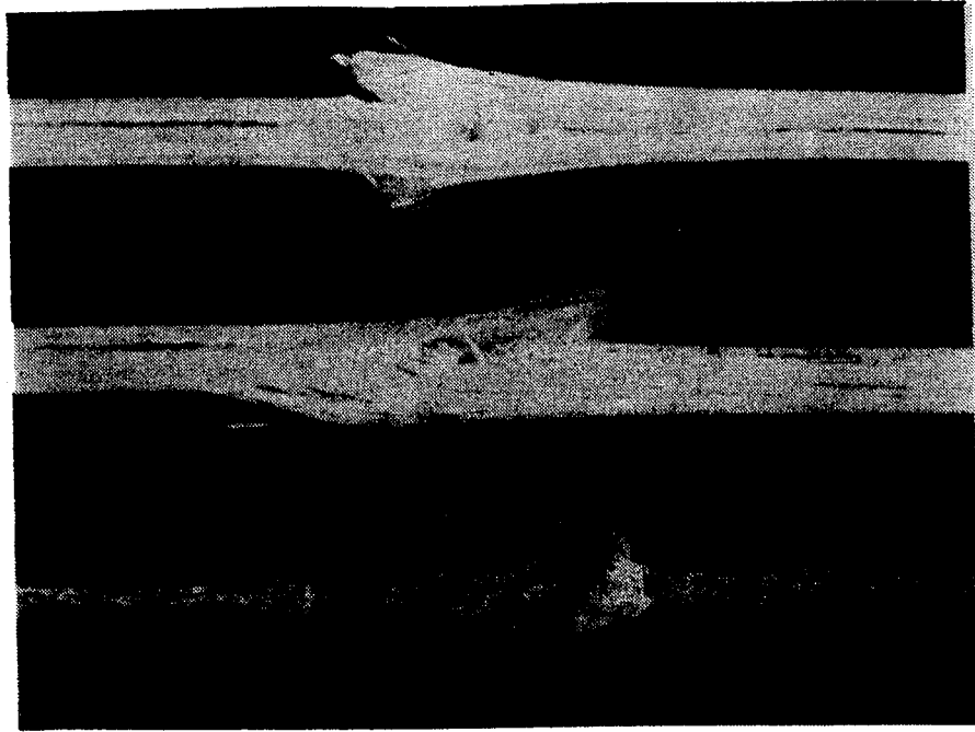
Figure 33. Failed Wyoming End-Loaded, Side-Supported Compression Test Specimens [6]
