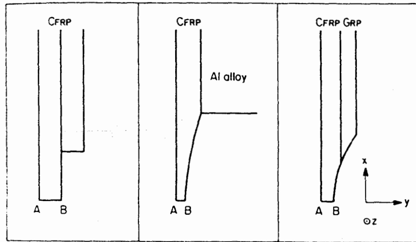
Modified D695 specimen
