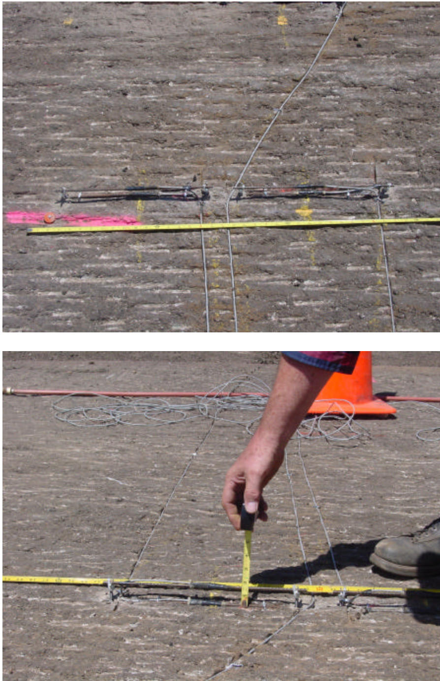
Figure 14. Embedded Strain Gages
