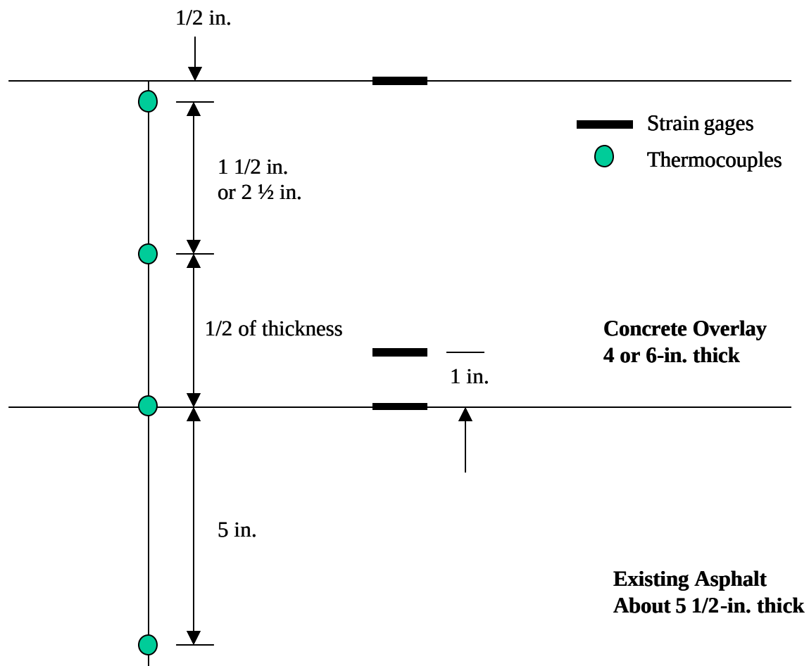
Figure 9 Typical Test Slab Layout -- Section View
