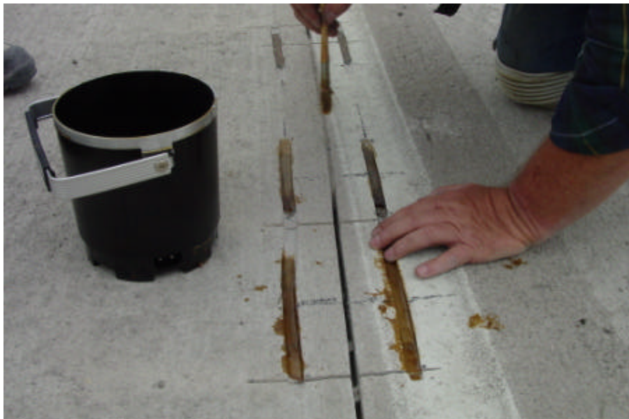
Figure 28. Applying Wax for Protection
