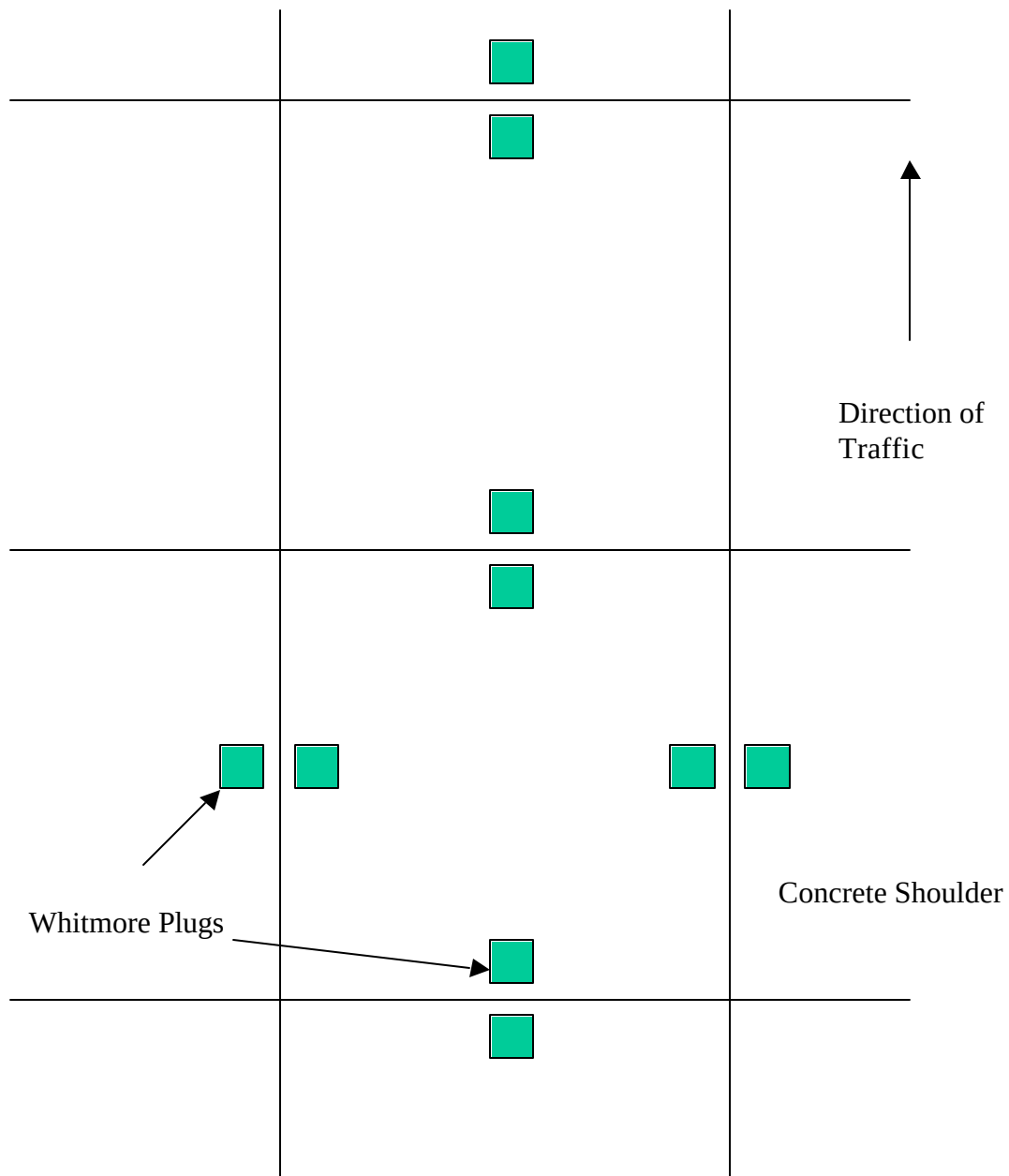
Figure 19 Typical Whitmore Plug Positions for Each Experimental Combination
