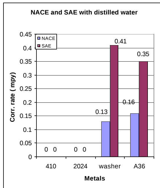
Fig. 2-9 Comparison of the SAE and SAE tests with distilled water
