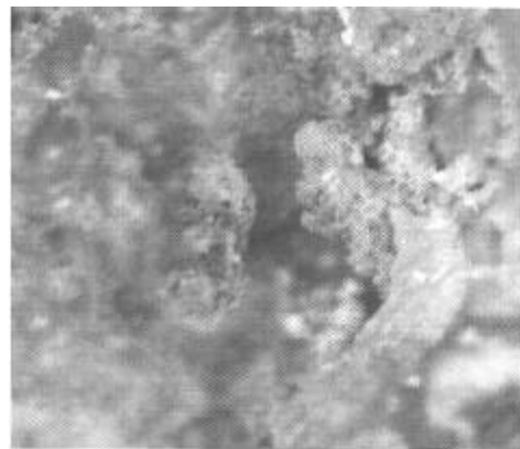
Figure 16b, SS410, \text{NaCl} , x150
