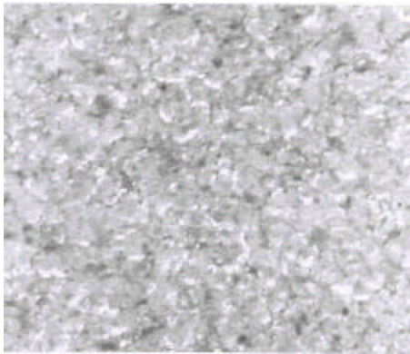
Figure 16g Al 5086, \text{MgCl}_2 , (x 150)
