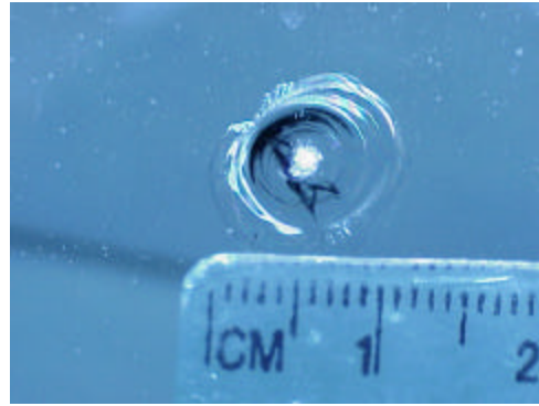
Fig 10 Conchoidal fracture
