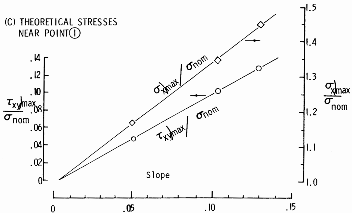
Figure 9. Predicted Maximum Stresses in "Bowtie" Specimen [2]
