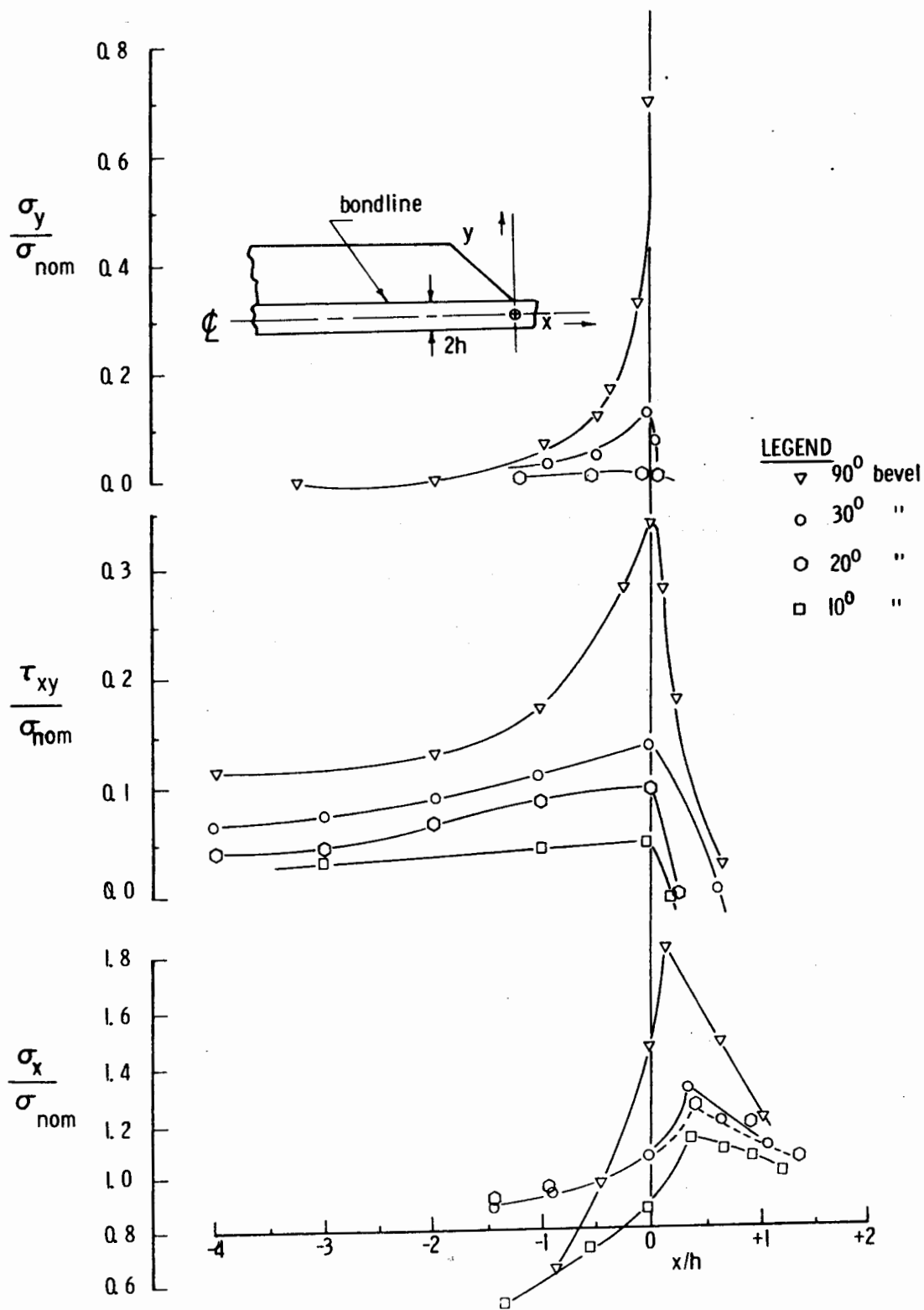
Figure 5. Theoretical Stresses in Tabbed Specimens [2]
