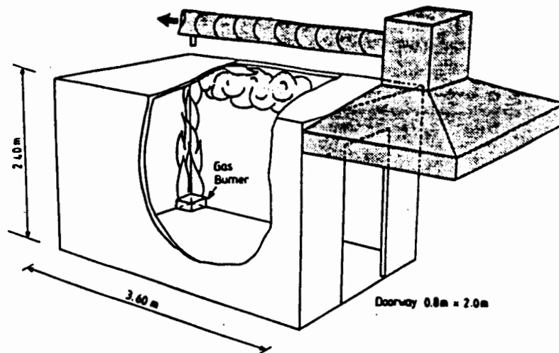
FIGURE 3. ROOM-CORNER TEST CONFIGURATION FROM SUNDSTROM (1986)
