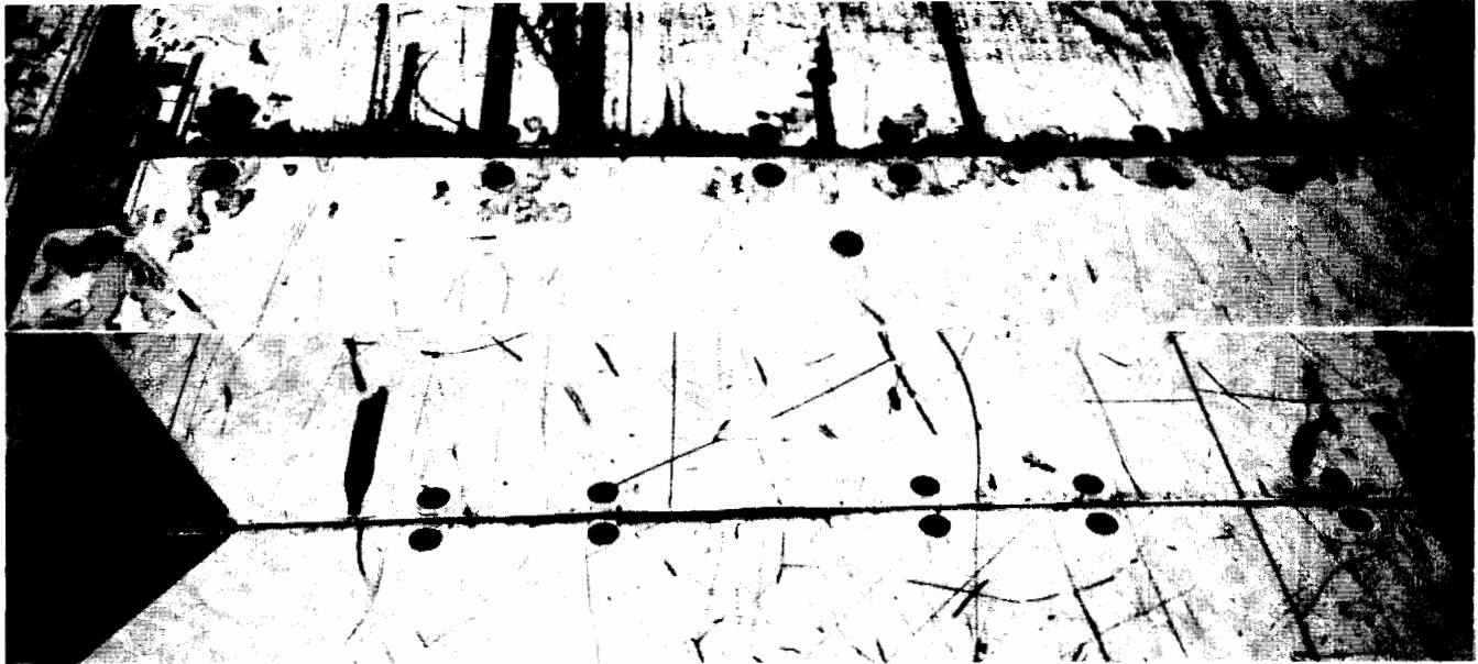
Figure 4. COMPARATIVE WEAR OF CARGO FLOOR PANELS IN SERVICE (1900 FLIGHTS) TOP: PHENOLIC UD PLIES ON HONEYCOMB CORE. BOTTOM: PEI/FABRIC ON H/COMB
