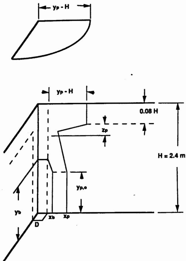
FIGURE 2. ILLUSTRATION OF PYROLYSIS AND BURN-OUT FRONTS
