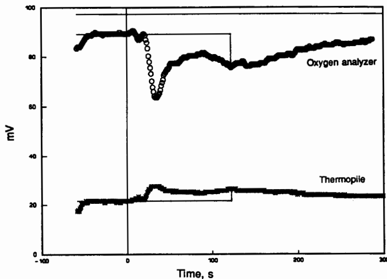
Fig. 4 Oxygen and thermal curves in an HRR measurement
