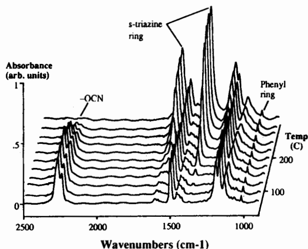
Figure 3: Curing of Low MW PT Resin (FTIR)
