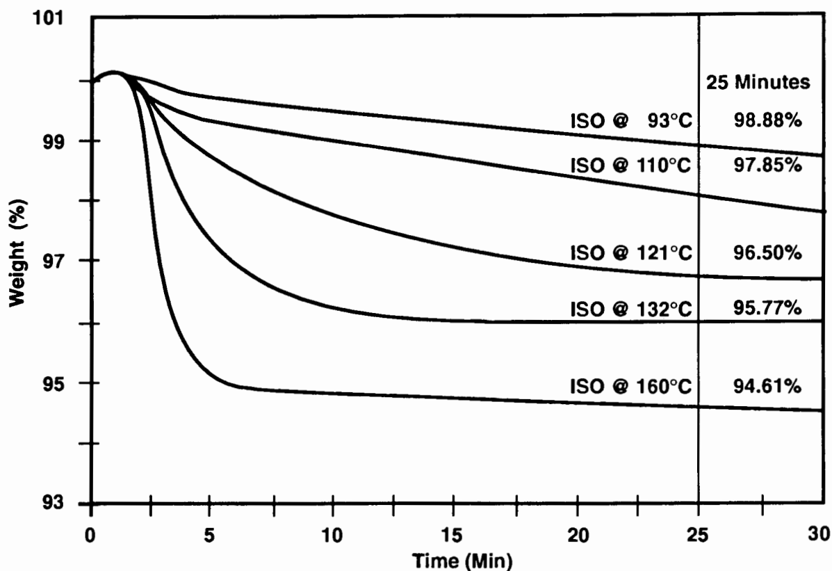
FIGURE 4: ISOTHERMAL THERMOGRAVAMETRIC ANALYSIS OF SPH 2400M/7781 AT VARIOUS TEMPERATURES.
