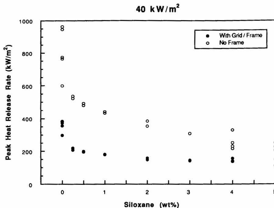
Figure 4. The effects of amount of siloxane on peak heat release rate of polycarbonate at external radaint flux of 40 kW/m 2 .
