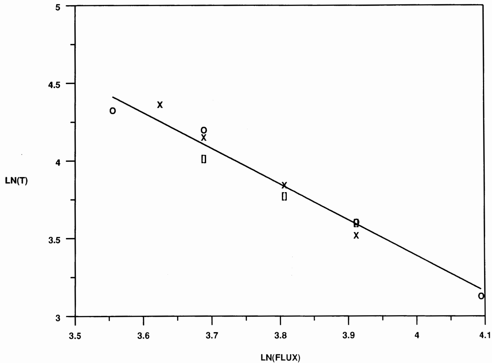
FIGURE 9. IGNITION TIMES CORRESPONDING TO DOSES OF 0 (O), 1.0 (X) AND 1.5 (□)
