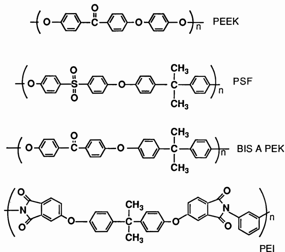
FIGURE 1: Engineering Thermoplastics Utilized Throughout This Study
