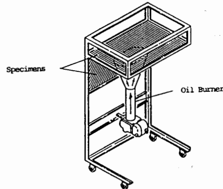
Figure 1 - Flame Penetration Resistance Test Apparatus
