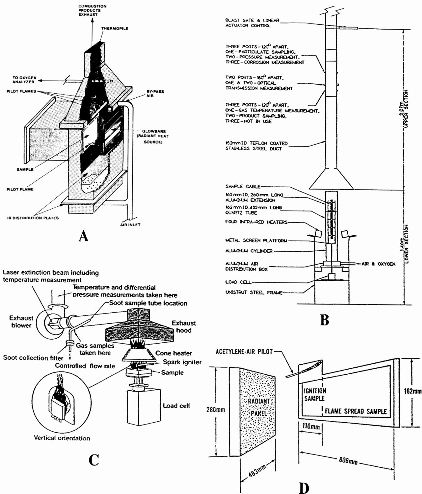
Figure 1. Heat Release and Flame Spread Apparatuses. (A): The OSU Apparatus; (B): The FMRC Apparatus; (C): The Cone Calorimeter; (D): The LIFT Apparatus.
