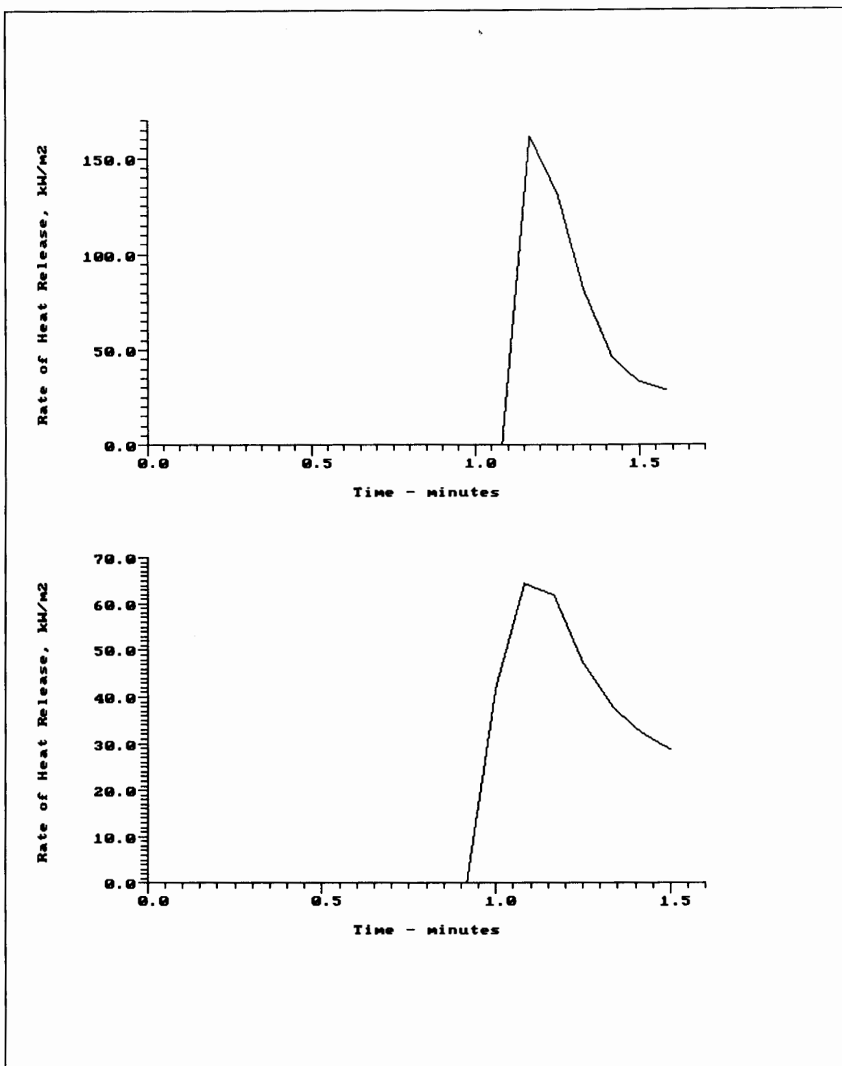
Figures 7 and 8. Measured rhr at 40 kW/m 2 for honeycomb panels before and after heat treatments. The tail extending beyond 1.5 minutes indicates a second stage in the combustion of these materials.
