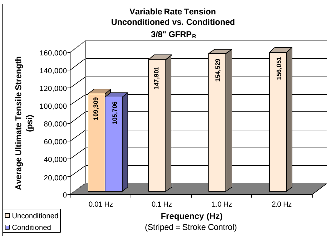
Figure 33: Variable Rate Tension 3/8" GFRP R
