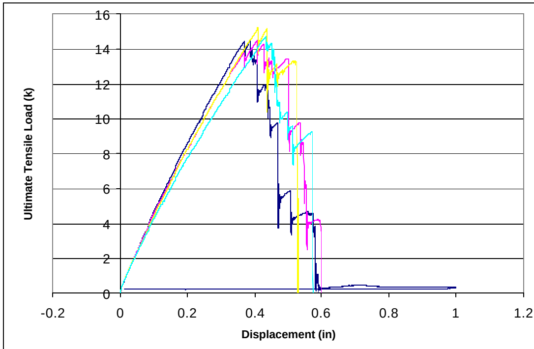
Figure 41: Linear behaviour with a non-linear region of cyclic load reductions after failure.
