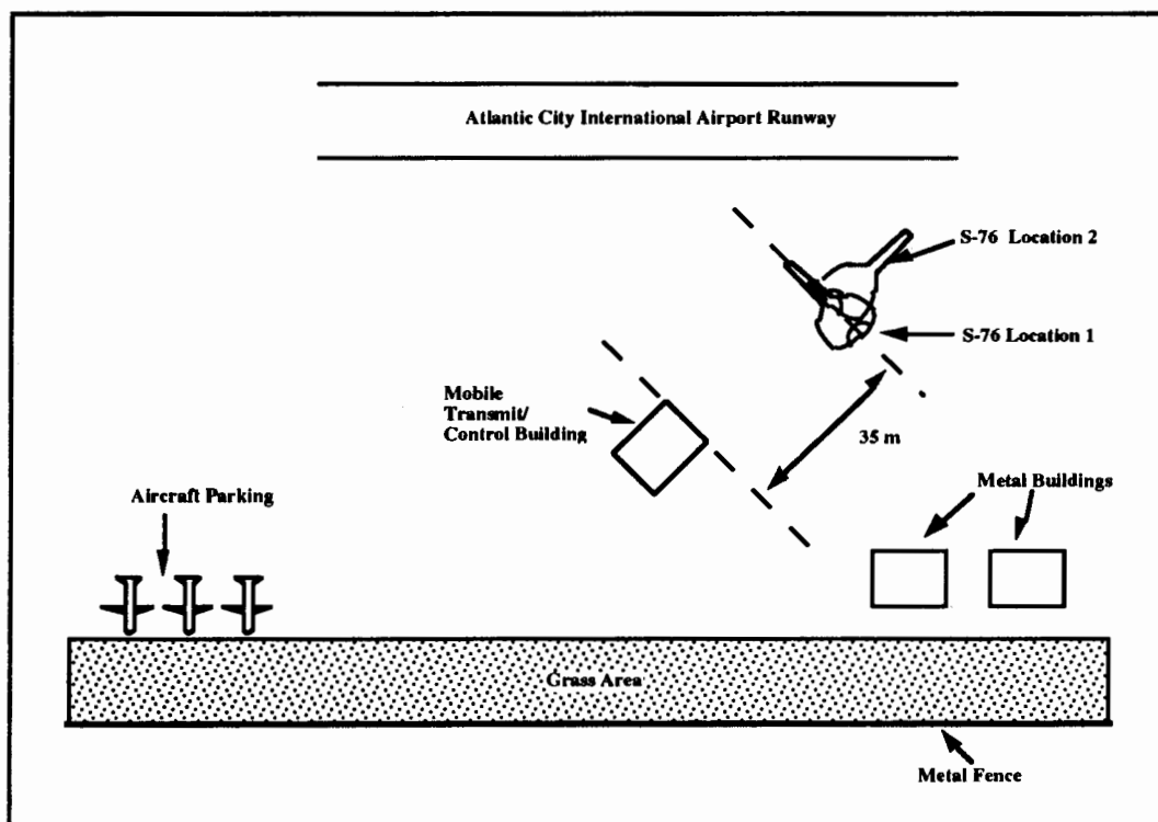
Figure 4-12. Test Area Layout
