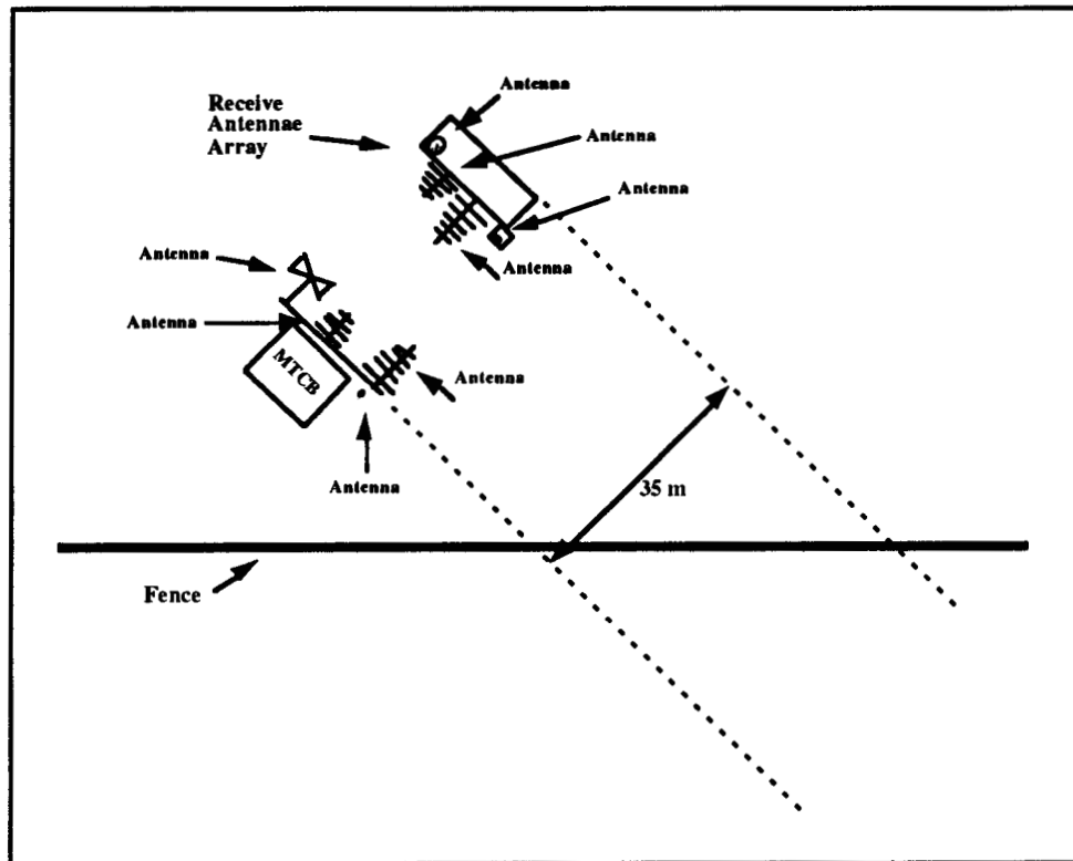
Figure 4-5. SCAL Configuration
