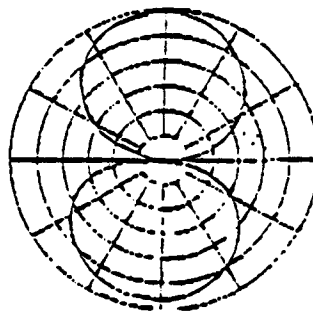
HORIZONTAL POLARIZATION
