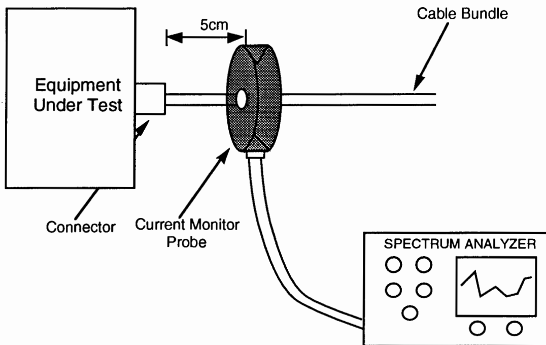
Figure 4-16. Current Monitor Probe Configuration
