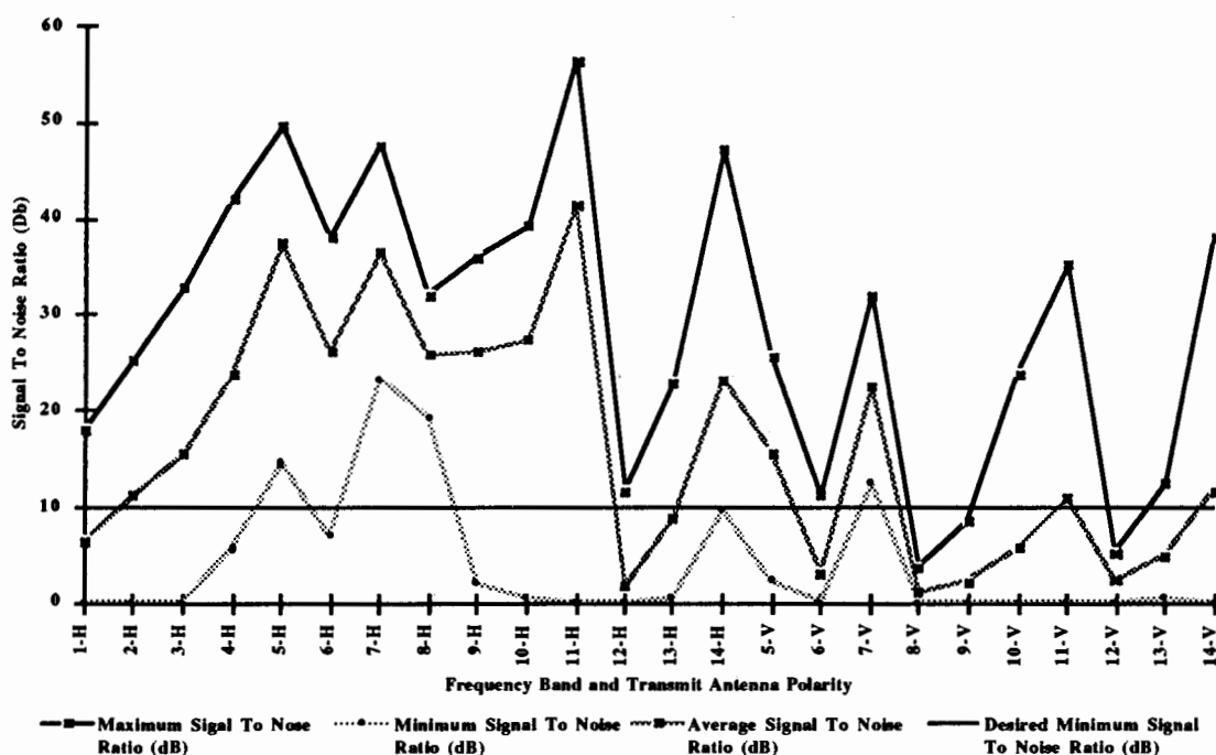
Figure 4-7. SCAL Set 1 SNR Chart
