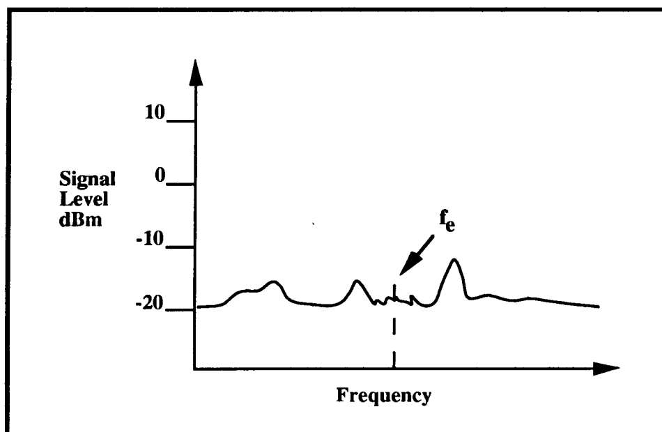
Figure 6-4. SCAL Signals Without Local Transmitter
