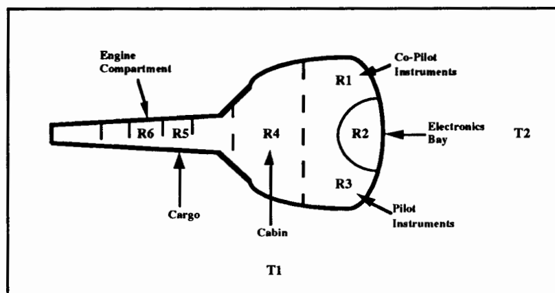
Figure 4-11 S-76 LLSF and LLSC Transmit/Receive Locations
