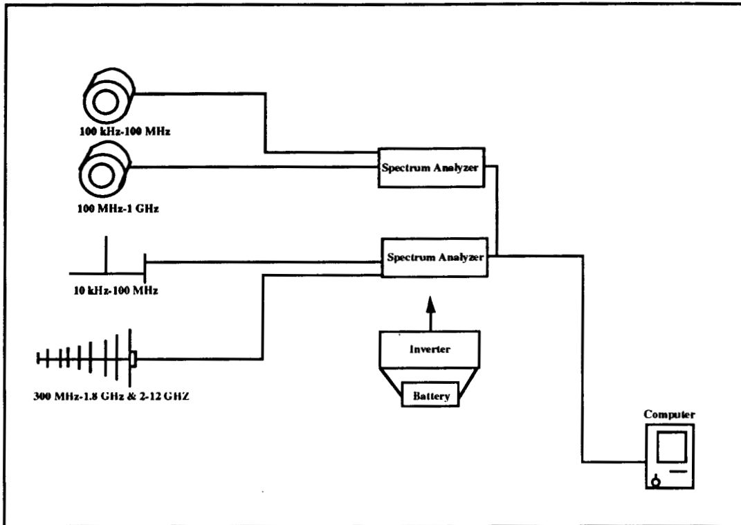
Figure 5-1. Flight Test Receive and Control Node
