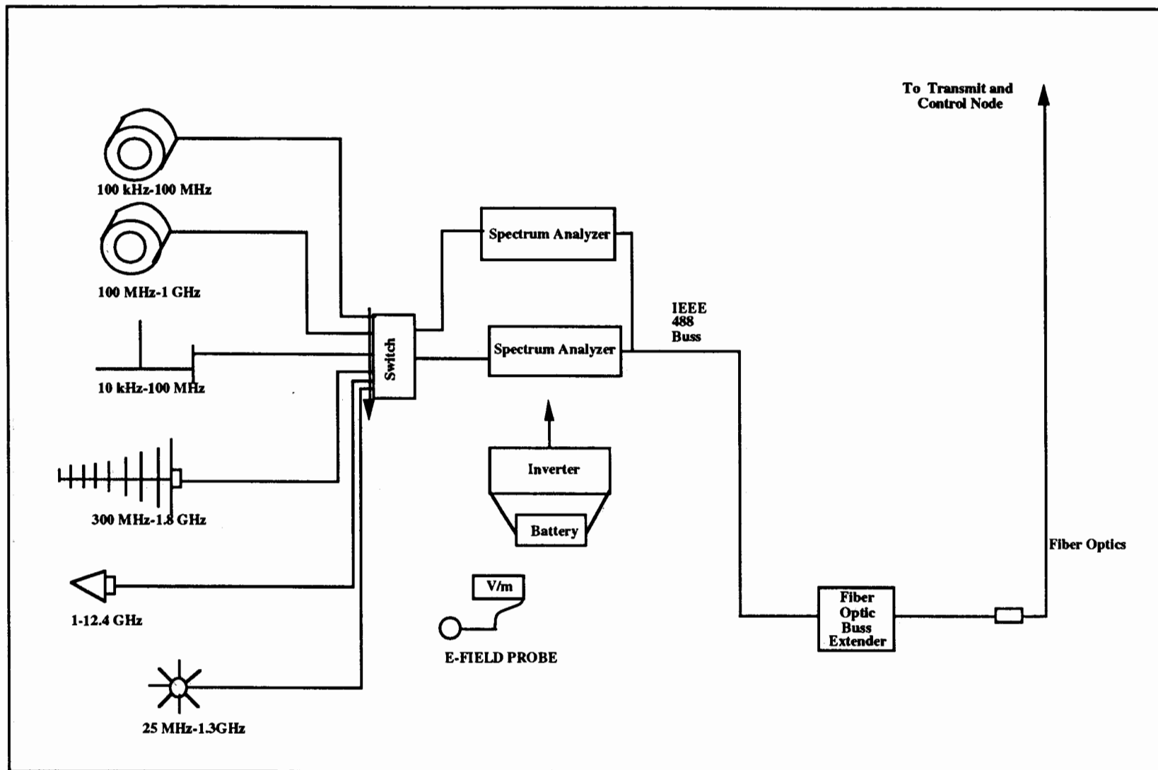
Figure 4-2. Test system Receive Node
