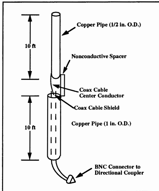
Figure 6-1. Bazooka Dipole
