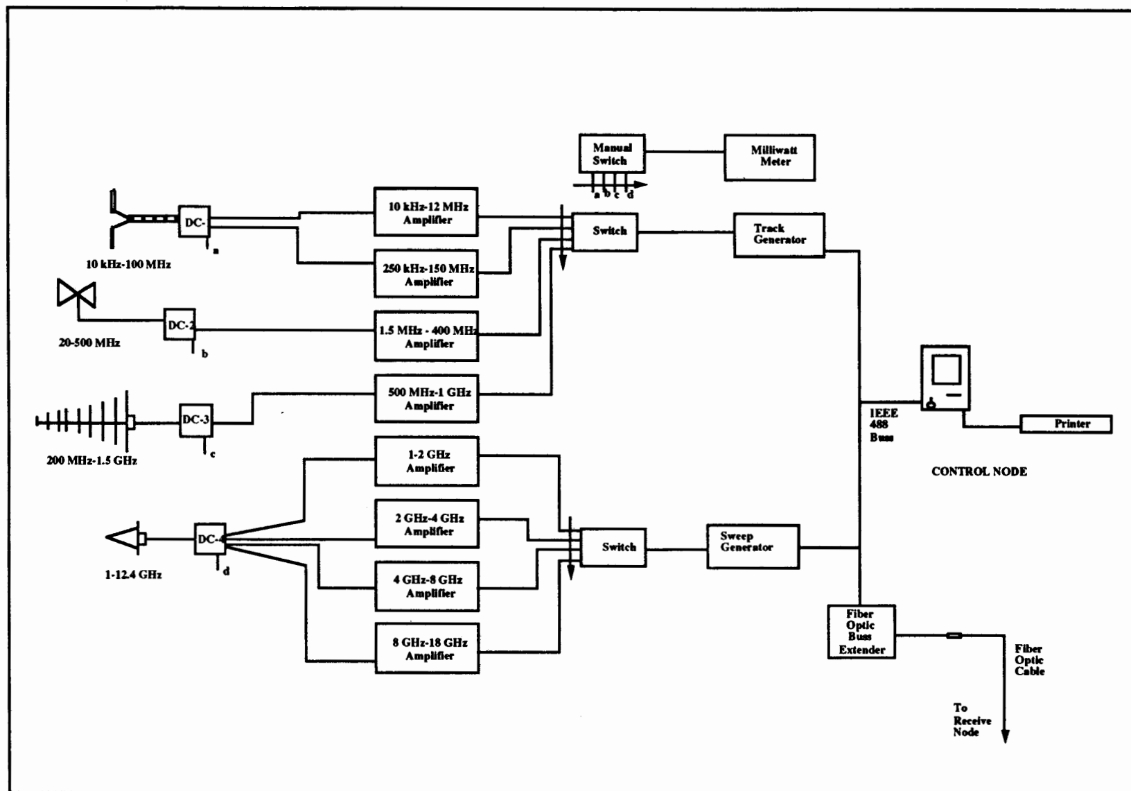
Figure 4-4. Test System Transmit and Control Node
