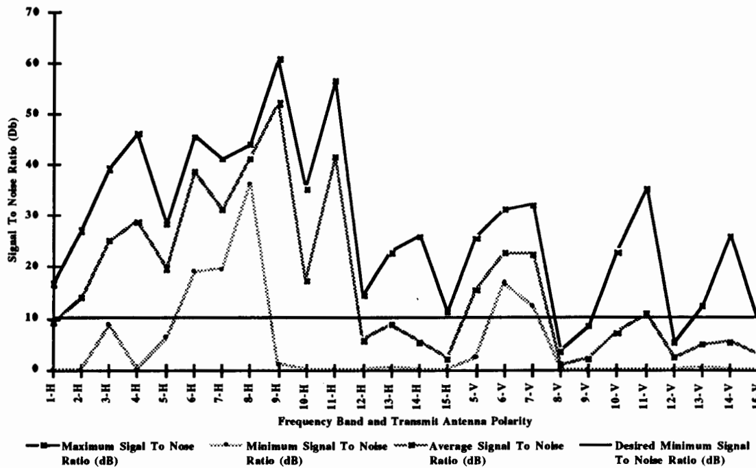
Figure 4-8. SCAL Set 2 SNR Chart
