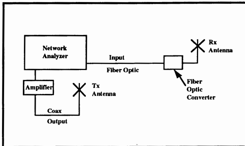
Figure 6-10. Network Analyzer Synchronized Sweep Configuration
