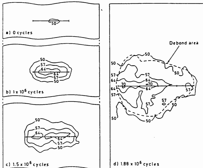
FIGURE 3-12. SPATE STRESS PATTERNS SHOWING VARIATION OF PATCH STRESSES IN FIBER DIRECTION DURING FALSTAFF LOADING
