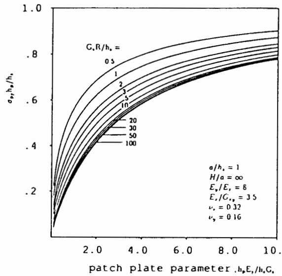
FIGURE 2-22. PATCH STRESS \sigma_{yy}^p AS A FUNCTION OF PATCH-STIFFNESS AND ADHESIVE FLEXIBILITY
