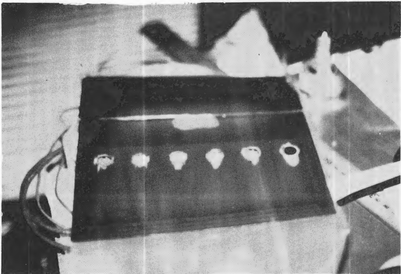
FIGURE 5-3. LAP JOINT DOUBLER SHOWING SHEAR PUNCHED HOLES
