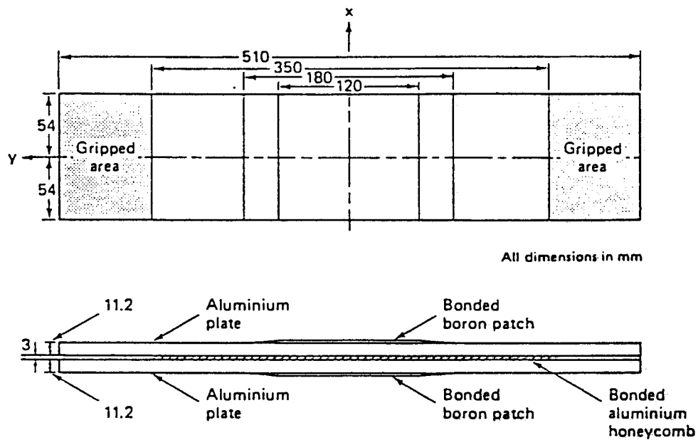
FIGURE 3-7 TEST GEOMETRY FOR THE SURFACE FLAW SPECIMEN
