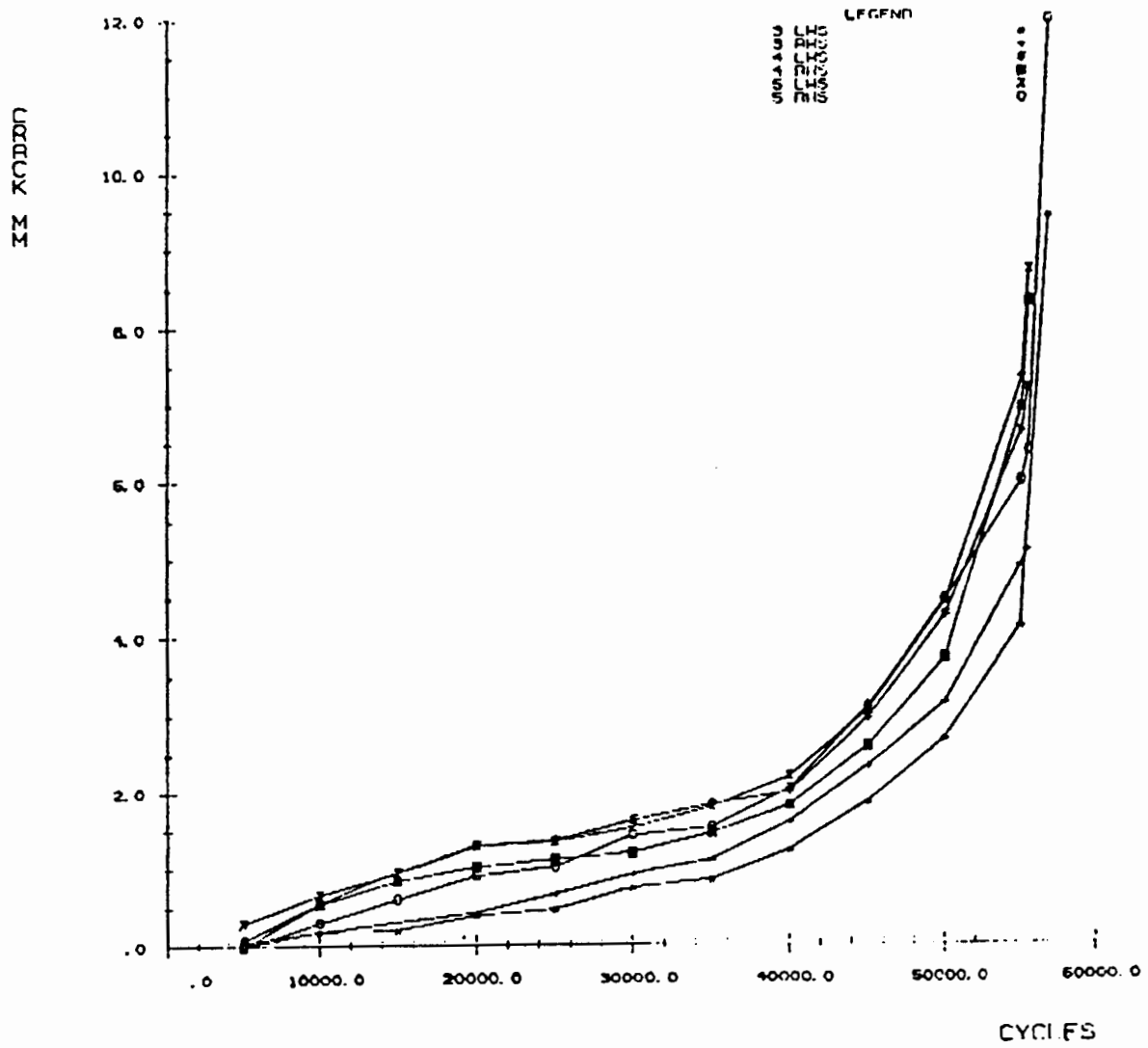
FIGURE 4-14. SPECIMEN A15 CRACK GROWTH DATA
