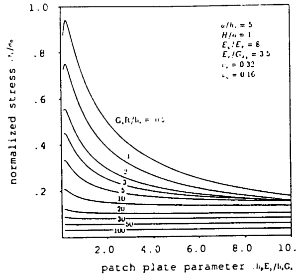
FIGURE 2-33. ADHESIVE SHEAR AT x=0 , y=0 AS A FUNCTION OF ADHESIVE FLEXIBILITY AND PATCH STIFFNESS
