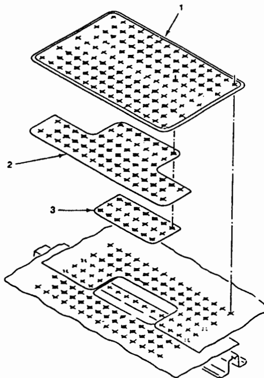
FIGURE 4-1. TYPICAL LAP JOINT FASTENED REPAIR
