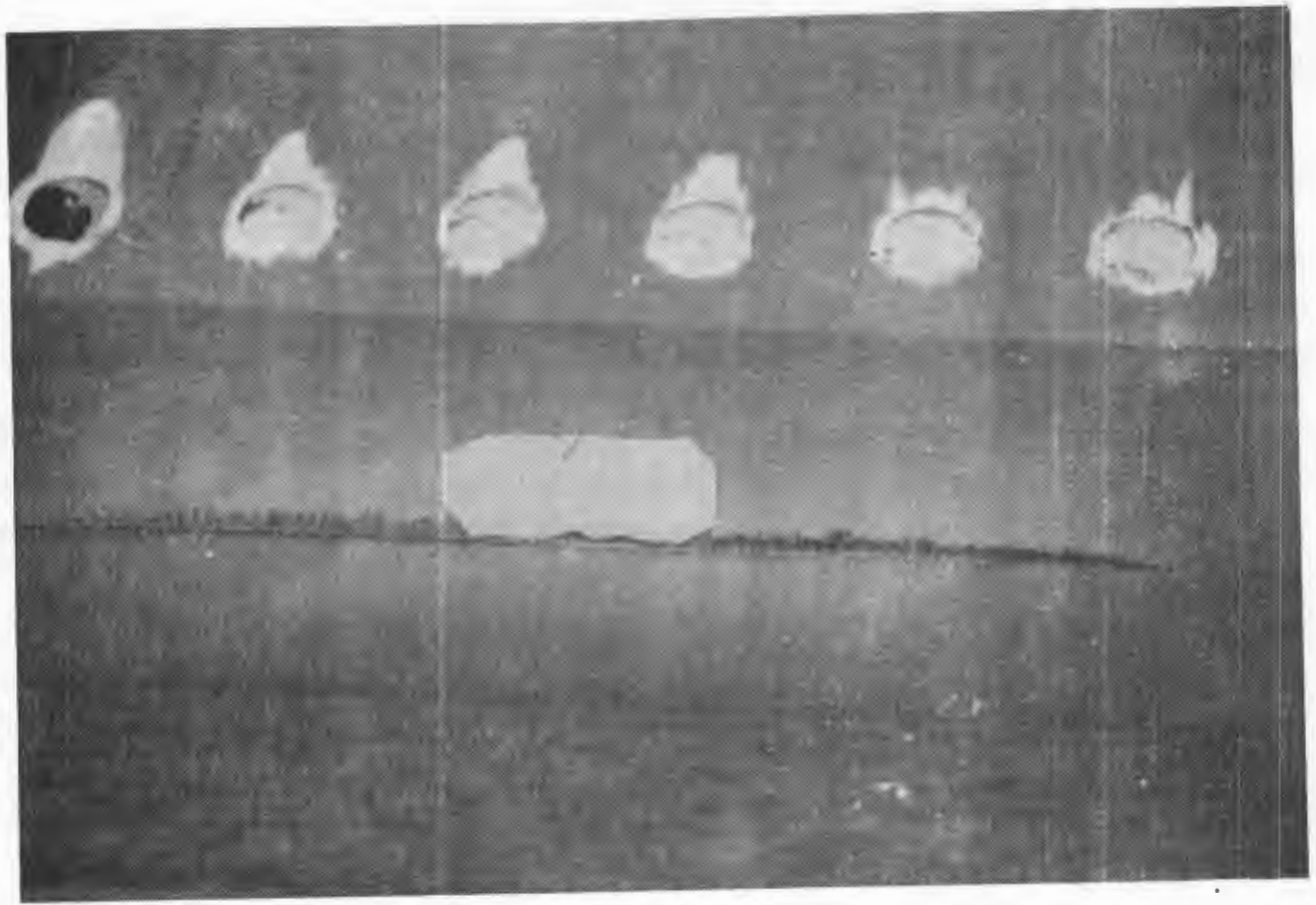
FIGURE 5-4. LAP JOINT DOUBLER TEFLON INSERT
