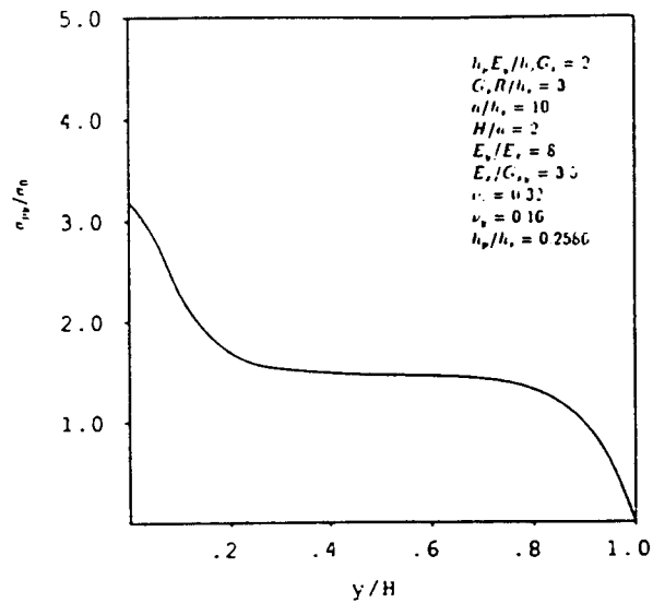
FIGURE 2-37. VARIATION OF PATCH TENSILE STRESS ALONG THE HEIGHT OF THE PATCH
