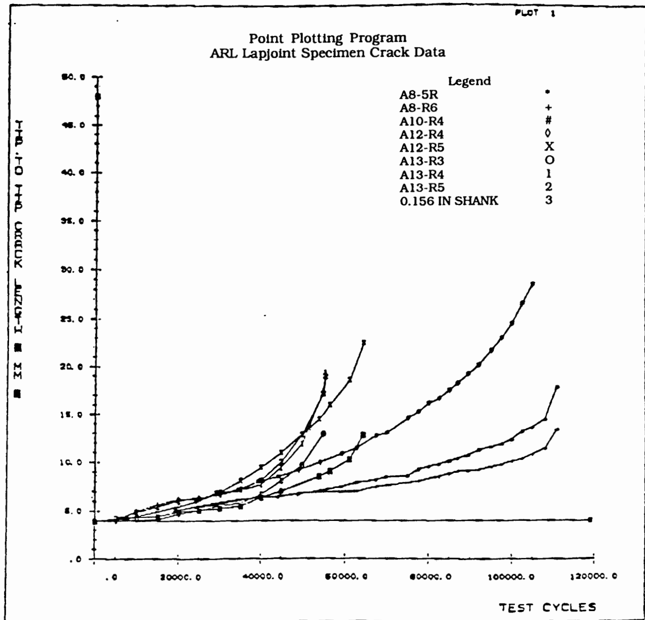
FIGURE 4-22. TEST CRACK GROWTH DATA
