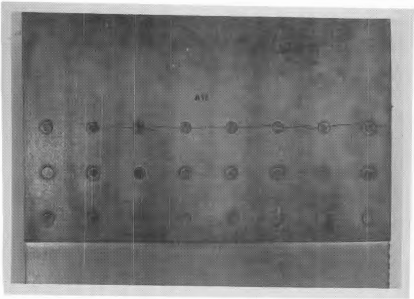
FIGURE 4-17. FAILURE OF SPECIMEN A12
