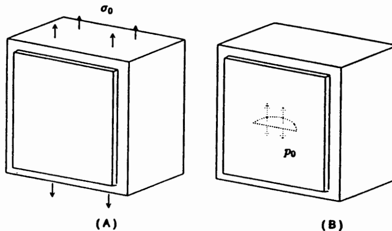
FIGURE 2-65. LINEAR SUPERPOSITION OF TWO PROBLEMS
