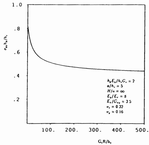
FIGURE 2-15. PATCH STRESS AT x=0, y=0 AS A FUNCTION OF ADHESIVE FLEXIBILITY
