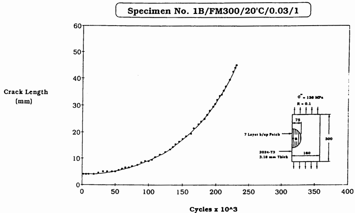
FIGURE 3-1. FATIGUE CRACK LENGTH FOR SPECIMEN 1B
