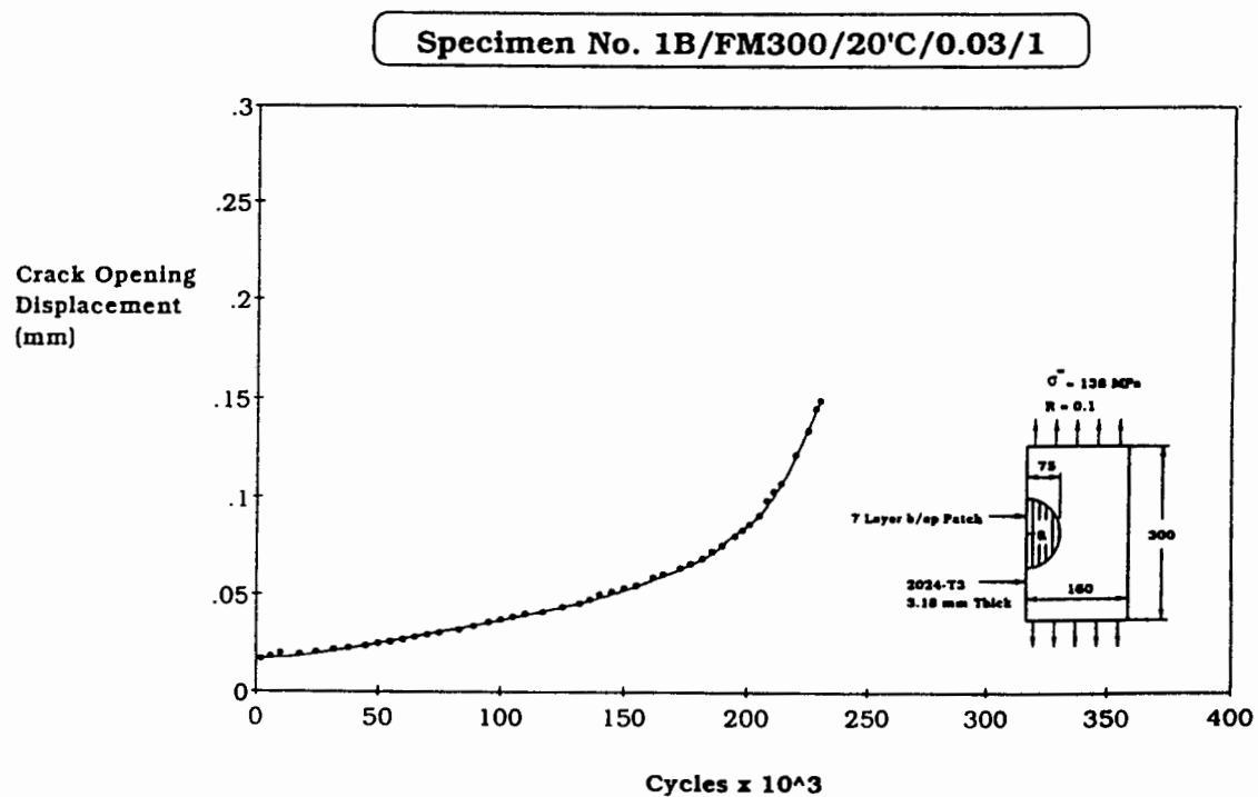
FIGURE 3-2. FATIGUE CRACK OPENING DISPLACEMENT FOR SPECIMEN 1B
