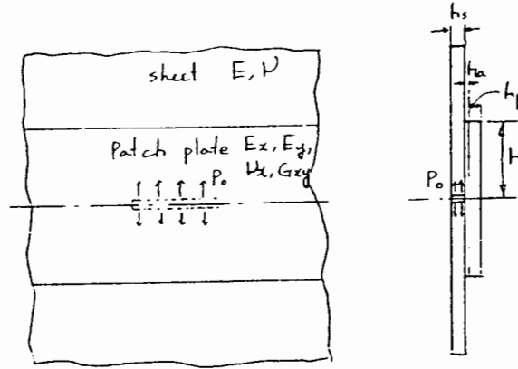
FIGURE 2-3. CRACKED METAL SHEET WITH A COMPOSITE PATCH LOADED ON THE CRACK FACE (PROBLEM B)
