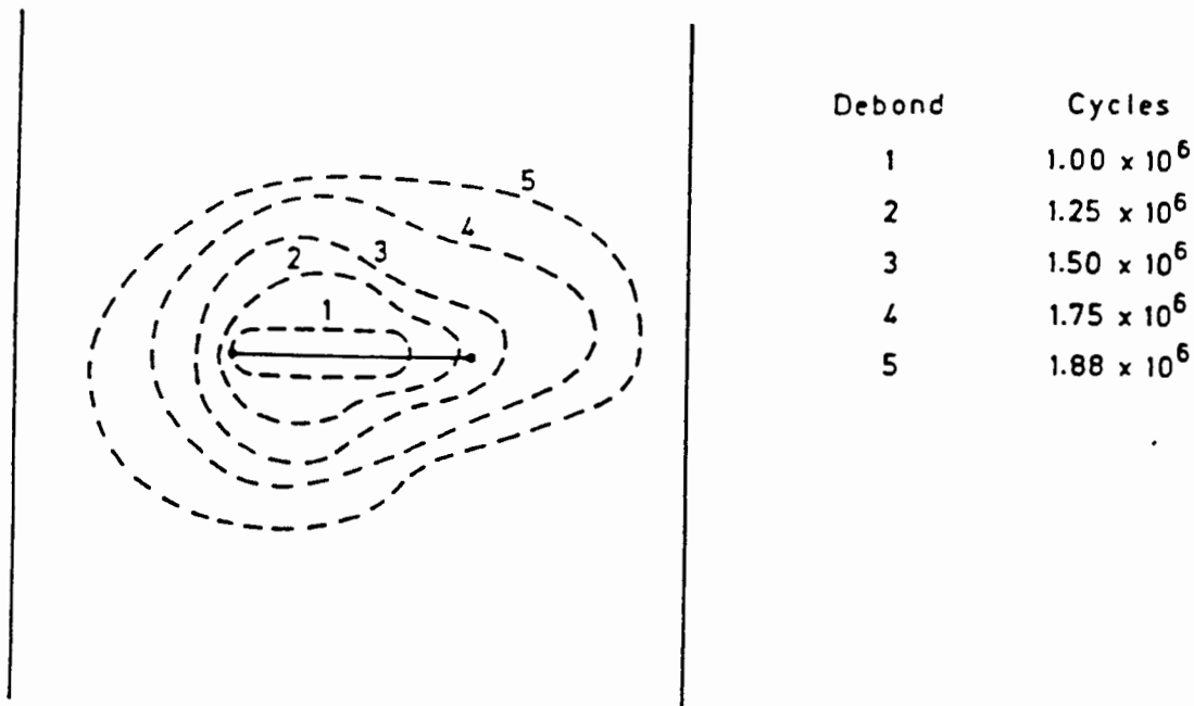
FIGURE 3-13. DEVELOPMENT OF DEBOND DURING FALSTAFF LOADING (SPECIMEN 16/17P)
