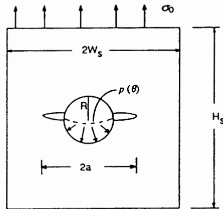
FIGURE 2-58. A FINITE PLATE WITH A HOLE, SUBJECT TO FAR-FIELD LOADING AND PIN-LOADING
