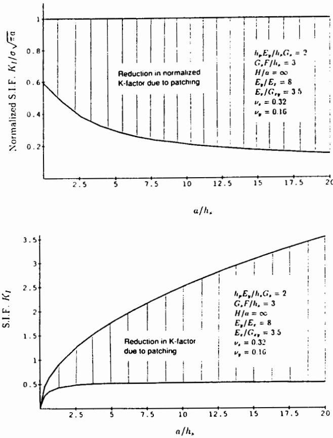
FIGURE 2-8. REDUCTION IN: (a) NORMALIZED S.I.F. DUE TO PATCHING AS A FUNCTION OF THE CRACK LENGTH; (b) THE ACTUAL S.I.F. (FOR \sigma_0=1 ) DUE TO PATCHING AS A FUNCTION OF THE CRACK LENGTH
