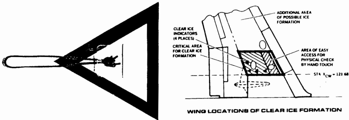
Figure 11 - VITACHROME (Tuft and Decal)
