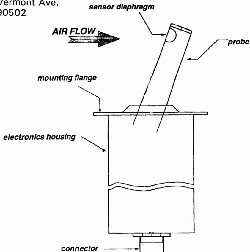
Figure 6 - VIBRO-METER (Model EW134)
