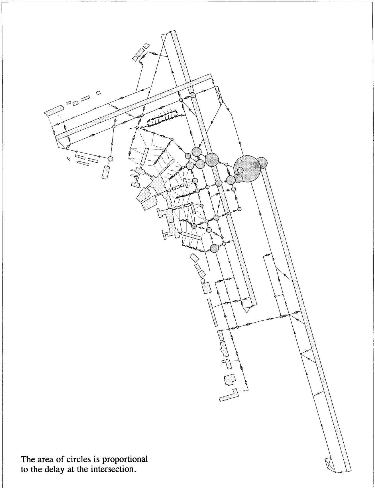
Fig. 3-3 Runway/Taxiway Crossing Delay for PHL Multiple Crossings Configuration
