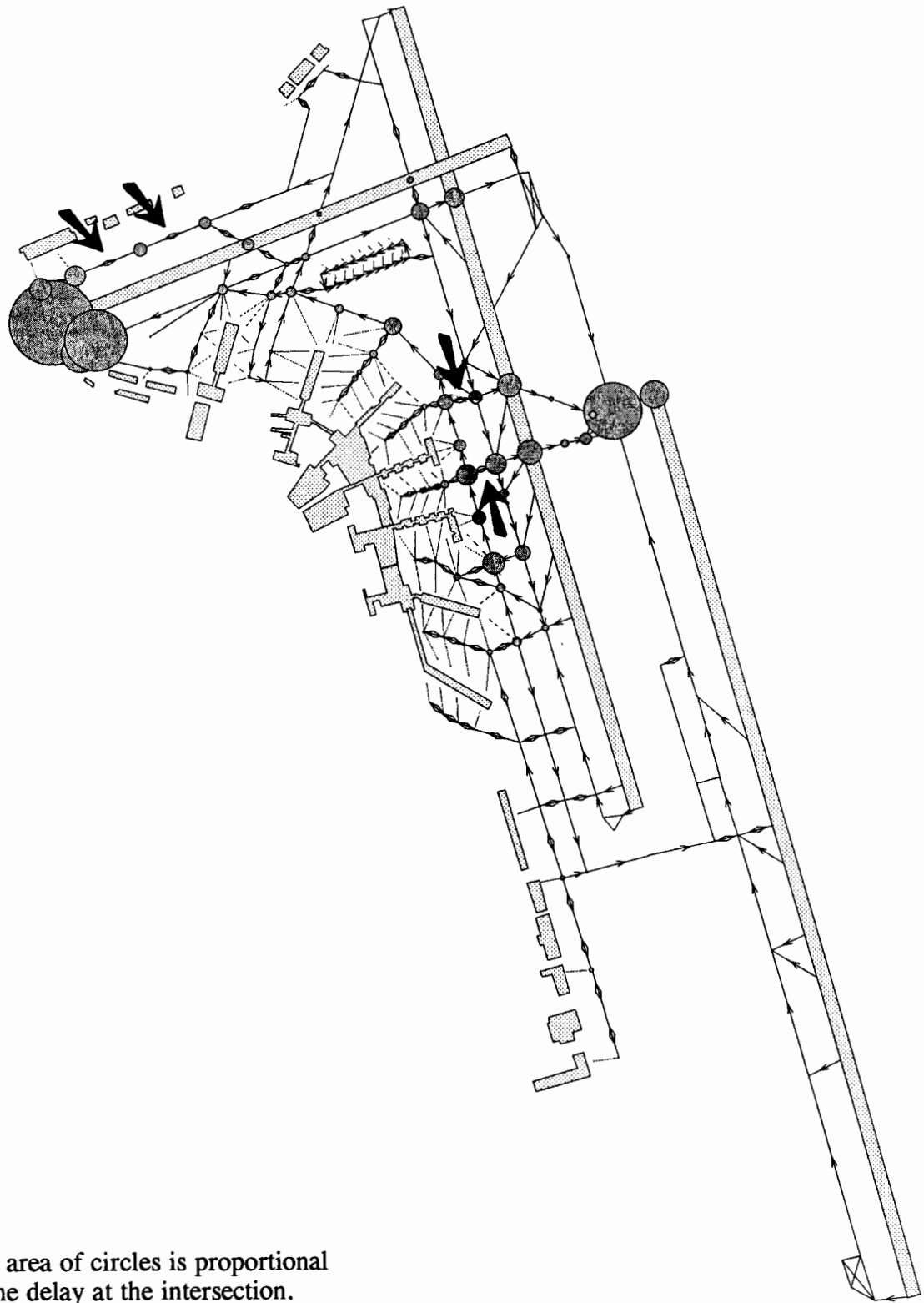
Fig. 7-1 PHL Runway and Taxiway Delay with Dual Lane Taxiways
