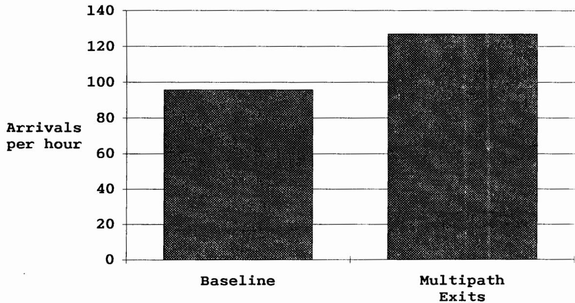
Fig. 5-6 JFK Capacity Improvement Due to Multipath Runway Exits
