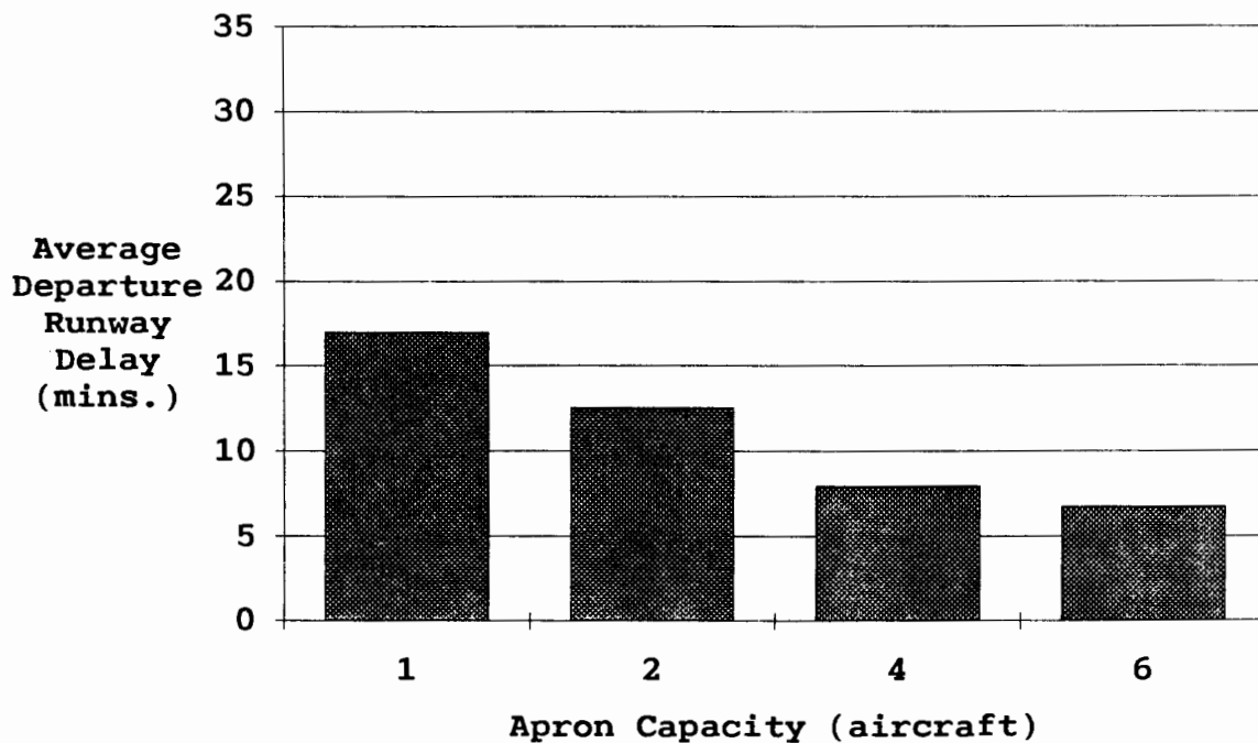
Fig. 4-2 IAD Delay Reduction Due to Multiple Departure Queues
