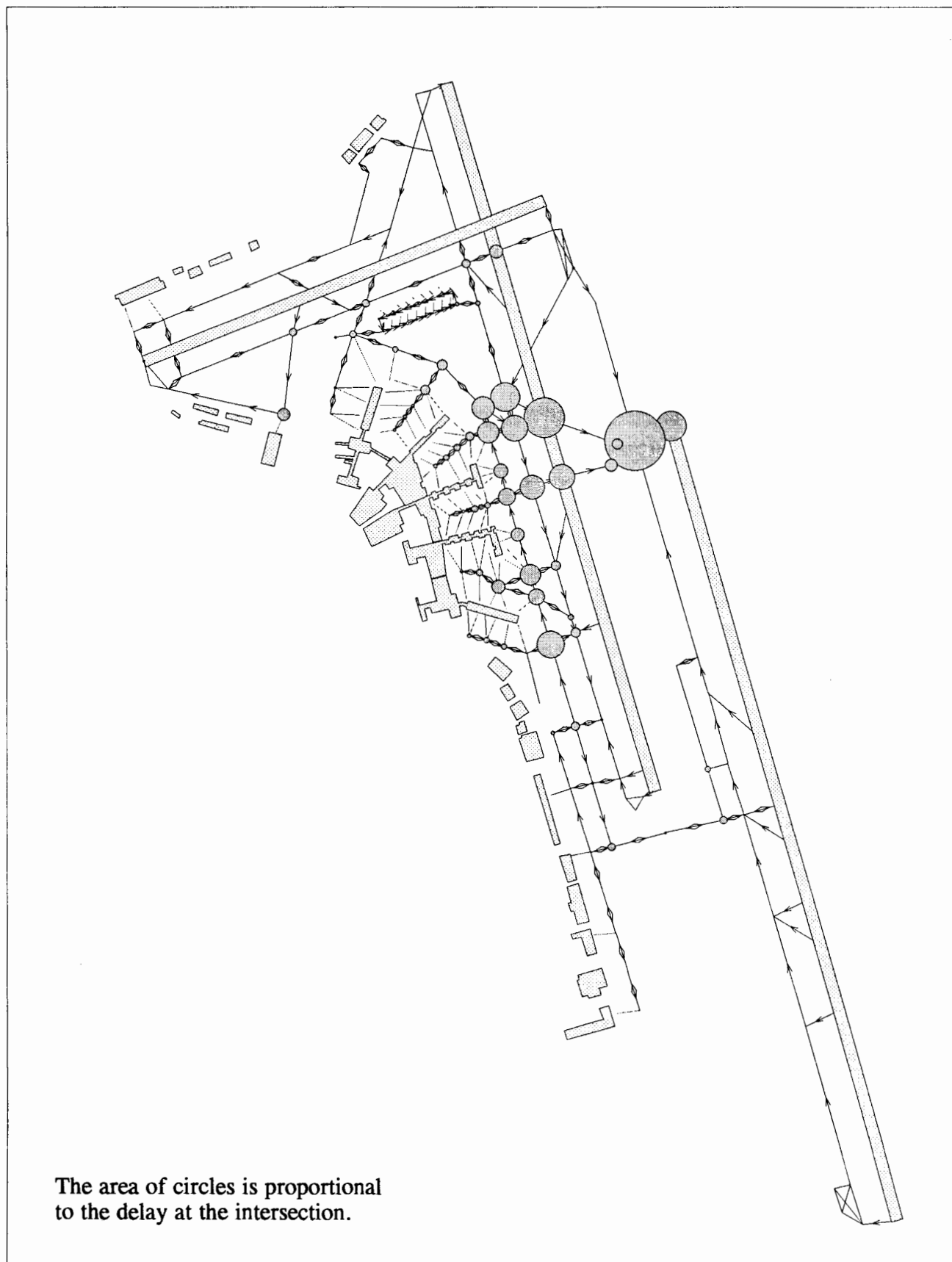
Fig. 3-2 Runway/Taxiway Crossing Delay for PHL Baseline Configuration
