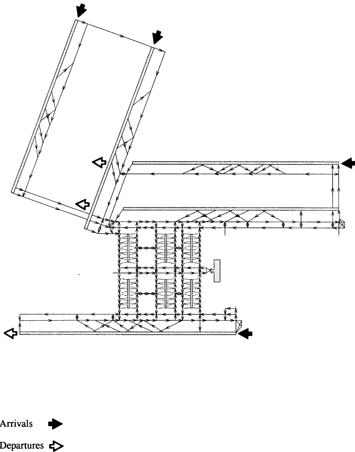
Fig. 6-4 IAD without Multipath Taxiways to/from Gates
