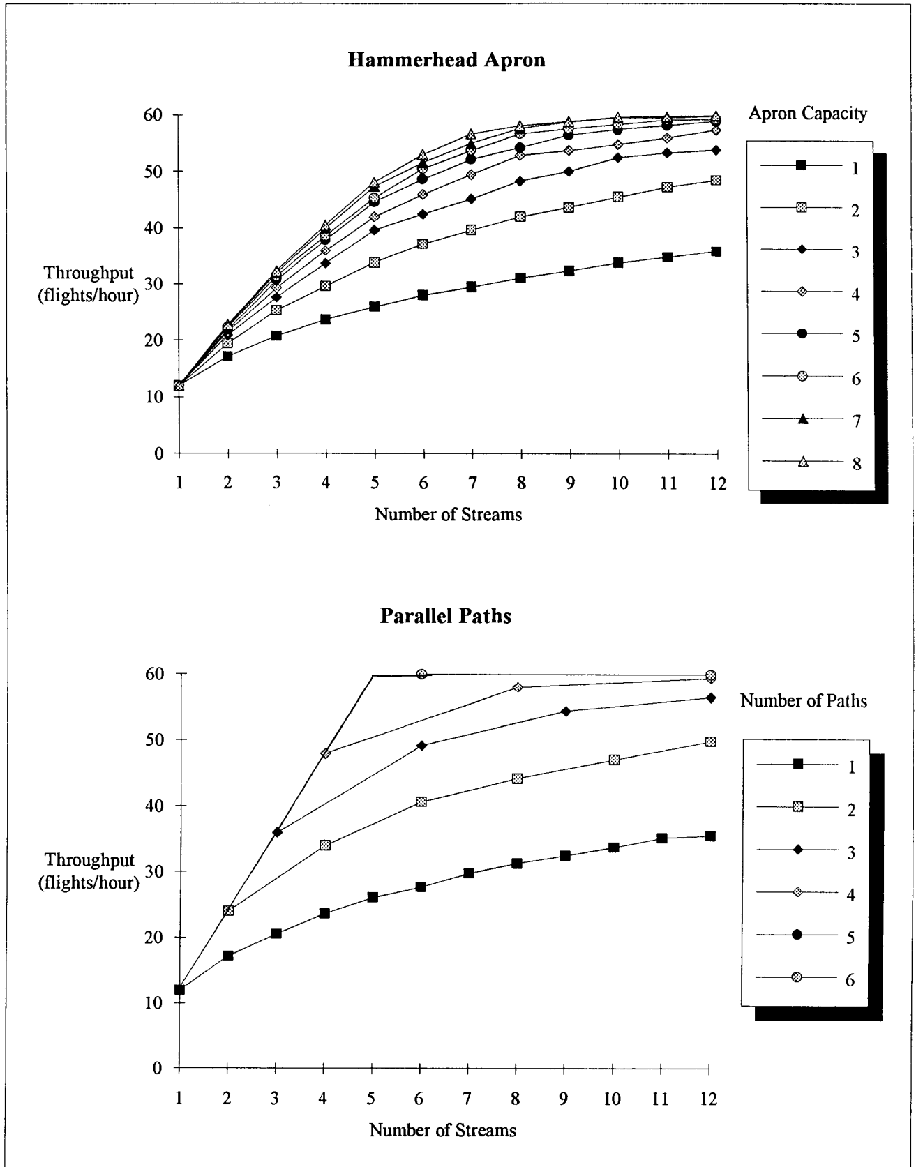
Fig. 4-1 Multiple Departure Queue Parameter Sensitivity
