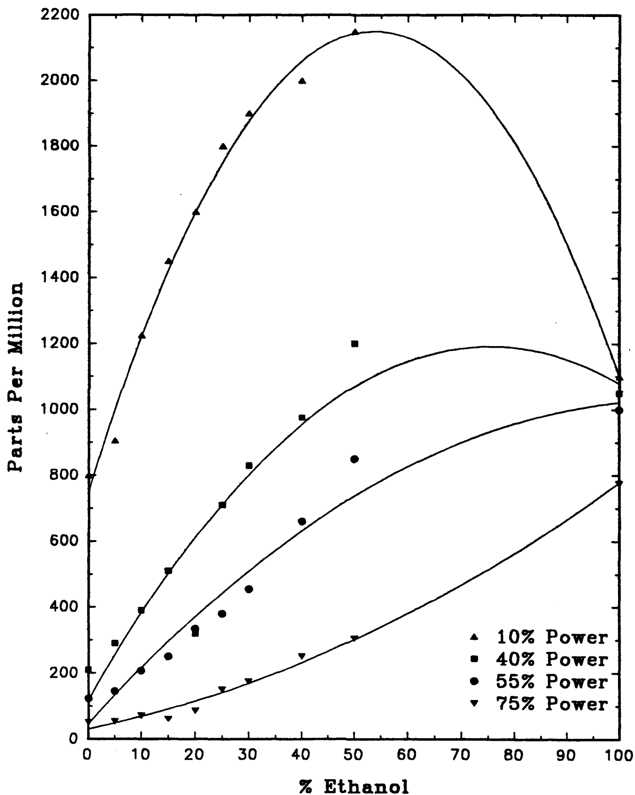
FIGURE 6. Effect of Ethanol Concentration on Exhaust Hydrocarbons at Constant Fuel Flow Rate
