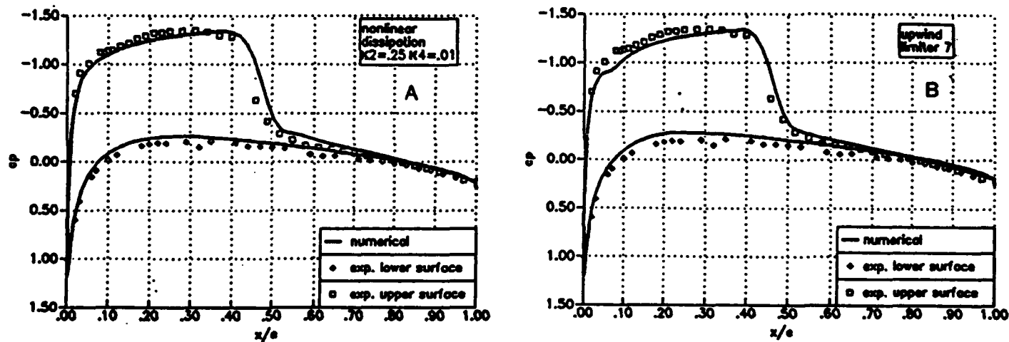
Fig. 7 Comparison of Experimental and Computational Pressure Distributions for NACA 0012 Airfoil Section, \alpha = 3.02^\circ , M = 0.752 , Re = 9.0 \times 10^6 , A. Explicit MacCormack Scheme with Non-linear Dissipation B. Explicit MacCormack Scheme with Upwind TVD Dissipation
