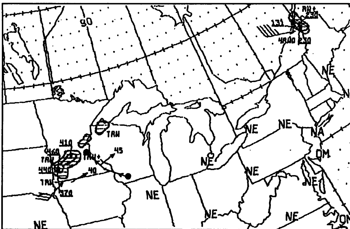
Figure 25. Radar Summary, 1635Z 27 JUN 1991.
