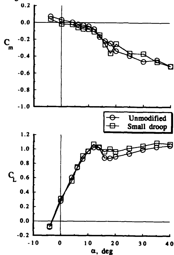
Figure 10. Longitudinal characteristics, small droop configuration.
