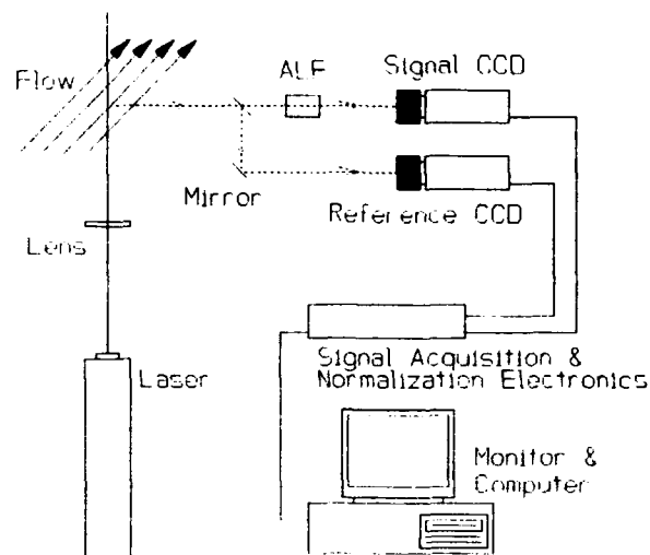
Figure 3. Simple one-component DGV system schematic. Basic DGV Specifications
