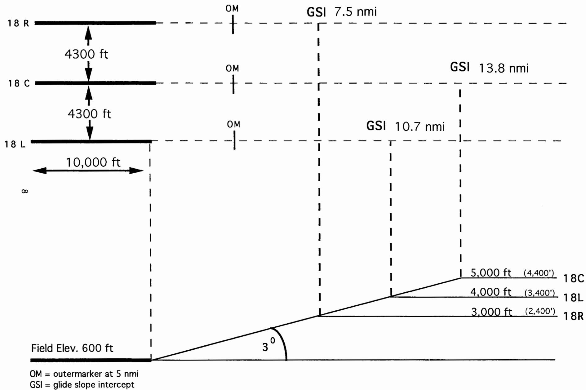
FIGURE 2. AIRPORT CONFIGURATION
