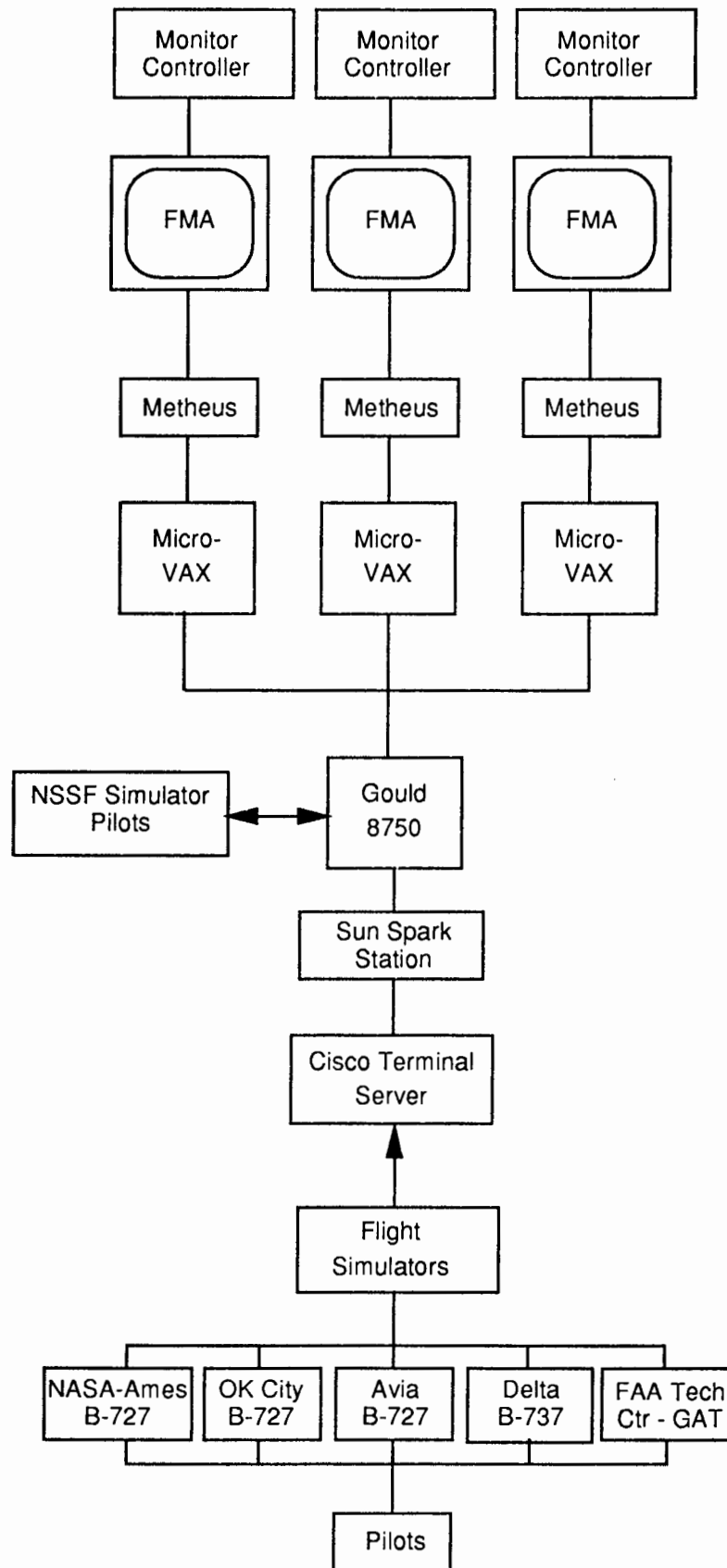
FIGURE 3. SCHEMATIC DIAGRAM OF NSSF CONFIGURATION
