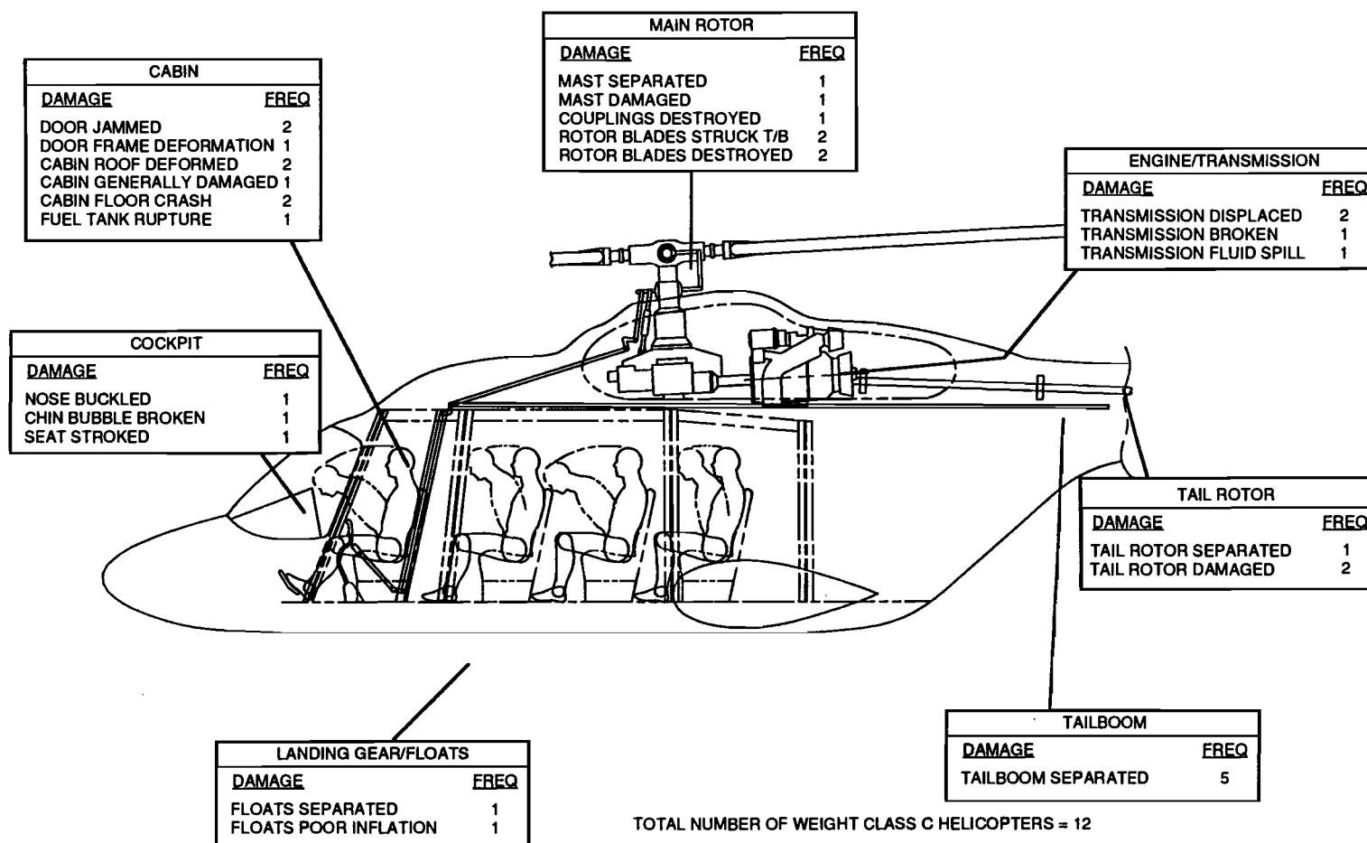
FIGURE 6. SUMMARY OF IMPACT DAMAGE FOR WEIGHT CLASS C ROTORCRAFT
