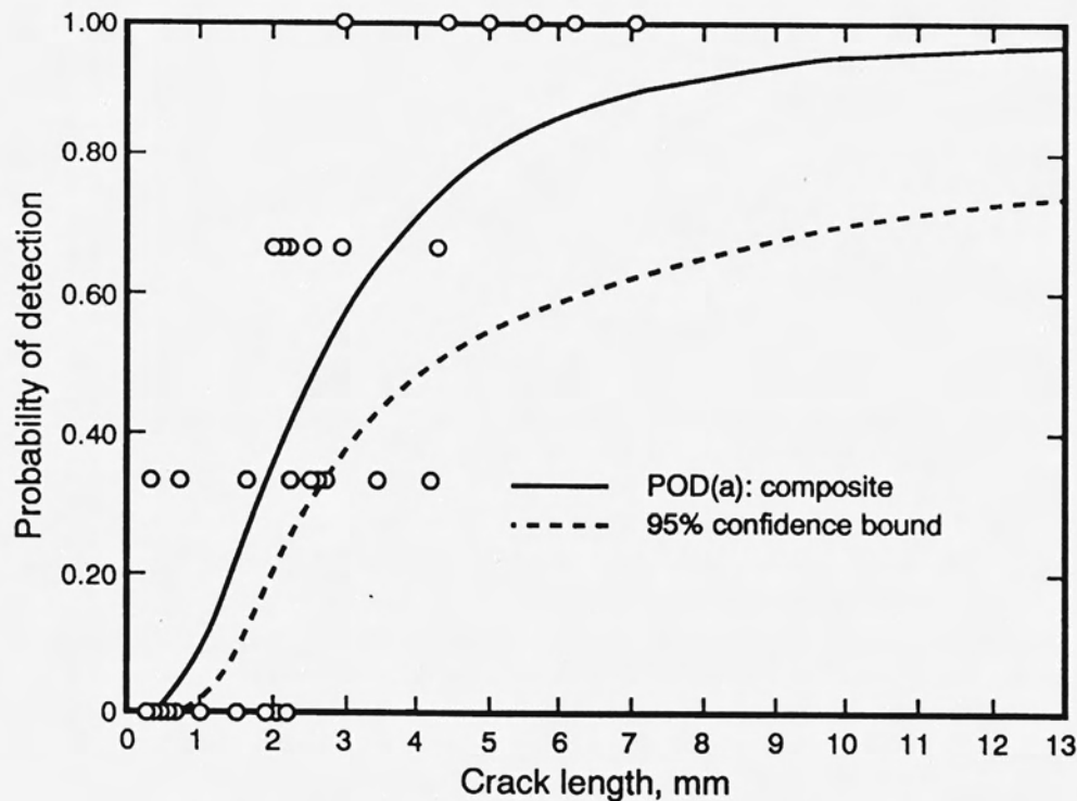
Figure 2. Example POD graph based on 3 inspections.
