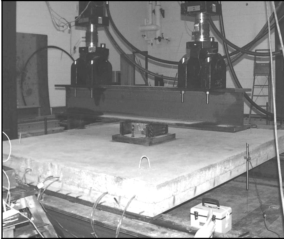
Figure 4.7 - Plate Load Testing Setup for Composite Slab Tests
