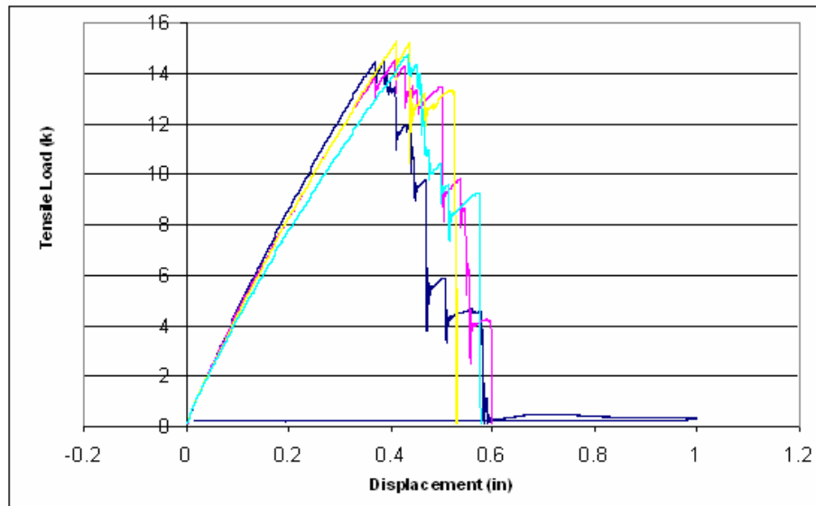
Figure 3.16 - Linear Behavior with a Non-Linear Region of Cyclic Load Reductions after Failure
