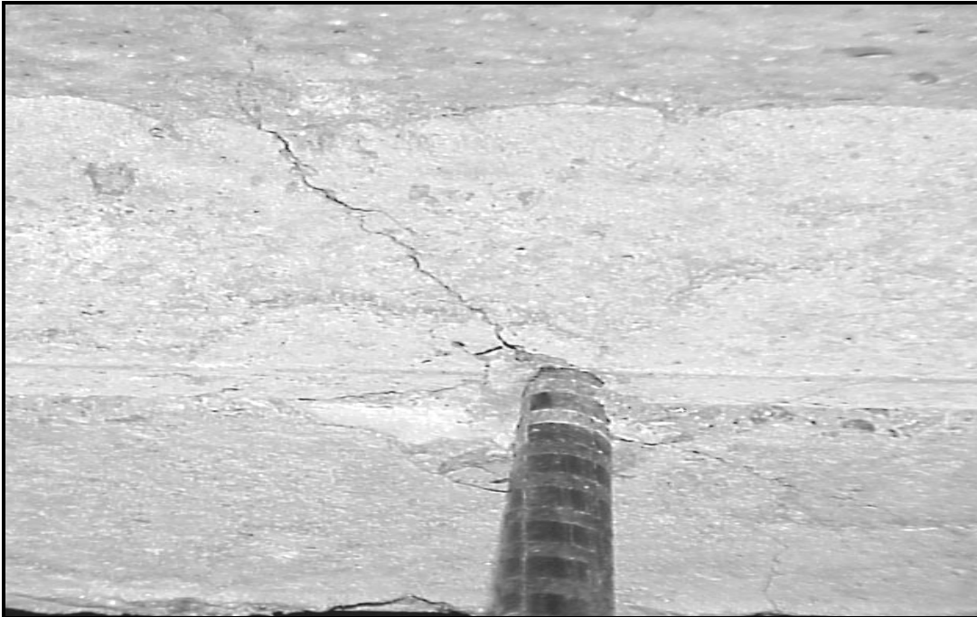
Figure 4.9 - Initial Cracking Surrounding the Prestressed CFRP Tendons
