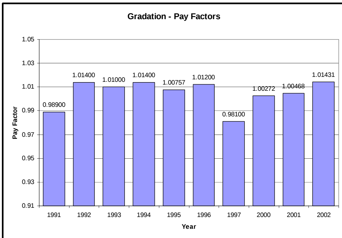
Figure 9. Gradation Pay Factors
