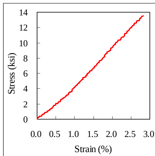
Figure 8. Tensile stress-strain curves of a GFRP bar after the free-thaw cyclic testing
