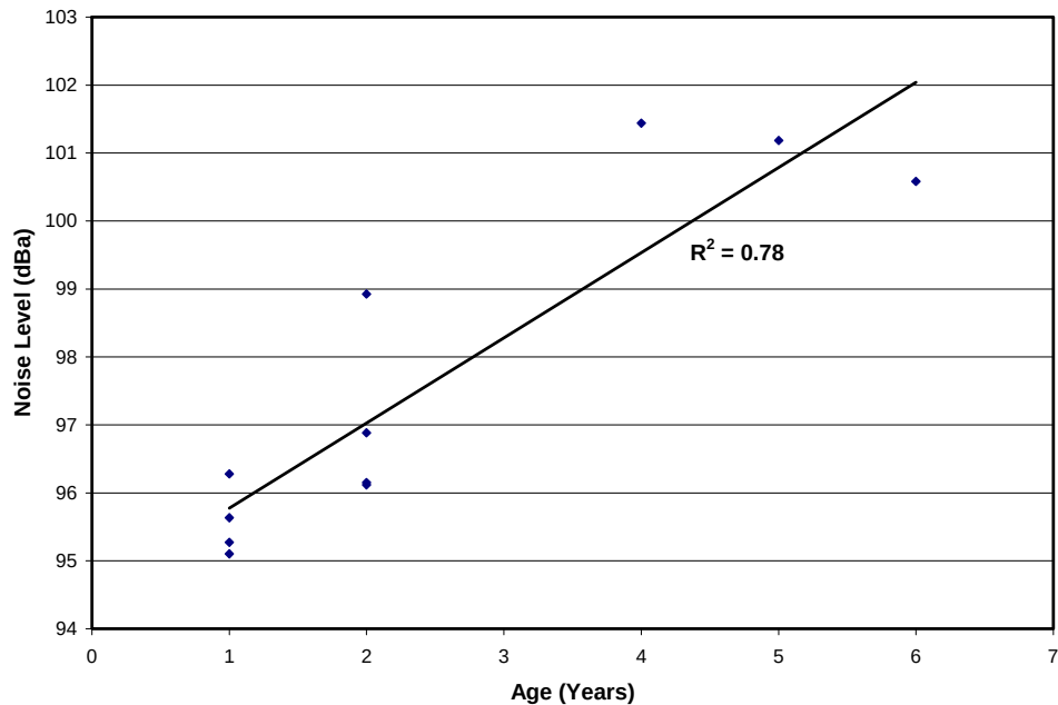
Figure 8 – Age versus Noise Level (dB(A)) for HMA Pavements Tested
