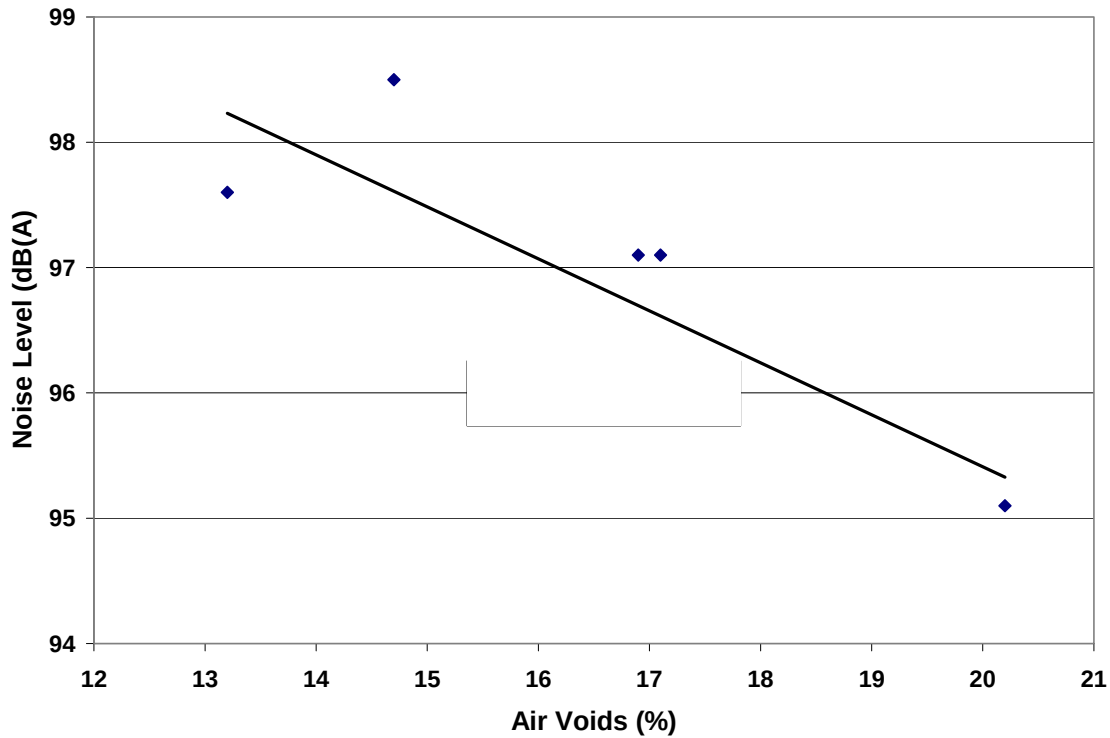
Figure 11 – Effect of Air Voids on Noise Level
