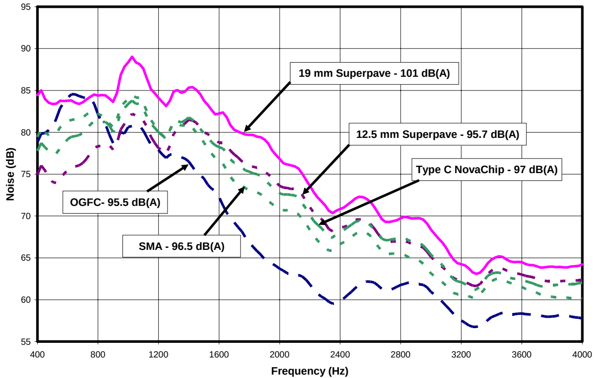
Figure 7 – Frequency Spectrum for HMA Pavements
