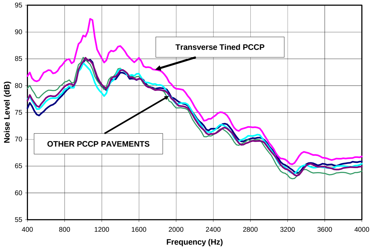
Figure 9 – Frequency Spectrum for PCCP Pavements
