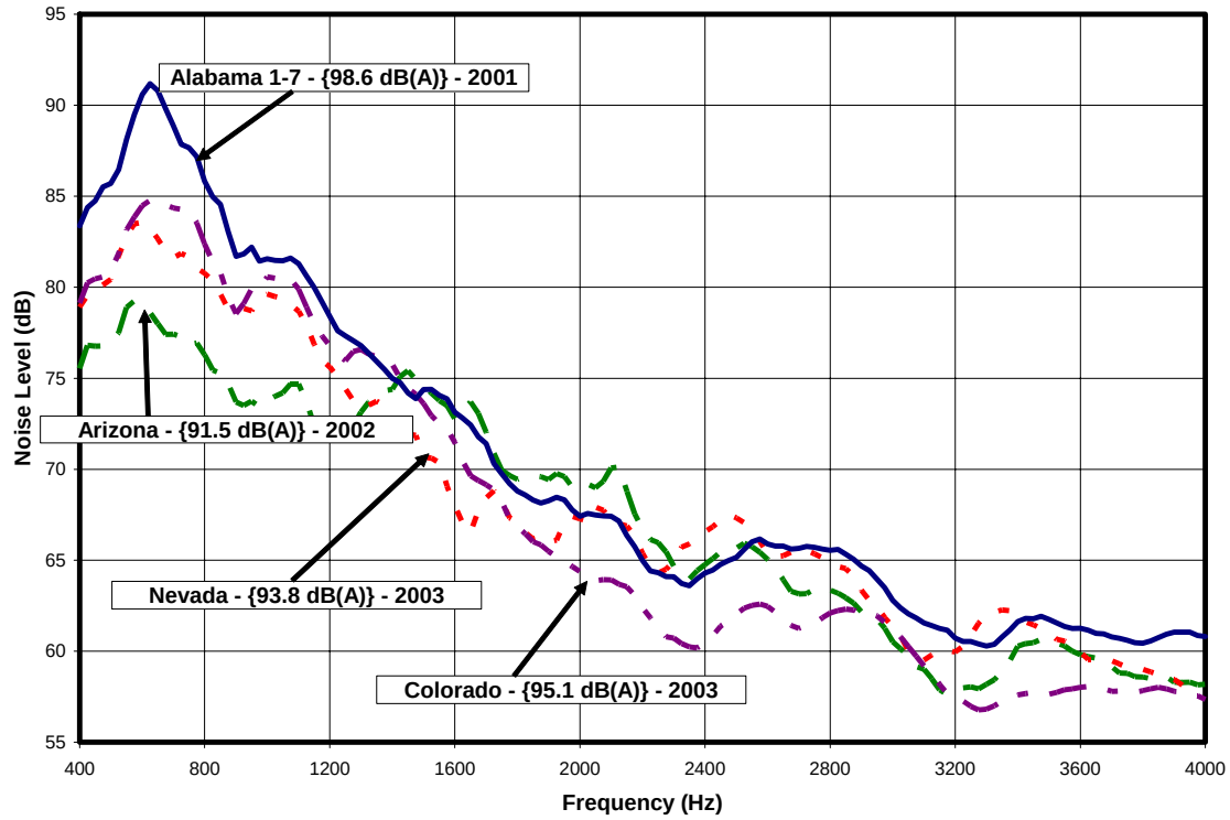
Figure 10 – Noise Spectrum for Different OGFC Mixes
