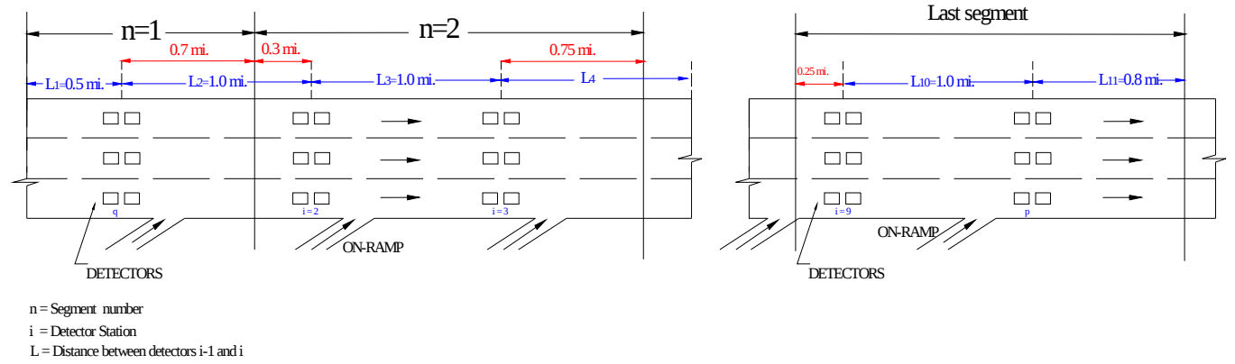
Figure 3.3. Example of Freeway Segments of Varying Lengths and Number of Detector Stations Within a Segment.
