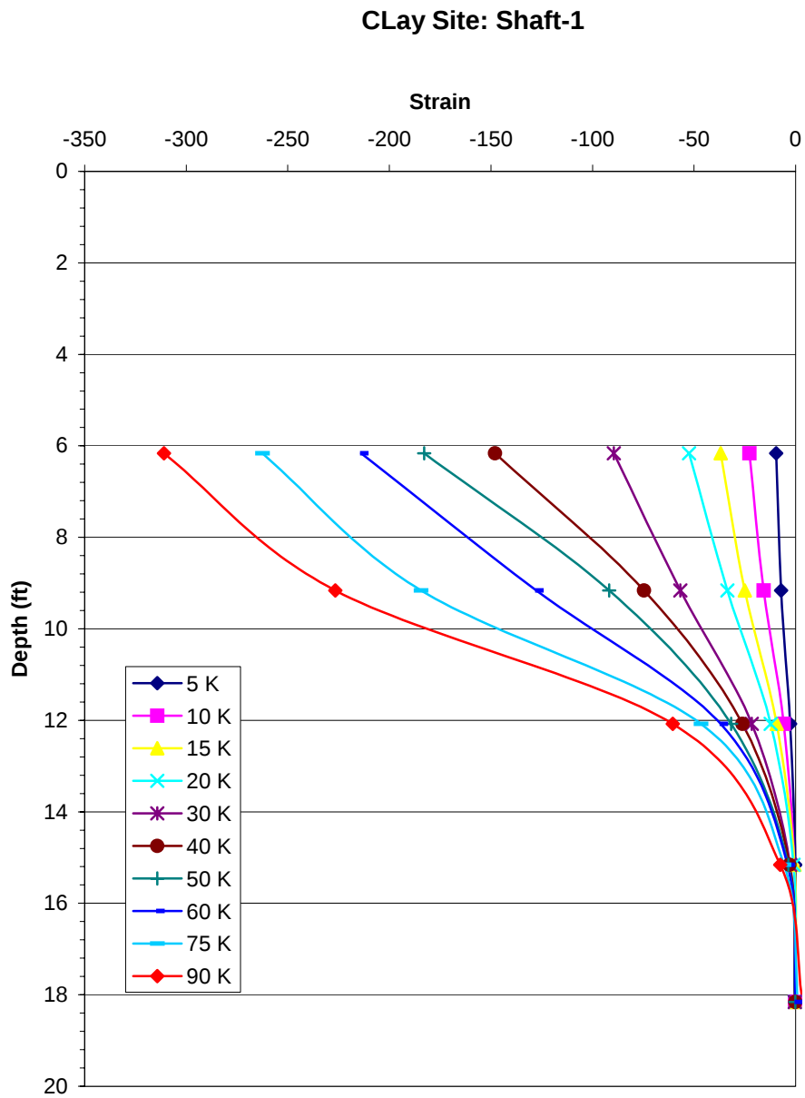
Figure 5.25. Test shaft #1, strain vs. depth on compression side
