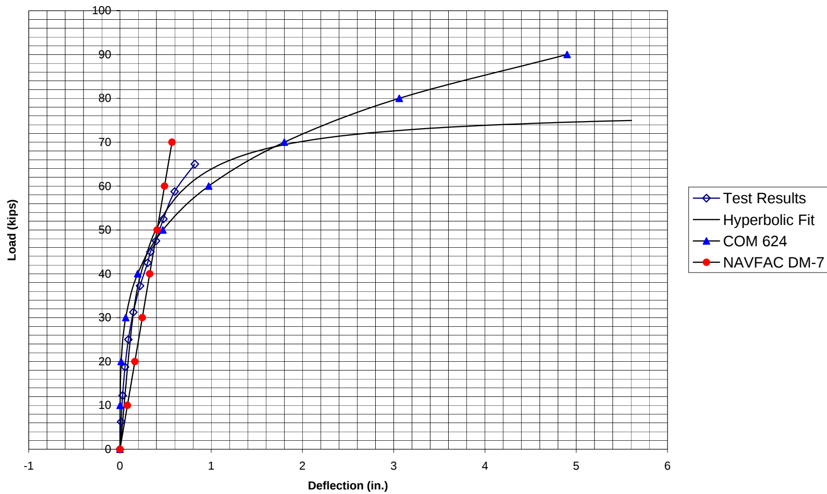
Figure 4.9 I-90 sound barriers, shaft 100 lateral load-deflection curves
