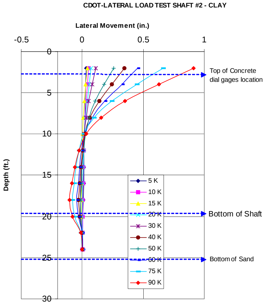
Figure 5.24 Load-deflection curves along the depth of test shaft #2 from inclinometer
