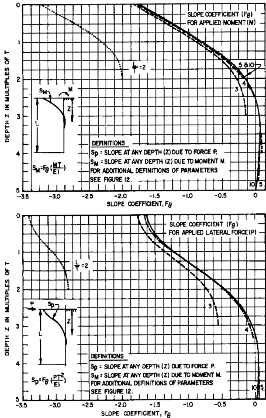
Figure B-20. Slope coefficient for pile with lateral load or moment
