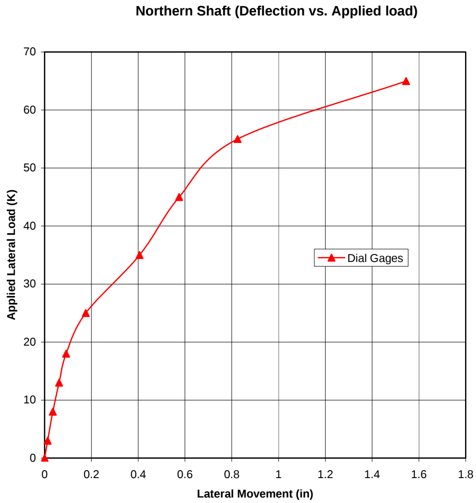
Figure 5.55 Load-deflection curve at the top of test shaft North from dial gages
