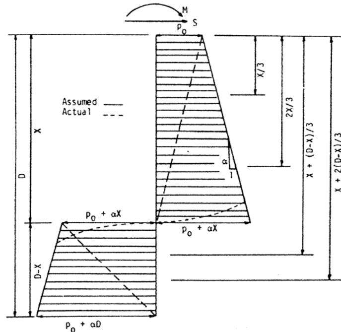
Figure B-12. Ultimate soil resistance for cohesive soil.
