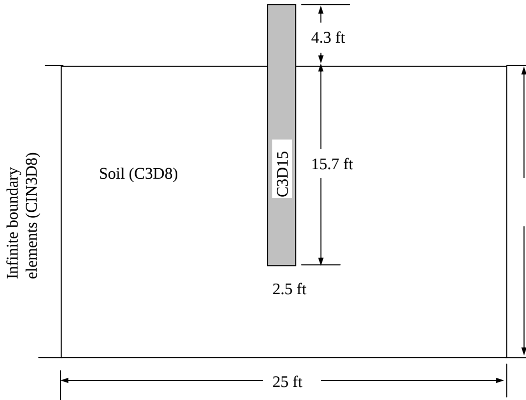
Figure 6.3 Dimensions of the final mesh for CDOT shaft simulations
