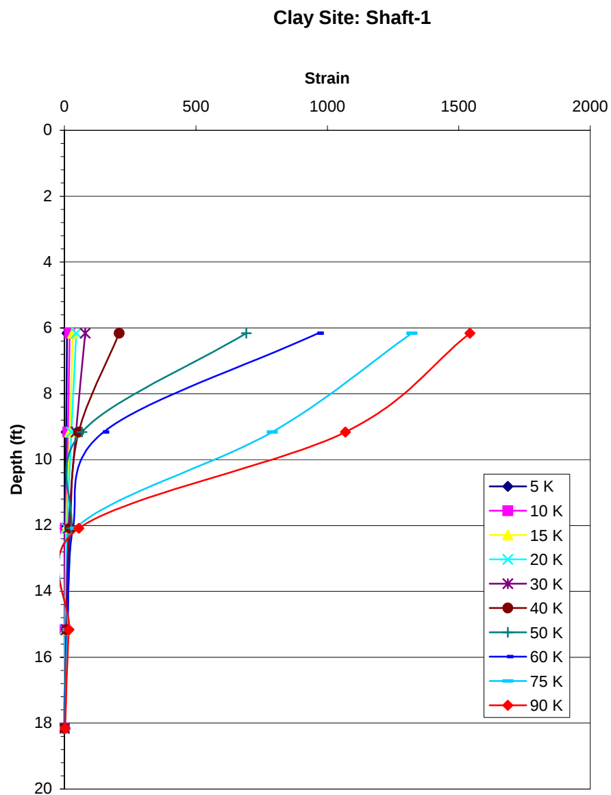
Figure 5.26. Test shaft #1, strain vs. depth on tension side
