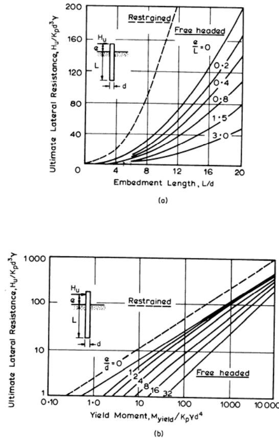
Figure B-7. Ultimate lateral resistance of piles in cohesionless soil (a) short (b) long (after Poulos and Davis)
