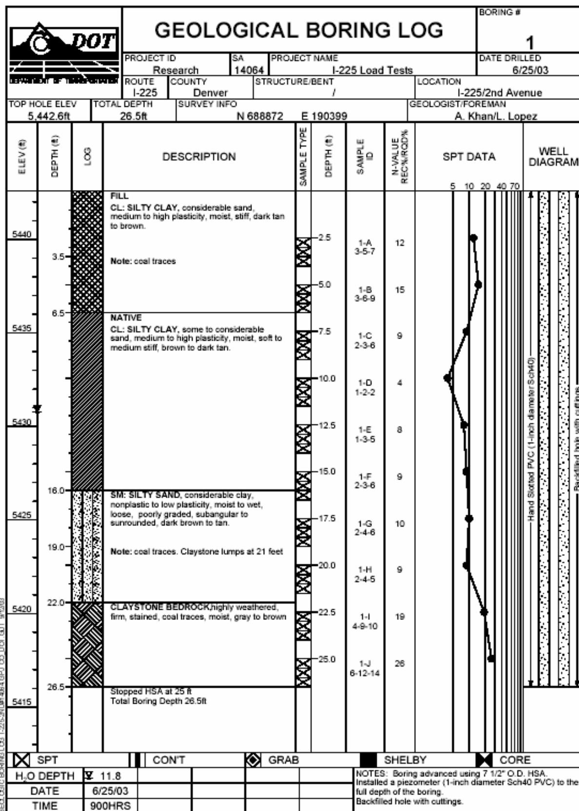
Figure 5.2a Test borings 1
