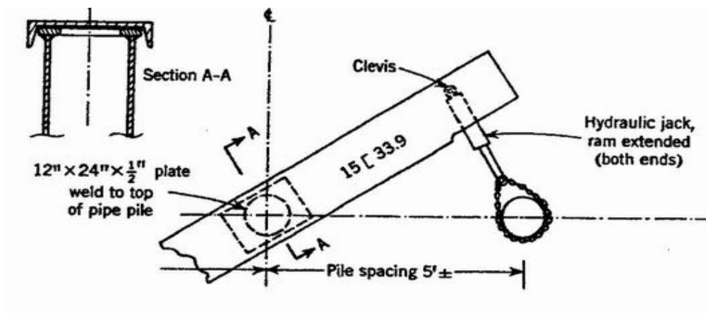
Figure C-11 Pile Torque Shear Test Set Up (After Stoll 1972)
