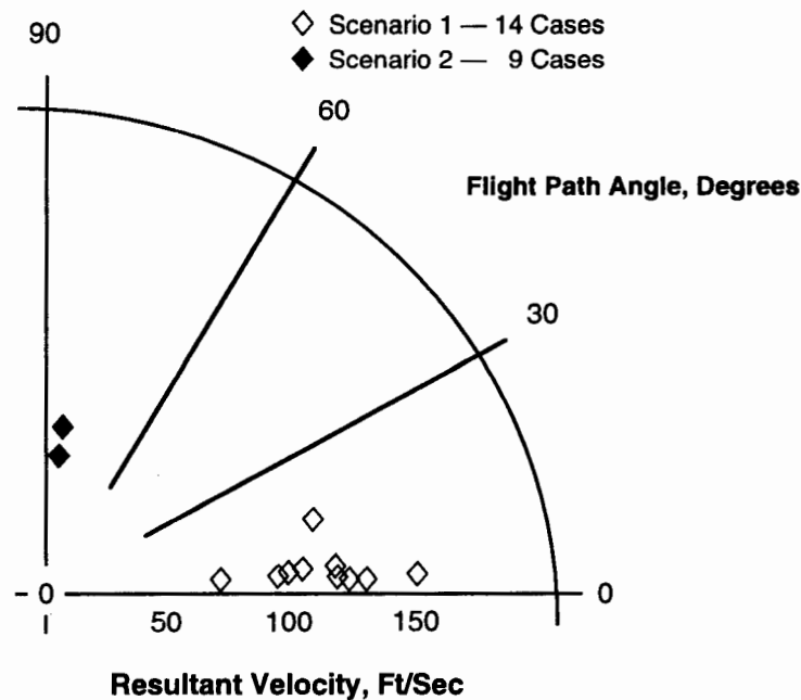
FIGURE 3.23. RESULTANT VELOCITY VS. FLIGHT PATH ANGLE RELATIVE TO IMPACT SCENARIO
