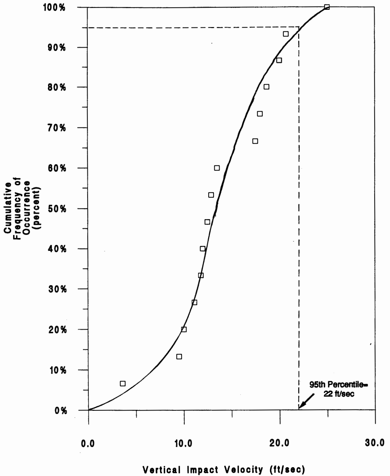
FIGURE 3.8. CUMULATIVE FREQUENCY OF OCCURRENCE OF VERTICAL IMPACT VELOCITIES, SURVIVABLE AND PARTIALLY SURVIVABLE ACCIDENTS
