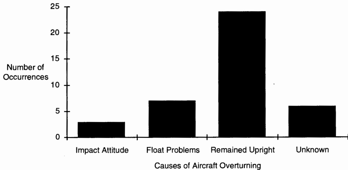
FIGURE 3.20. DISTRIBUTION OF CAUSES OF AIRCRAFT OVERTURNING
