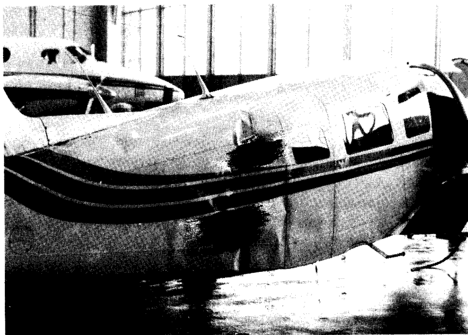
FIGURE 4.6. CASE STUDY 4, RIGHT VIEW OF REAR FUSELAGE DAMAGE
