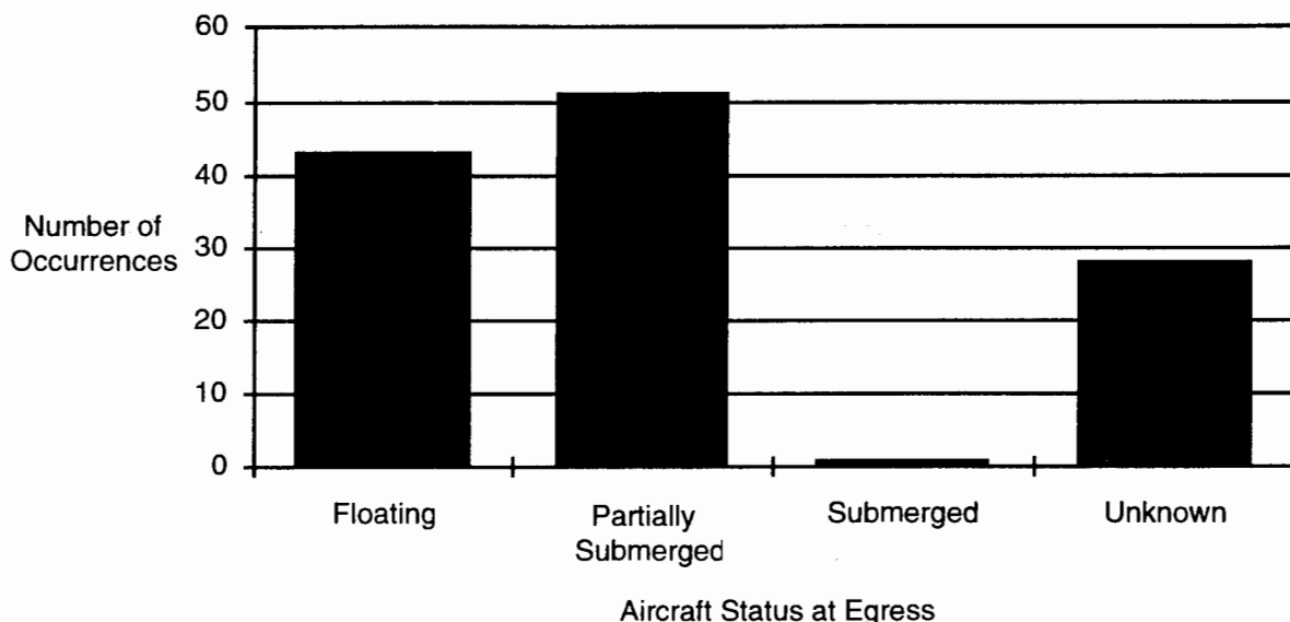
FIGURE 3.21. DISTRIBUTION OF AIRCRAFT STATUS AT TIME OF OCCUPANT EGRESS
