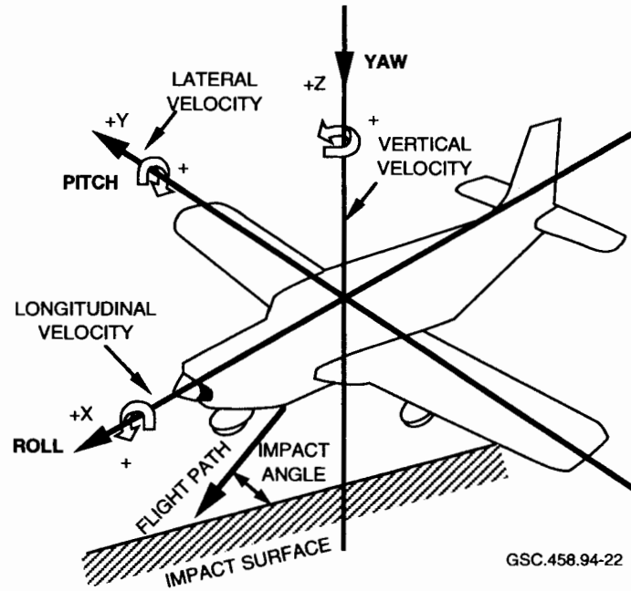
FIGURE 7.1. AIRCRAFT ATTITUDE AND VELOCITY COMPONENT DIRECTIONS
