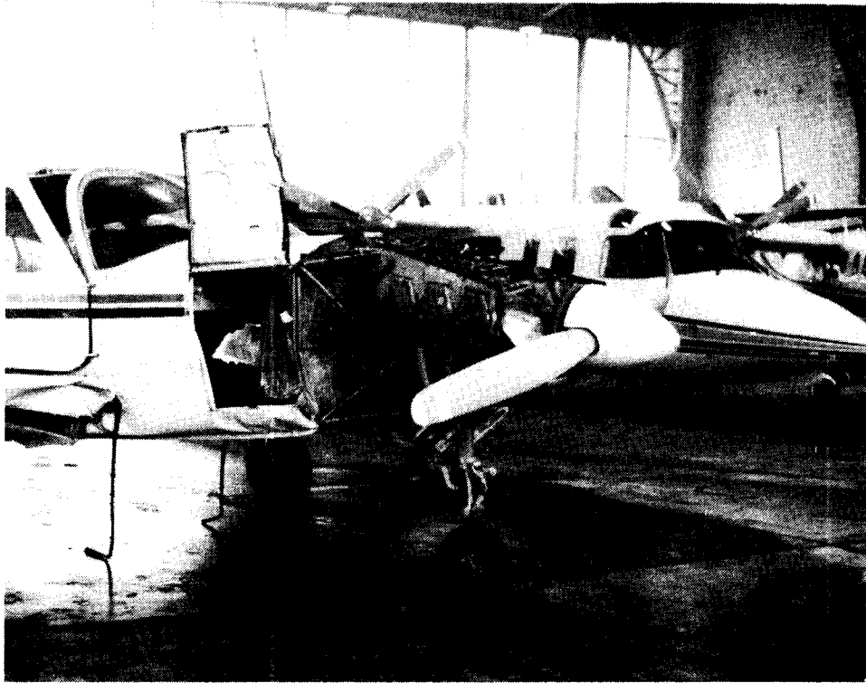
FIGURE 4.7. CASE STUDY 4, RIGHT VIEW OF NOSE DAMAGE
