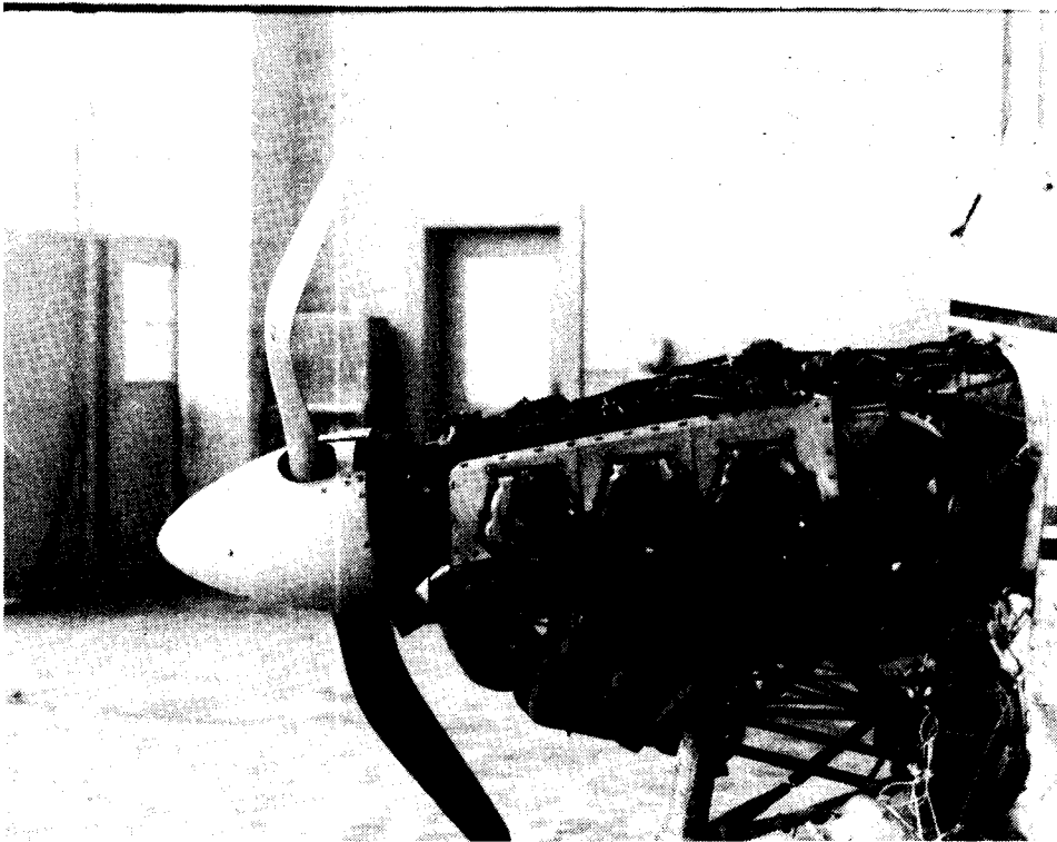
FIGURE 4.8. CASE STUDY 4, LEFT VIEW OF NOSE DAMAGE
