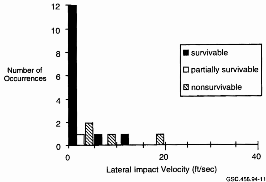
FIGURE 3.11. DISTRIBUTION OF LATERAL IMPACT VELOCITY RELATIVE TO ACCIDENT SURVIVABILITY
