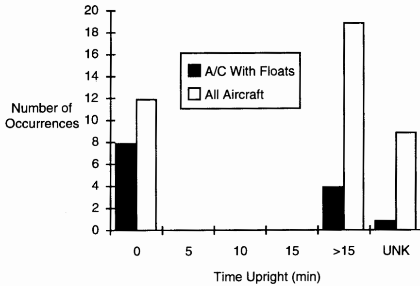
FIGURE 3.19. AIRCRAFT TIME UPRIGHT RELATIVE TO AIRCRAFT FLOAT CONFIGURATION
