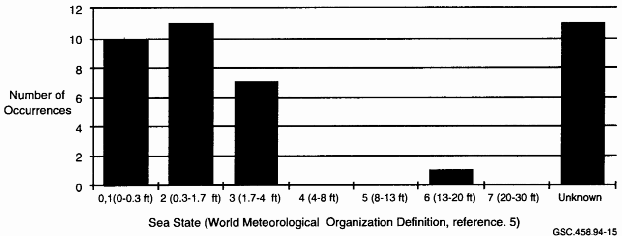
FIGURE 3.17 SEA STATES ENCOUNTERED BY AIRCRAFT, TOTAL SAMPLE
