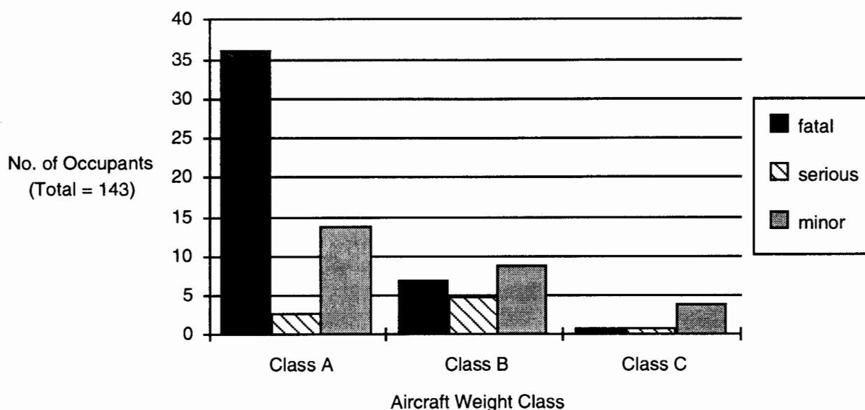
FIGURE 3.2. INJURY SEVERITY DISTRIBUTION BY AIRCRAFT WEIGHT CLASS
