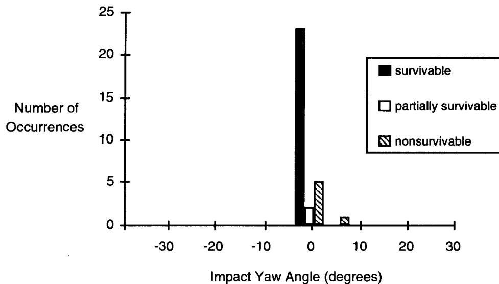
FIGURE 3.6. DISTRIBUTION OF IMPACT YAW ANGLE RELATIVE TO ACCIDENT SURVIVABILITY, TOTAL SAMPLE
