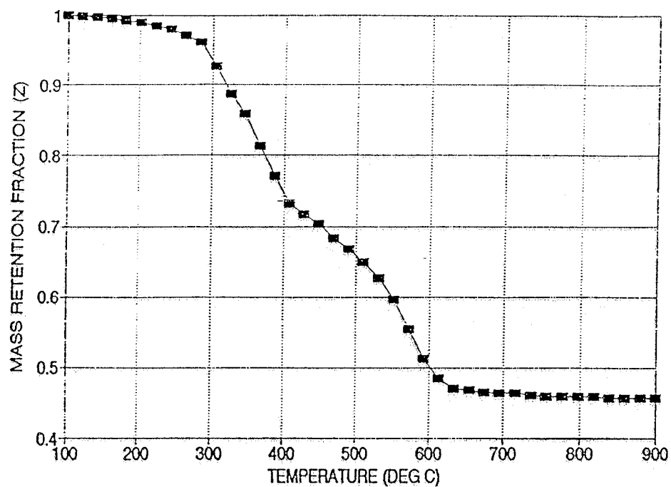
Figure 4. TGA Plot for Panel A.
