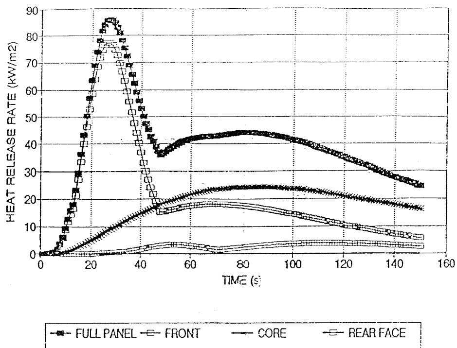
Figure 10. Calculated Contributions of Panel A Components to the Heat Release Rate at an Exposure of 35 kW/m 2 .
