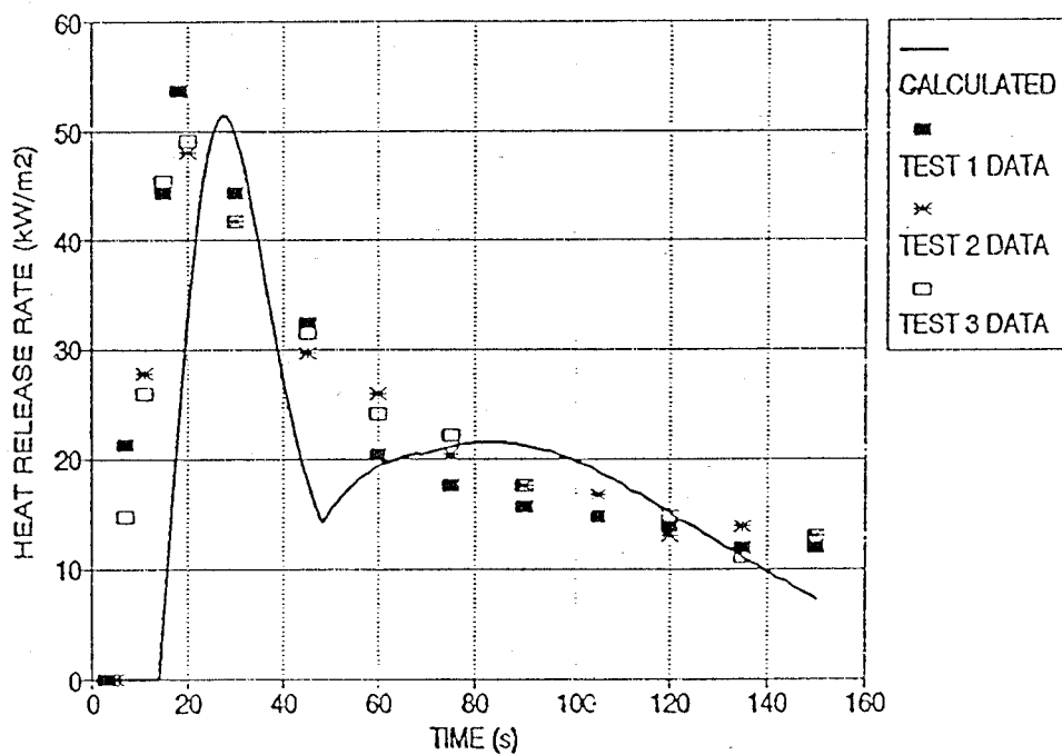
Figure 11. Heat release rate of Panel A in OSU at 35 kW/m 2 .
