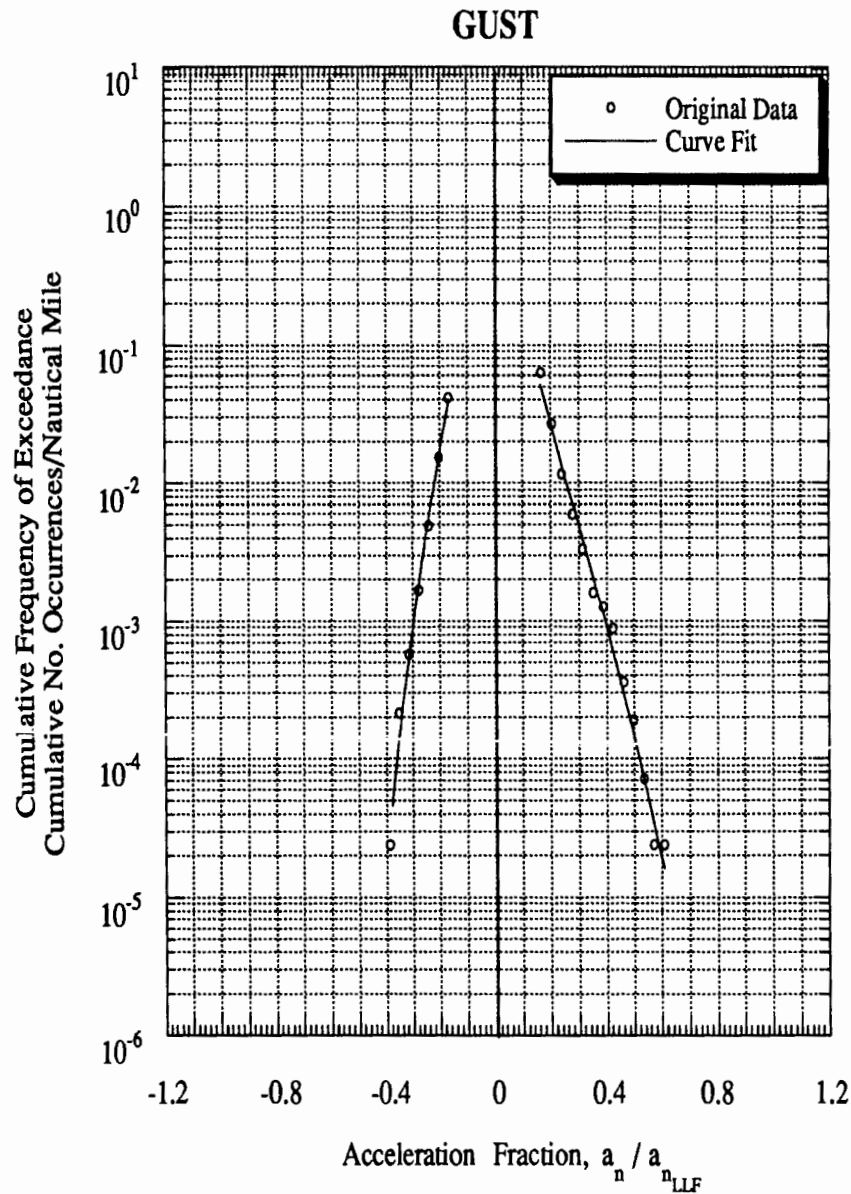
Figure C-4 Load Spectra for Airplane 14, Single-Engine, Basic Flight Instruction
