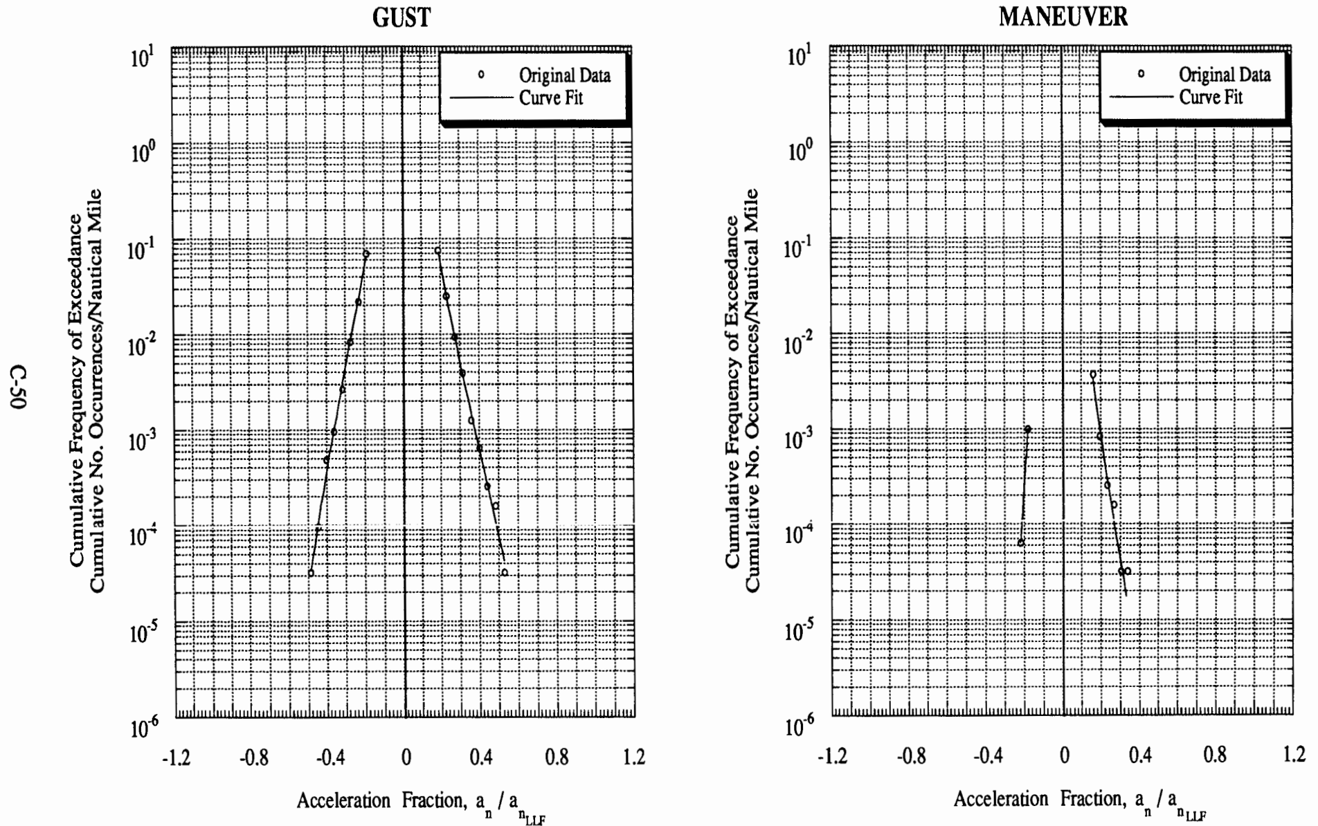
Figure C-22 Load Spectra for Airplane 10, Single-Engine, Business/Personal
