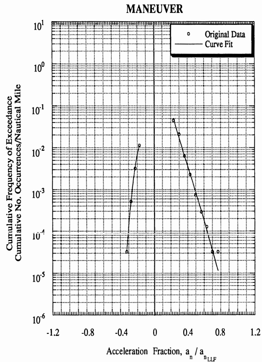
Figure C-90 Load Spectra for Airplane 23, Large Airplanes, Special Usage
