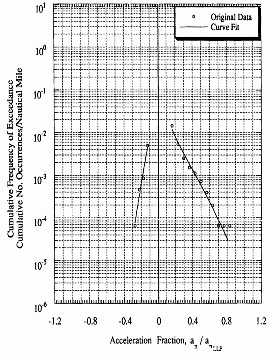
Figure C-81 Load Spectra for Airplane 1 3 , Twin-Engine, Executive Jet
