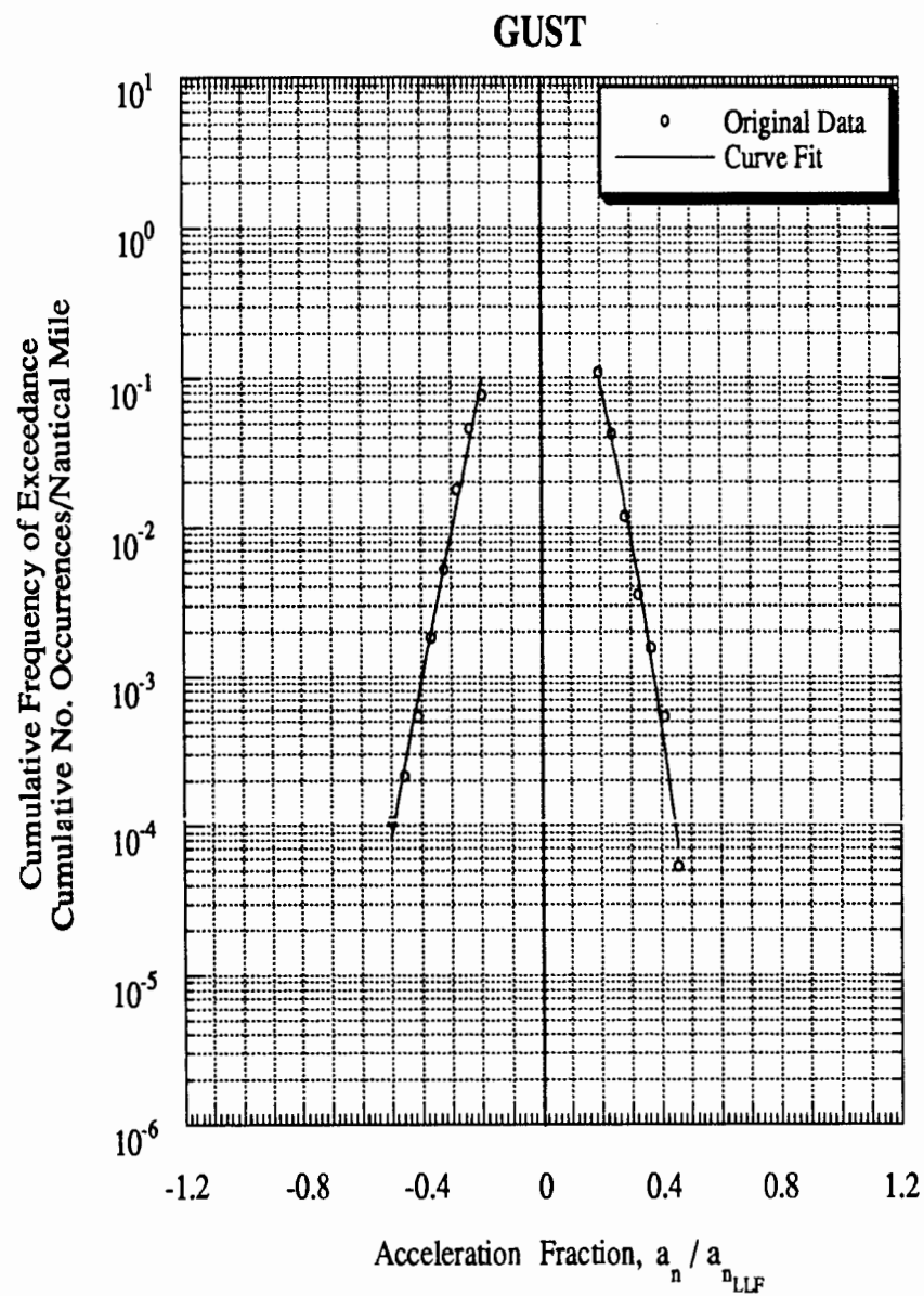
Figure C-61 Load Spectra for Airplane 36, Aerial Application
