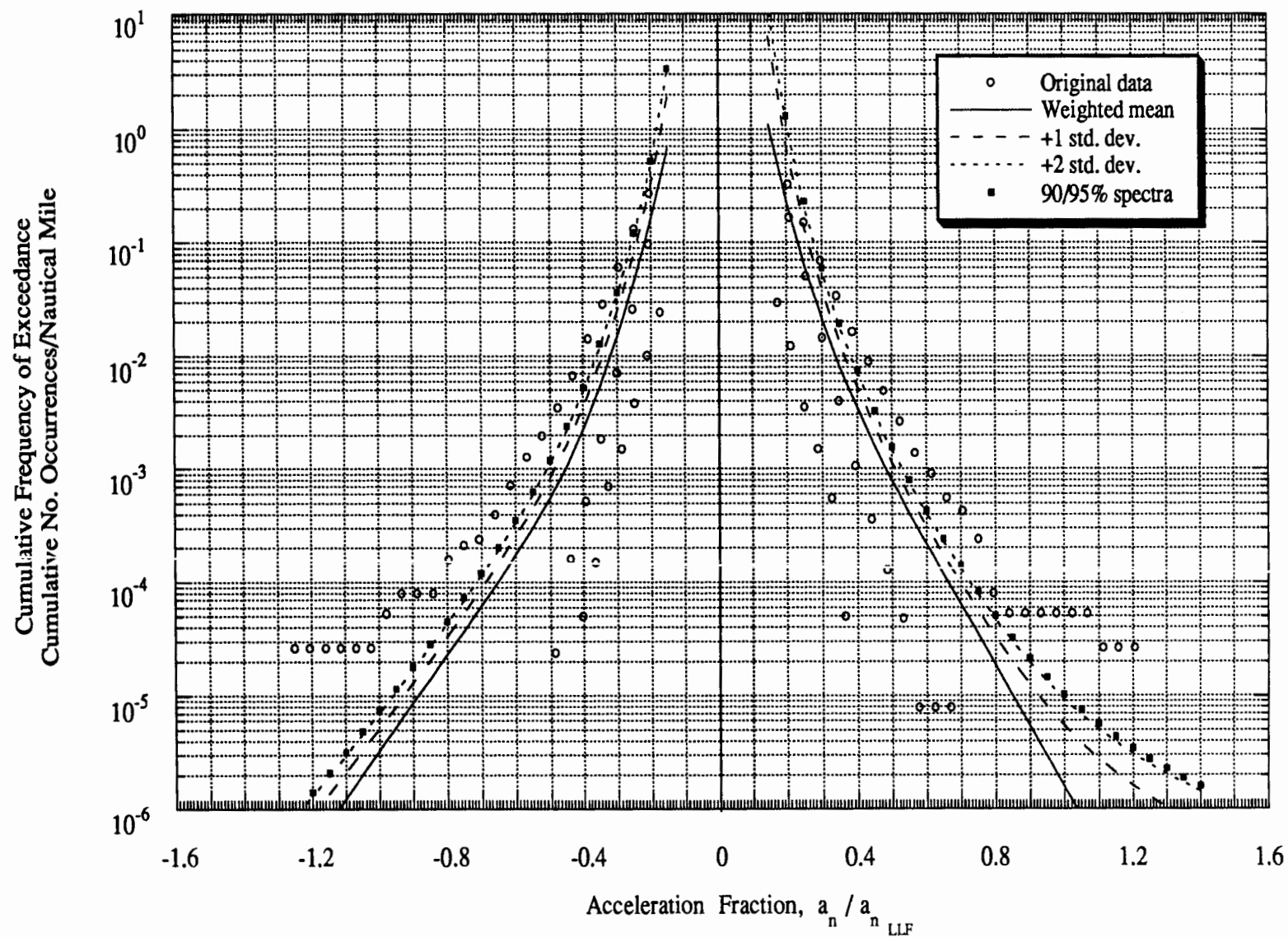
Figure D-13 Gust Load Spectra: Twin-Engine Special Usage
