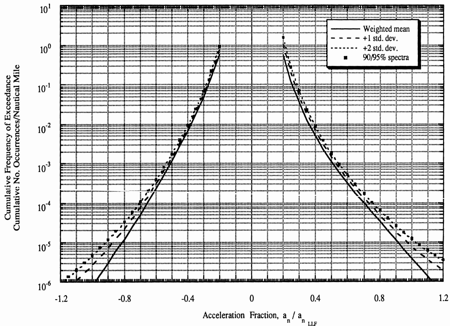
Figure 2-8 Gust Load Spectra: Single-Engine Special Usage
