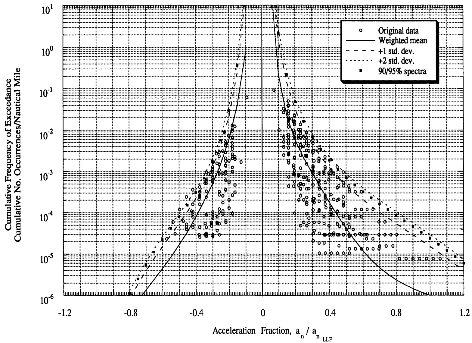
Figure D-4 Maneuver Load Spectra: Single-Engine General Usage, Business/Personal
