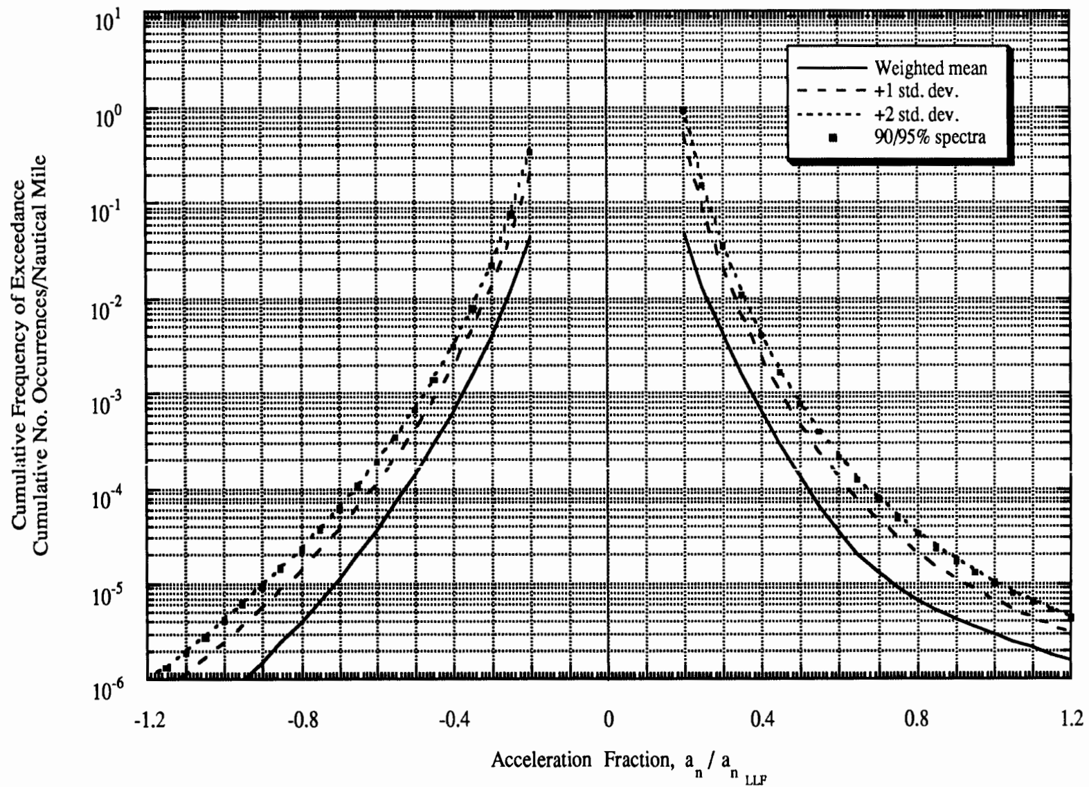
Figure 2-12 Gust Load Spectra: Twin-Engine General Usage
