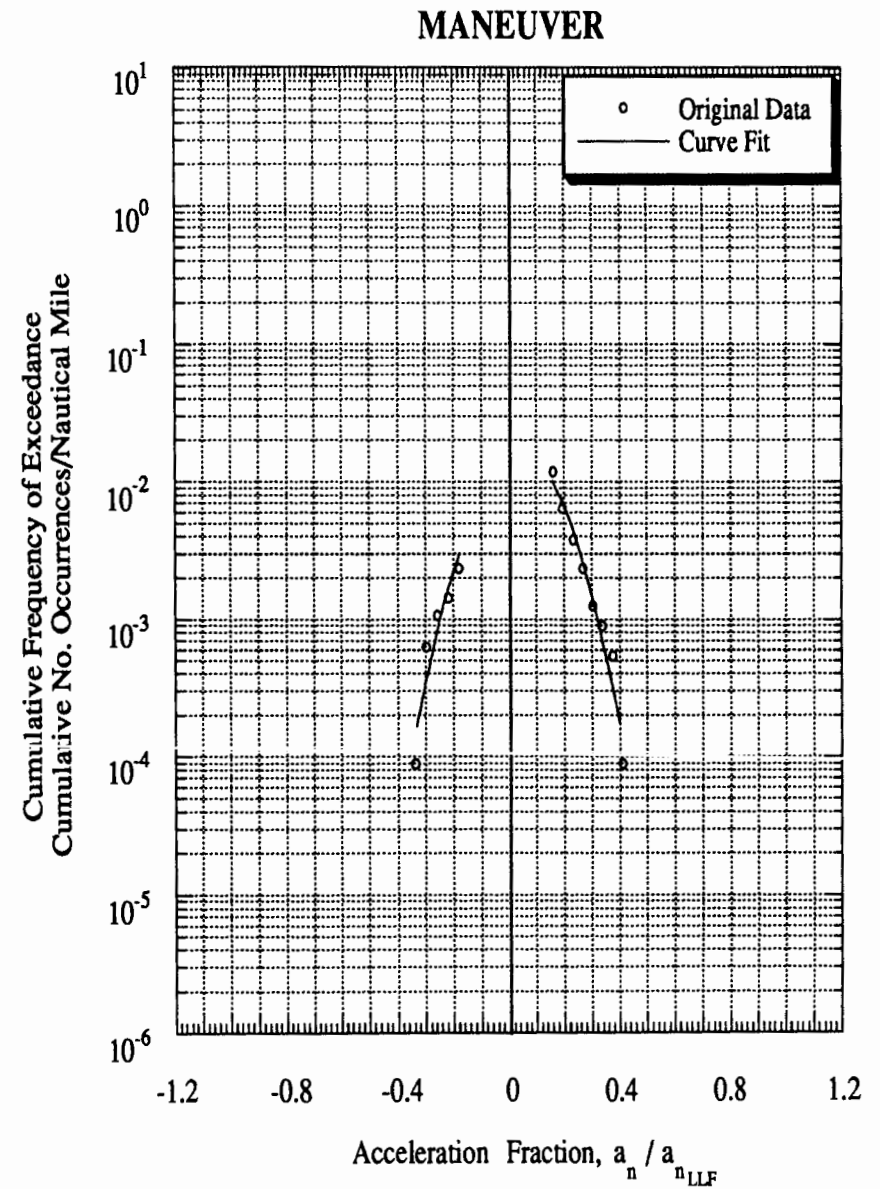
Figure C-32 Load Spectra for Airplane 13 1 , Single-Engine, Business/Personal
