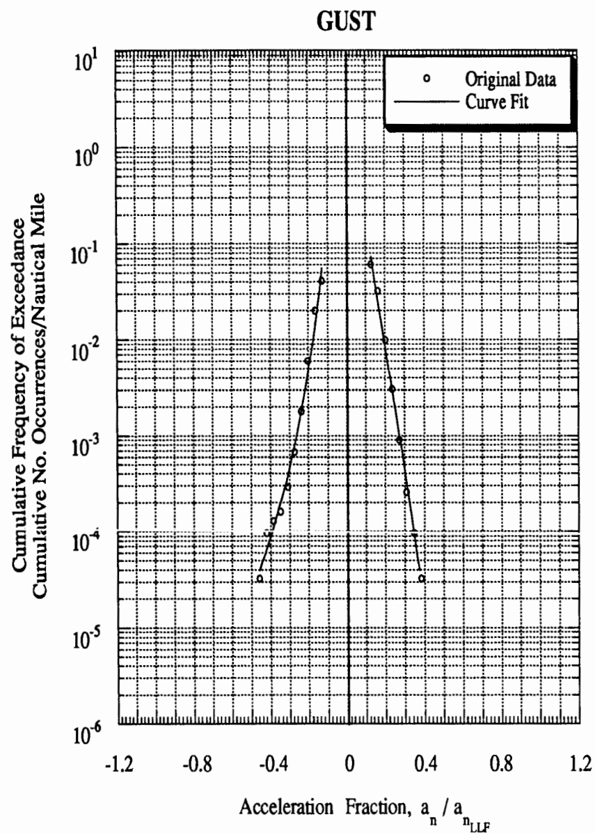
Figure C-90 Load Spectra for Airplane 23, Large Airplanes, Special Usage
