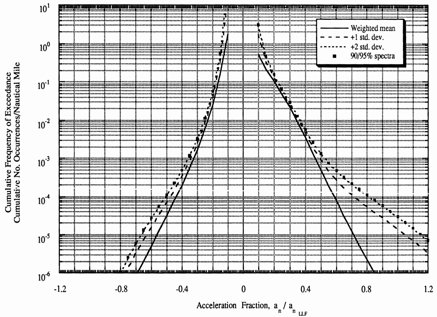
Figure 2-9 Maneuver Load Spectra: Single-Engine Special Usage
