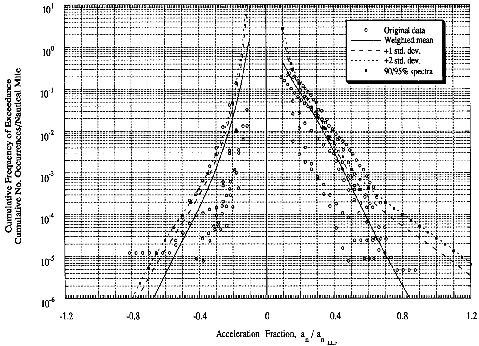
Figure D-16 Maneuver Load Spectra: Single and Twin-Engine Special Usage
