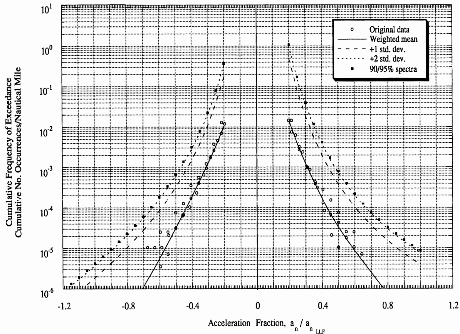
Figure D-17 Gust Load Spectra: Single and Twin-Engine Pressurized General Usage
