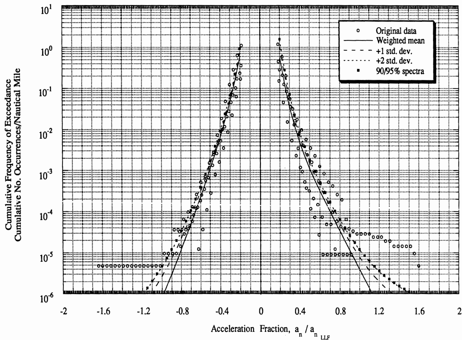
Figure D-7 Gust Load Spectra: Single-Engine Special Usage
