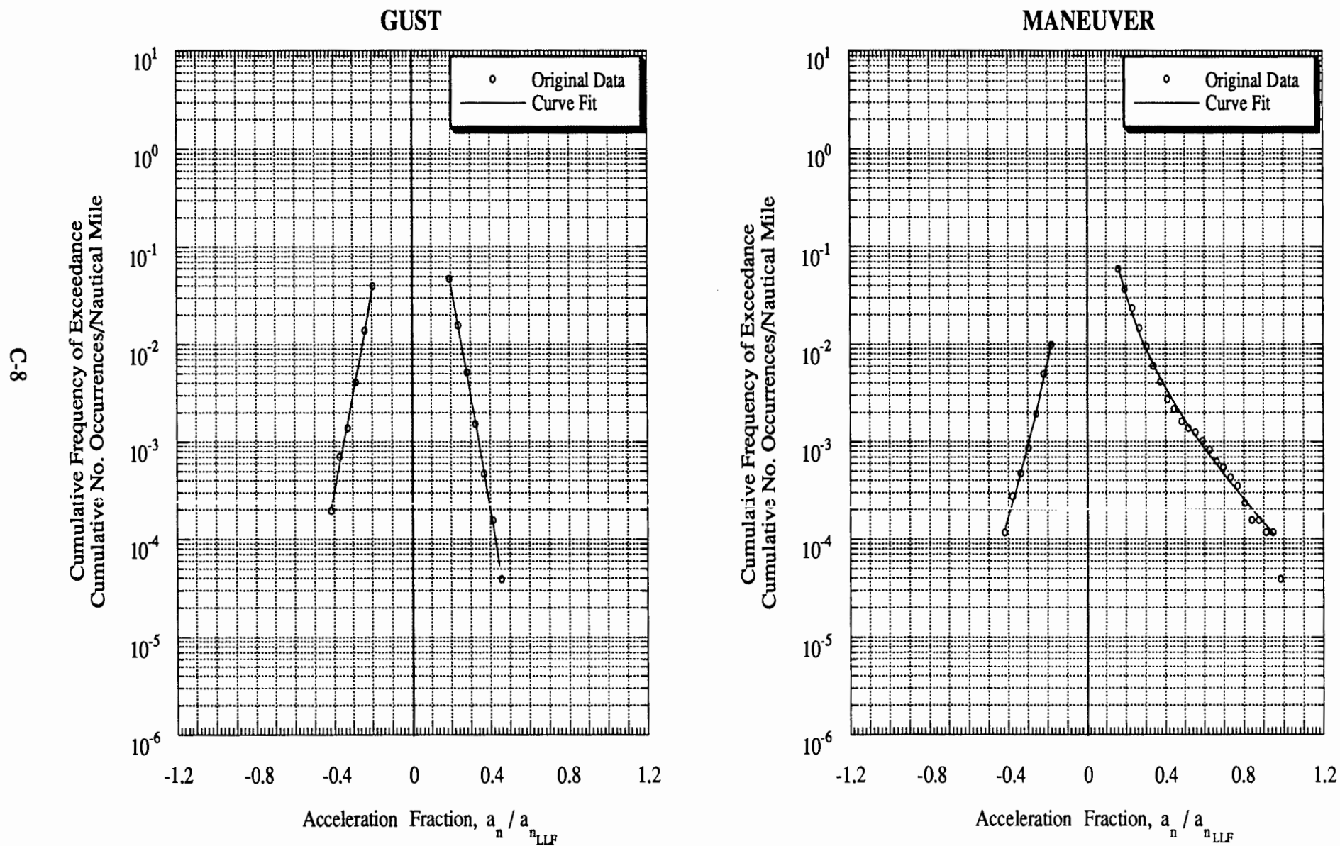
Figure C-1 Load Spectra for Airplane 12B, Single-Engine, Basic Flight Instruction
