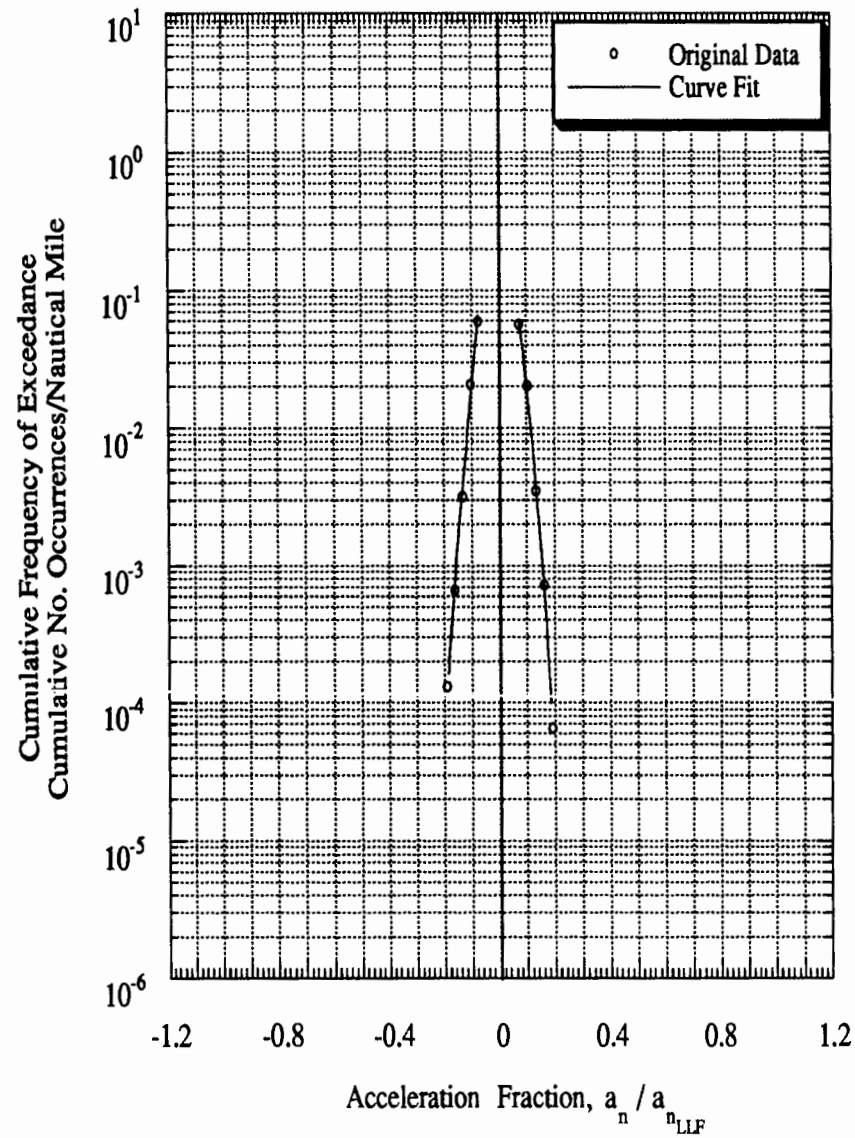
Figure C-81 Load Spectra for Airplane 1 3 , Twin-Engine, Executive Jet
