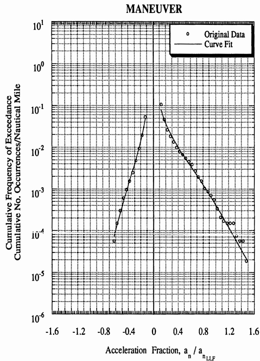
Figure C-88 Load Spectra for Airplane 21, Large Airplanes, Special Usage
