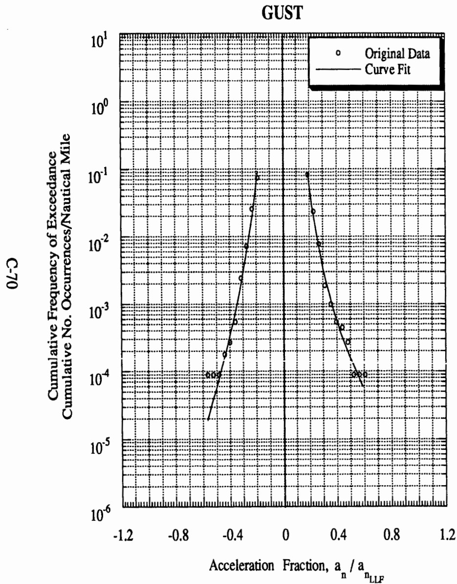
Figure C-32 Load Spectra for Airplane 13 1 , Single-Engine, Business/Personal
