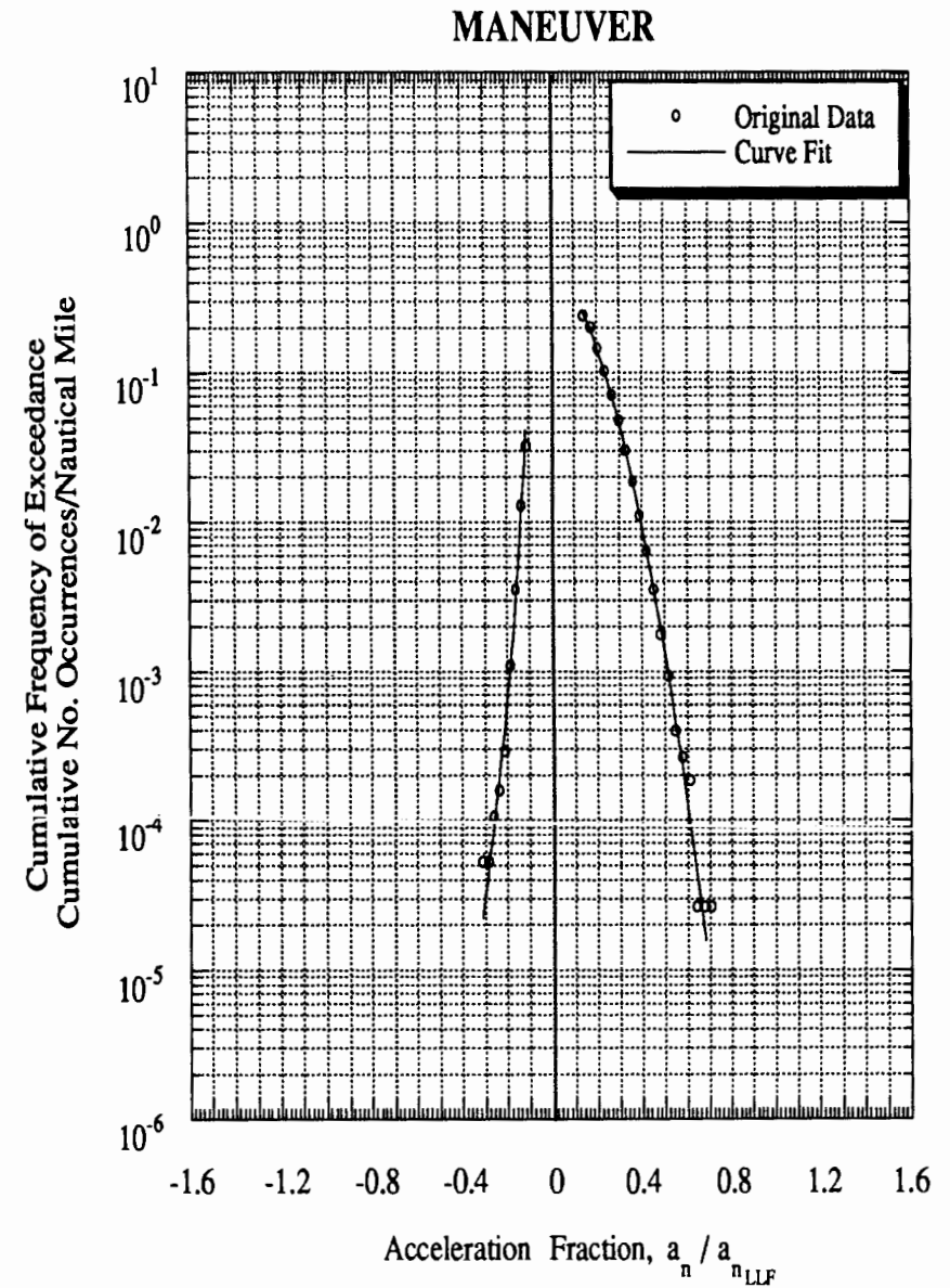
Figure C-74 Load Spectra for Airplane 25, Twin-Engine, Special Usage
