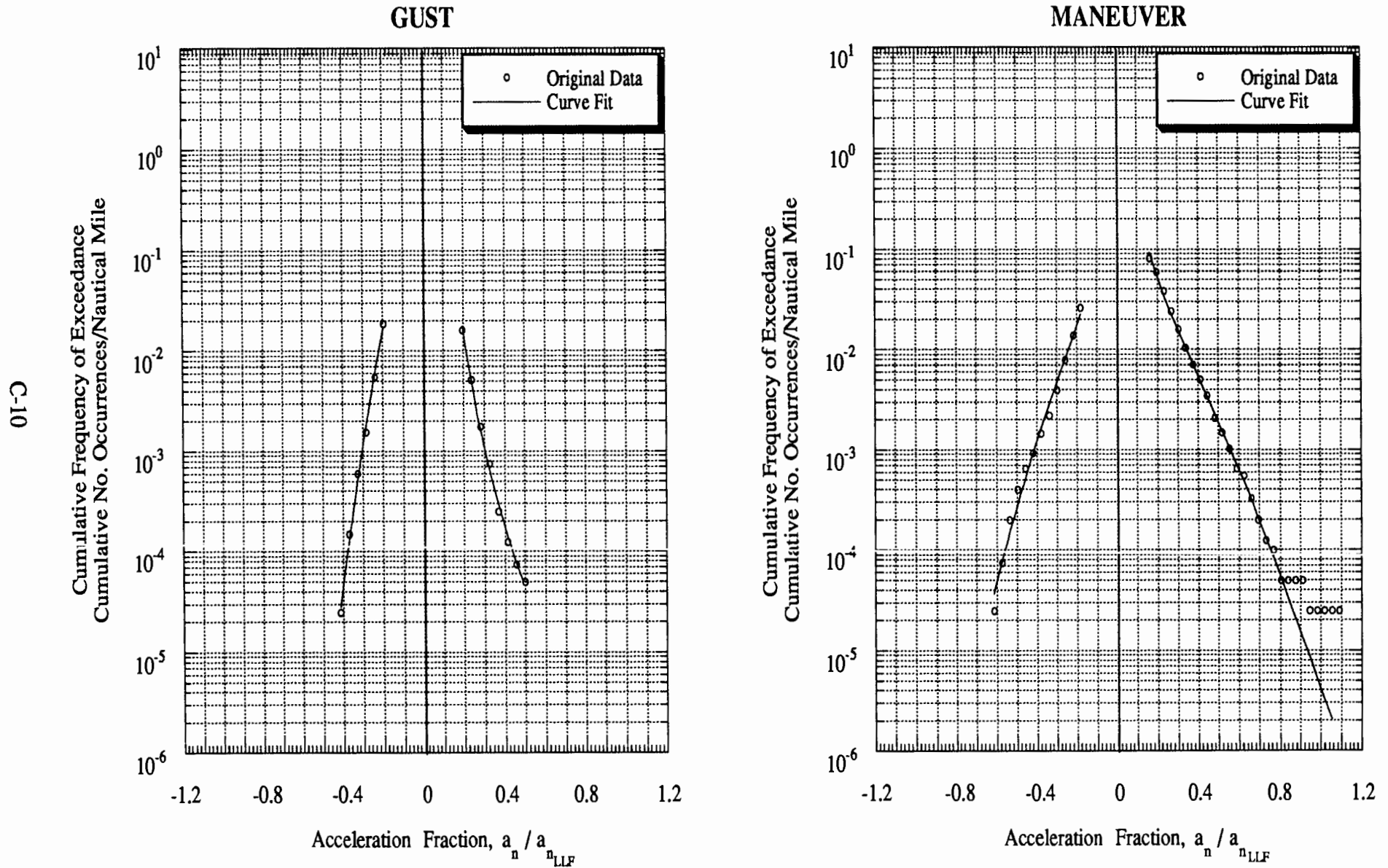
Figure C-2 Load Spectra for Airplane 12B 1 , Single-Engine, Basic Flight Instruction
