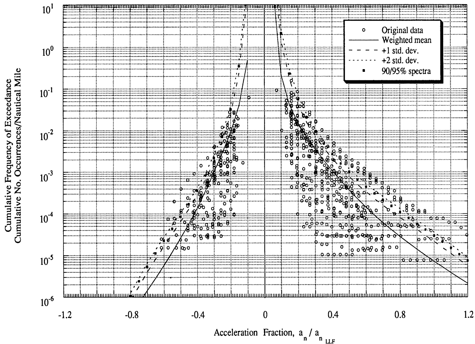
Figure D-6 Maneuver Load Spectra: Single-Engine General Usage (Basic Flight Instruction and Business/Personal Combined)
