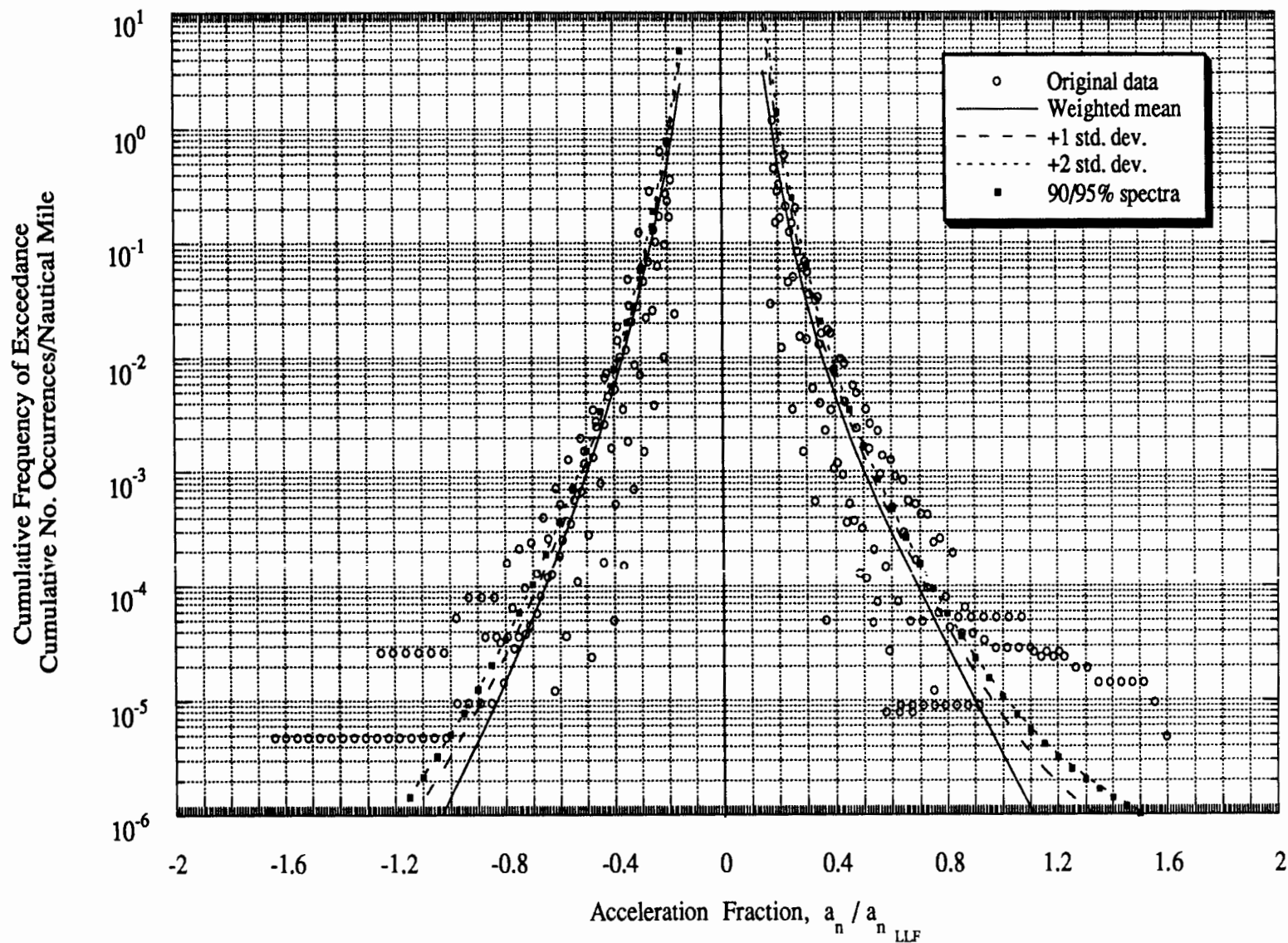
Figure D-15 Gust Load Spectra: Single and Twin-Engine Special Usage
