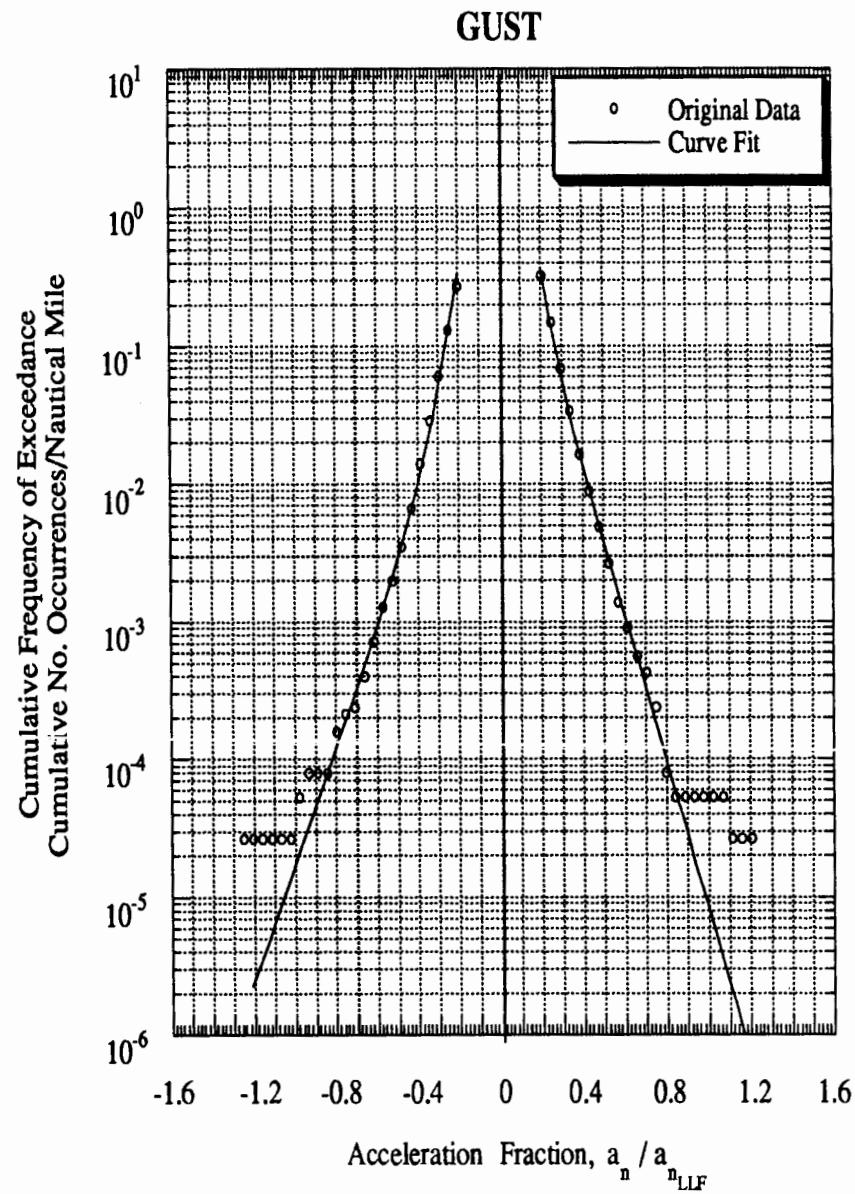
Figure C-74 Load Spectra for Airplane 25, Twin-Engine, Special Usage
