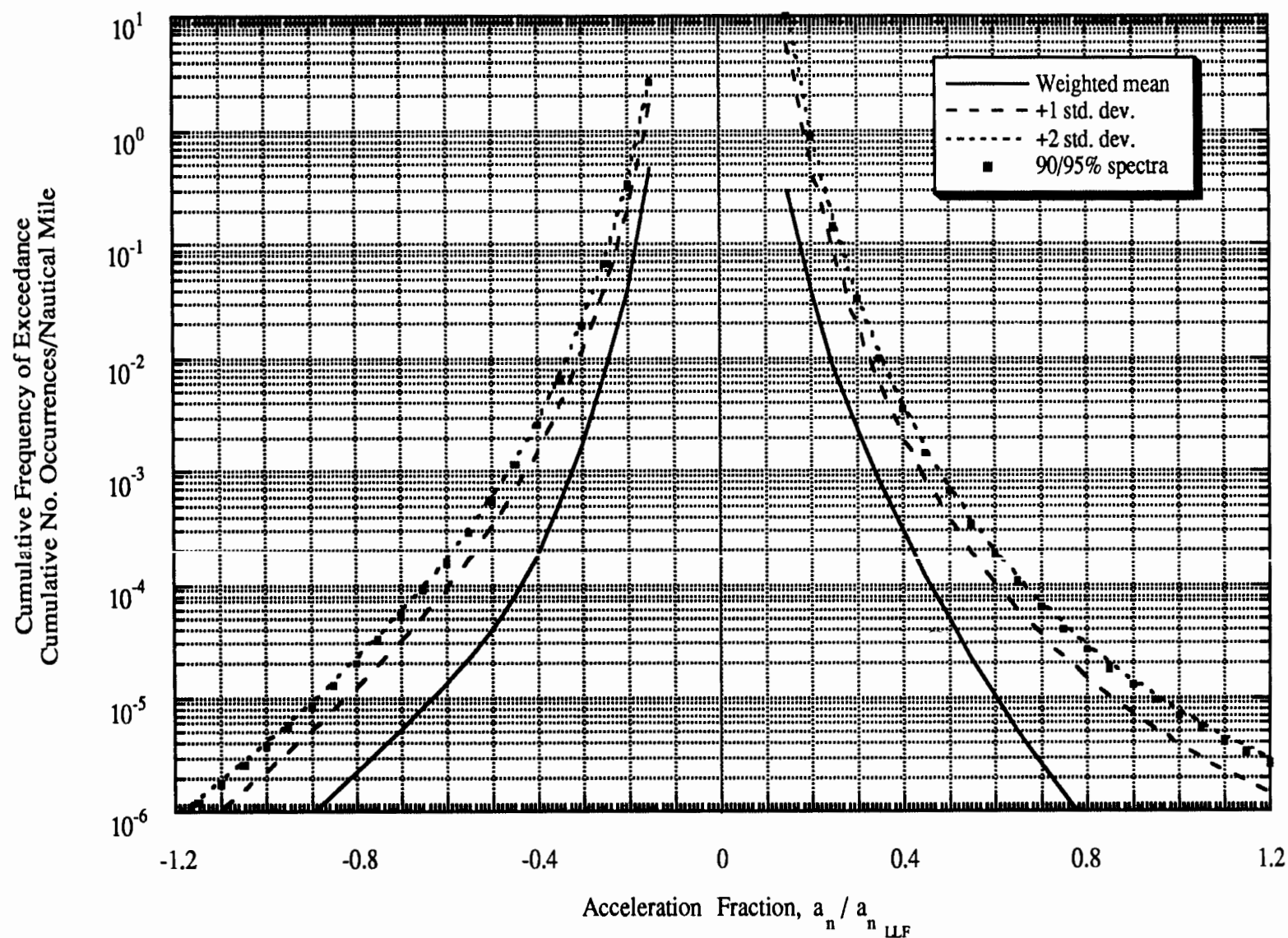
Figure 2-2 Gust Load Spectra: Single-Engine General Usage, Basic Flight Instruction
