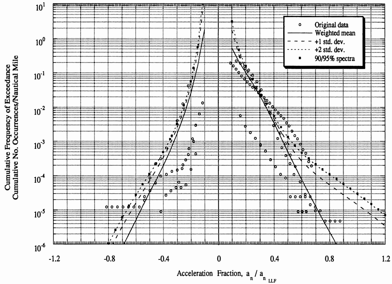
Figure D-8 Maneuver Load Spectra: Single-Engine Special Usage
