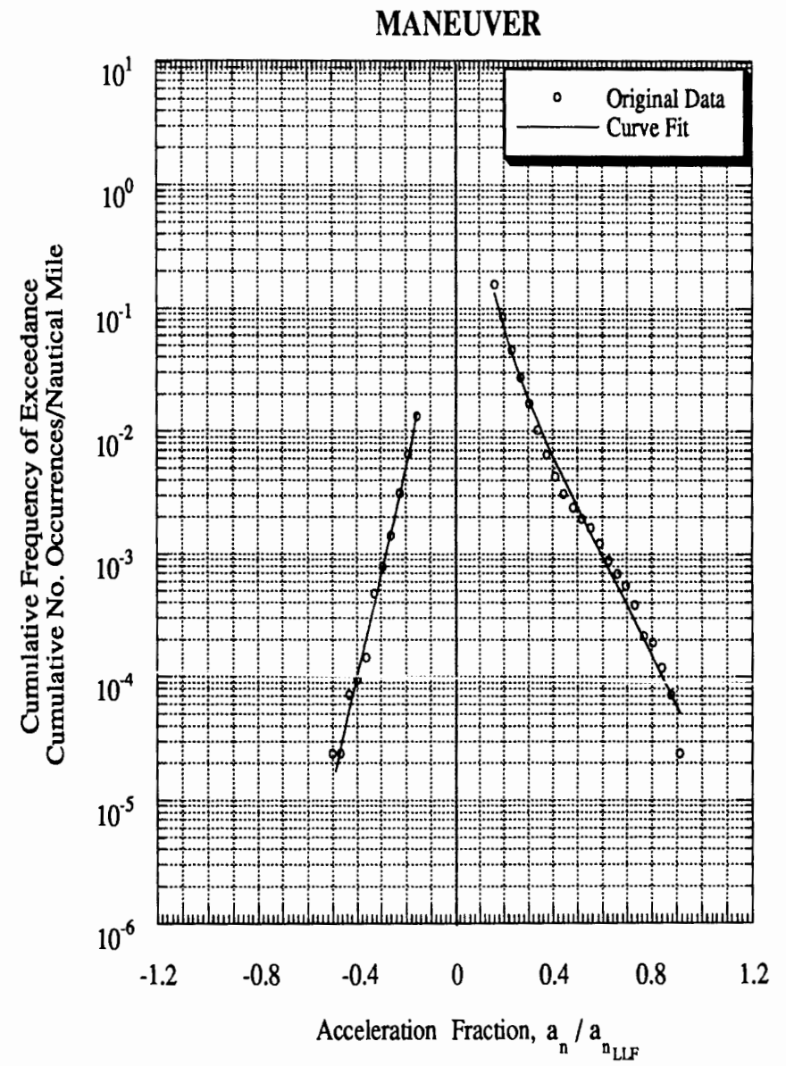
Figure C-4 Load Spectra for Airplane 14, Single-Engine, Basic Flight Instruction
