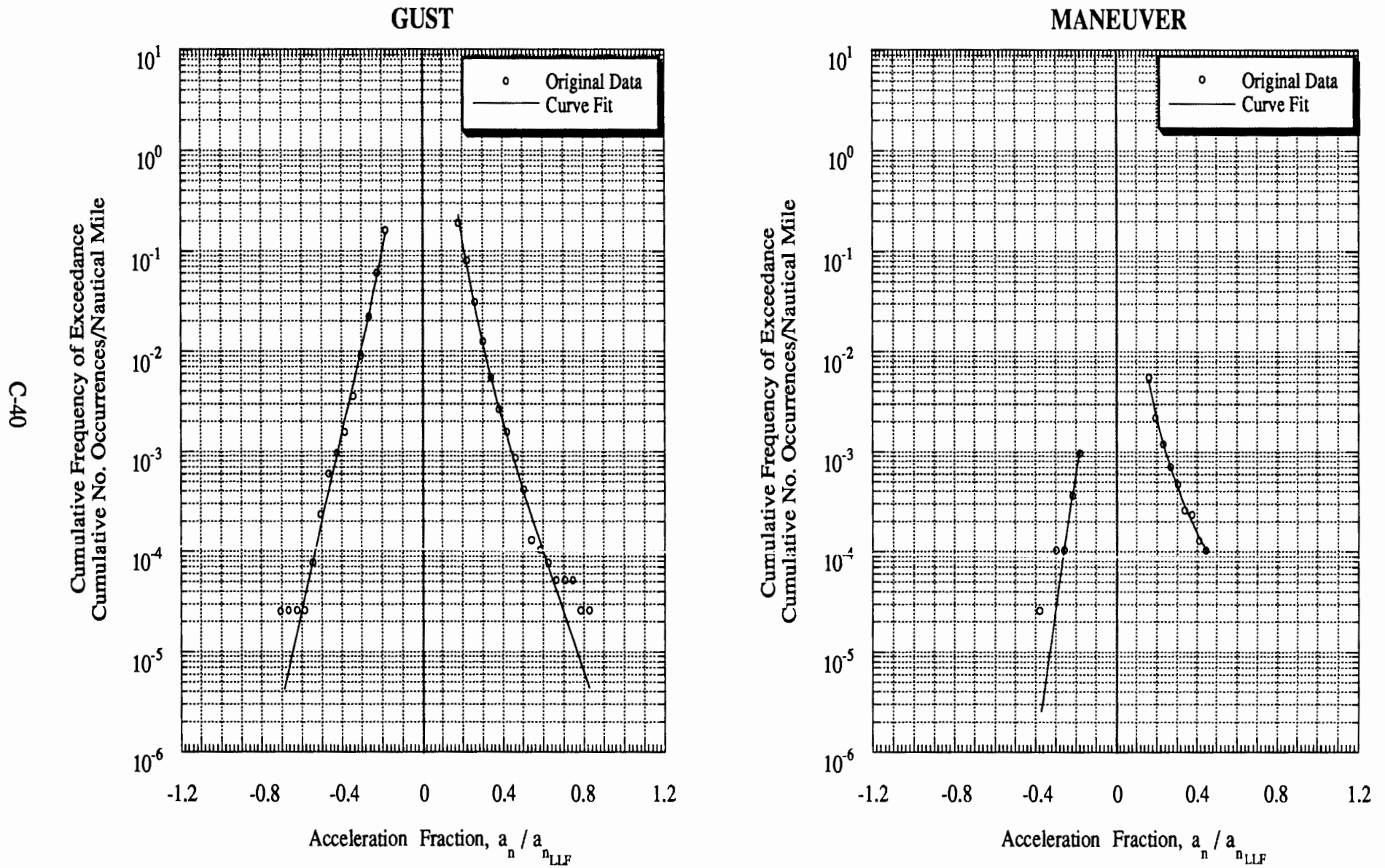
Figure C-17 Load Spectra for Airplane 8, Single-Engine, Business/Personal
