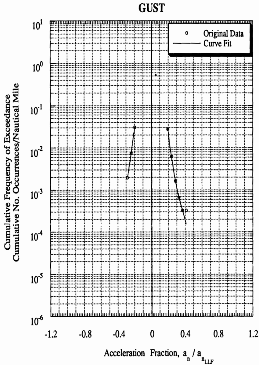
Figure C-26 Load Spectra for Airplane 12, Single-Engine, Business/Personal
