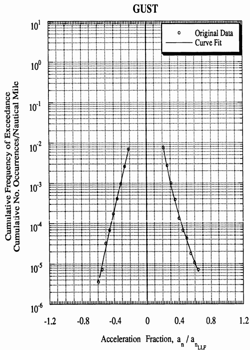
Figure C-77 Load Spectra for Airplane 3 1 , Pressurized, General Usage
