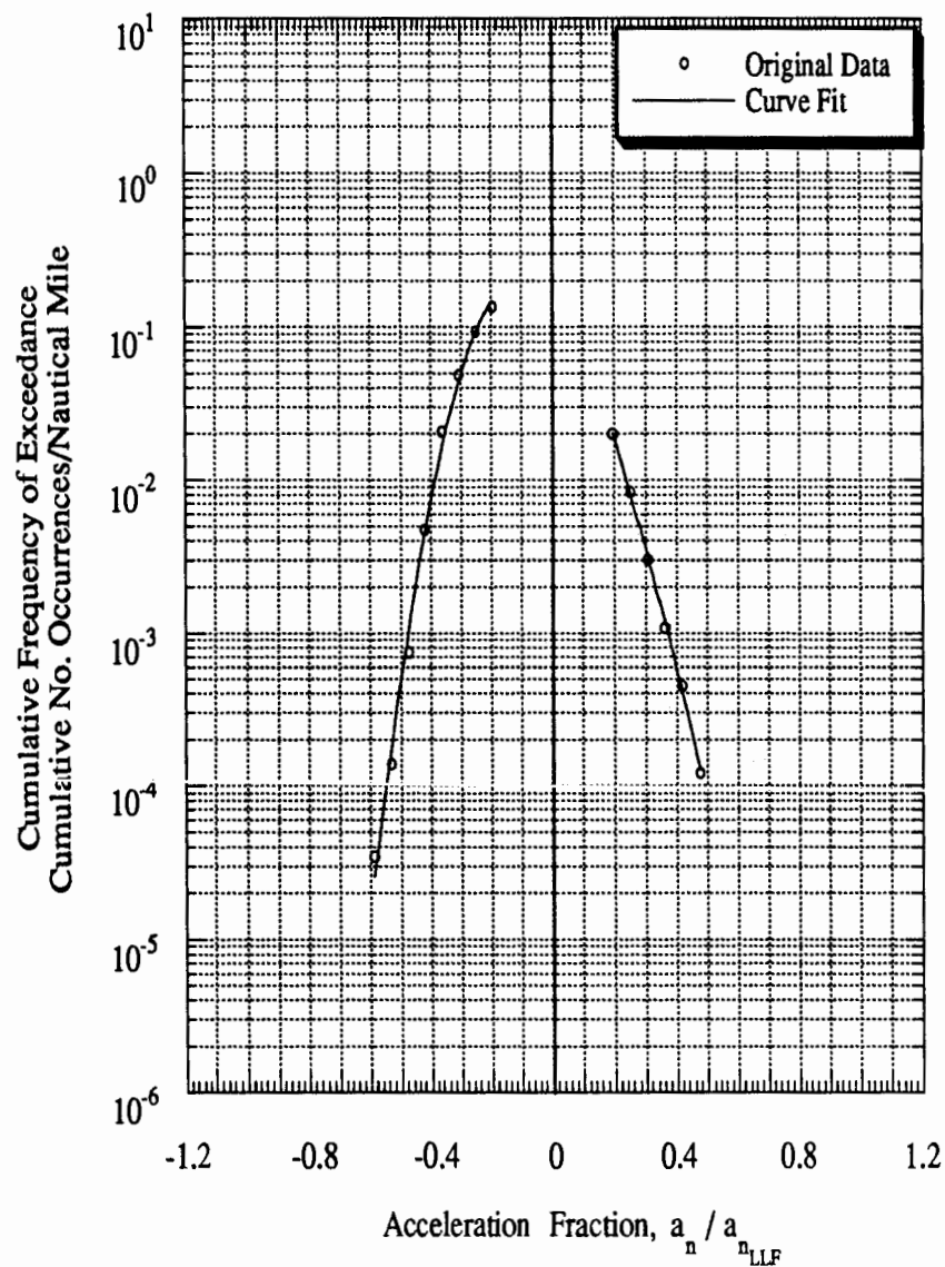
Figure C-87 Load Spectra for Airplane 20 1 , Large Airplanes, Special Usage
