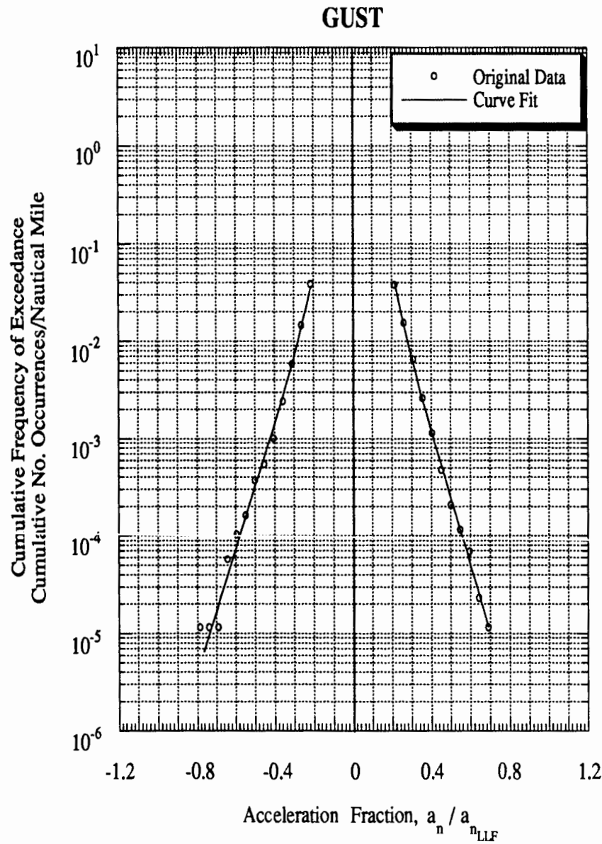
Figure C-66 Load Spectra for Airplane 5, Twin-Engine, General Usage
