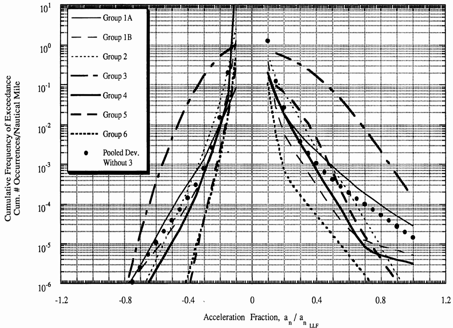
Figure E-12 Maneuver: Weighted Standard Deviation for Each Group and Pooled Without Group 3
