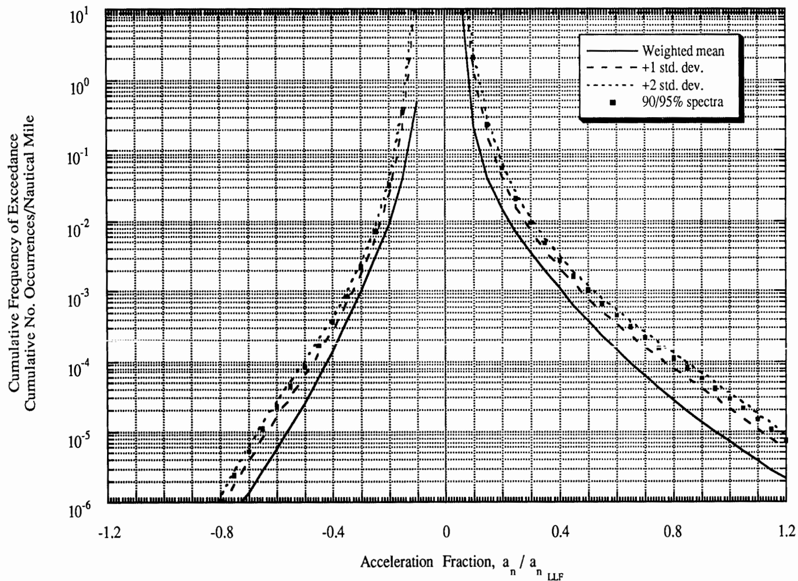
Figure 2-7 Maneuver Load Spectra: Single-Engine General Usage (Basic Flight Instruction and Business/Personal Combined)
