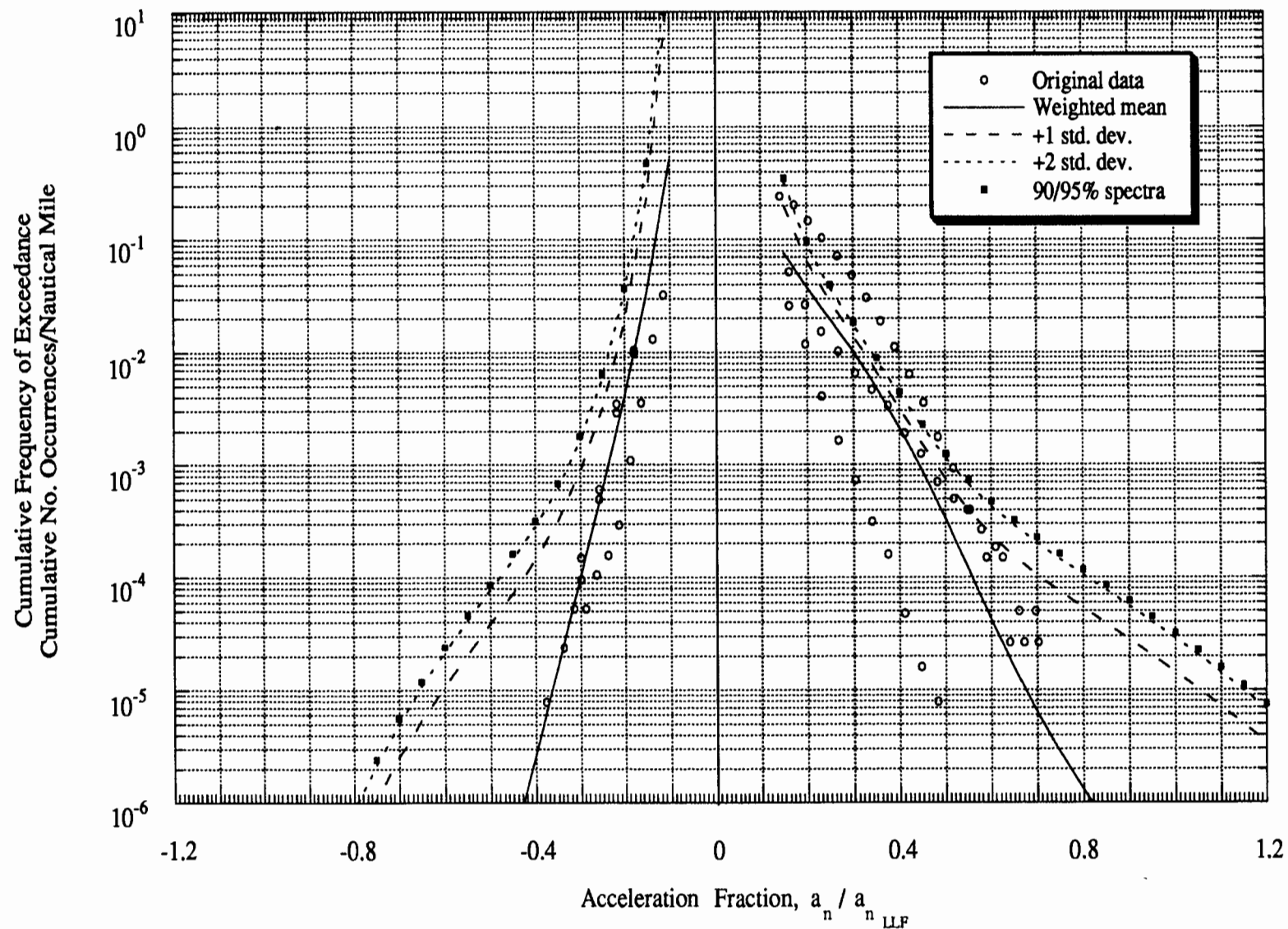
Figure D-14 Maneuver Load Spectra: Twin-Engine Special Usage
