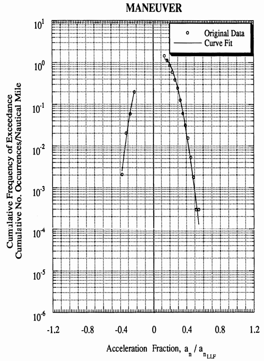
Figure C-51 Load Spectra for Airplane 33A, Aerial Application
