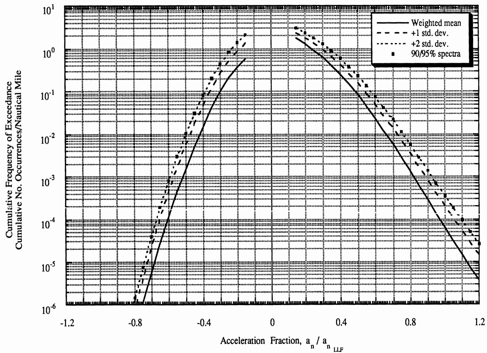
Figure 2-11 Maneuver Load Spectra: Single-Engine Aerial Application
