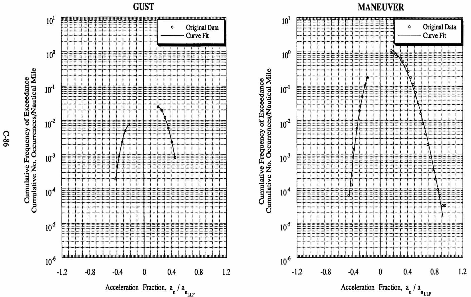
Figure C-40 Load Spectra for Airplane 29 1 , Aerial Application
