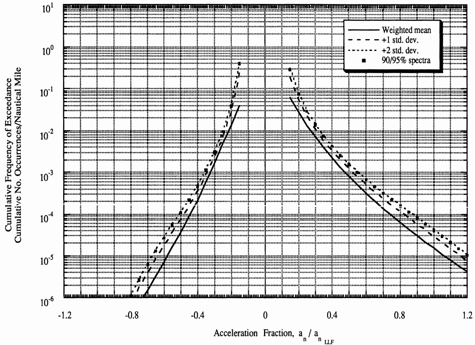
Figure 2-3 Maneuver Load Spectra: Single-Engine General Usage, Basic Flight Instruction
