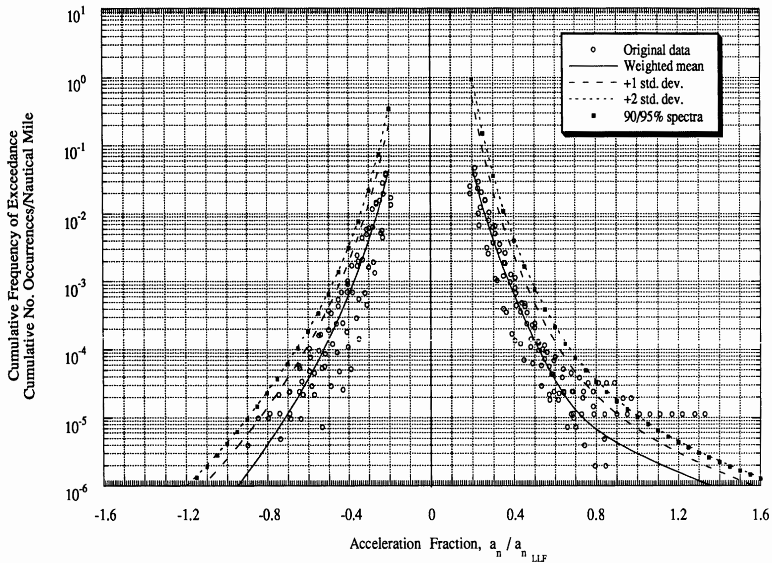
Figure D-11 Gust Load Spectra: Twin-Engine General Usage
