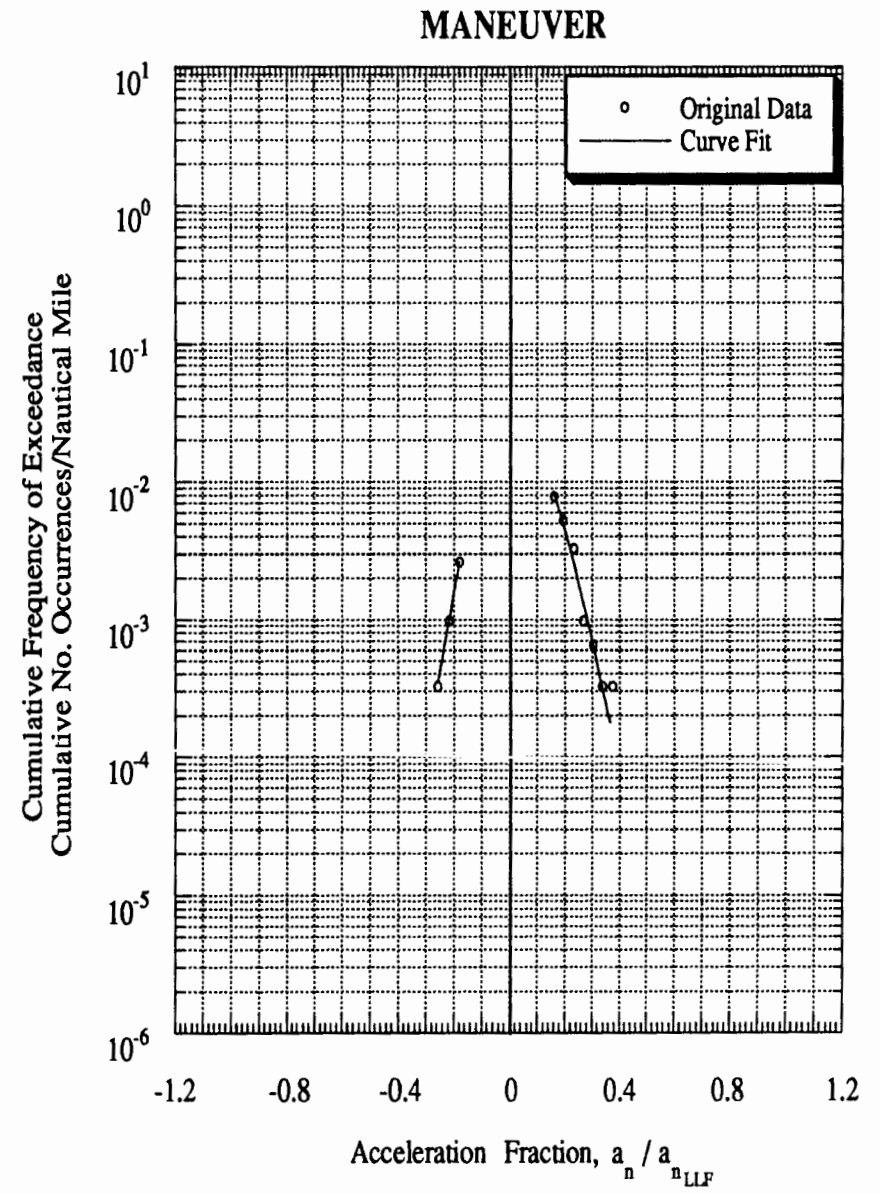
Figure C-26 Load Spectra for Airplane 12, Single-Engine, Business/Personal
