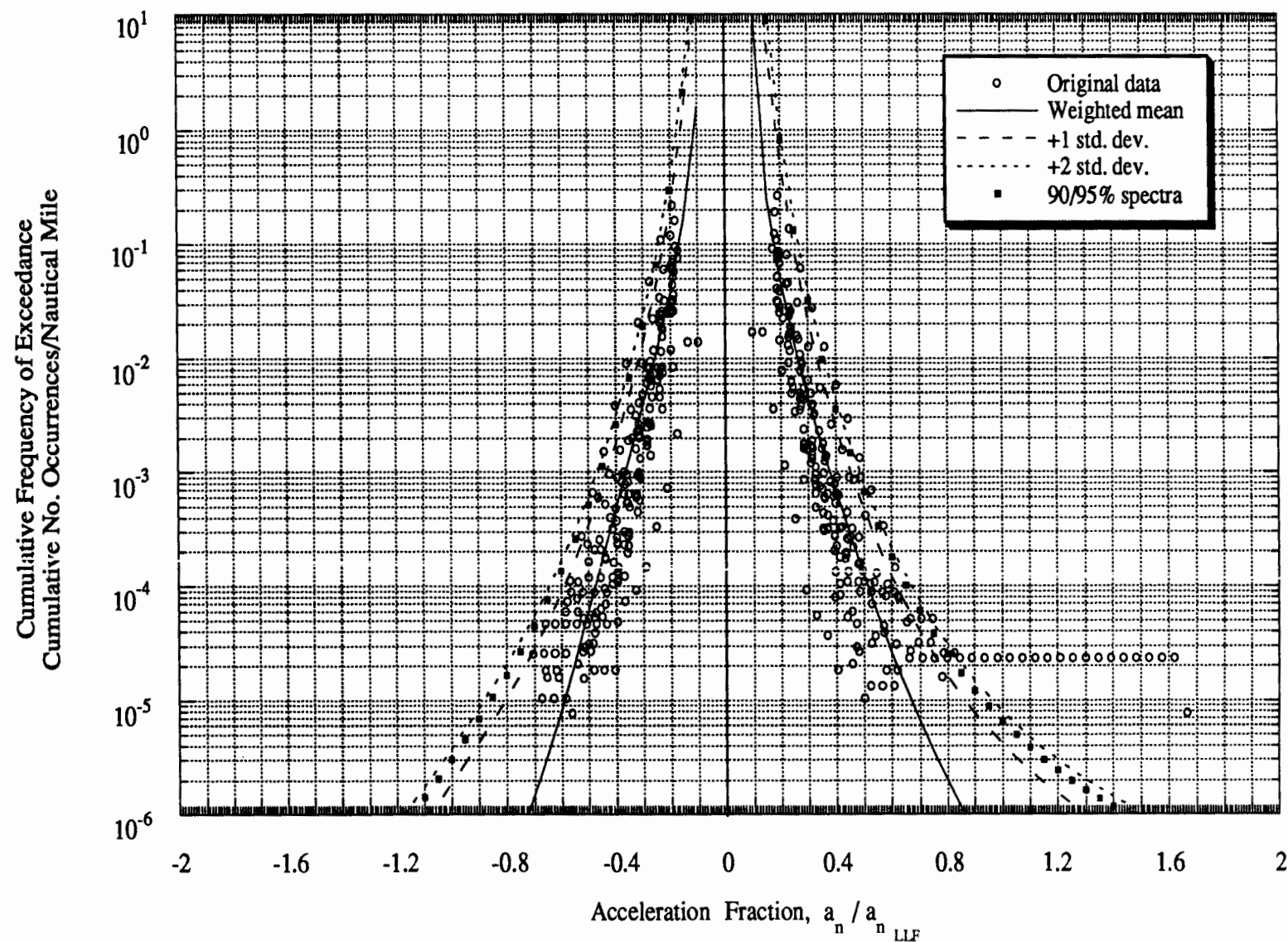
Figure D-3 Gust Load Spectra: Single-Engine General Usage, Business/Personal
