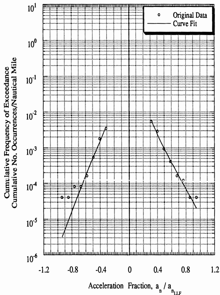
Figure C-84 Load Spectra for Airplane 19, Large Airplanes, Special Usage
