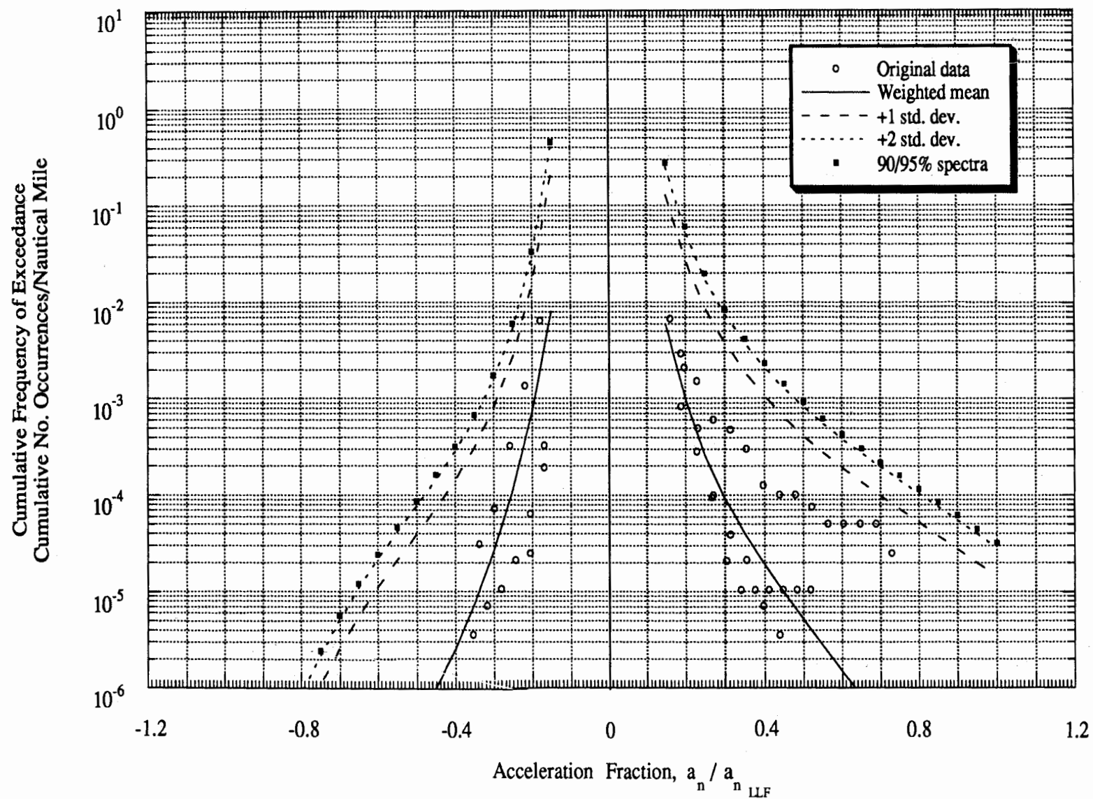
Figure D-18 Maneuver Load Spectra: Single and Twin-Engine Pressurized General Usage
