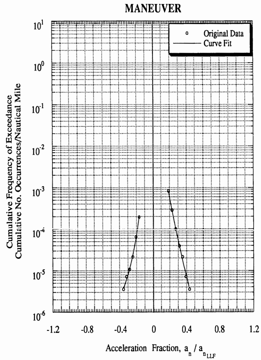
Figure C-77 Load Spectra for Airplane 3 1 , Pressurized, General Usage
