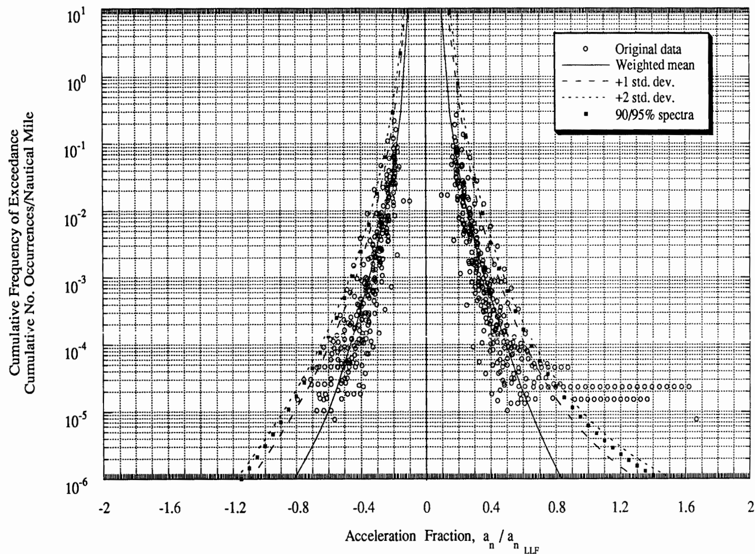
Figure D-5 Gust Load Spectra: Single Engine General Usage (Basic Flight Instruction and Business/Personal Combined)
