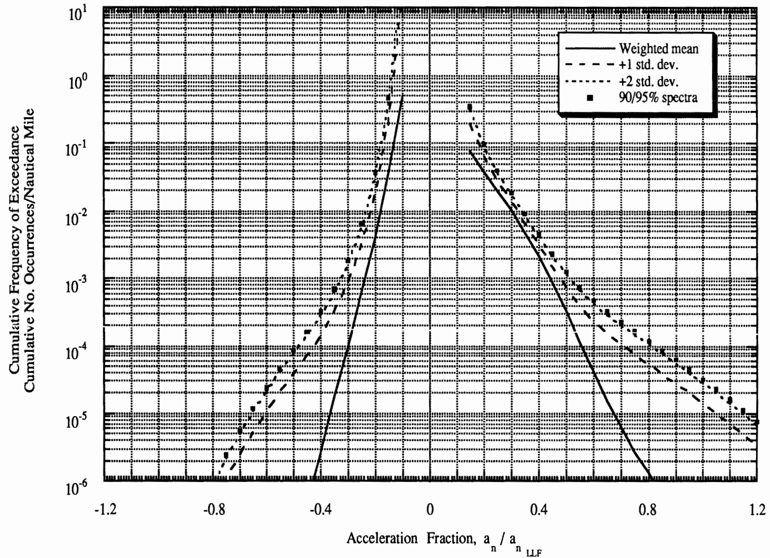
Figure 2-15 Maneuver Load Spectra: Twin-Engine Special Usage
