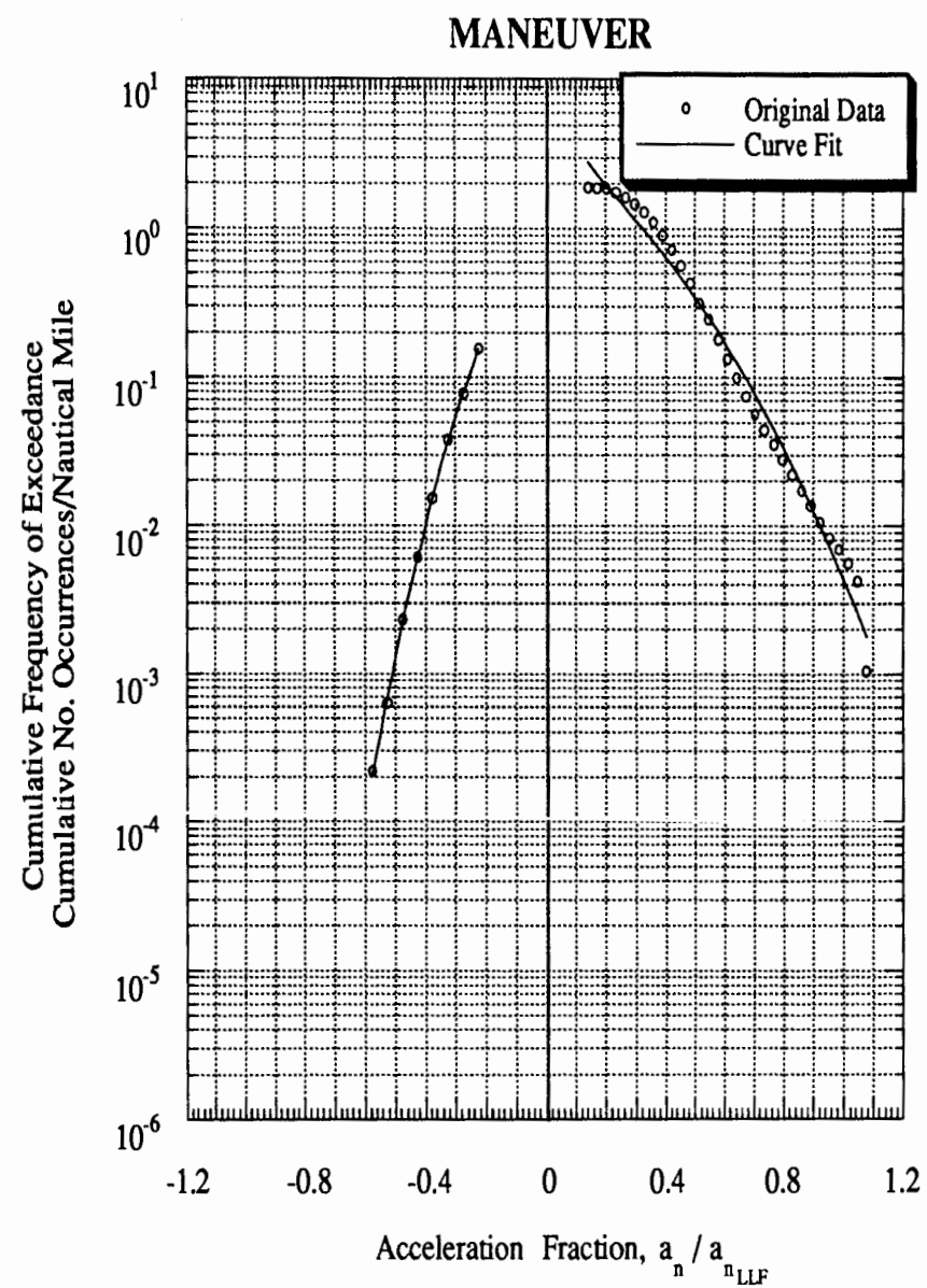
Figure C-47 Load Spectra for Airplane 32 1 , Aerial Application
