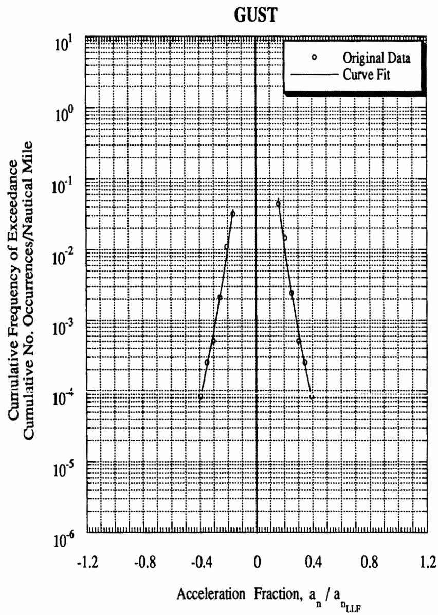
Figure C-91 Load Spectra for Airplane 24, Large Airplanes, Special Usage
