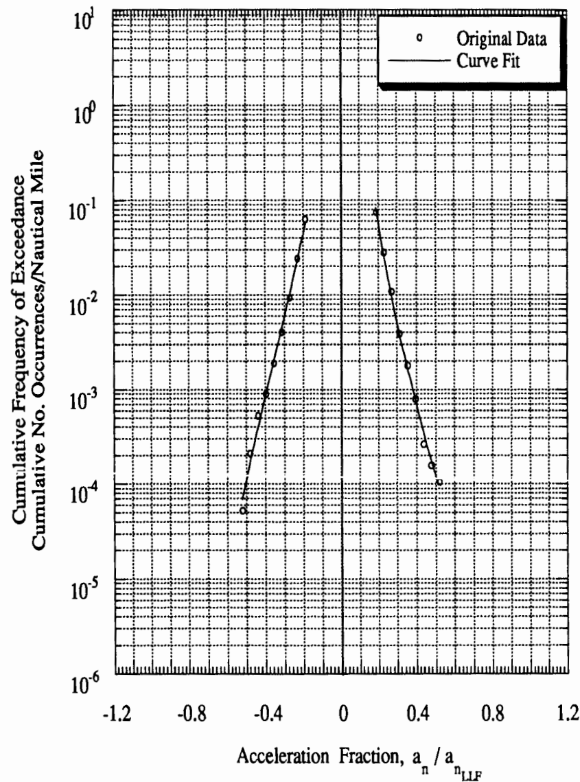
Figure C-16 Load Spectra for Airplane 7C 1 , Single-Engine, Business/Personal
