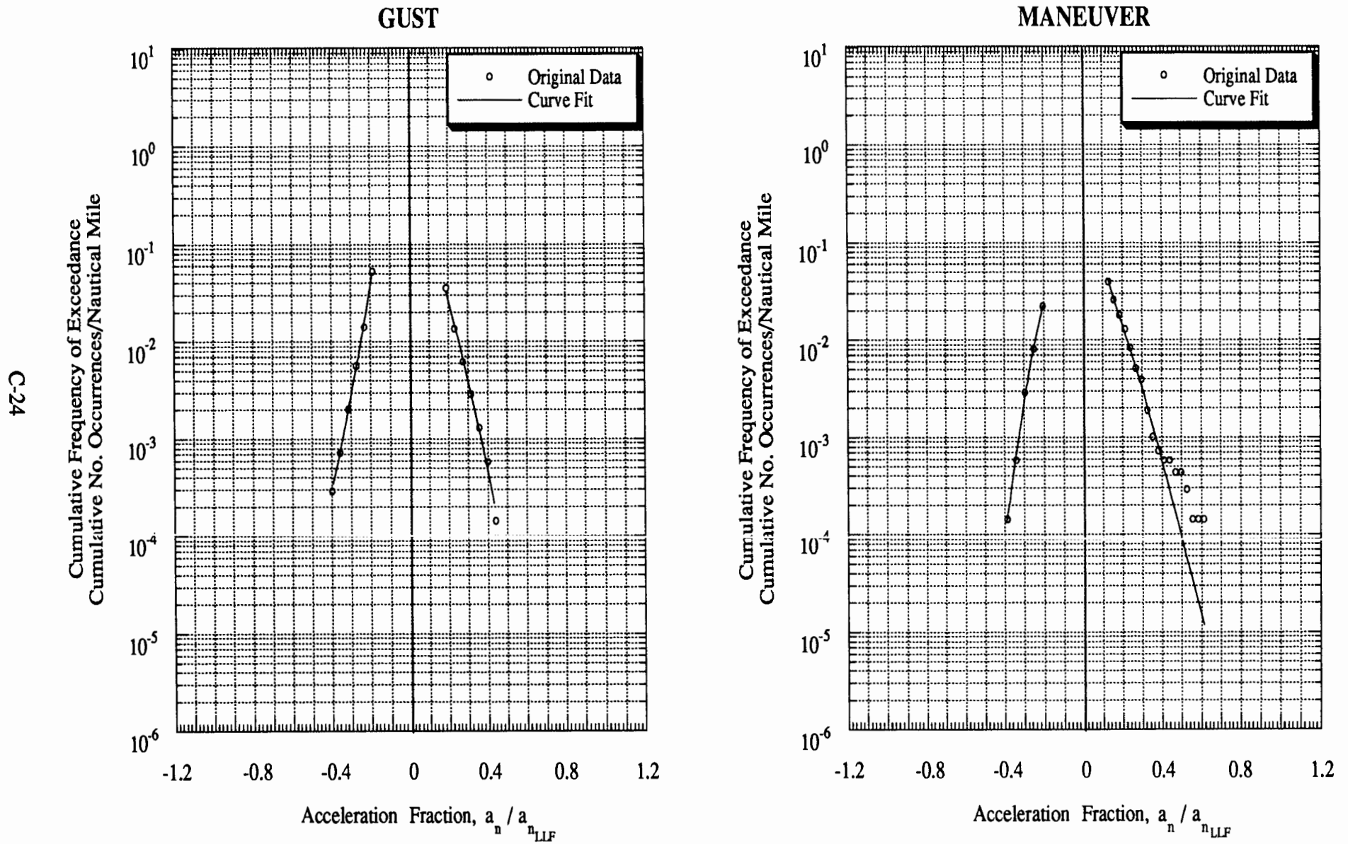
Figure C-9 Load Spectra for Airplane 18, Single-Engine, Basic Flight Instruction
