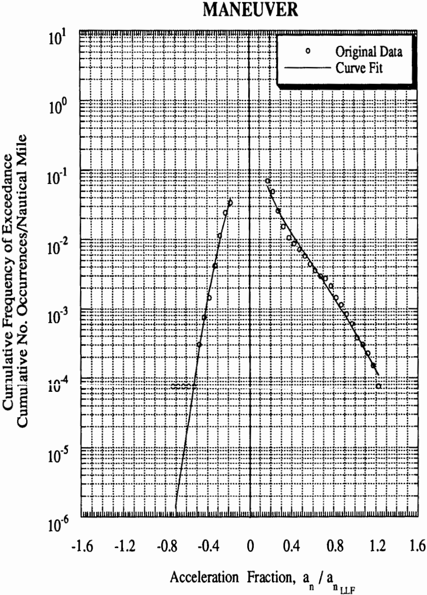
Figure C-96 Load Spectra for Airplane 24 5 , Large Airplanes, Special Usage
