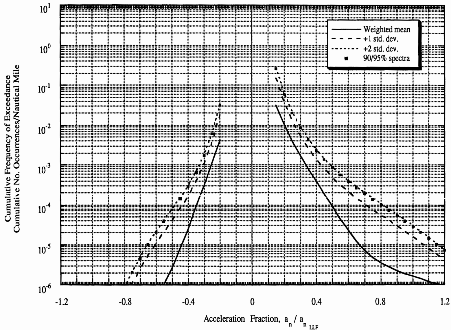
Figure 2-13 Maneuver Load Spectra: Twin-Engine General Usage
