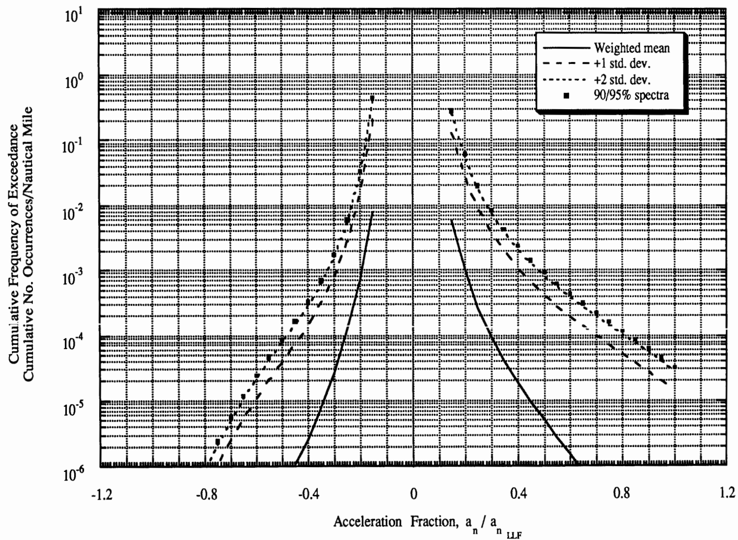
Figure 2-19 Maneuver Load Spectra: Single and Twin-Engine Pressurized General Usage
