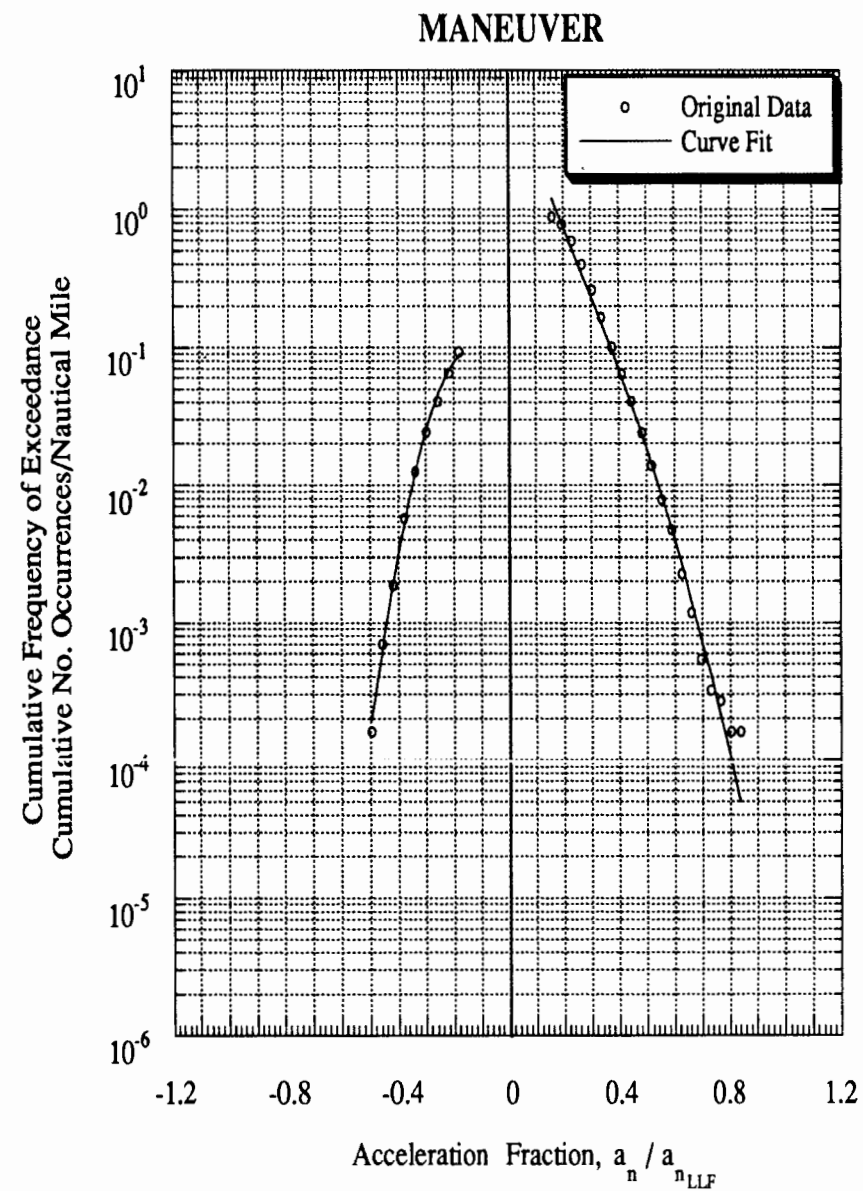
Figure C-61 Load Spectra for Airplane 36, Aerial Application
