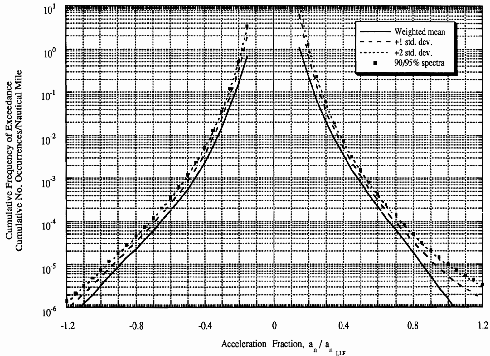
Figure 2-14 Gust Load Spectra: Twin-Engine Special Usage
