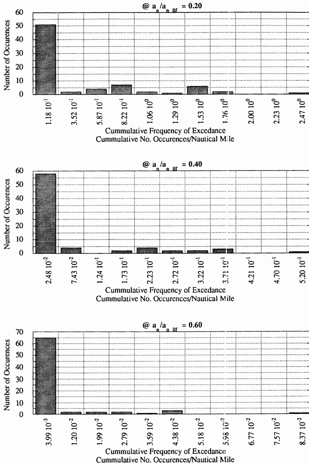
Figure E-7 Normal Histogram: Positive Maneuver, All Statistical Aircraft
