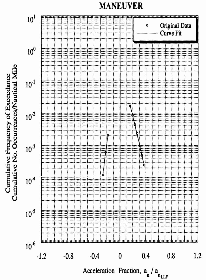
Figure C-28 Load Spectra for Airplane 12 2 , Single-Engine, Business/Personal
