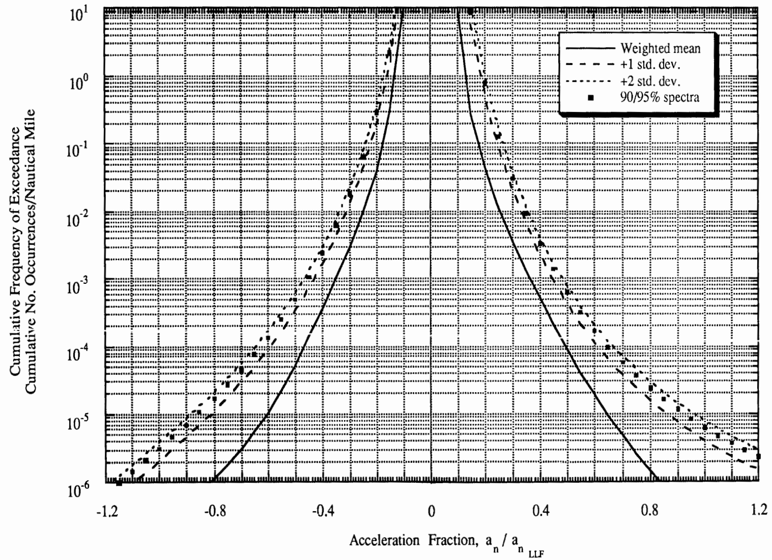
Figure 2-6 Gust Load Spectra: Single Engine General Usage (Basic Flight Instruction and Business/Personal Combined)
