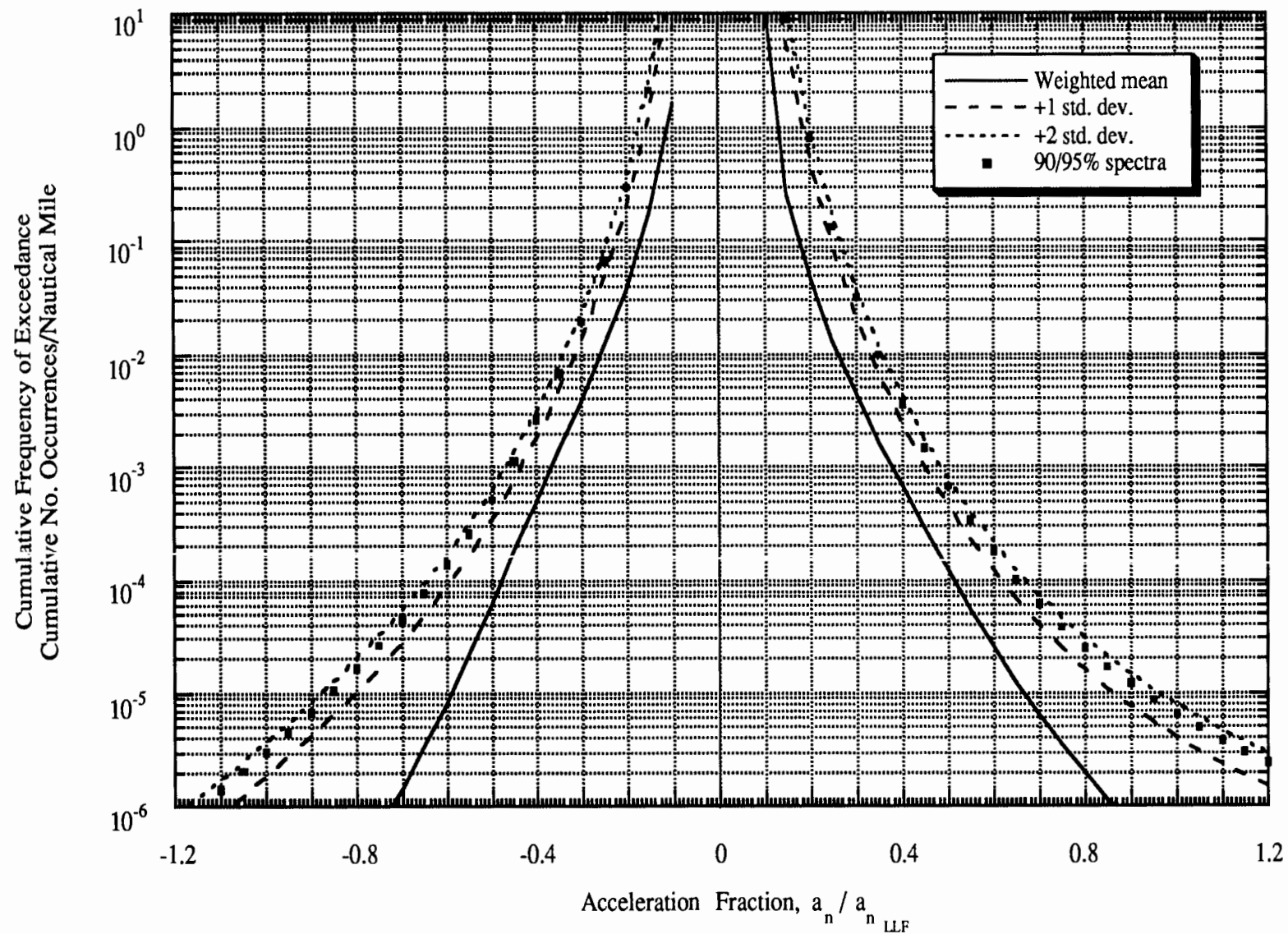
Figure 2-4 Gust Load Spectra: Single-Engine General Usage, Business/Personal
