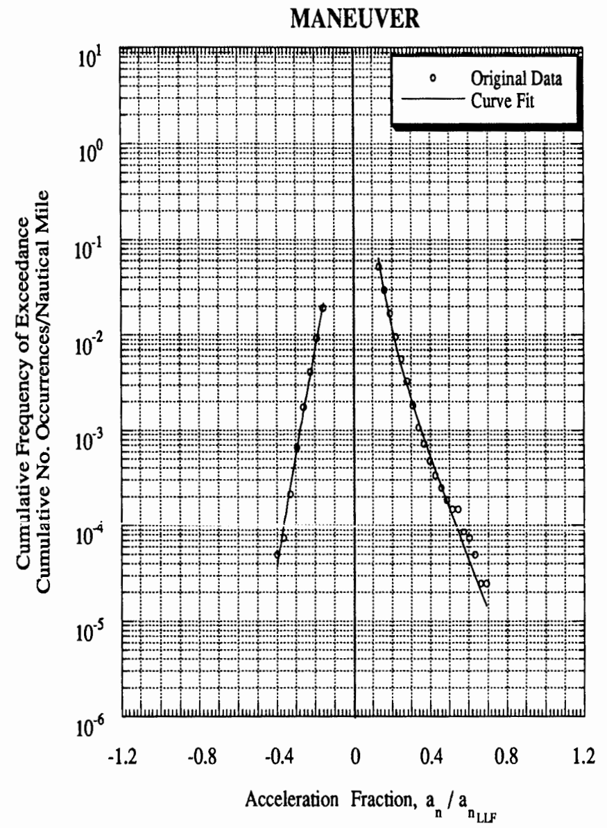
Figure C-5 Load Spectra for Airplane 14A, Single-Engine, Basic Flight Instruction
