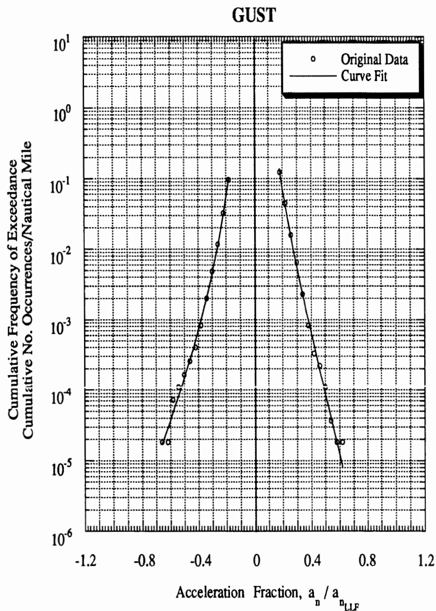
Figure C-21 Load Spectra for Airplane 9A, Single-Engine, Business/Personal
