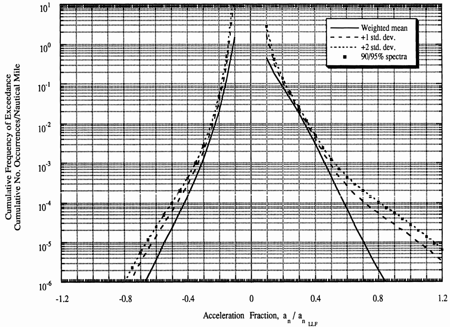
Figure 2-17 Maneuver Load Spectra: Single and Twin-Engine Special Usage
