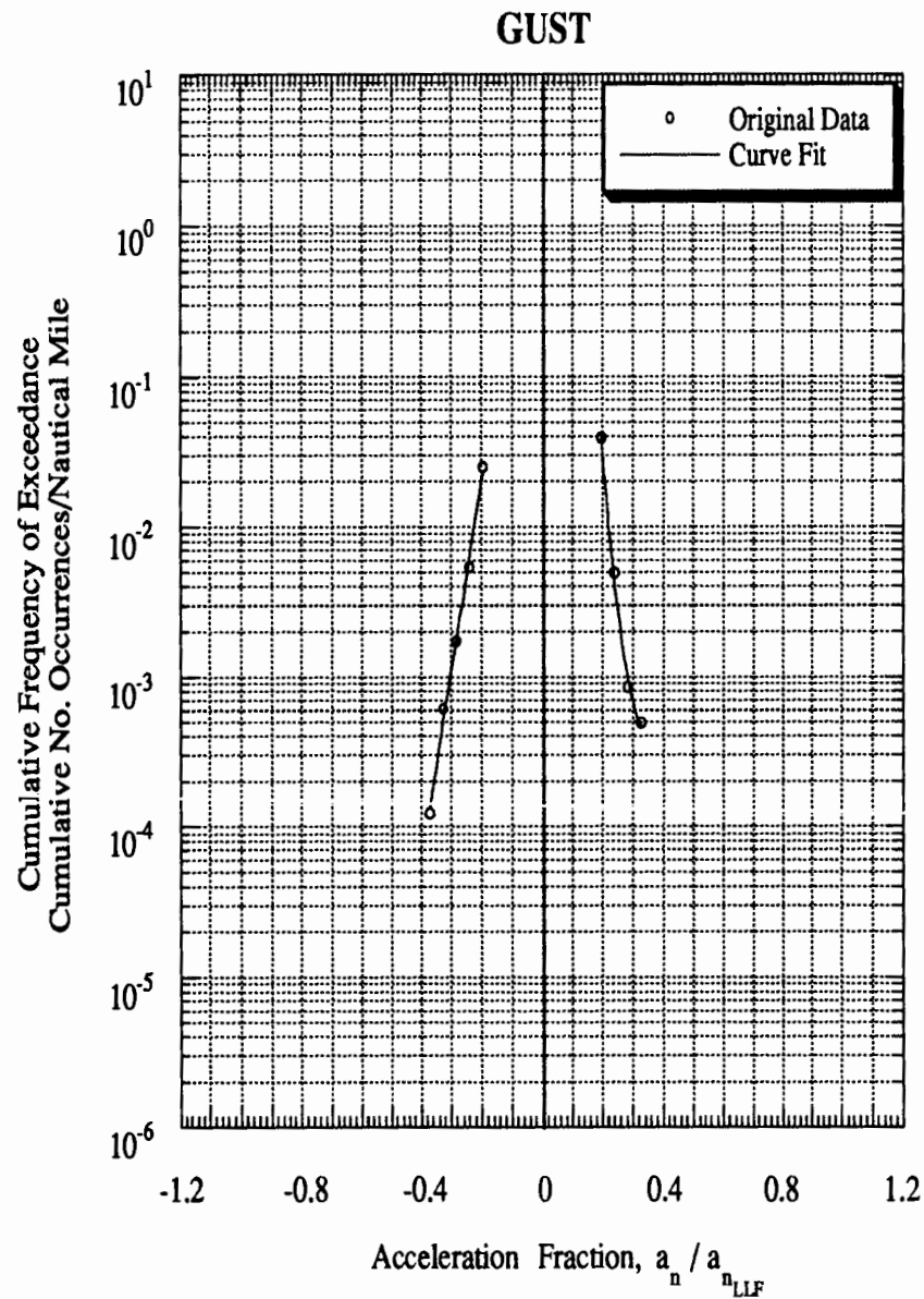
Figure C-28 Load Spectra for Airplane 12 2 , Single-Engine, Business/Personal
