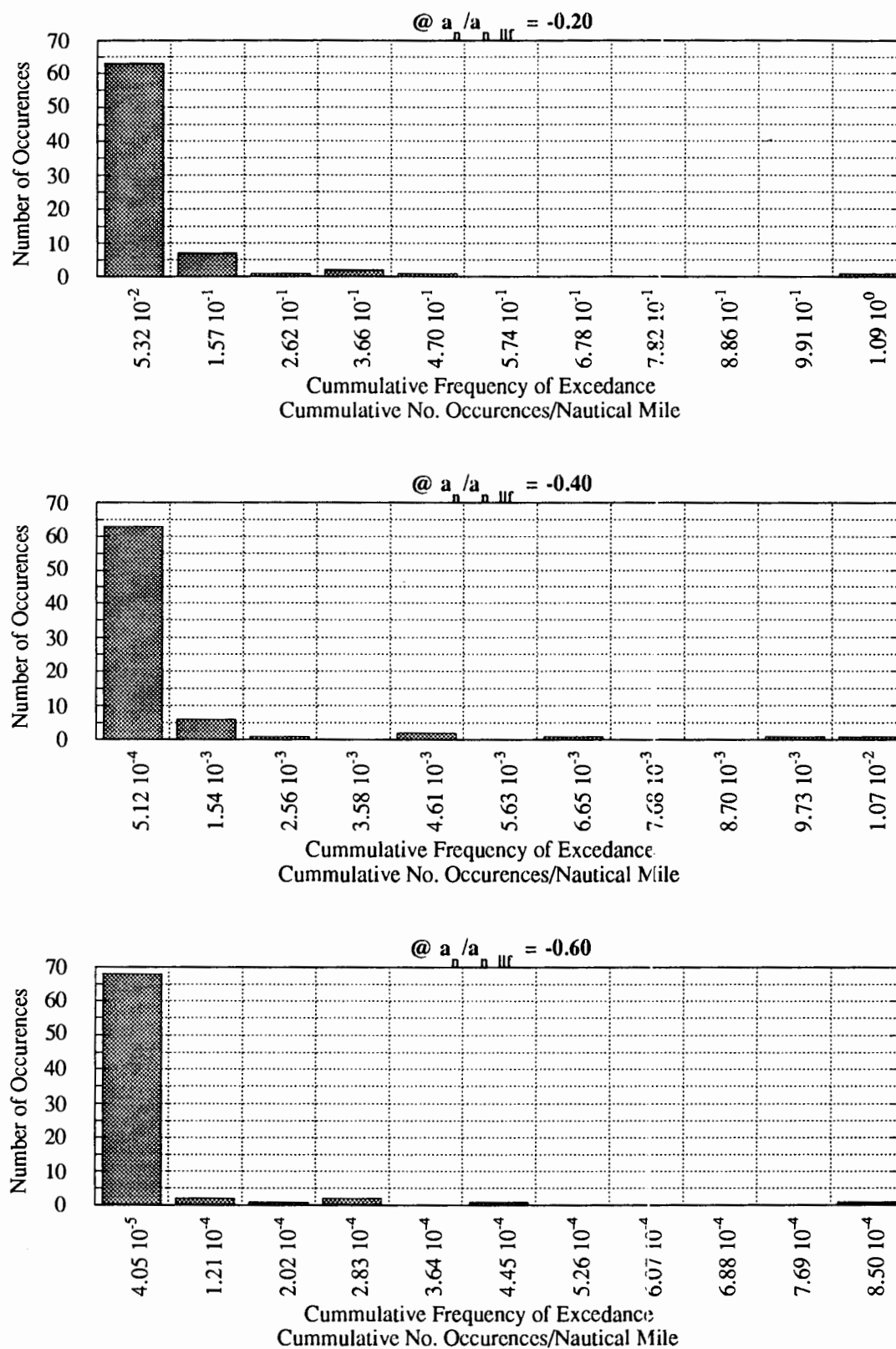
Figure E-1 Normal Histogram: Negative Gust, All Statistical Aircraft
