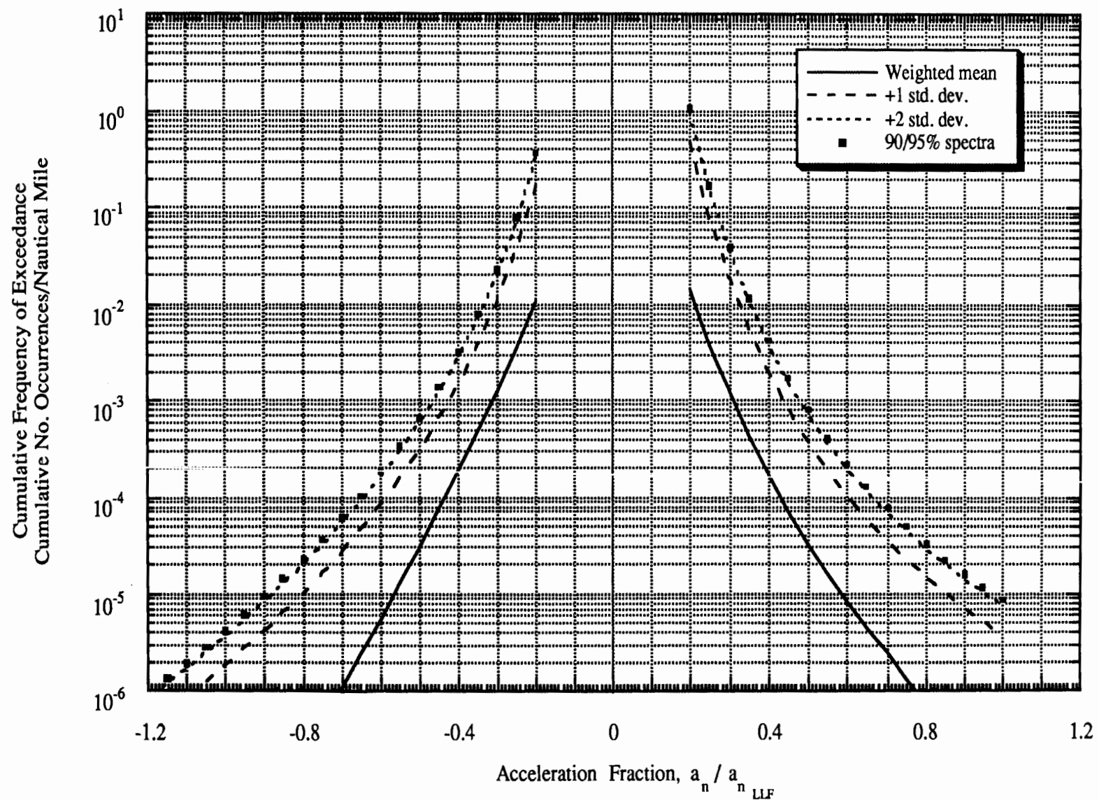
Figure 2-18 Gust Load Spectra: Single and Twin-Engine Pressurized General Usage
