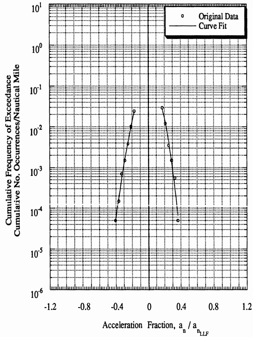
Figure C-73 Load Spectra for Airplane 4 1 , Twin-Engine, Special Usage
