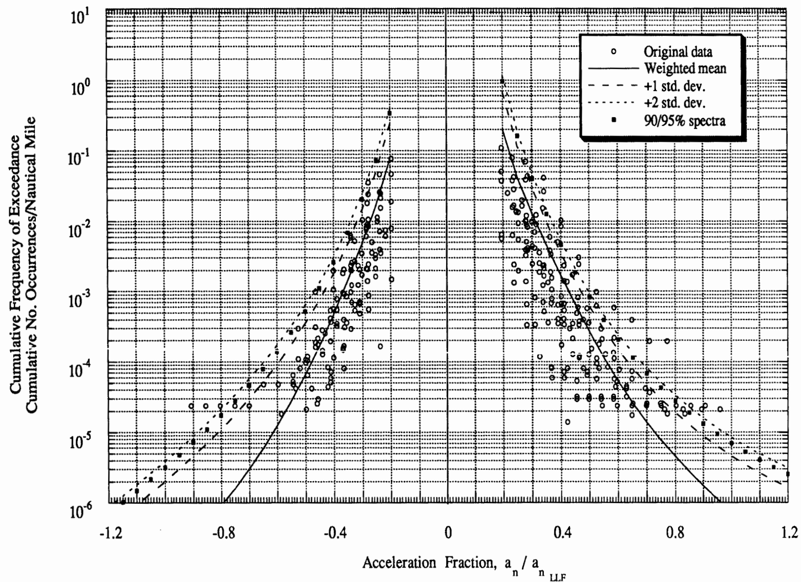
Figure D-9 Gust Load Spectra: Single-Engine Aerial Application
