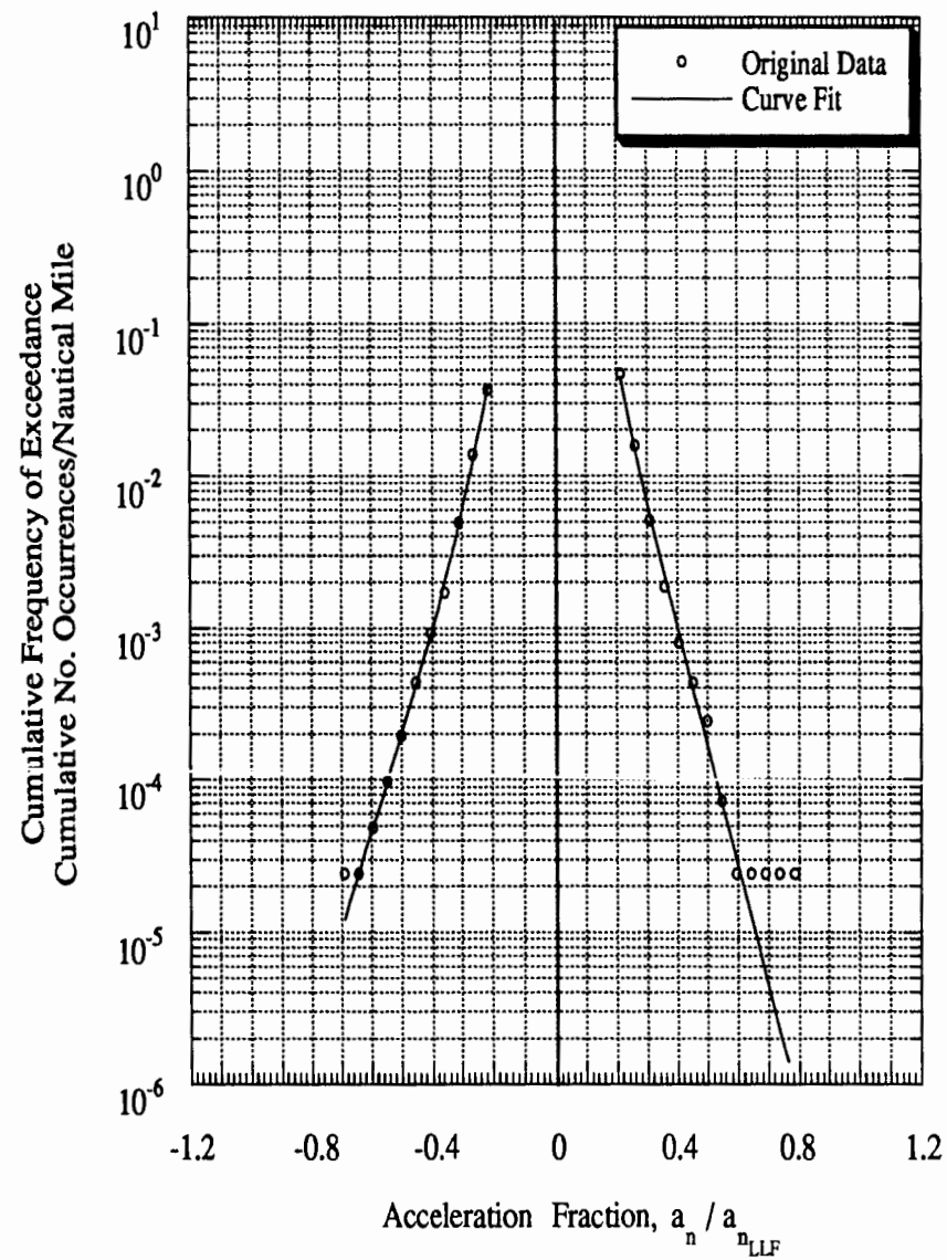
Figure C-67 Load Spectra for Airplane 5 1 , Twin-Engine, General Usage
