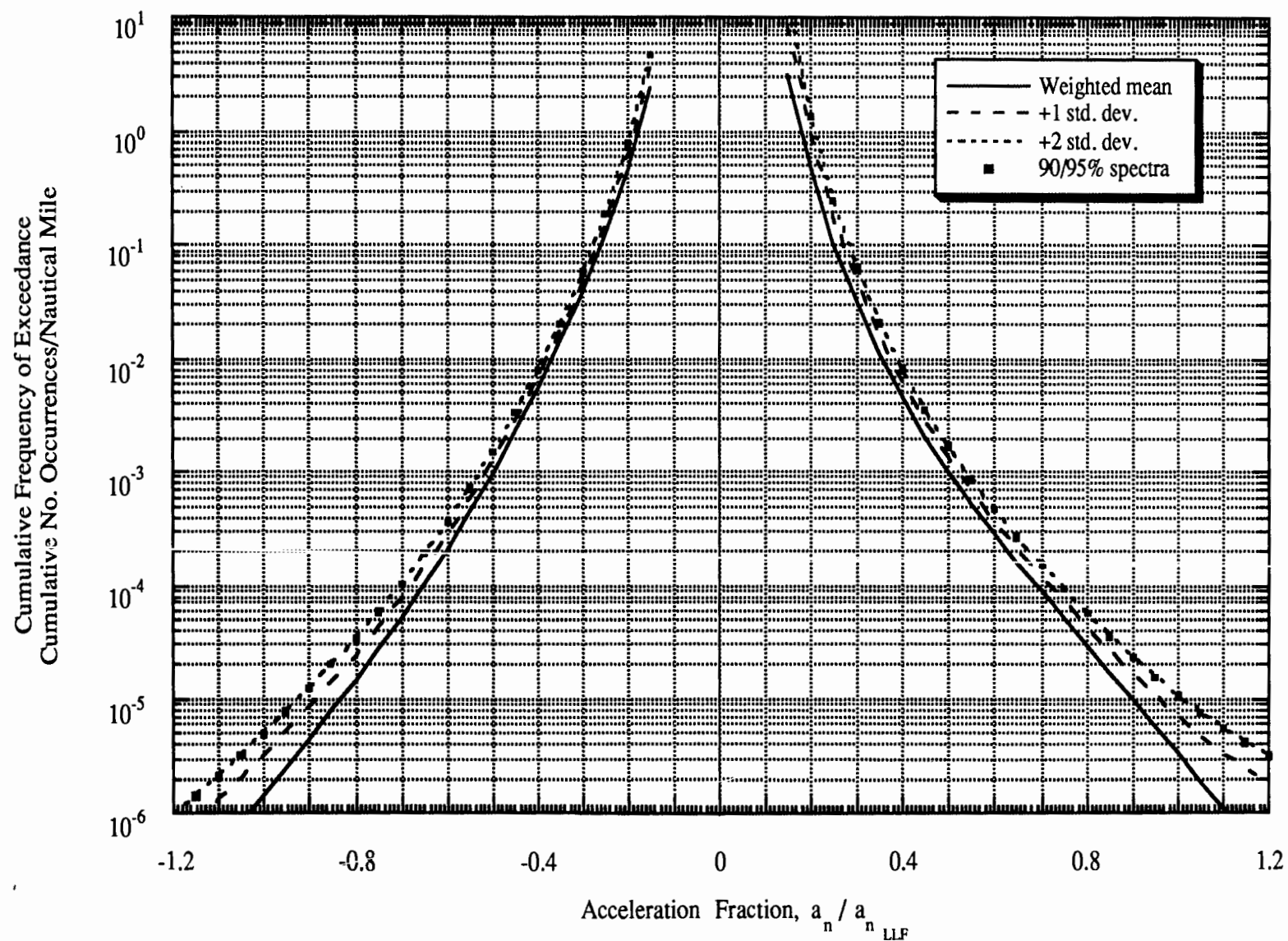
Figure 2-16 Gust Load Spectra: Single and Twin-Engine Special Usage
