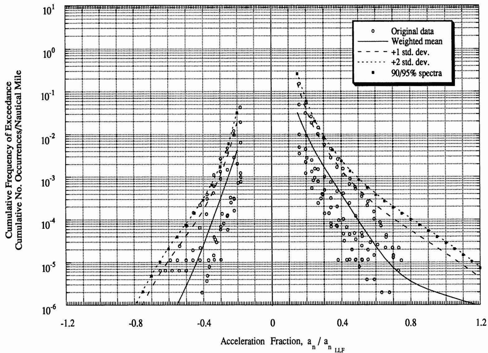
Figure D-12 Maneuver Load Spectra: Twin-Engine General Usage
