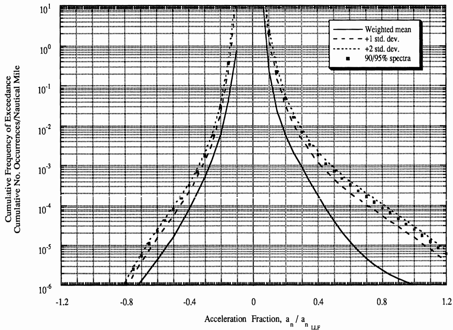
Figure 2-5 Maneuver Load Spectra: Single-Engine General Usage, Business/Personal
