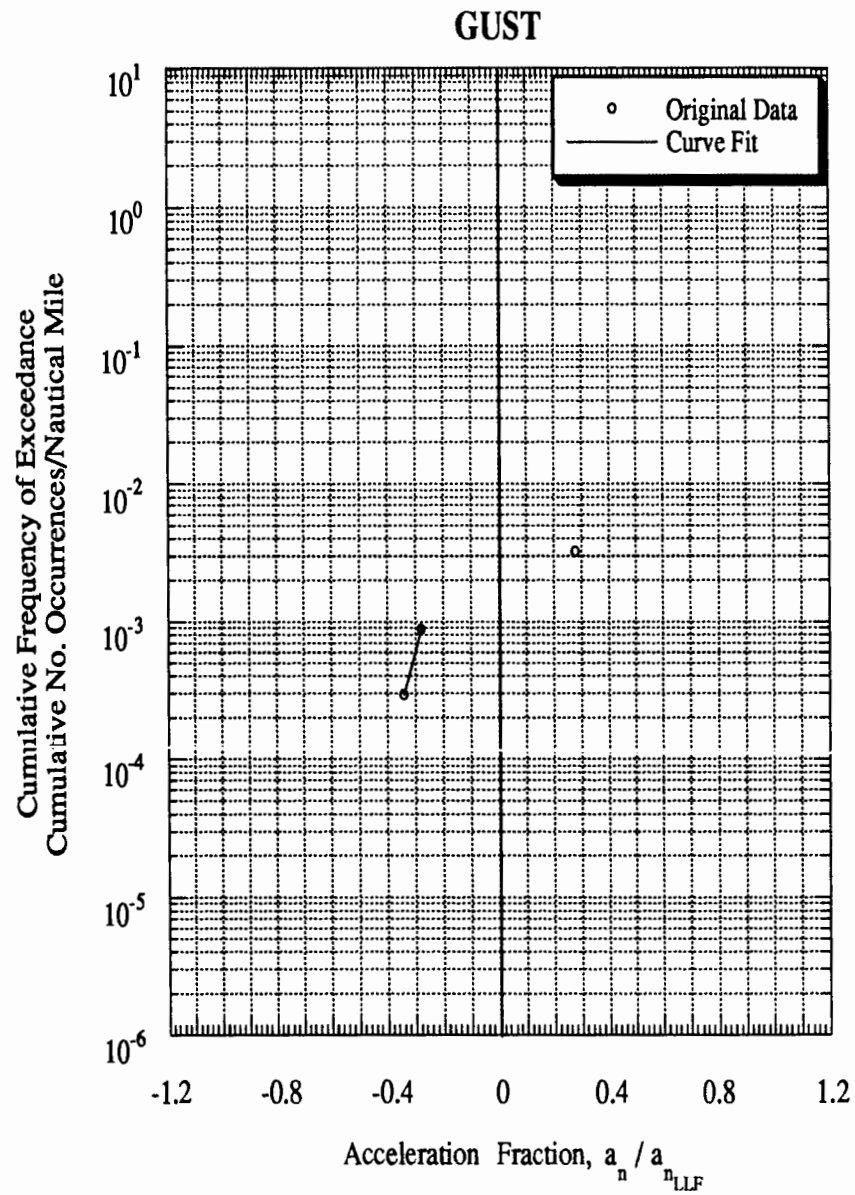
Figure C-51 Load Spectra for Airplane 33A, Aerial Application
