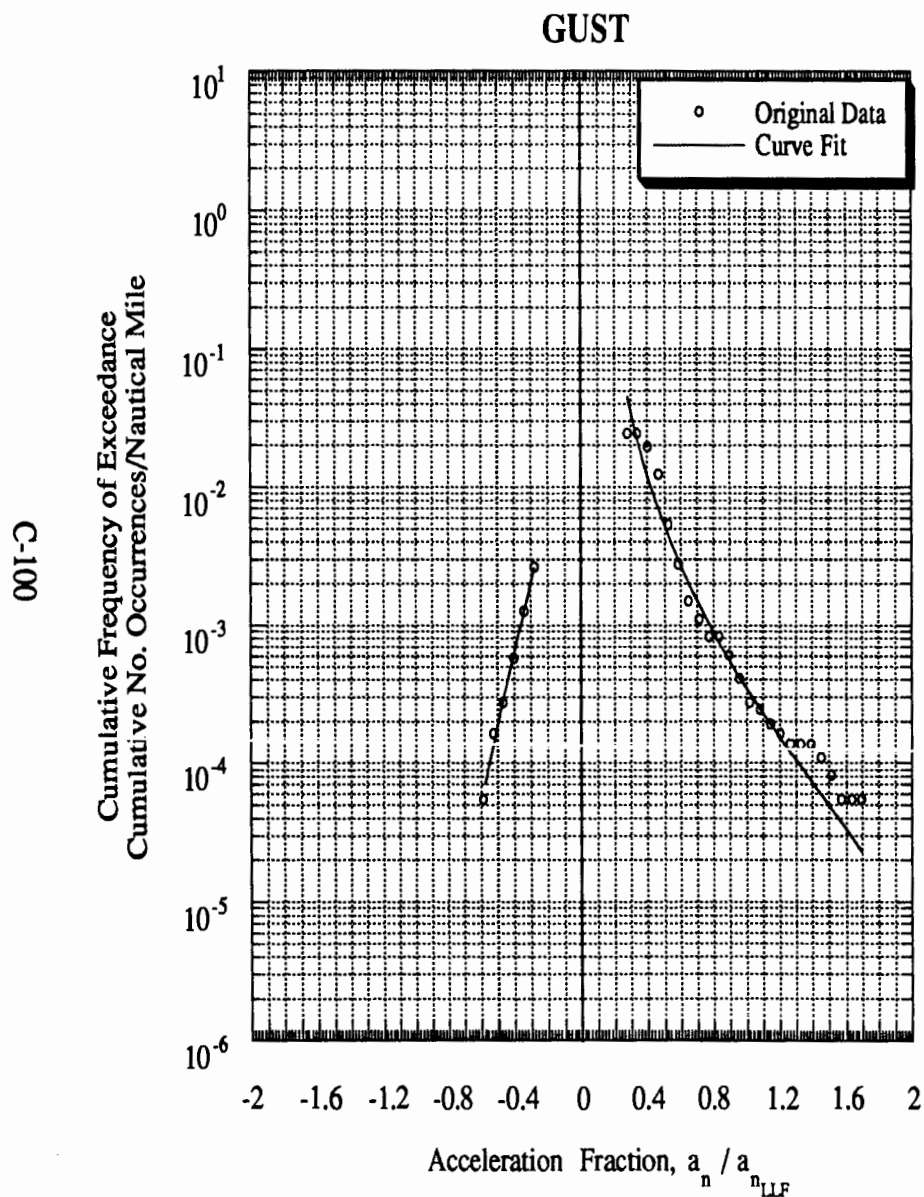
Figure C-47 Load Spectra for Airplane 32 1 , Aerial Application
