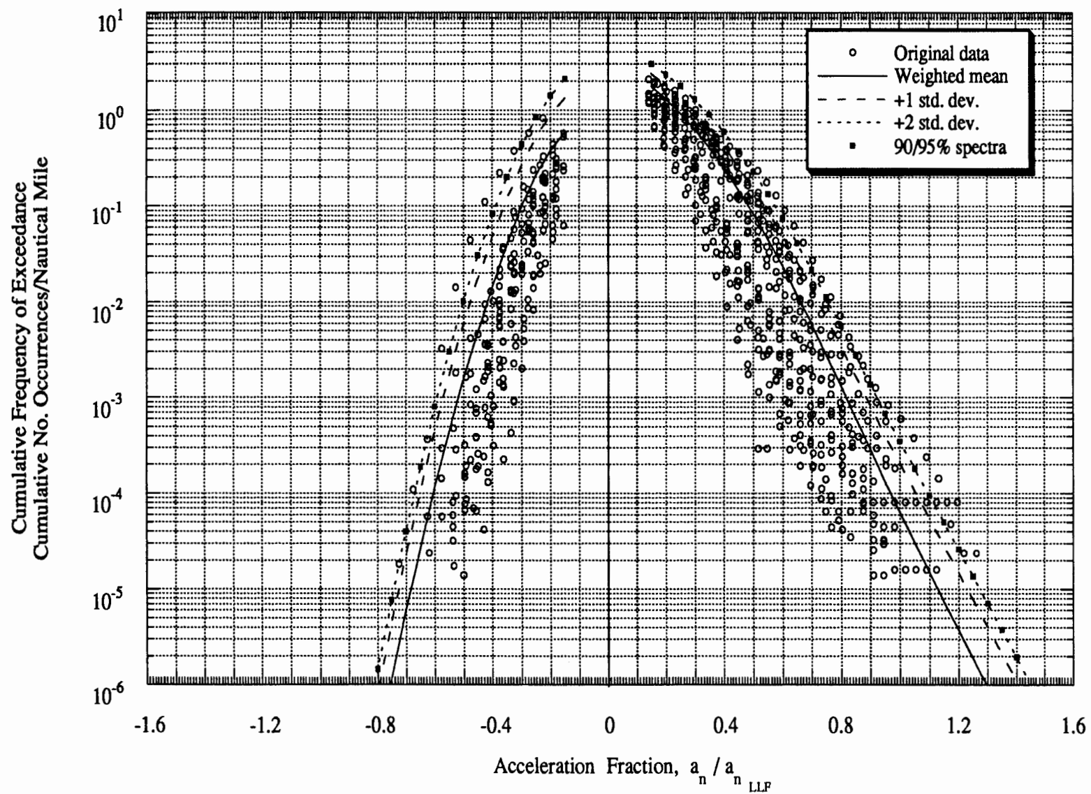
Figure D-10 Maneuver Load Spectra: Single-Engine Aerial Application
