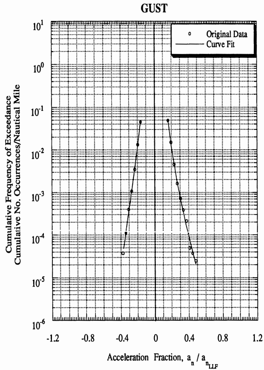
Figure C-5 Load Spectra for Airplane 14A, Single-Engine, Basic Flight Instruction
