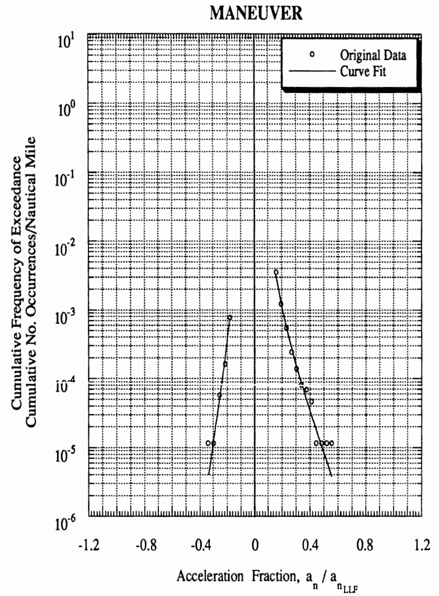
Figure C-66 Load Spectra for Airplane 5, Twin-Engine, General Usage
