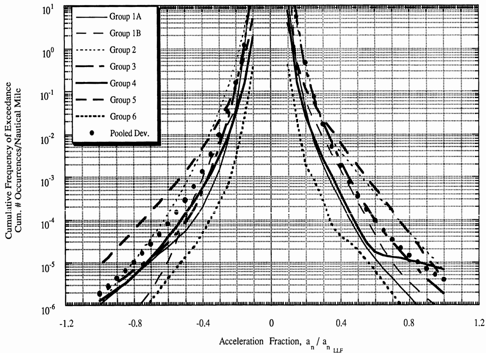
Figure E-13 Gust:Weighted Standard Deviation for Each Group and Pooled
