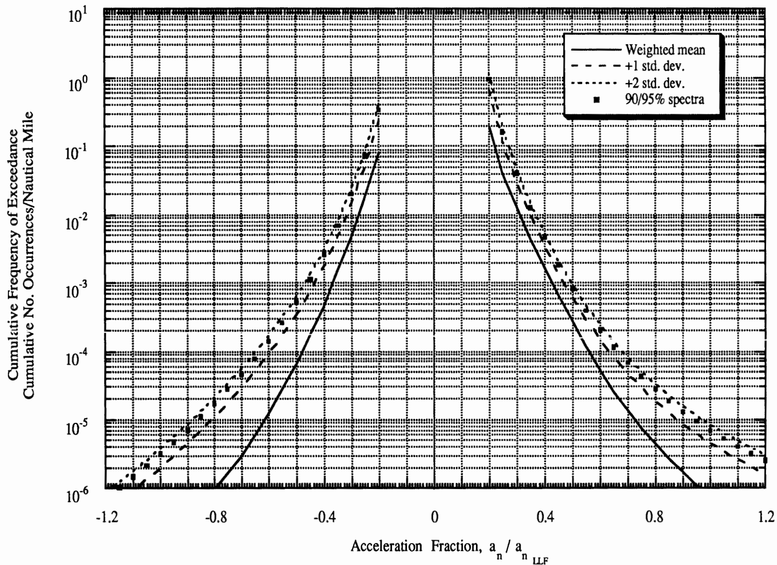
Figure 2-10 Gust Load Spectra: Single-Engine Aerial Application
