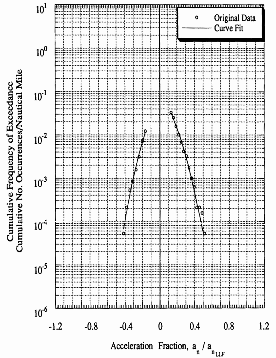
Figure C-16 Load Spectra for Airplane 7C 1 , Single-Engine, Business/Personal
