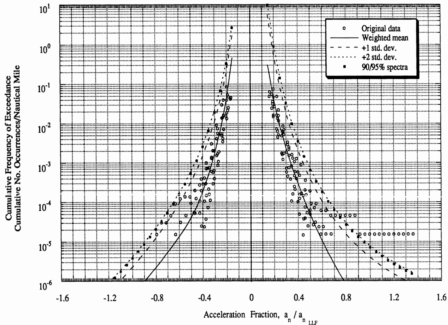
Figure D-1 Gust Load Spectra: Single-Engine General Usage, Basic Flight Instruction
