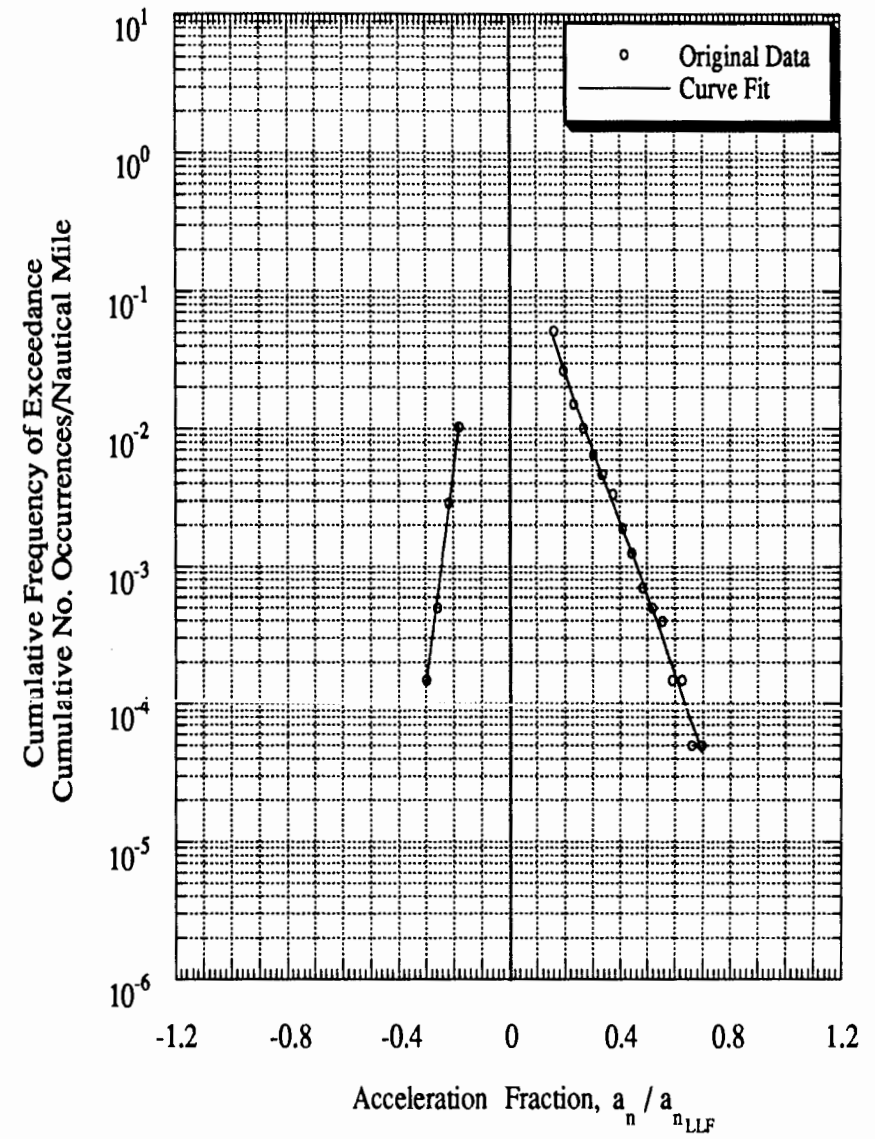
Figure C-73 Load Spectra for Airplane 4 1 , Twin-Engine, Special Usage
