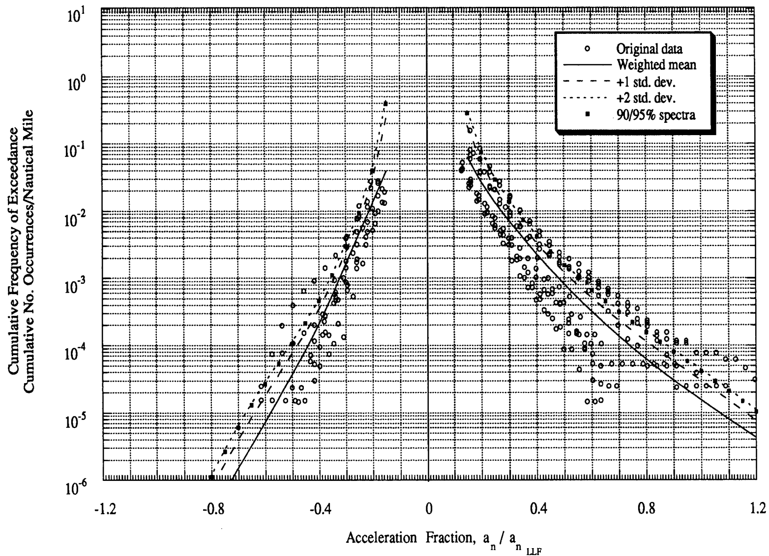
Figure D-2 Maneuver Load Spectra: Single-Engine General Usage, Basic Flight Instruction
