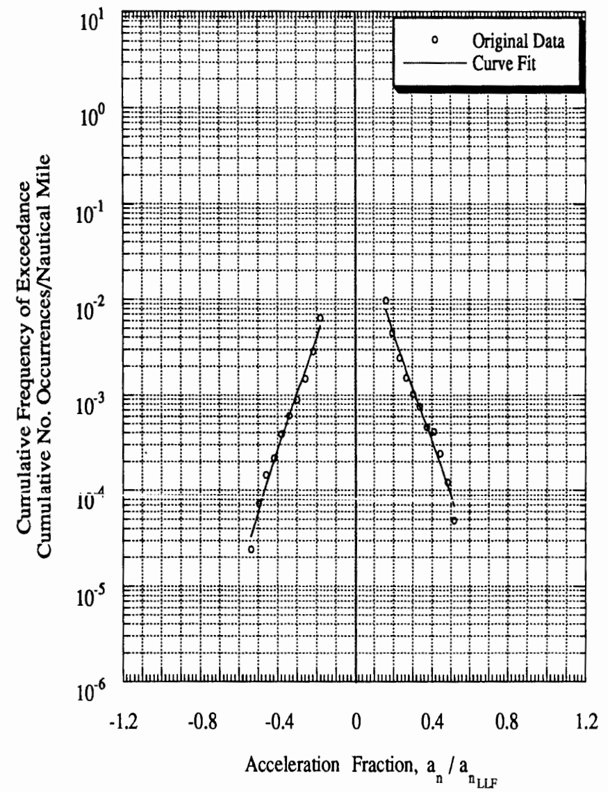
Figure C-67 Load Spectra for Airplane 5 1 , Twin-Engine, General Usage
