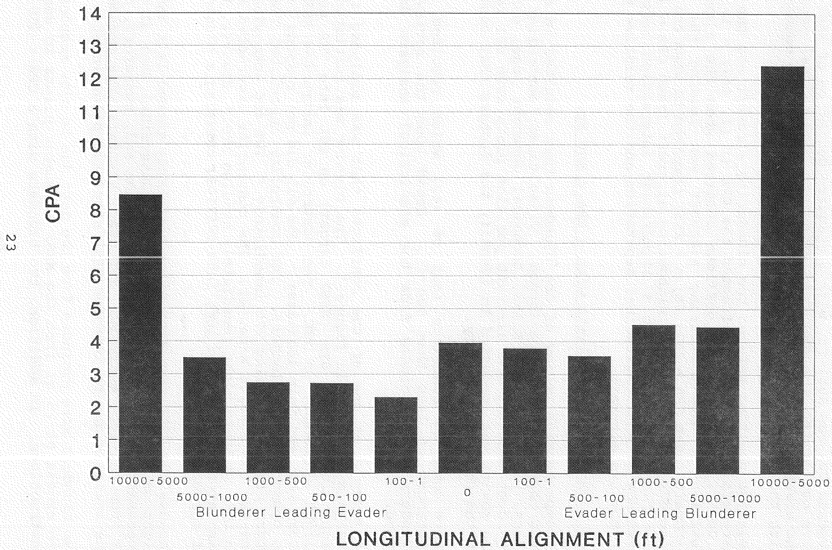
FIGURE 6. EFFECT OF LONGITUDINAL SEPARATION ON CPA
