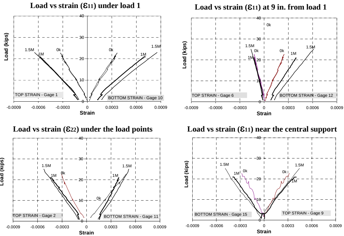
Figure 7-26 Load-strain curves at 1,500,000 cycles for span1
