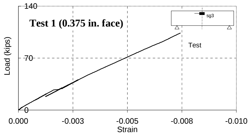
Figure 5-12 Load-strain curve for Test 1 (gage sg3)
