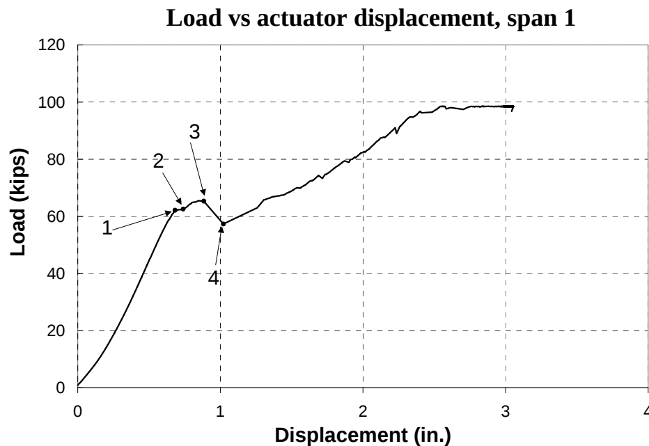
Figure 7-28 Load- actuator displacement curve for Span 1
