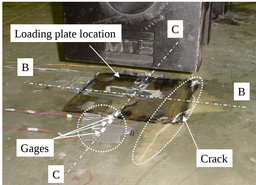
Figure 7-31 Crack located outside the loading plate in Span 1
