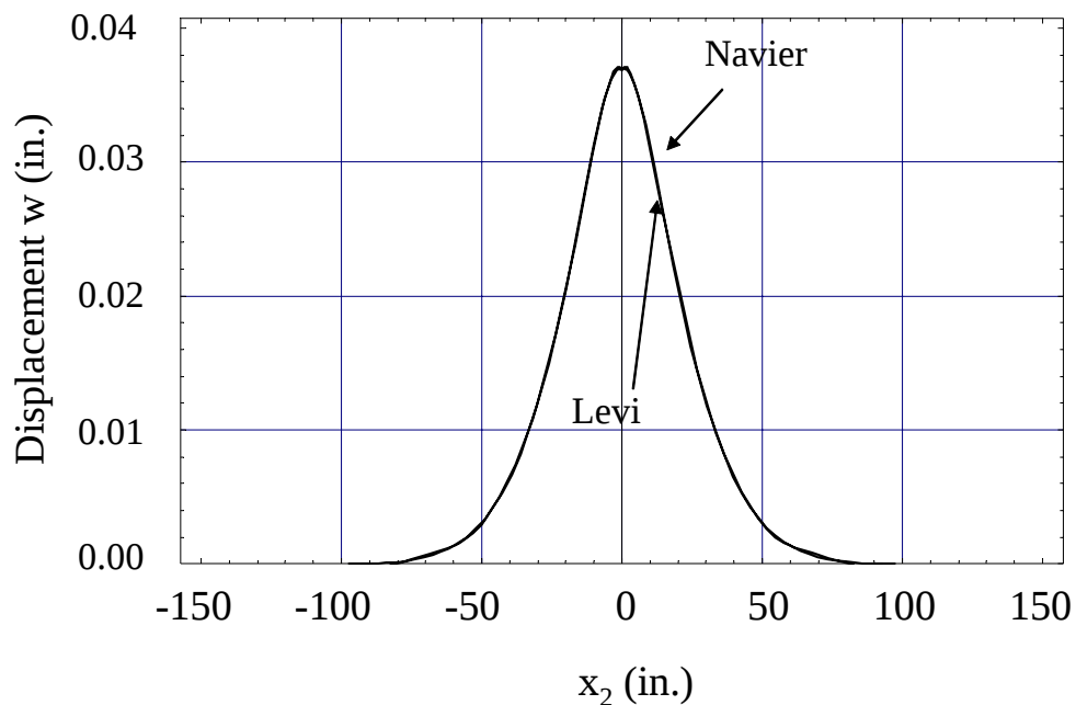
Figure 8-9 Displacement along section A-A at 26 kips
