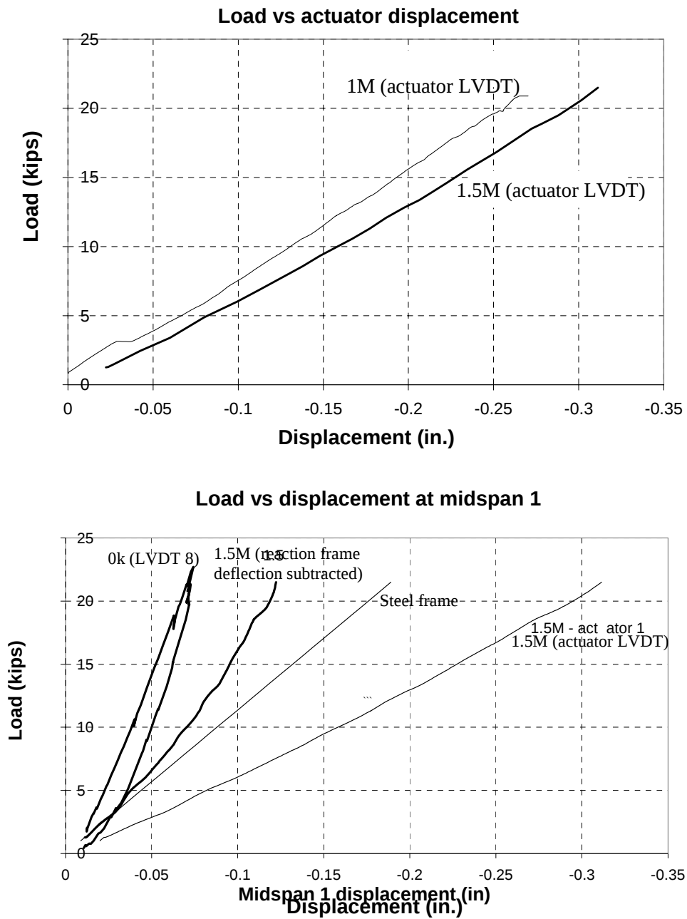
Figure 7-25 Load-displacement curves for Span 1
