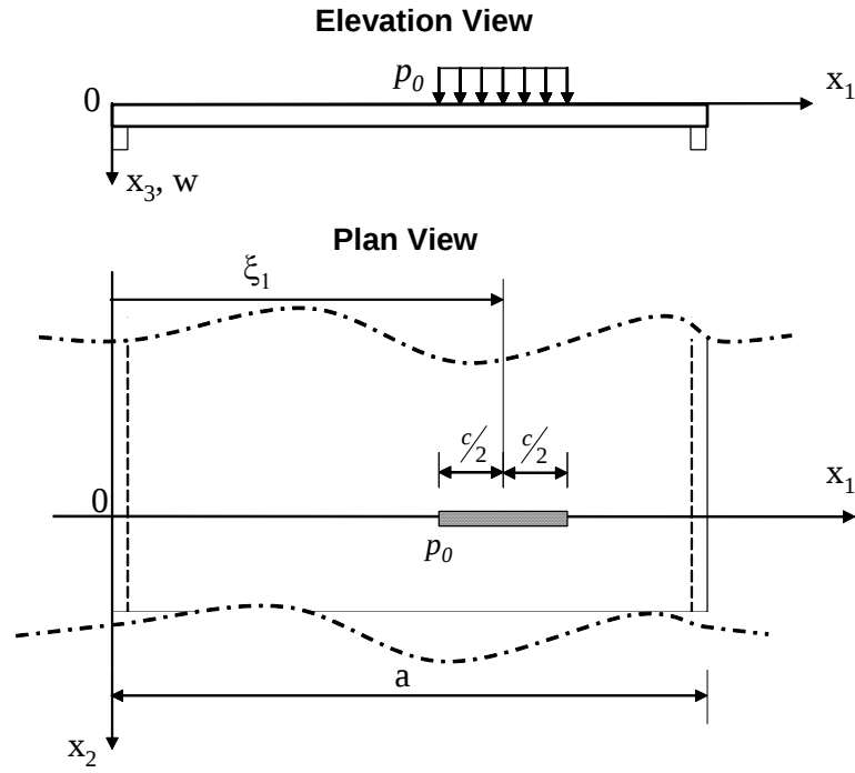
Figure 8-4 Uniform line load condition
