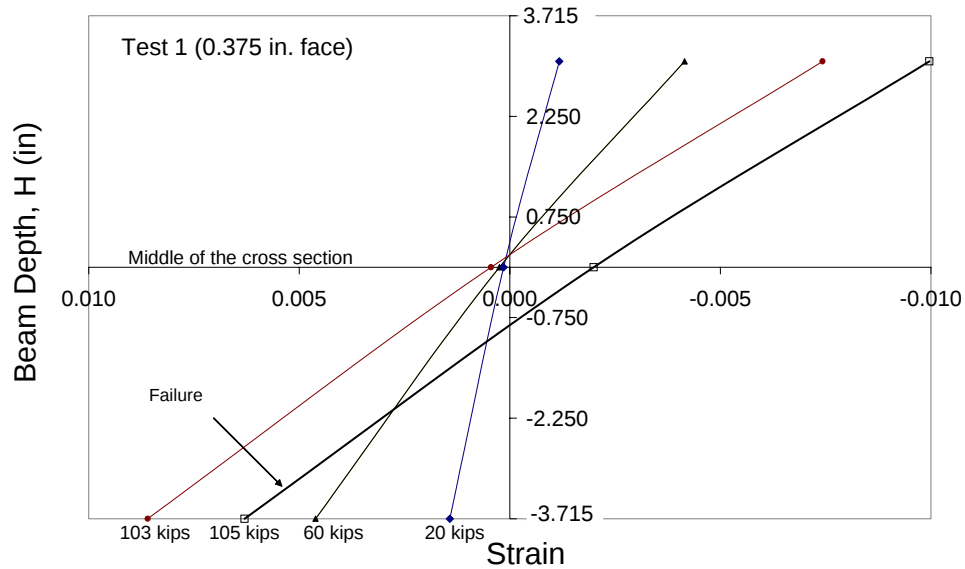
Figure 5-15 Strain profiles at different loading stages for Test 1 (midspan)
