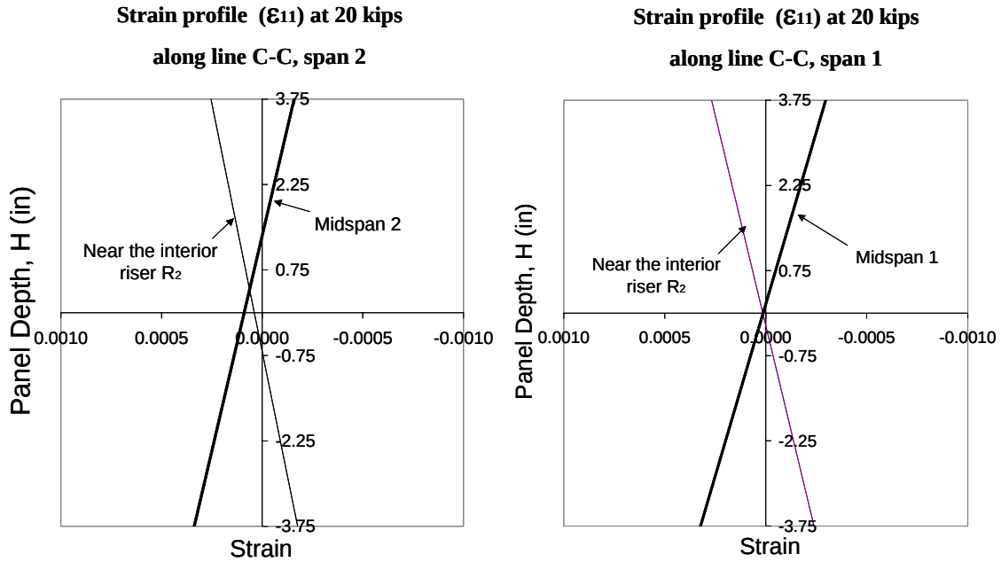
Figure 7-17 Panel strain profiles
