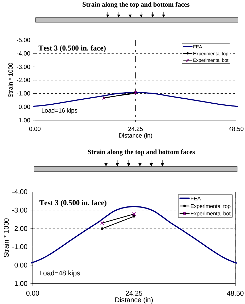
Figure 6-17 Strain distribution along the top and bottom faces of the beam in Test 3 at different loading stages (only the top stain is shown for the FEA)
