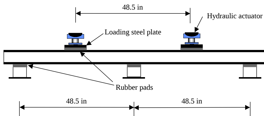
Figure 7-2 Test setup
