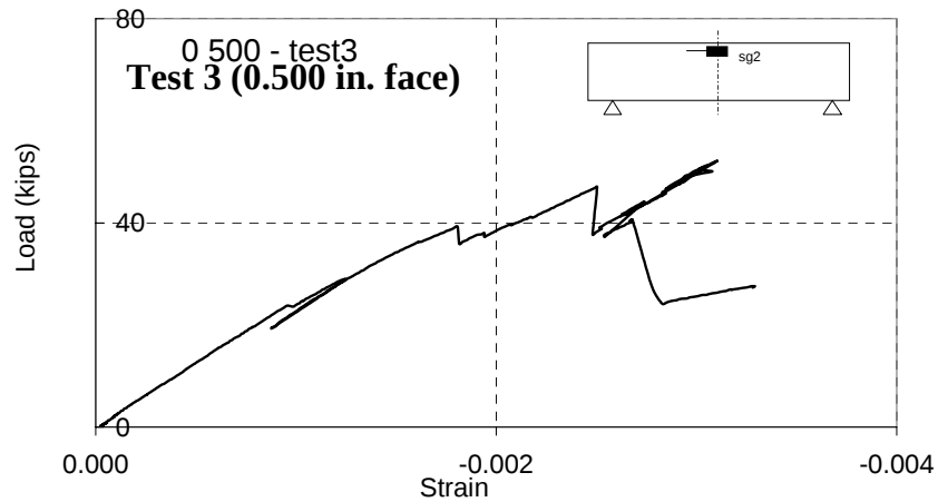
Figure 5-33 Load-strain curve for Test 3 (gage sg2)
