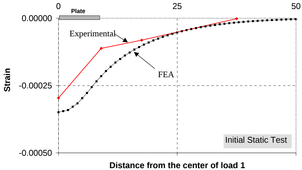
Figure 9-18 Strains \varepsilon_{11} on the top of the panel along section A-A of Span 1
