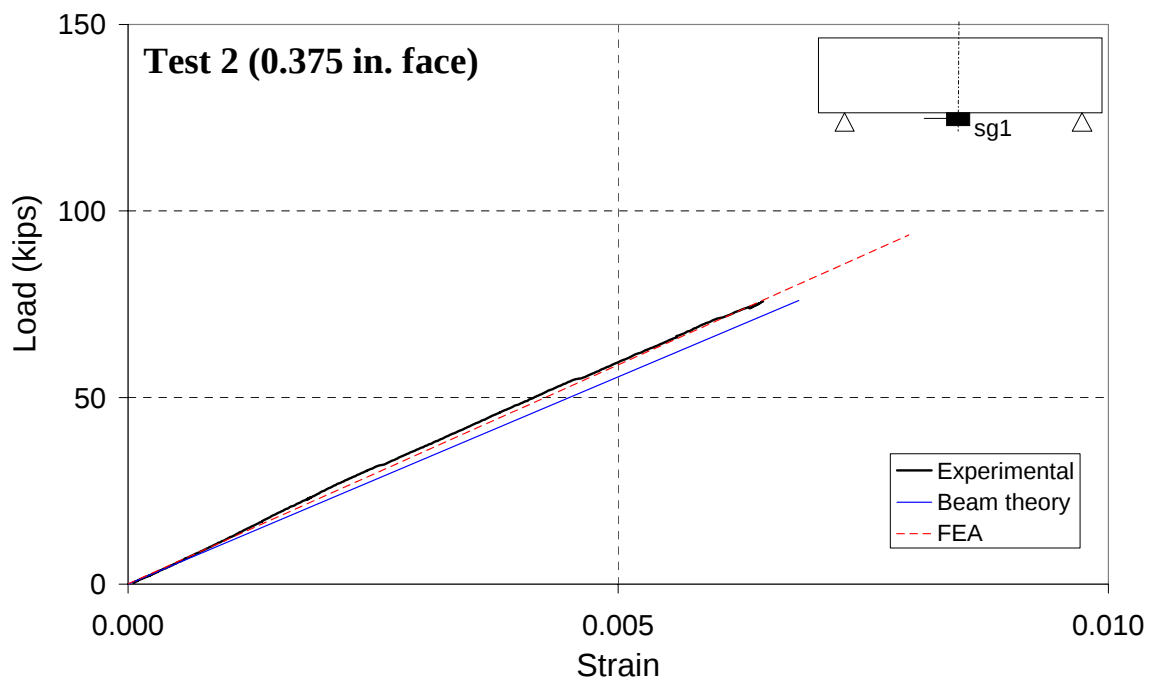
Figure 6-8 Analytical and numerical load-strain curves for bottom strain at midspan for Test 2
