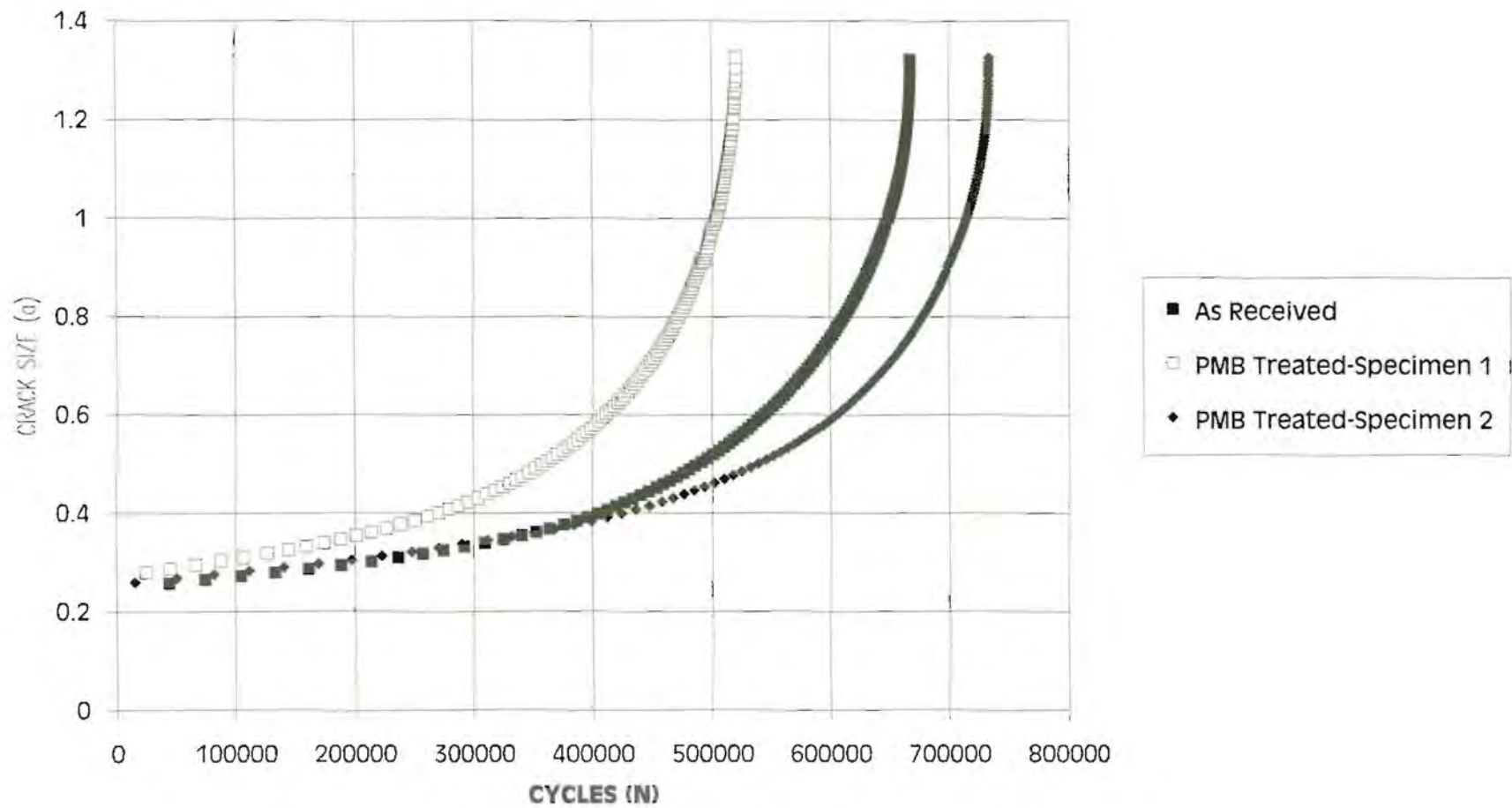
FIGURE 3.10 CRACK SIZE VS CYCLES - 0.05", 2024-T3, ANODIZED
