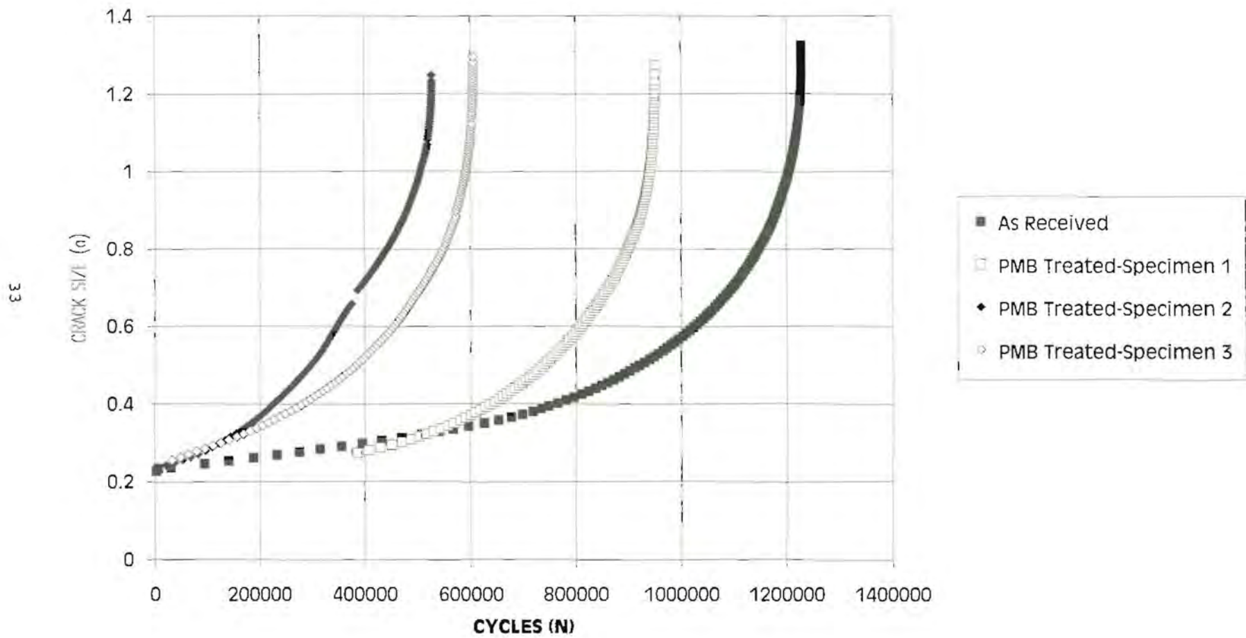
FIGURE 3.11 CRACK SIZE VS CYCLES - 0.032", 2024-T3, ALCLAD
