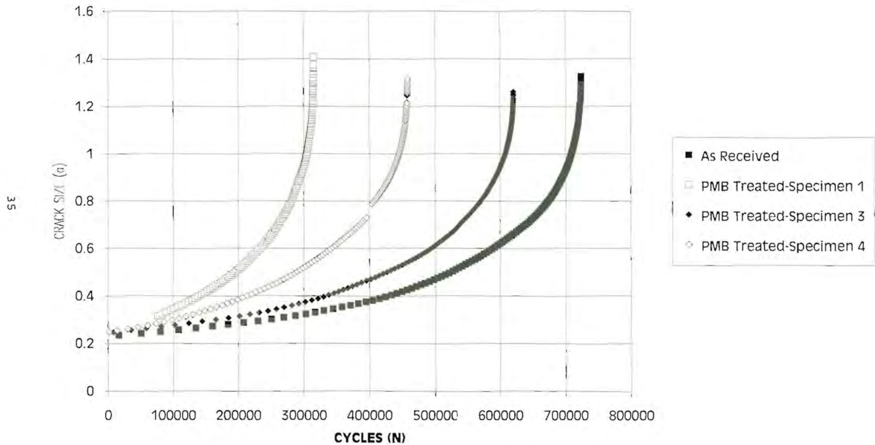
FIGURE 3.13 CRACK SIZE VS CYCLES - 0.050" , 2024-T3, ALCLAD
