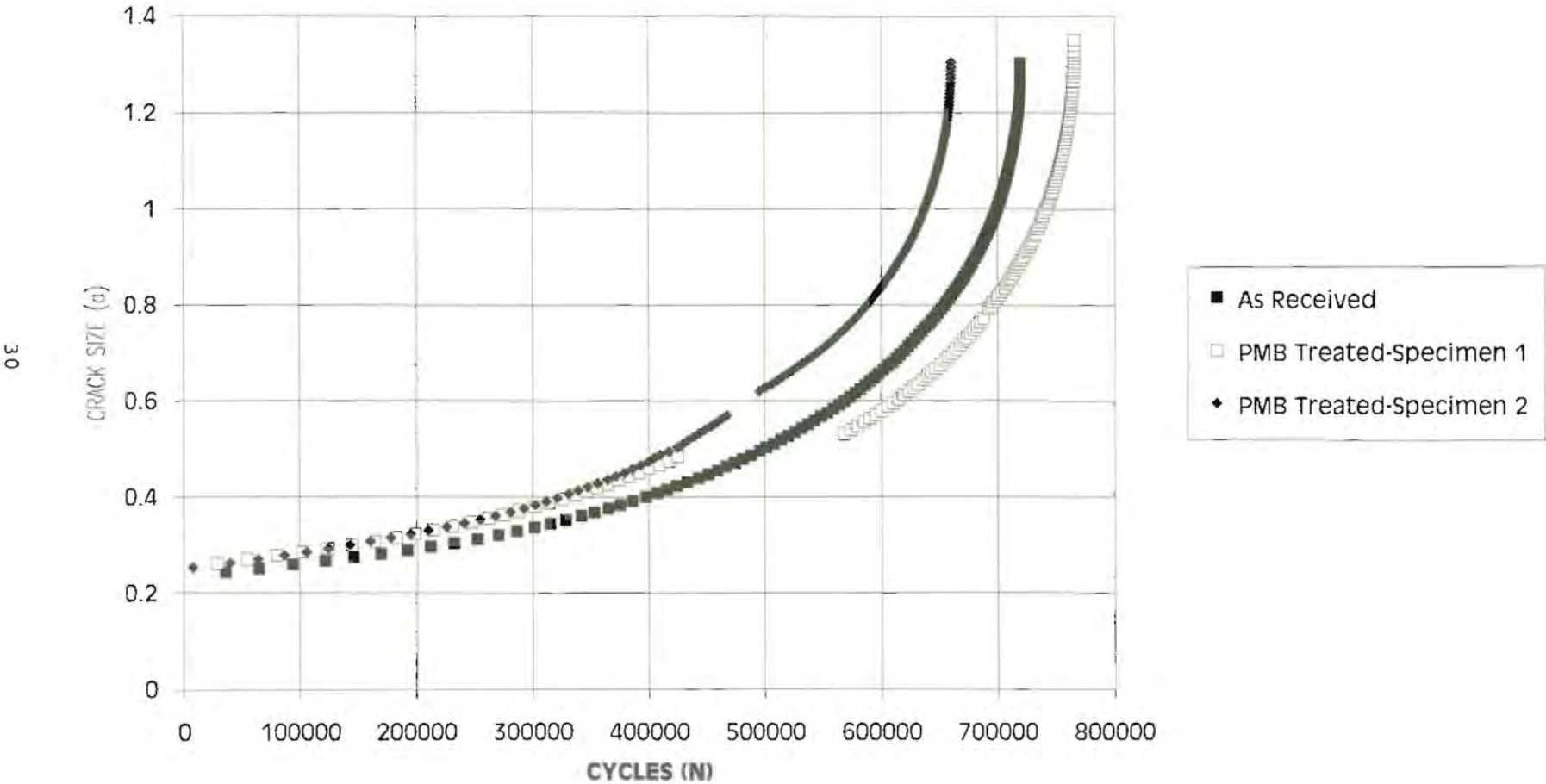
FIGURE 3.8 CRACK SIZE VS CYCLES - 0.032", 2024-T3, ANODIZED
