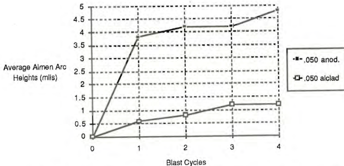
Figure 3.7 Comparative Average Arc Heights - 2024-T3 0.050 inch Anodized and 2024-T3 0.050 inch Alclad Aluminum
