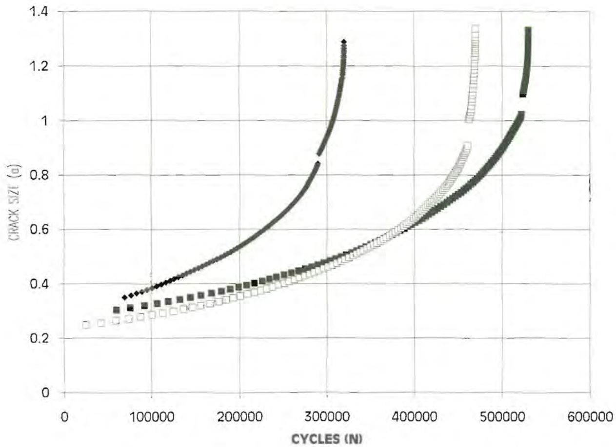
FIGURE 3.12 CRACK SIZE VS CYCLES - 0.040", 2024-T3, ALCLAD
