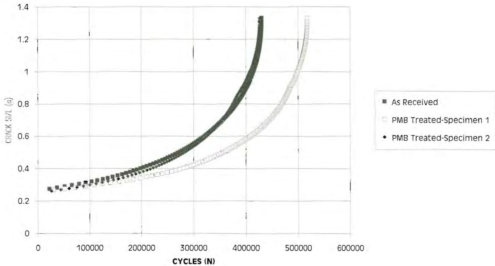
FIGURE 3.9 CRACK SIZE VS CYCLES - 0.040", 2024-T3, ANODIZED
