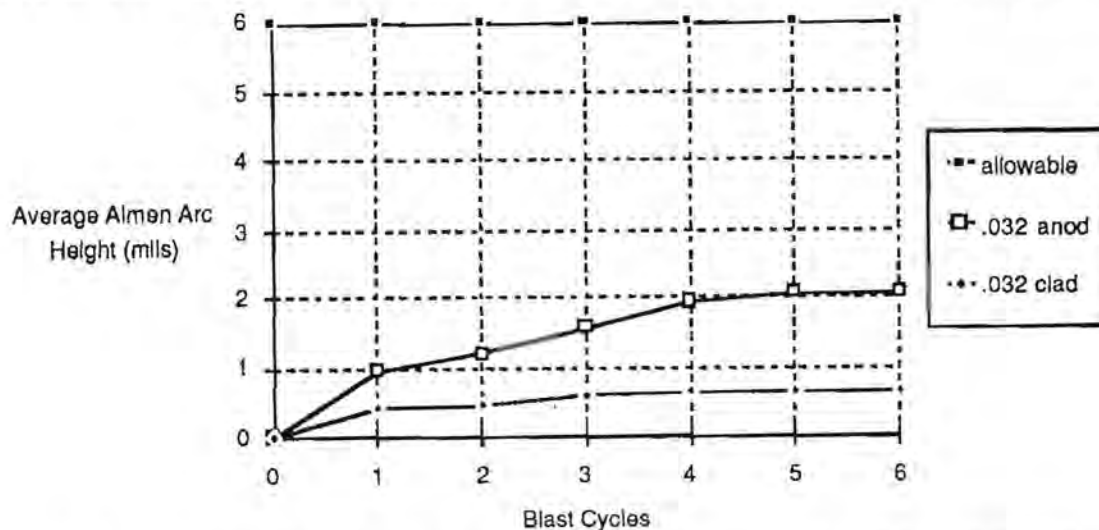
Figure 3.37 MBB Average Almen Strip Arc Heights, 26 psi on 2024-T3 0.032 Anodized and 0.032 Alclad Aluminum
