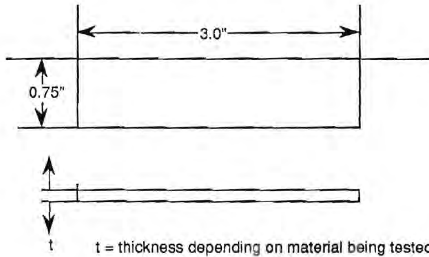
Figure C.1 Almen Strip Specified Dimensions
