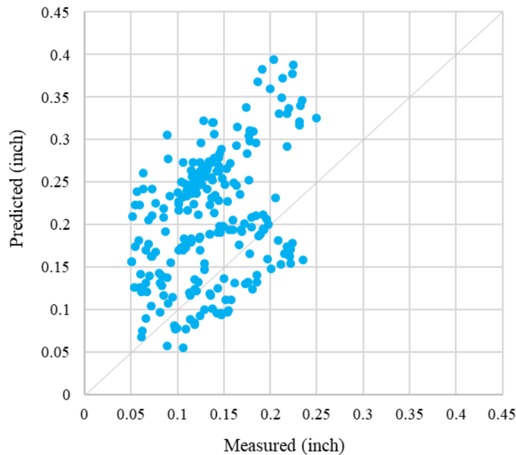
Figure 25. Measured Versus Predicted Total Rutting for Flexible Pavements from Refinement
