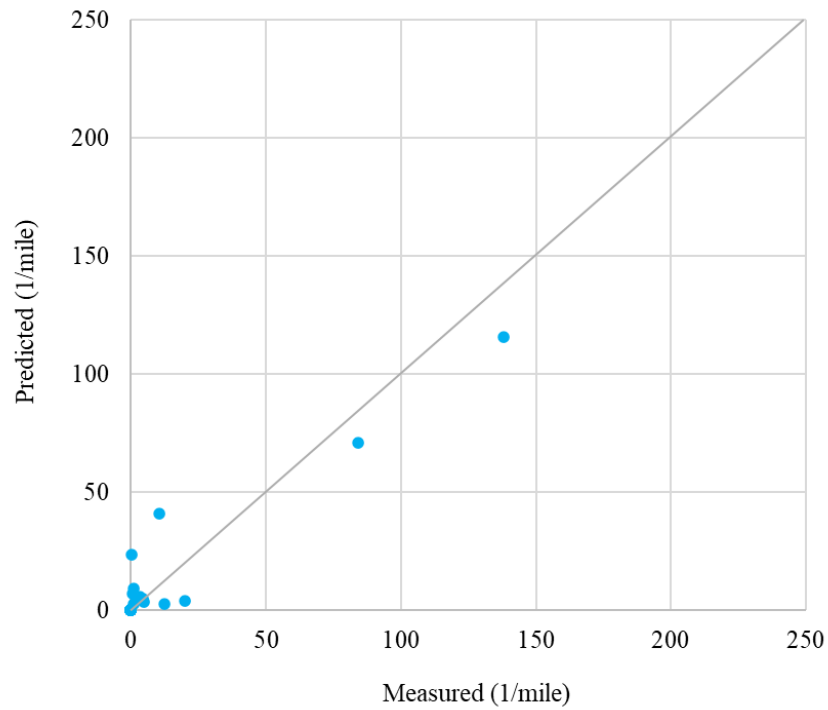
Figure 22. Measured Versus Predicted Punchouts for Continuously Reinforced Concrete Pavements from the Preliminary Validation Process
