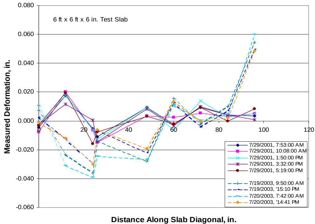
Figure 5.11. Diagonal Profile Measurements for S.H. 121 Test Section 4
