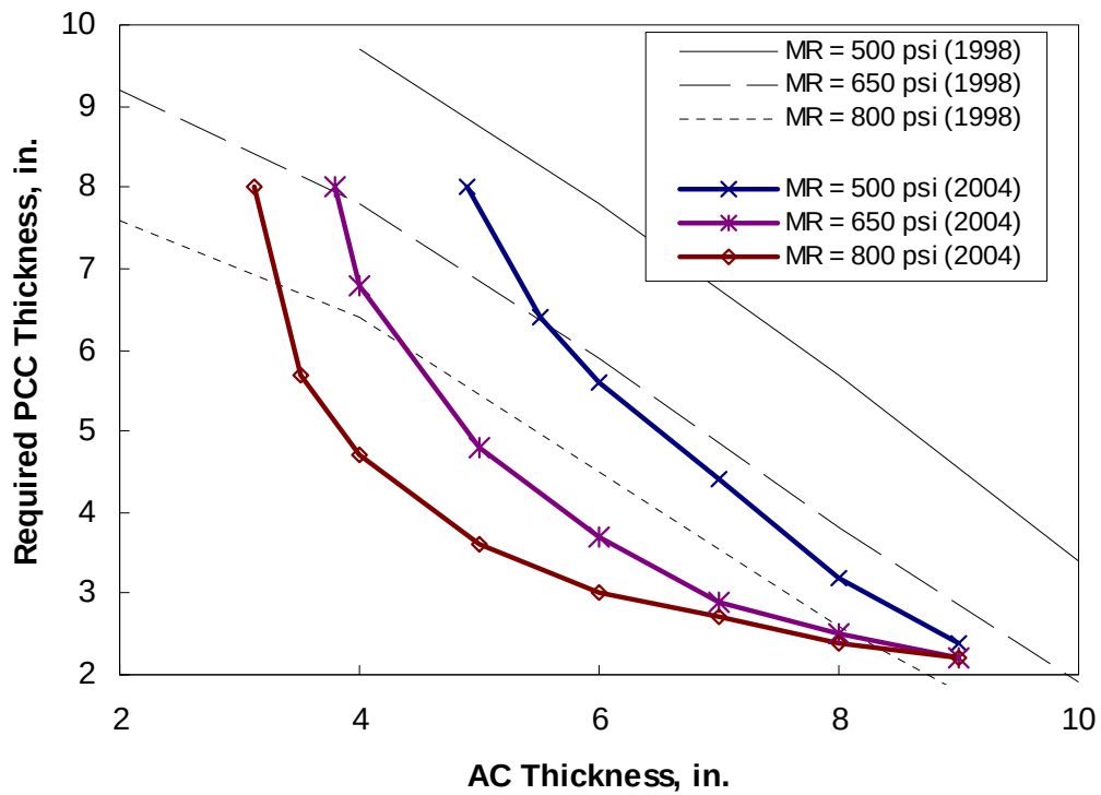
Figure 7.3. PCC Thickness Sensitivity to Concrete Modulus of Rupture
