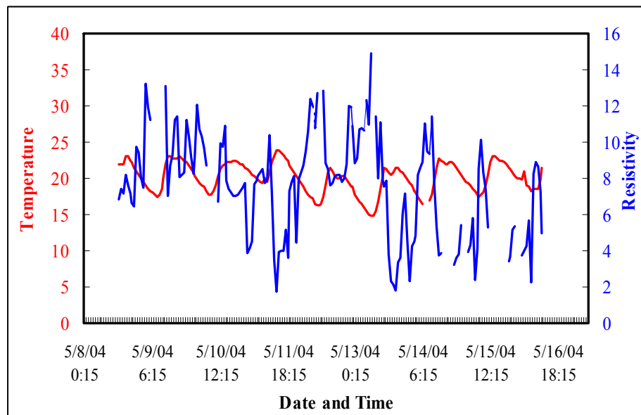
Figure 3-21 Comparison of both resistivity ( \Omega\cdot\text{cm} ) and temperature ( ^{\circ}\text{C} ) profile Chloride Level (volts)
