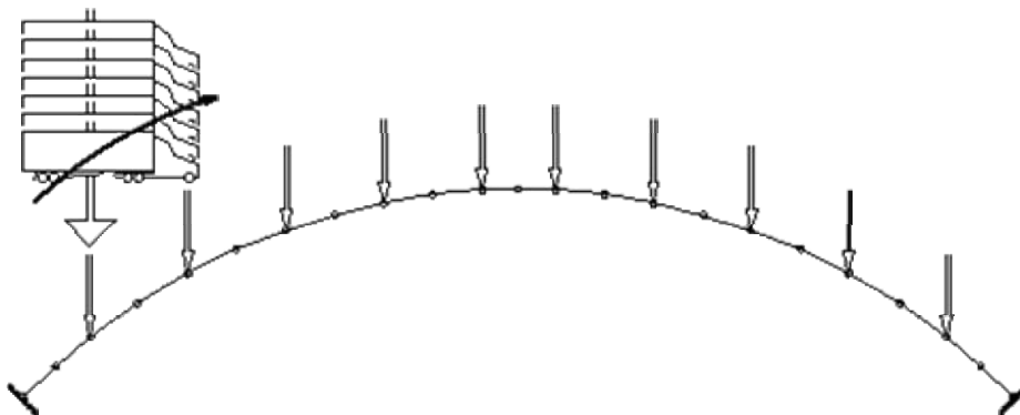
Figure 1-26 SAP2000 arch model with moveable truck load
