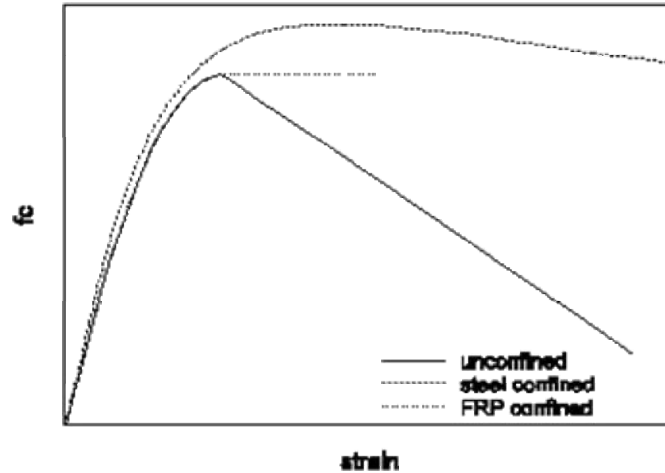
Figure 1-17 Three constitutive models for concrete
