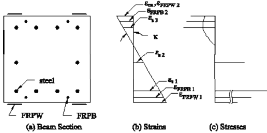
Figure 1-20 Strains and stresses in the section
