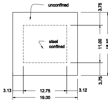
Figure B. 2 FC section dimensions and concrete regions
