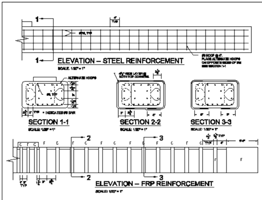
Figure 1-33 Reinforcing details for one side of AR specimen (Other side similar)
