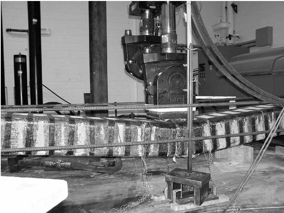
Figure 1-44 A single piston was used to apply the center load to the AR specimen. This picture was taken near the end of the test.
