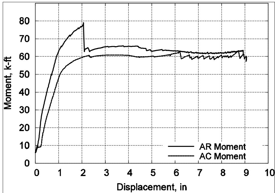
Figure 1-76 M vs. mid-span deflection for arch specimens
