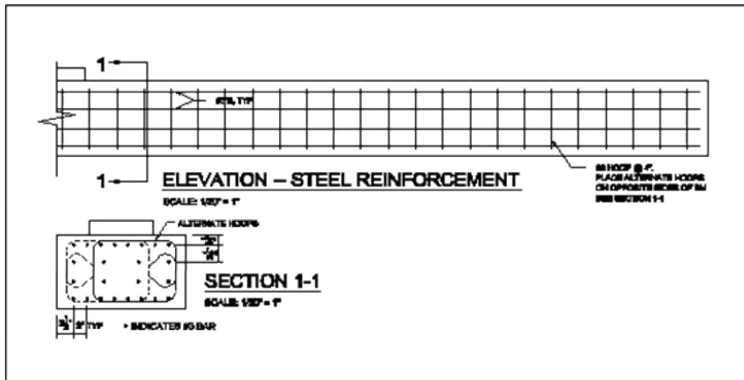
Figure 1-34 Reinforcing details for one side of AC specimen (Other side similar)
