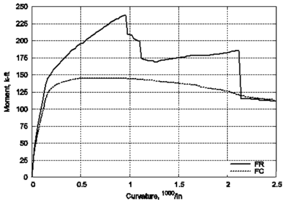
Figure 1-35 Nominal moment-curvature plots for foundation specimens
