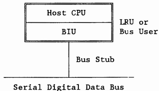
FIGURE 2.1-1. DATA BUS COMPONENTS
