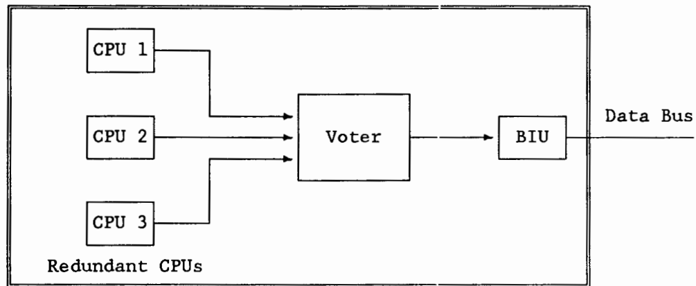
FIGURE 5.2-5. OUTPUT VOTING
