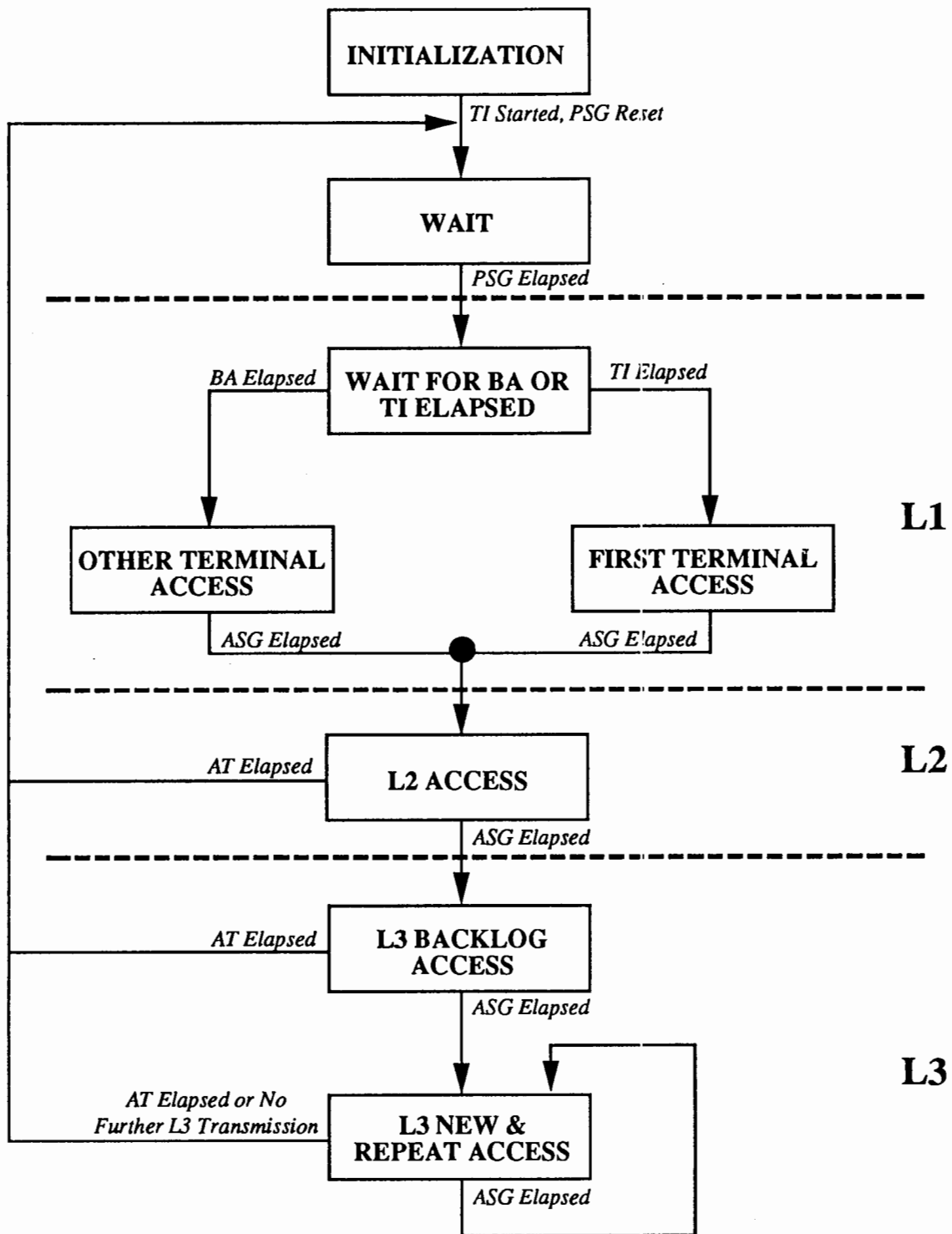
FIGURE 5.3-12. ACCESS PROTOCOL OVERVIEW FOR ARINC 629 BUS (ARINC Specification 629, Part 1, Attachment 7b, 1990)
