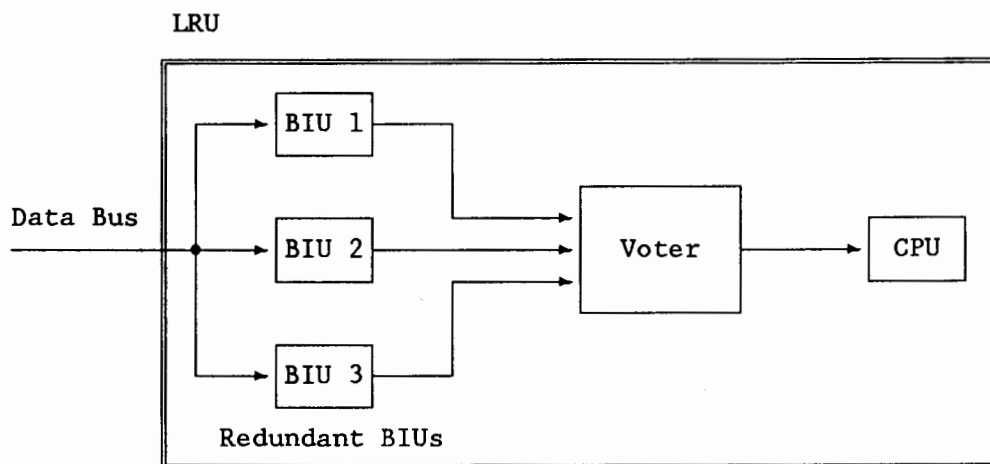
FIGURE 5.2-4. INPUT VOTING
