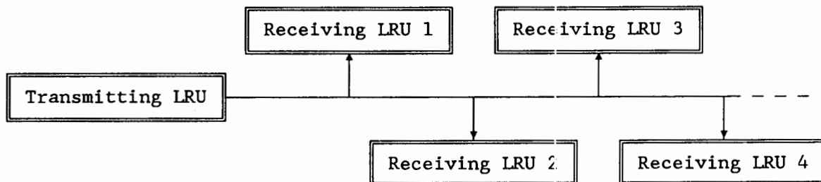
FIGURE 2.1-2. UNIDIRECTIONAL BUS ARCHITECTURE
