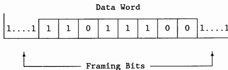
FIGURE 5.2-3. DATA FRAMING
