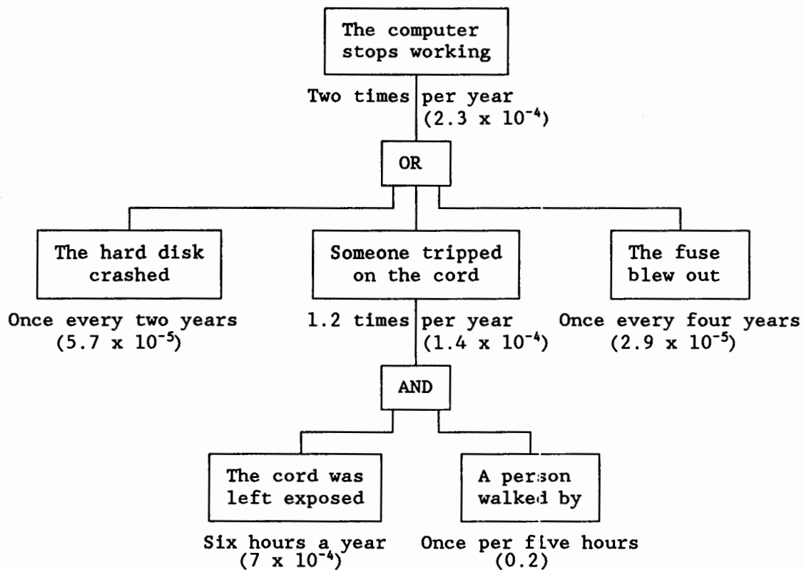
FIGURE 5.4-2. QUANTITATIVE FAULT TREE ANALYSIS
