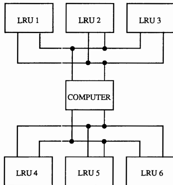
MULTIPLE BUS TOPOLOGY WITH REDUNDANCY
