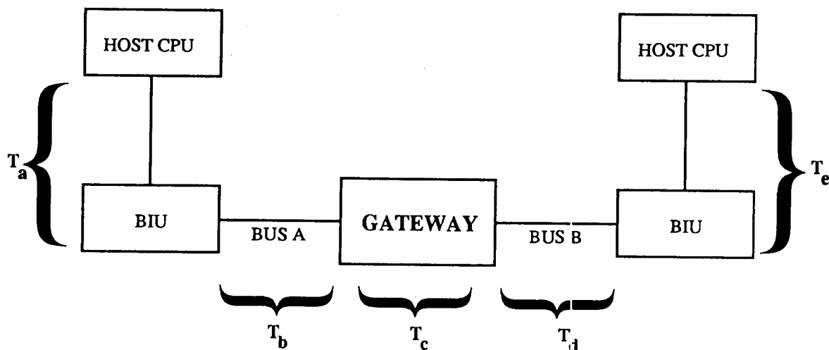
FIGURE 5.1-4. DATA BUS DELAY WITH A GATEWAY
