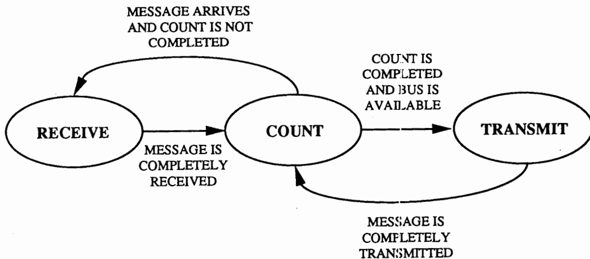
FIGURE B-1. DTSA ACCESS PROTOCOL STATE DIAGRAM
