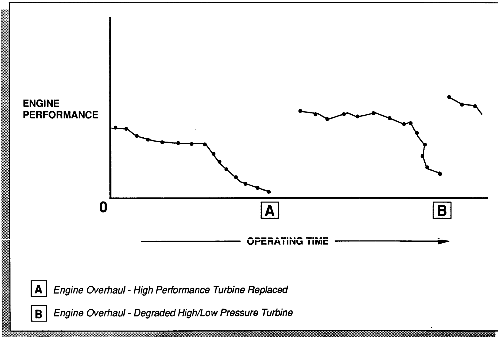
FIGURE 5-8 Maintenance Correlation
