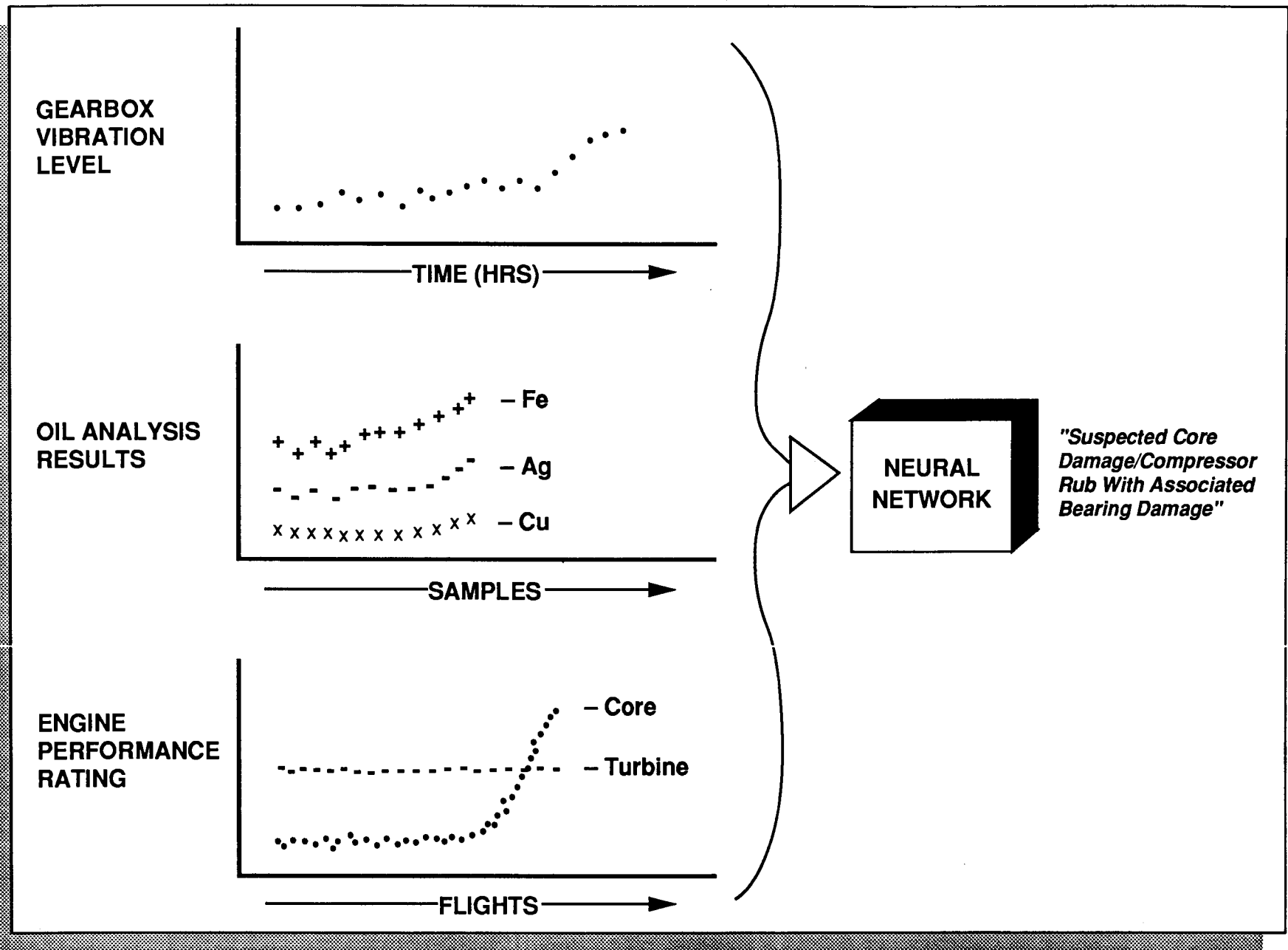
FIGURE 5-9 Pattern Recognition With Neural Networks
