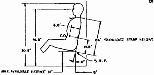
50 TH PERCENTILE SEATING CONFIGURATION FOR BULKHEAD OR FLOOR-MOUNTED SEATS (NOT APPLICABLE FOR SEATS OVER FUELTANKS)
