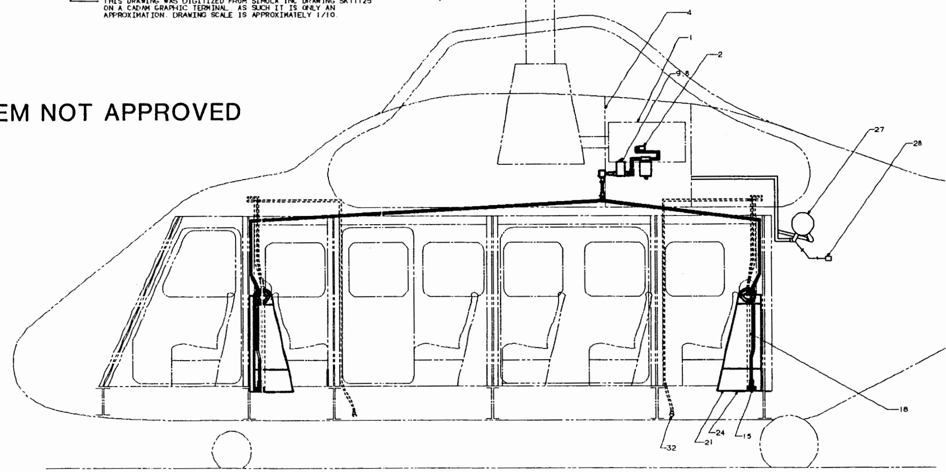
Figure 24. Fuel system configuration for the generic heavy rotorcraft.
