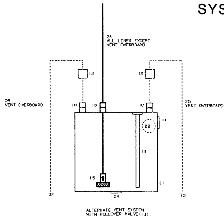
Figure 15. Schematic diagram of the selected fuel system (No. 3) for the generic light rotorcraft.
