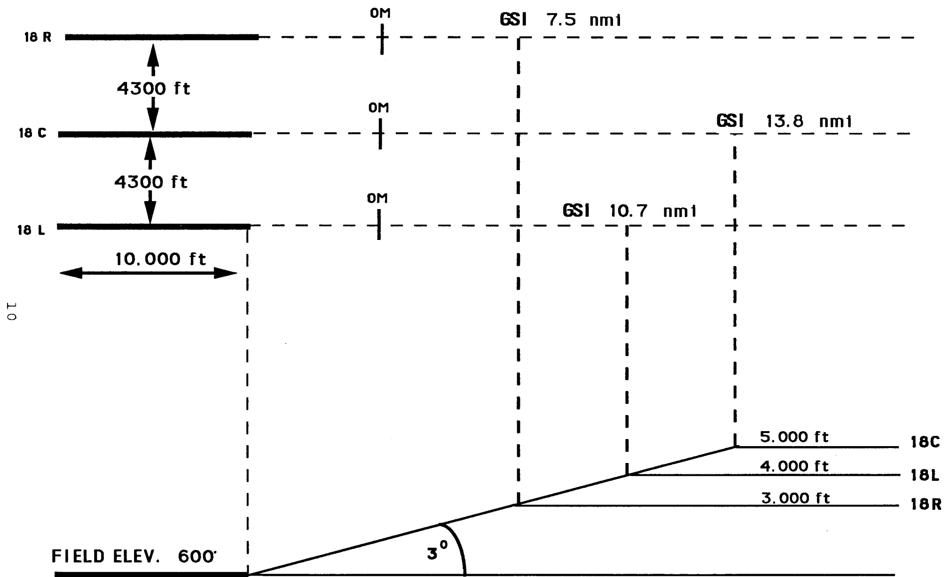
FIGURE 2. AIRPORT CONFIGURATION
