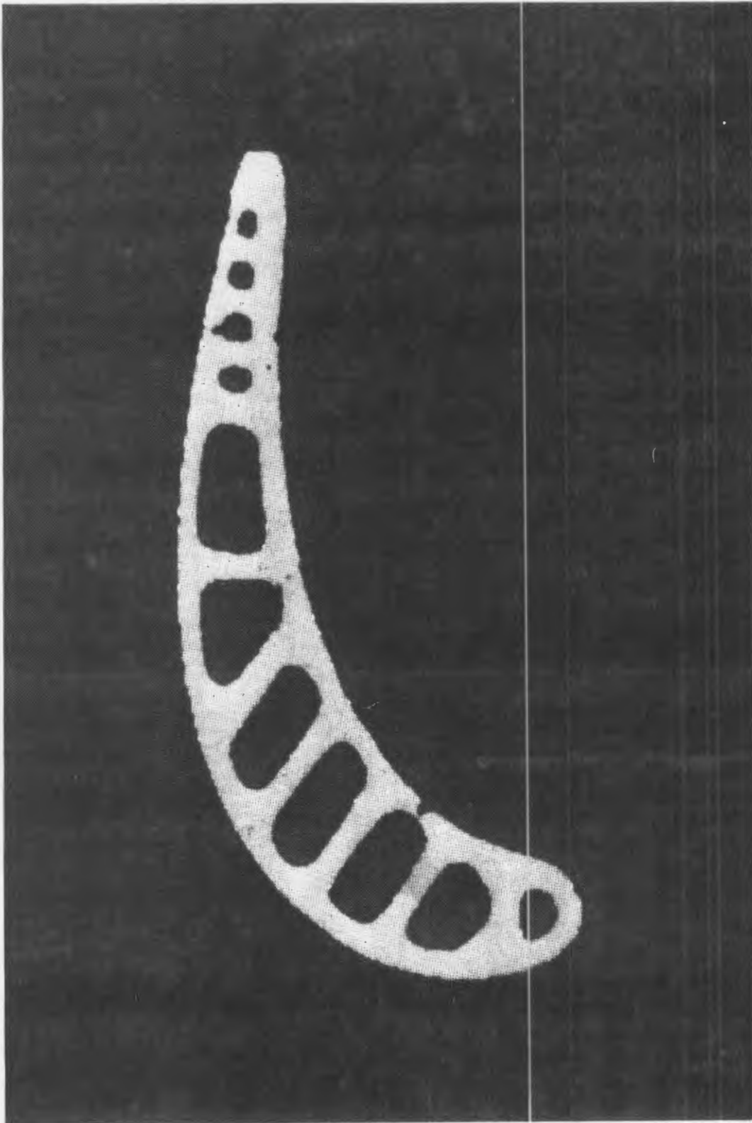
FIGURE 14. CROSS-SECTIONAL VIEW OF A JET ENGINE TURBINE BLADE MADE BY COMPUTED TOMOGRAPHY Courtesy of General Electric Co.
