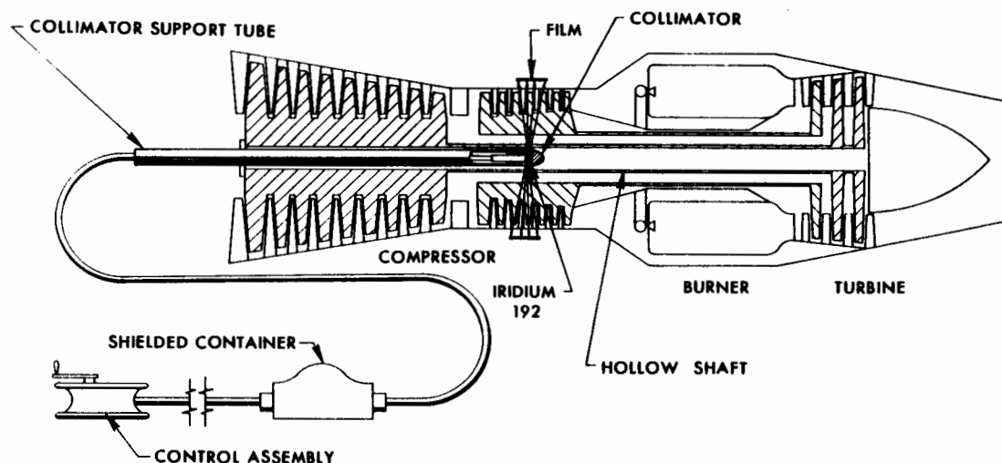
FIGURE 55. ISOTOPE RADIOGRAPHIC INSPECTION OF ENGINE
