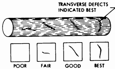
FIGURE 46. LONGITUDINAL MAGNETIZATION DEFECT INDICATIONS
