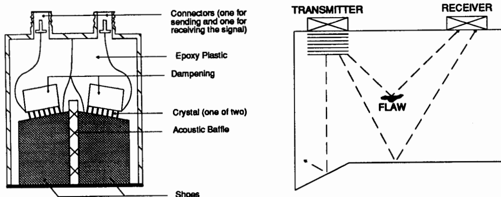
FIGURE 30. ILLUSTRATIONS USING SEPARATE TRANSDUCERS FOR SENDING AND RECEIVING, OR "PITCH-CATCH"
