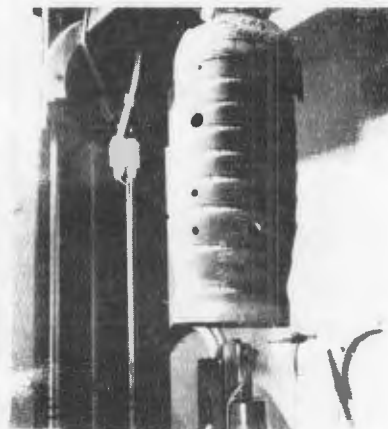
FIGURE 13. A MICROFOCUS X-RAY SYSTEM USED TO INSPECT A JT8D ENGINE BURNER CAN
