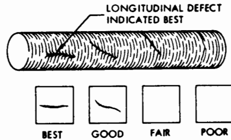
FIGURE 47. CIRCULAR MAGNETIZATION DEFECT INDICATIONS
