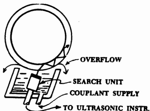
FIGURE 32. BUBBLER ANGLE-BEAM TESTING FOR PIPE INSPECTION
