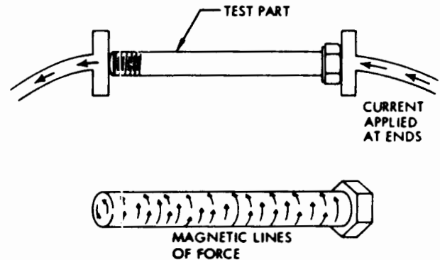
FIGURE 41. ILLUSTRATION OF CIRCULAR MAGNETISM
