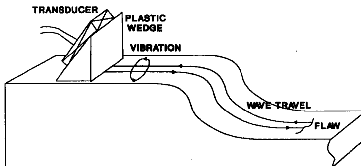
FIGURE 25. SURFACE WAVE PARTICLE MOTION IS ORBITAL, CONSISTING OF BOTH PARALLEL AND PERPENDICULAR COMPONENTS
