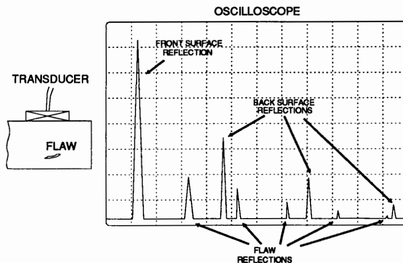
FIGURE 34. ILLUSTRATION OF A TYPICAL A-SCAN DISPLAY
