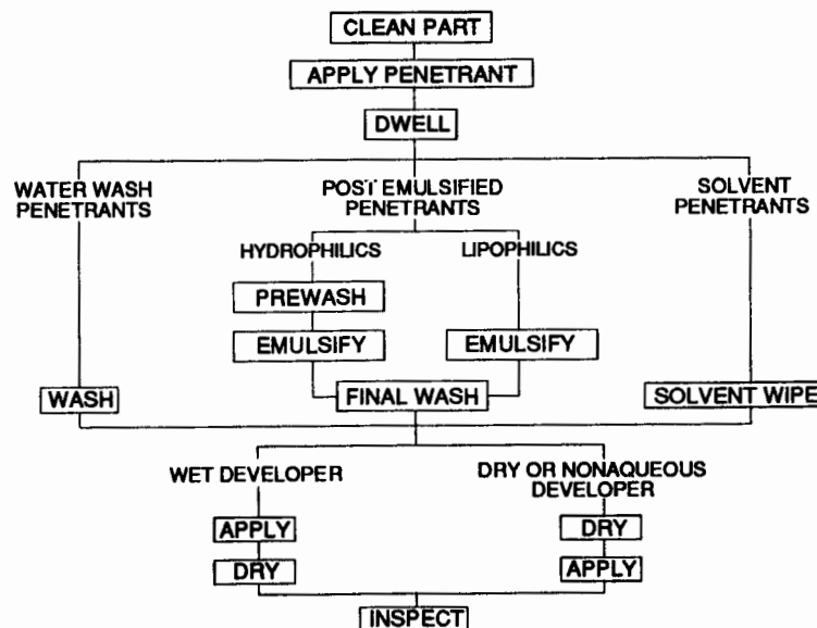
FIGURE 38. BLOCK DIAGRAM OF THE PENETRANT PROCESS
