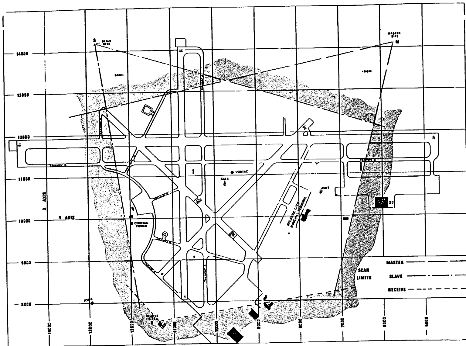
FIGURE A-6. BRASSBOARD DAS SITING AND COVERAGE AT NAFEC
