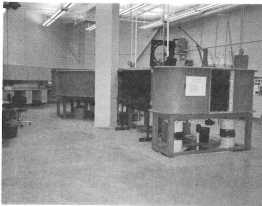
FIGURE 12. FLOW VISUALIZATION LABORATORY
