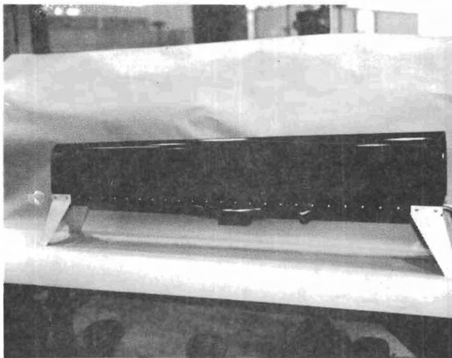
FIGURE 8. COMPOSITE LEADING EDGE MODEL (NON-PROTECTED)
