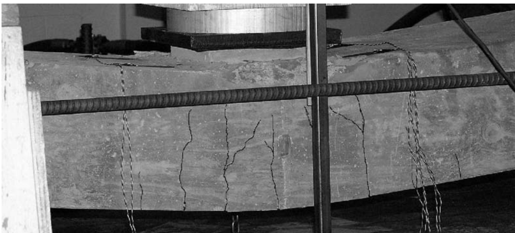
Figure 1-48 Crack pattern at end of test (AC specimen)
