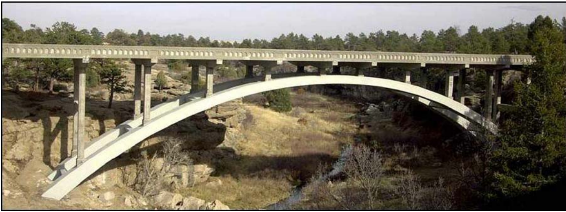
Figure 2-5 Repaired Castlewood Canyon Bridge, Franktown, Colorado
