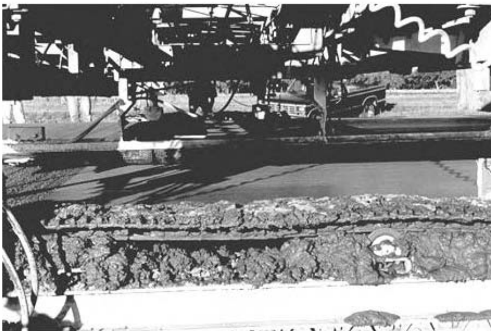
Photo 8: Installation of transverse astro-turf texture
