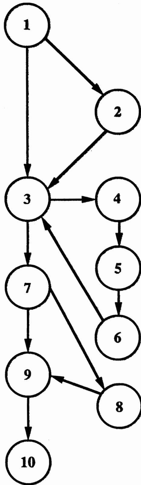
FIGURE 3.3-3. A PROGRAM CONTROL GRAPH OF FORTRAN CODE
