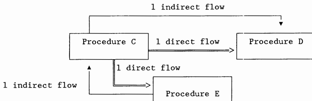
FIGURE 3.7-2. EXAMPLE OF INDIRECT LOCAL INFORMATION FLOW
