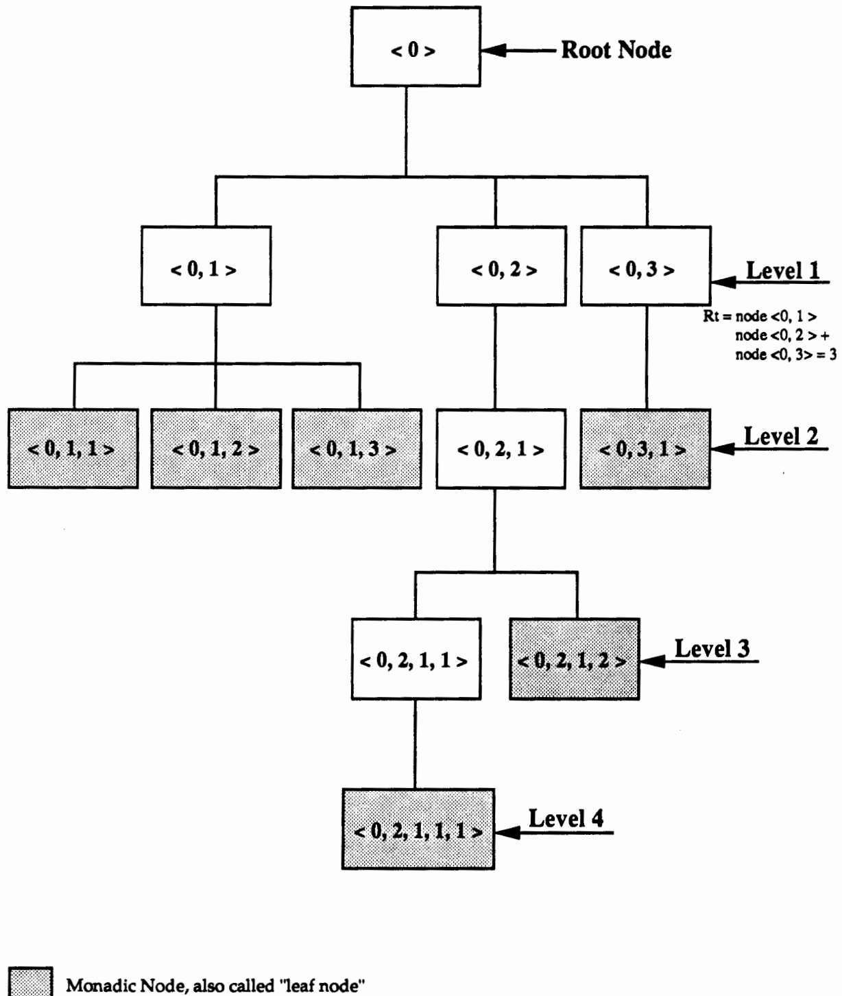
FIGURE 3.6-4. TREE STRUCTURE OF A PROGRAM
