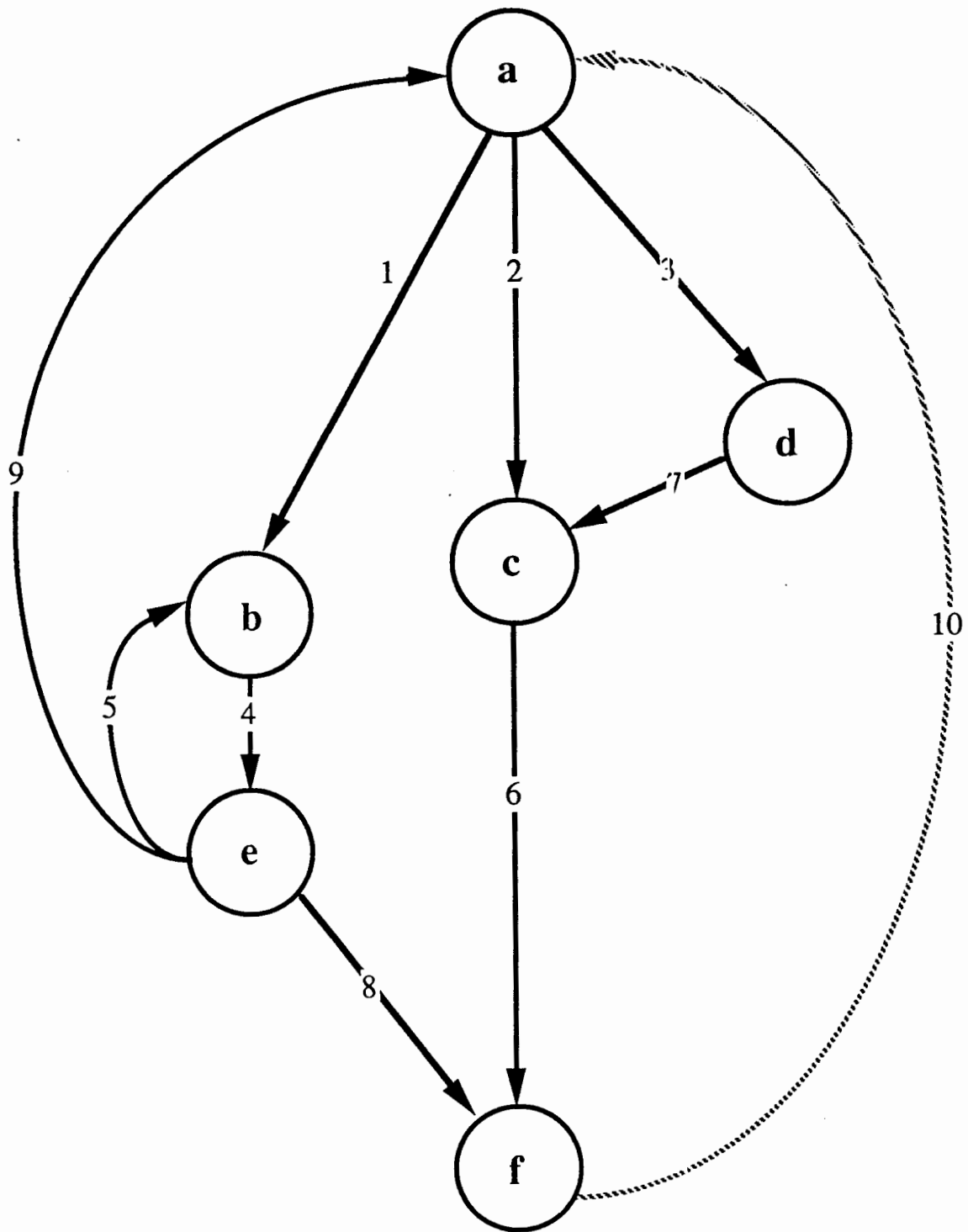
FIGURE 3.3-8. GRAPH WITH EDGE BACK
