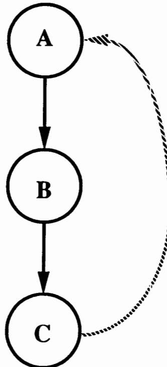
FIGURE 3.3-4. A STRONGLY-CONNECTED GRAPH
