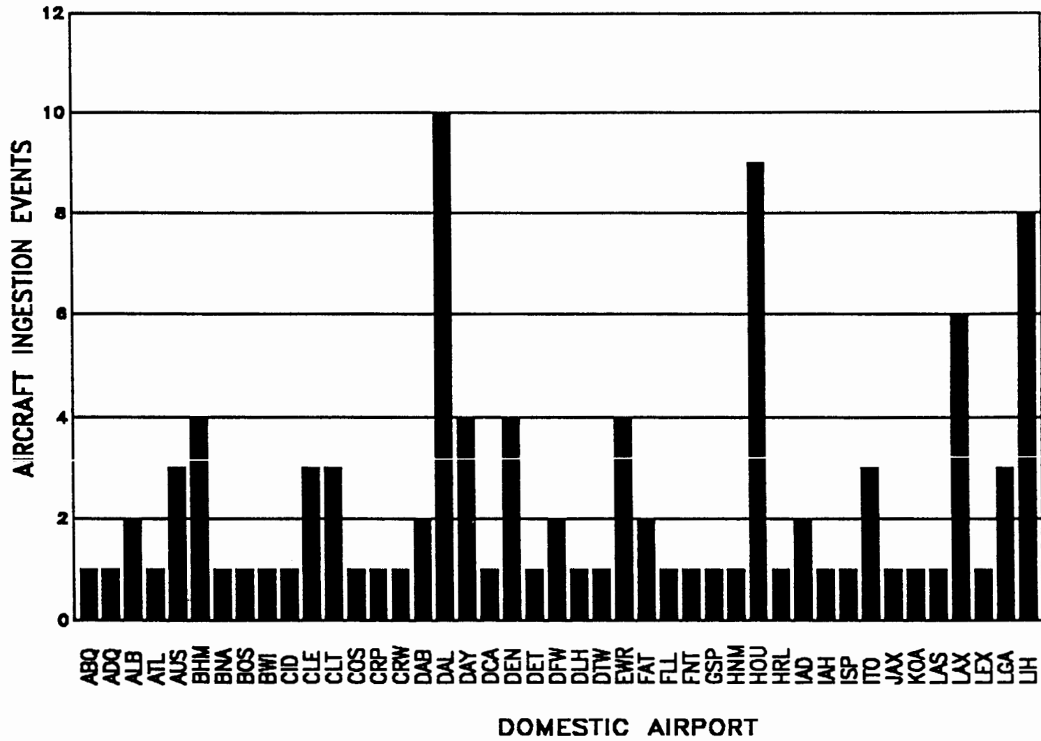
Figure 5.1 Histogram of Aircraft Ingestion Events at Domestic Airports.
