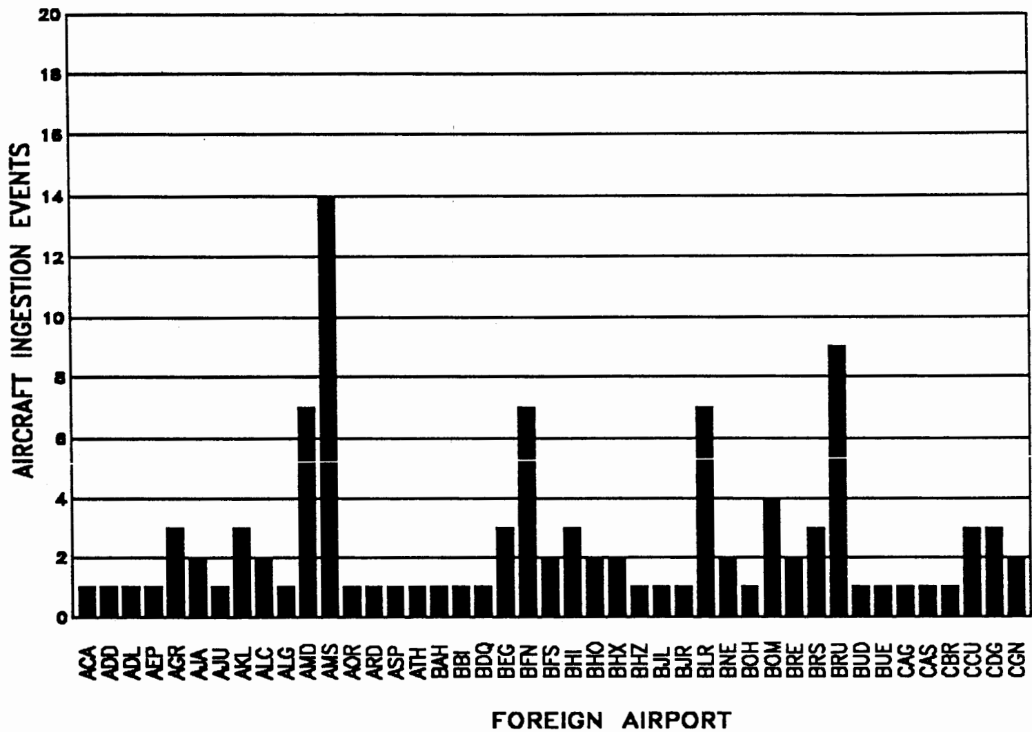
Figure 5.2 Histogram of Aircraft Ingestion Events at Foreign Airports.
