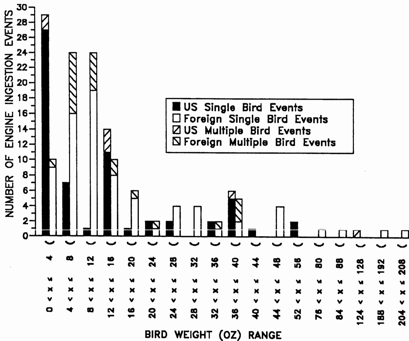
Figure 3.3. Histogram of Number of Birds Ingested by Weight Class.
