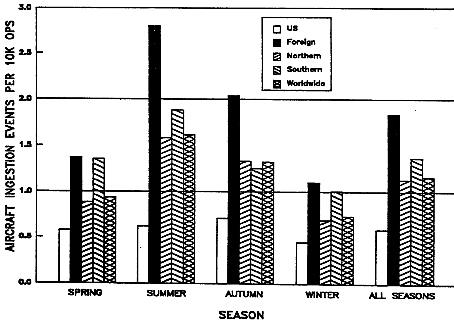
Figure 3.5 Seasonal Aircraft Ingestion Rates.
