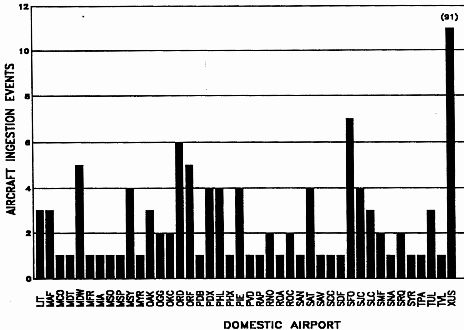
Figure 5.1 Histogram of Aircraft Ingestion Events at Domestic Airports. (Concluded)
