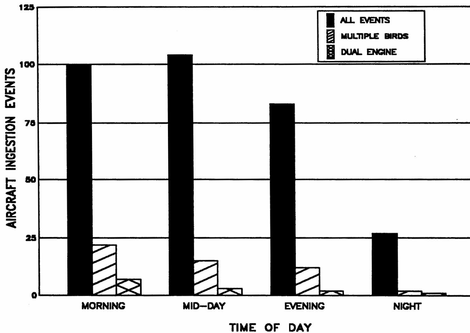
Figure 3.6 Histogram of Aircraft Ingestion Events by Time of Day.
