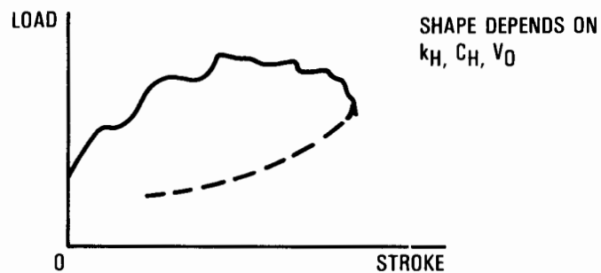
Figure 3-3. Impact Surface Structural Models
