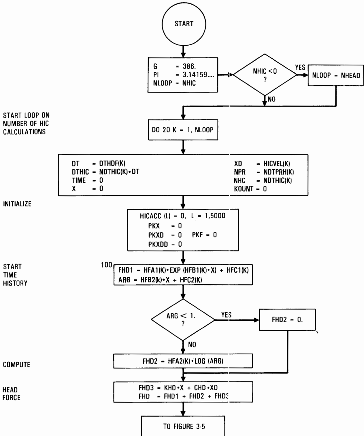
Figure 3-4. Flow Diagram for Head Impact Load Calculation
