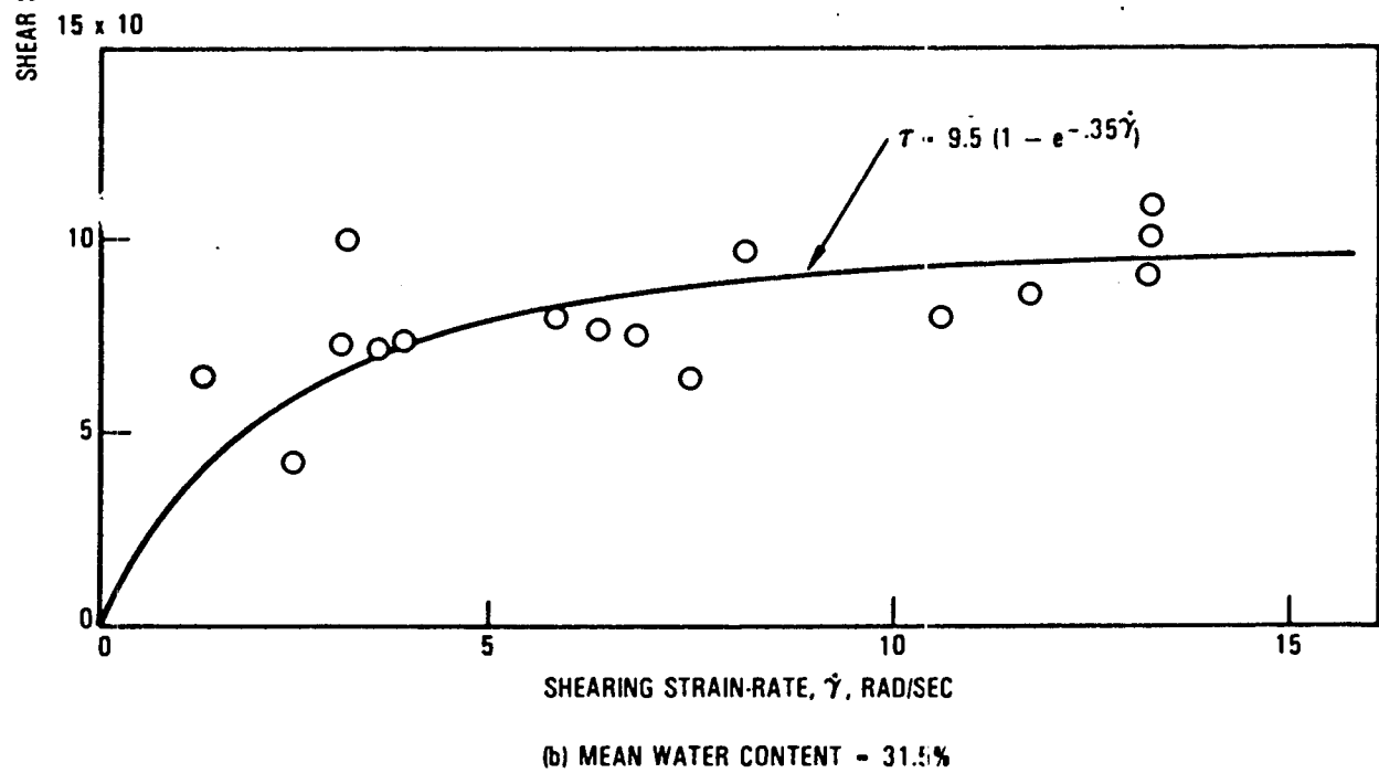
Figure B-3. Plot of Shearing Stress versus Strain Rate (Reference 1)
