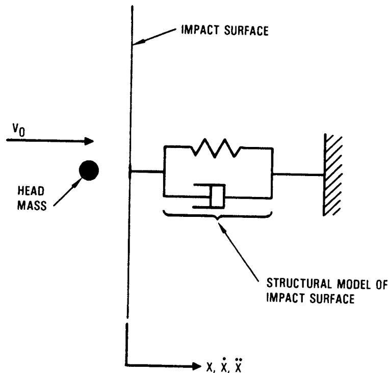
Figure 3-2. Head Impact Model
