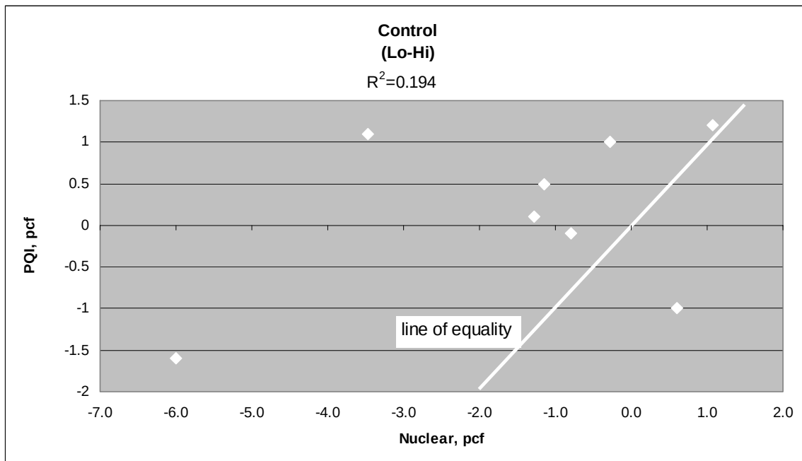
Figure 12 – Regression Analysis of Nuclear and PQI “Control” Data
