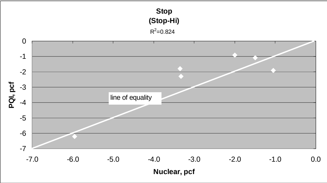
Figure 14 – Regression Analysis of Nuclear and PQI “Stop” Data
