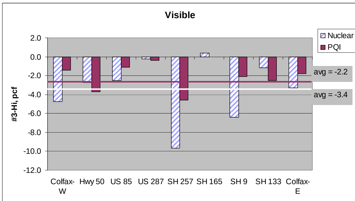
Figure 9- Nuclear and PQI Density Comparison for “Visible” Data
