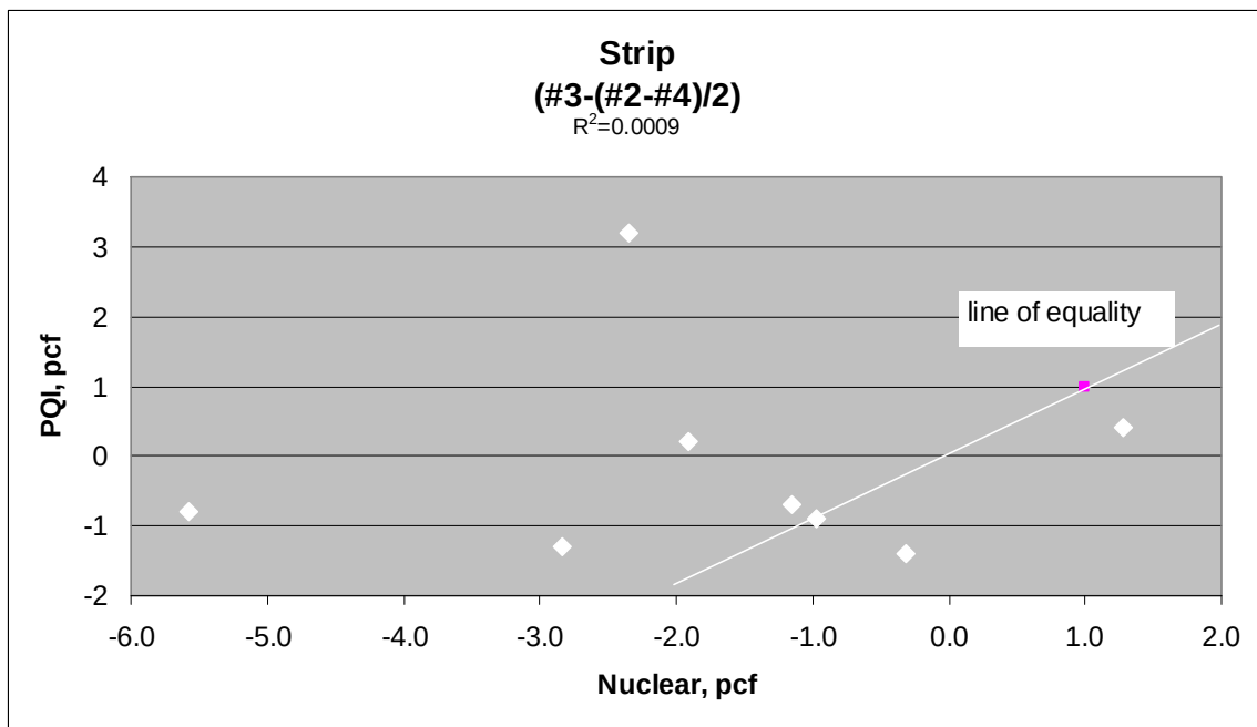
Figure 8 – Regression Analysis of Nuclear and PQI “Strip” Data
