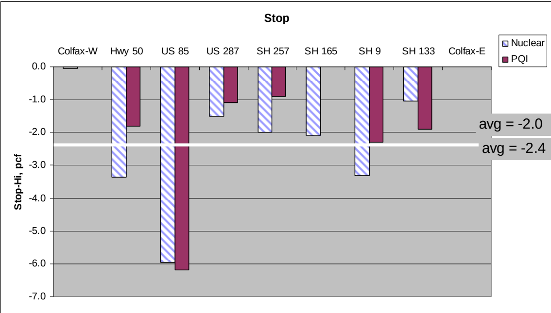
Figure 13- Nuclear and PQI Density Comparison for “Stop” Data
