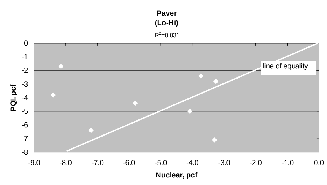
Figure 16 – Regression Analysis of Nuclear and PQI "Paver" Data
