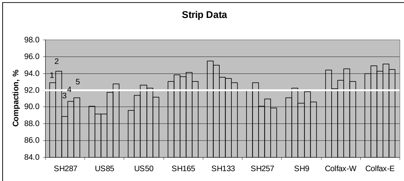
Figure 17 – Effect of Density Differences on Compaction for “Strip” Data Set
