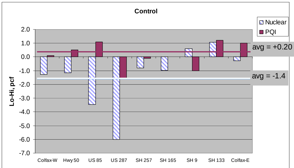
Figure 11- Nuclear and PQI Density Comparison for “Control” Data
