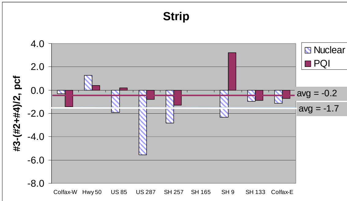
Figure 7- Nuclear and PQI Density Comparison for “Strip” Data
