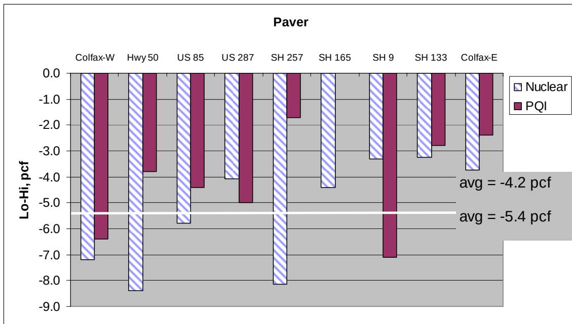
Figure 15- Nuclear and PQI Density Comparison for "Paver" Data
