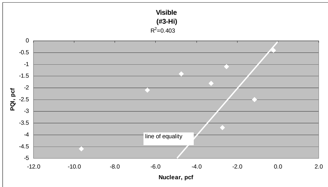
Figure 10 – Regression Analysis of Nuclear and PQI “Visible” Data
