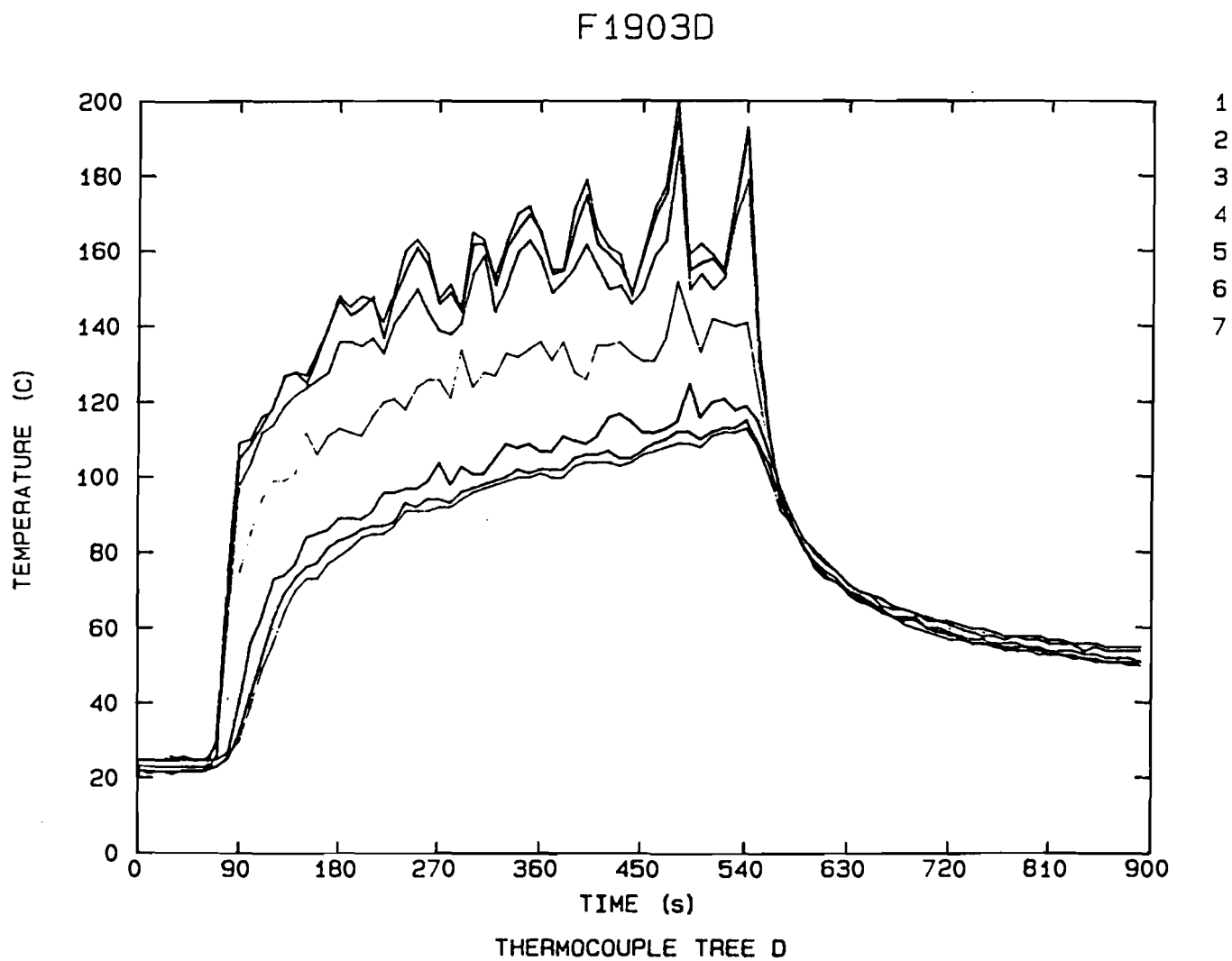
Fig. 31 Gas Temperature-Time Trace, TC Tree D, 40 kW Fire
