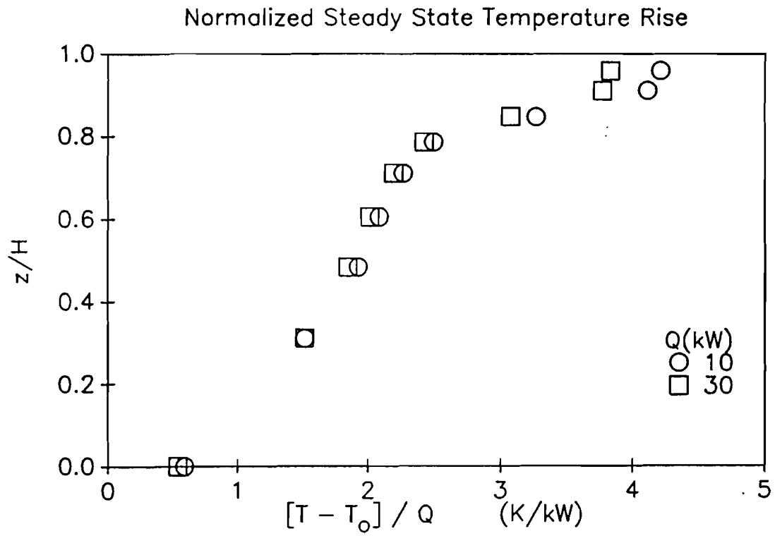
Fig. 4 Vertical Temperature Distribution
