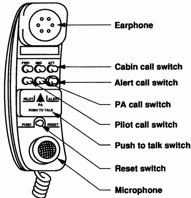
Figure 3-11. Communications Handset.
