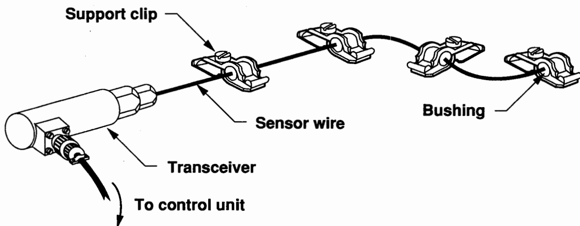
Figure 6-4. Schlumberger Acoustic Thermal Monitoring System.
