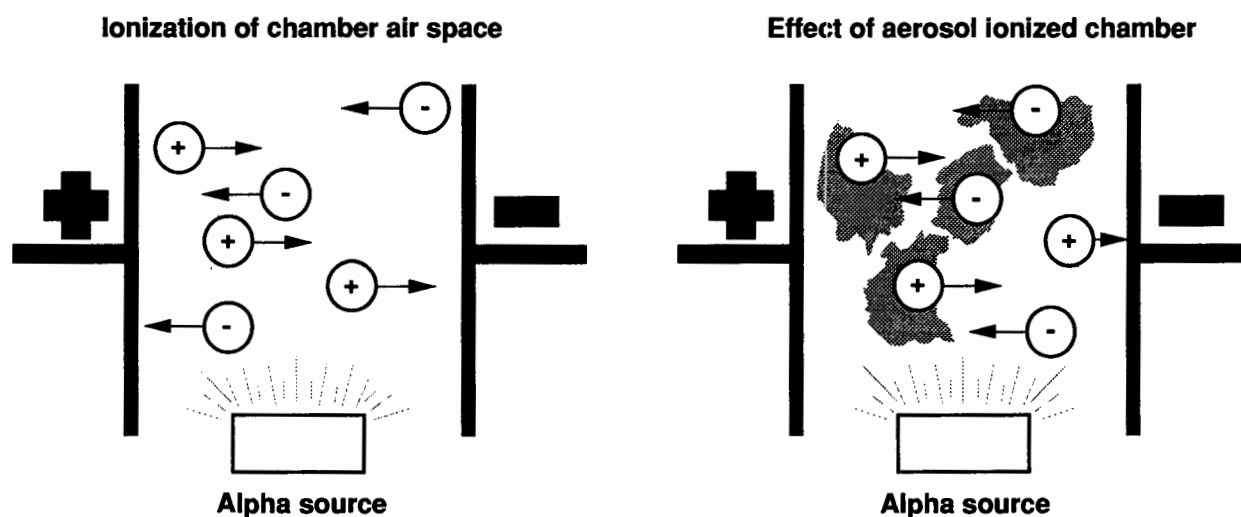
Figure 4-8. Ionization Detector.
