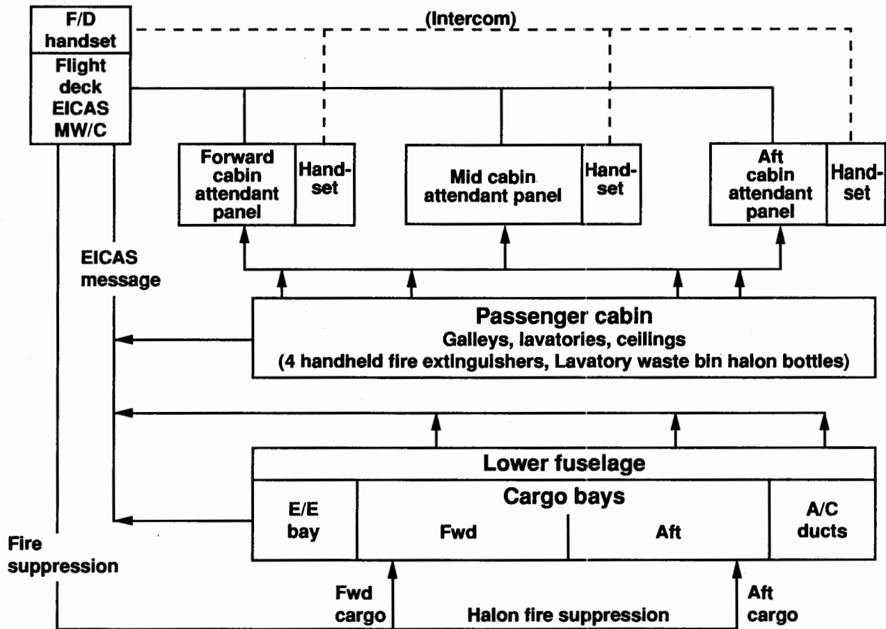
Figure 5-1. ACES Concept A.
