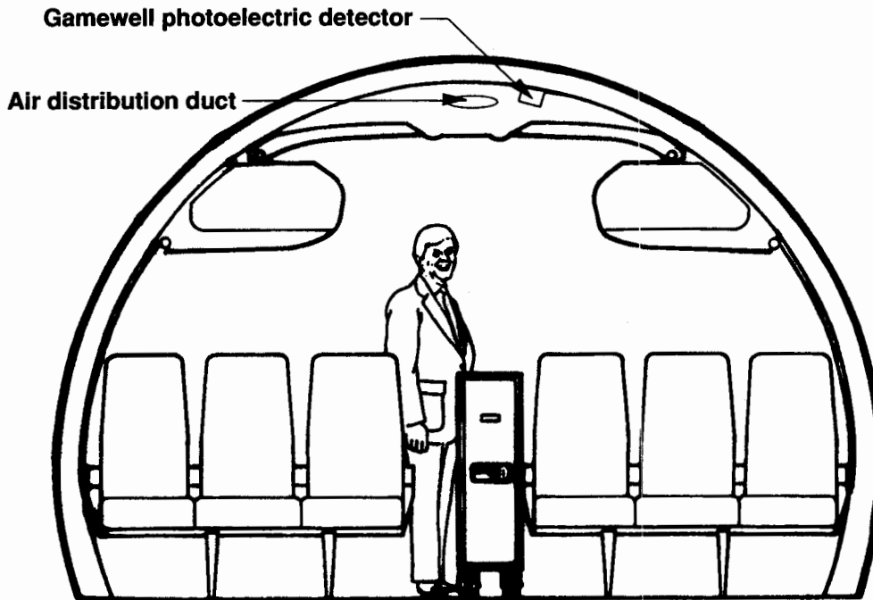
Figure 5-8. Attic Detectors.
