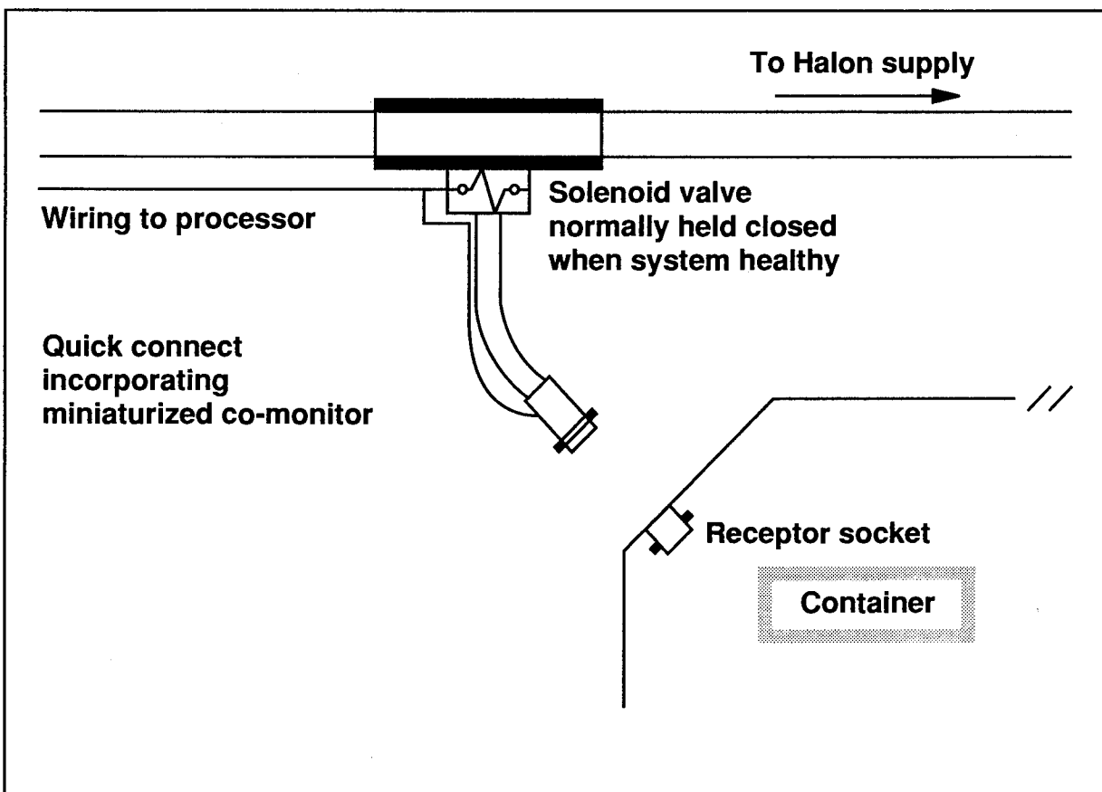
Figure 6-5. Pellex Combi/Freighter Smoke Detection System.
