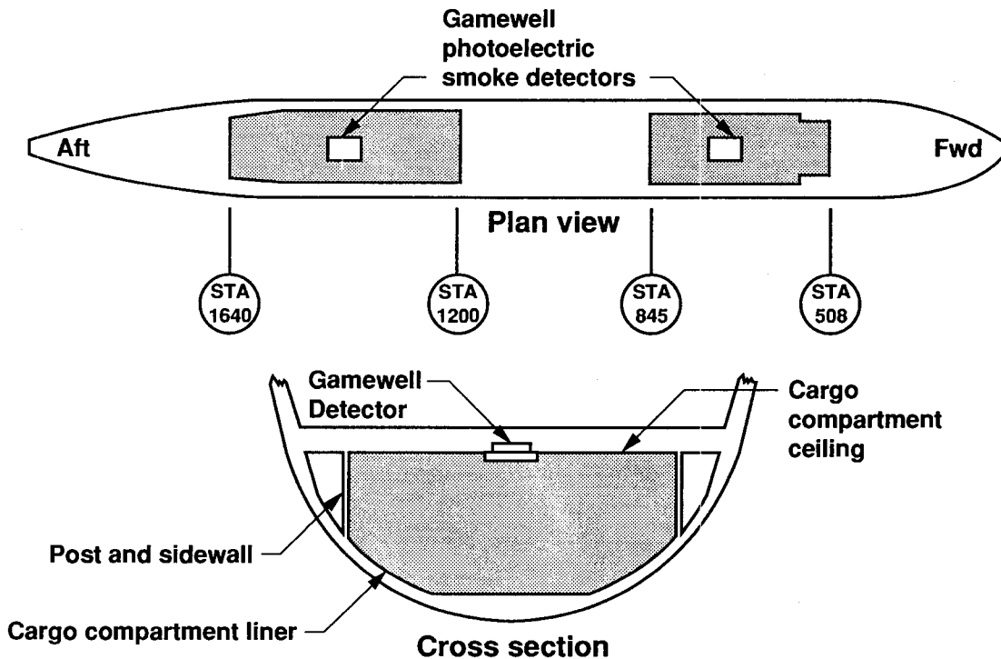
Figure 5-4. Lower Cargo Compartments.
