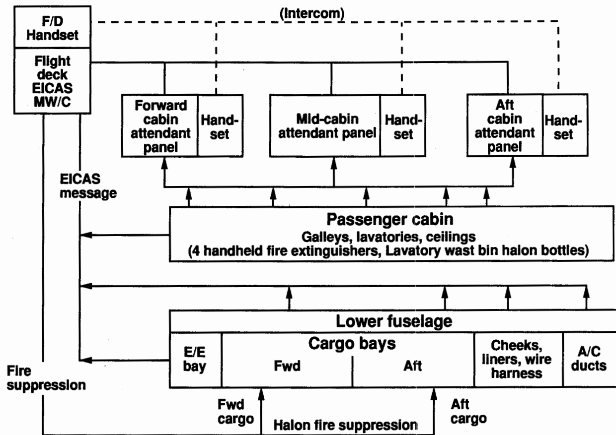
Figure 6 -1. ACES Concept B.
