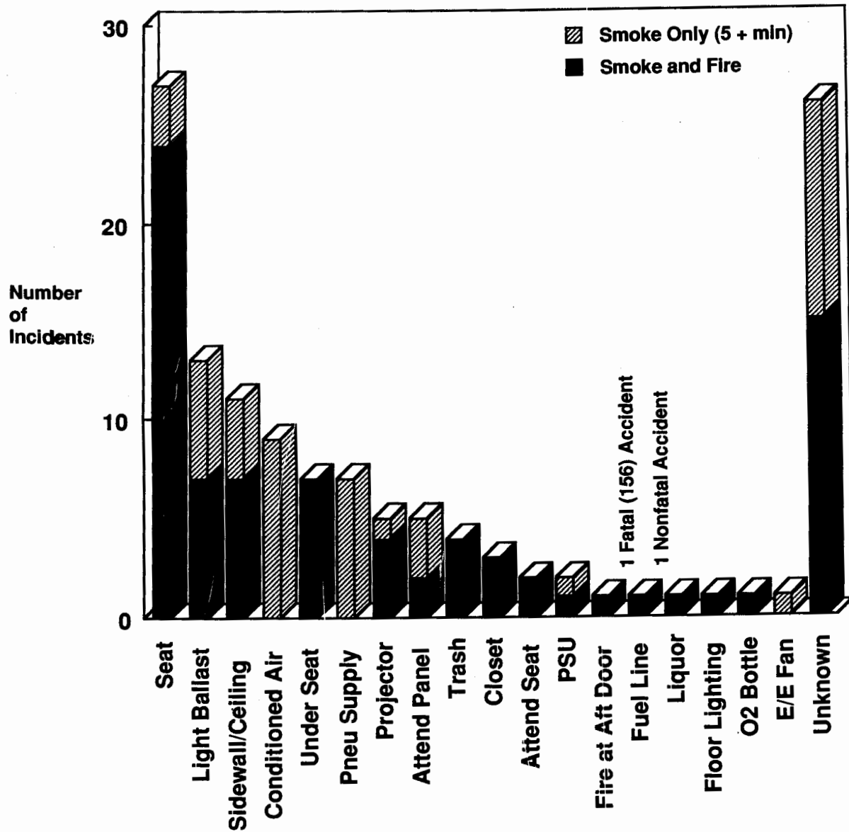
Figure 4-4. Passenger Cabin – Inflight Smoke/Fire Incidents.
