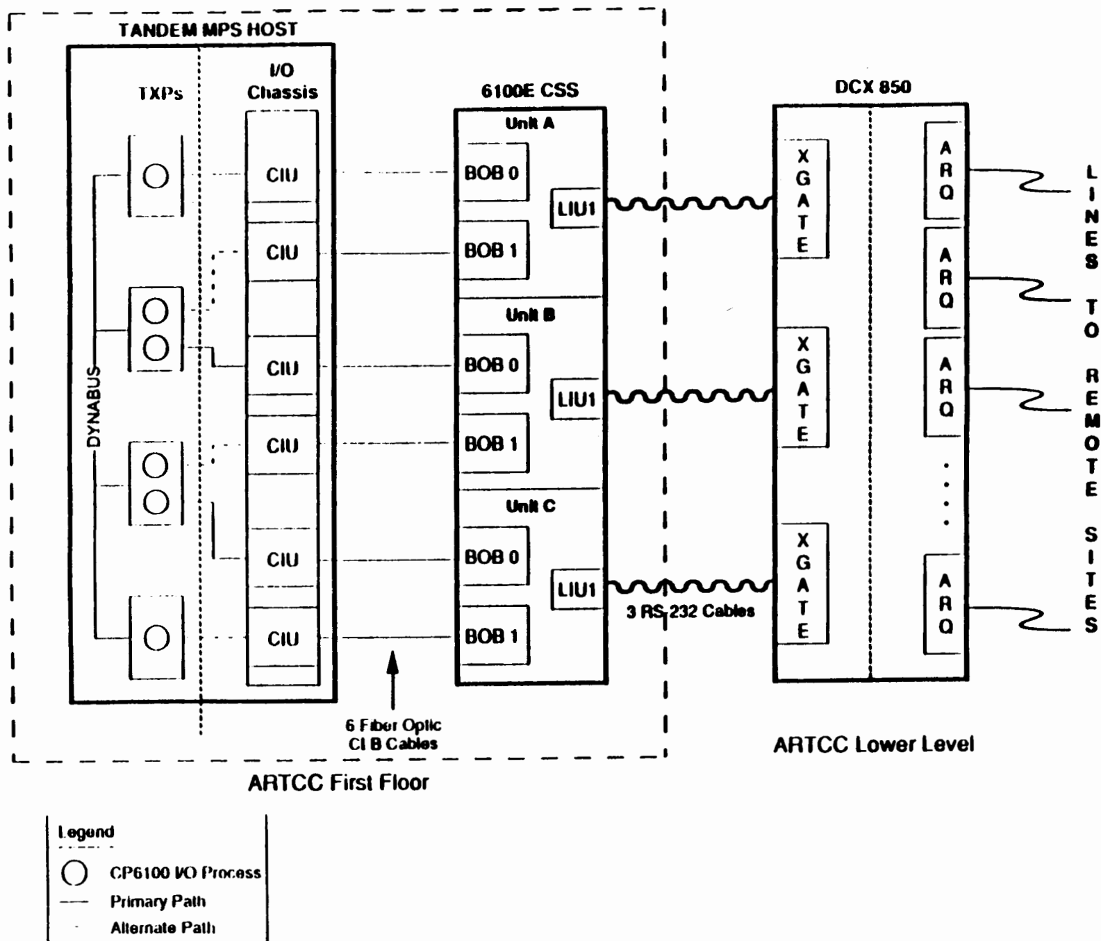
FIGURE 3-3. X.25 INTERFACE/6100E CSS ALTERNATIVE
