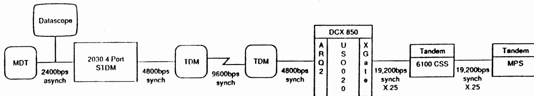
c) X.25/6100 CSS
