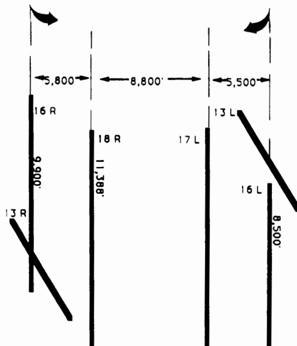
FIGURE 7. GRAPHICAL REPRESENTATION OF THE CONDITIONS IN THE RUNWAY THREATENED ANALYSES
