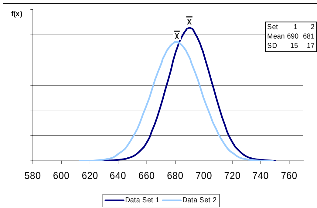
Figure 1. Example: Passing Results for both the F and t Tests.
