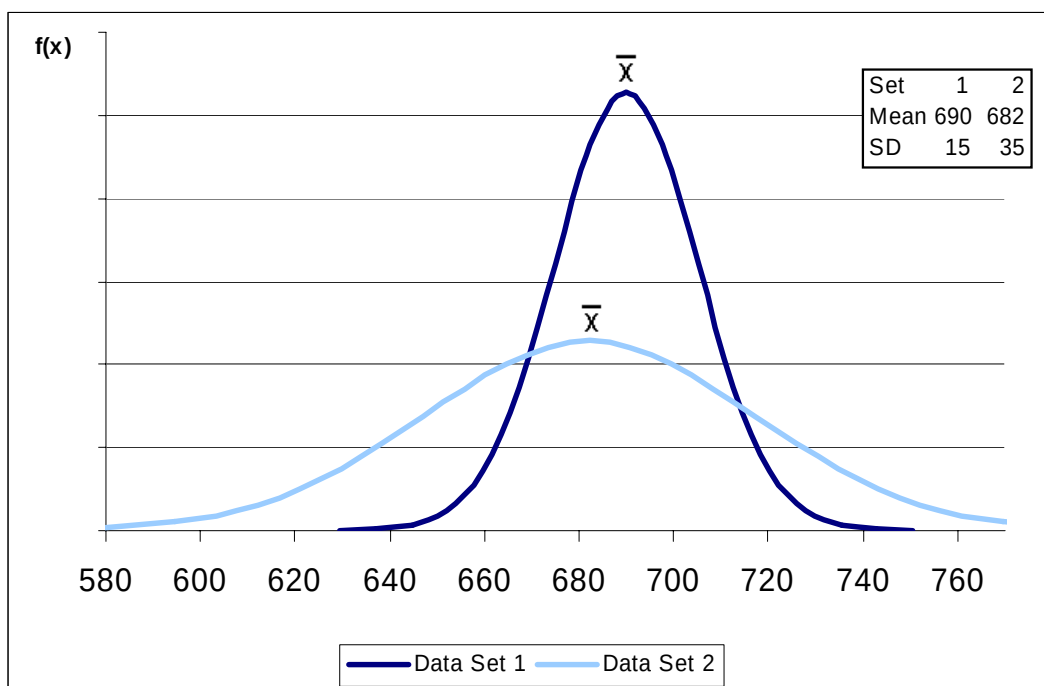
Figure 2. Example: F Test Showing Significant Difference, Standard Deviations
